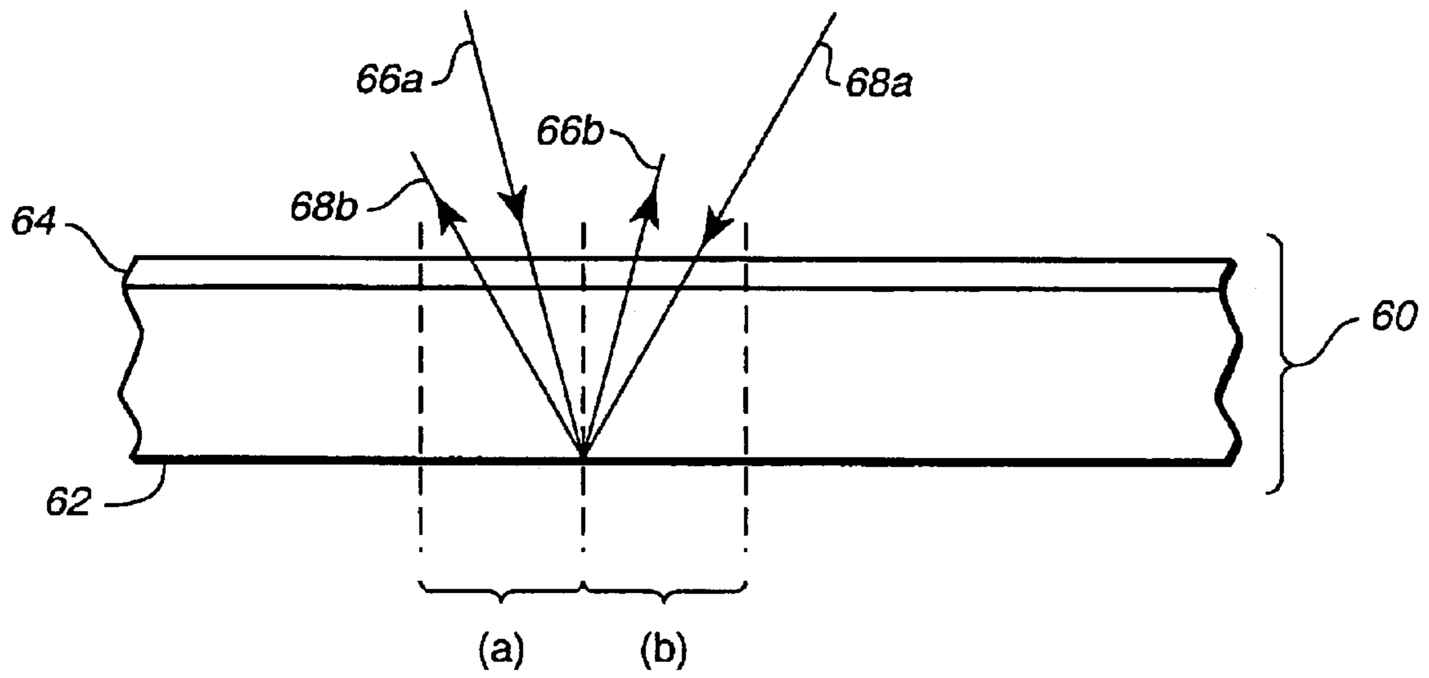
FIG. 3 (PRIOR ART)
