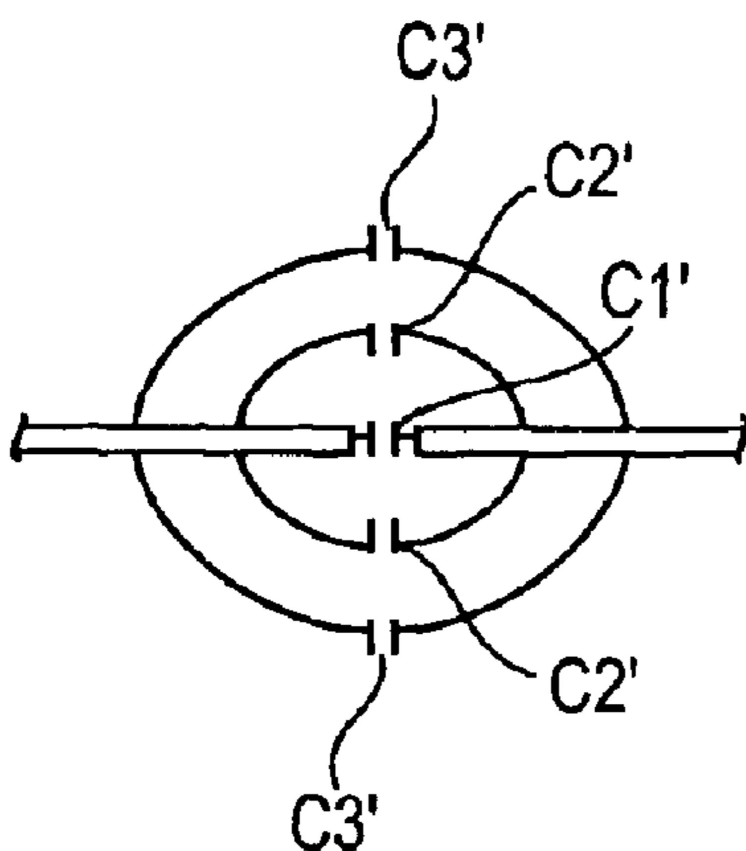
FIG. 19C PRIOR ART
