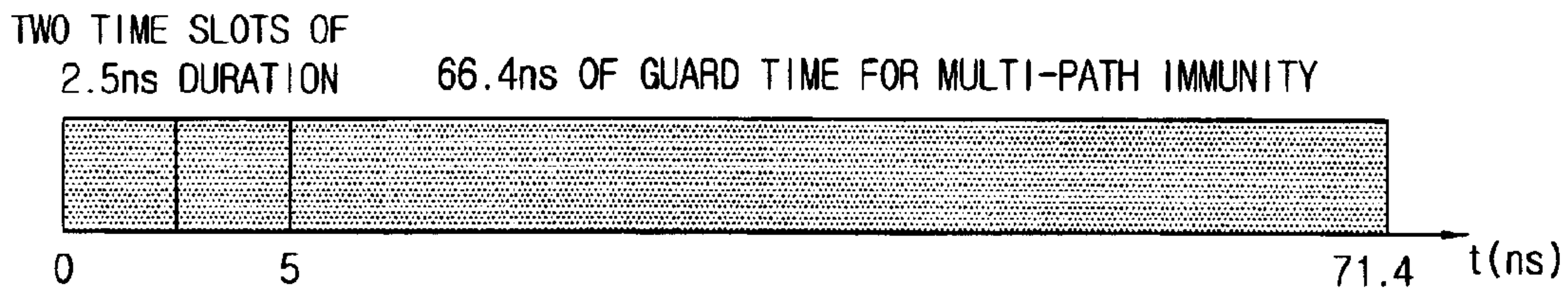
BINARY PPM-APPLIED TIME FRAME STRUCTURE
