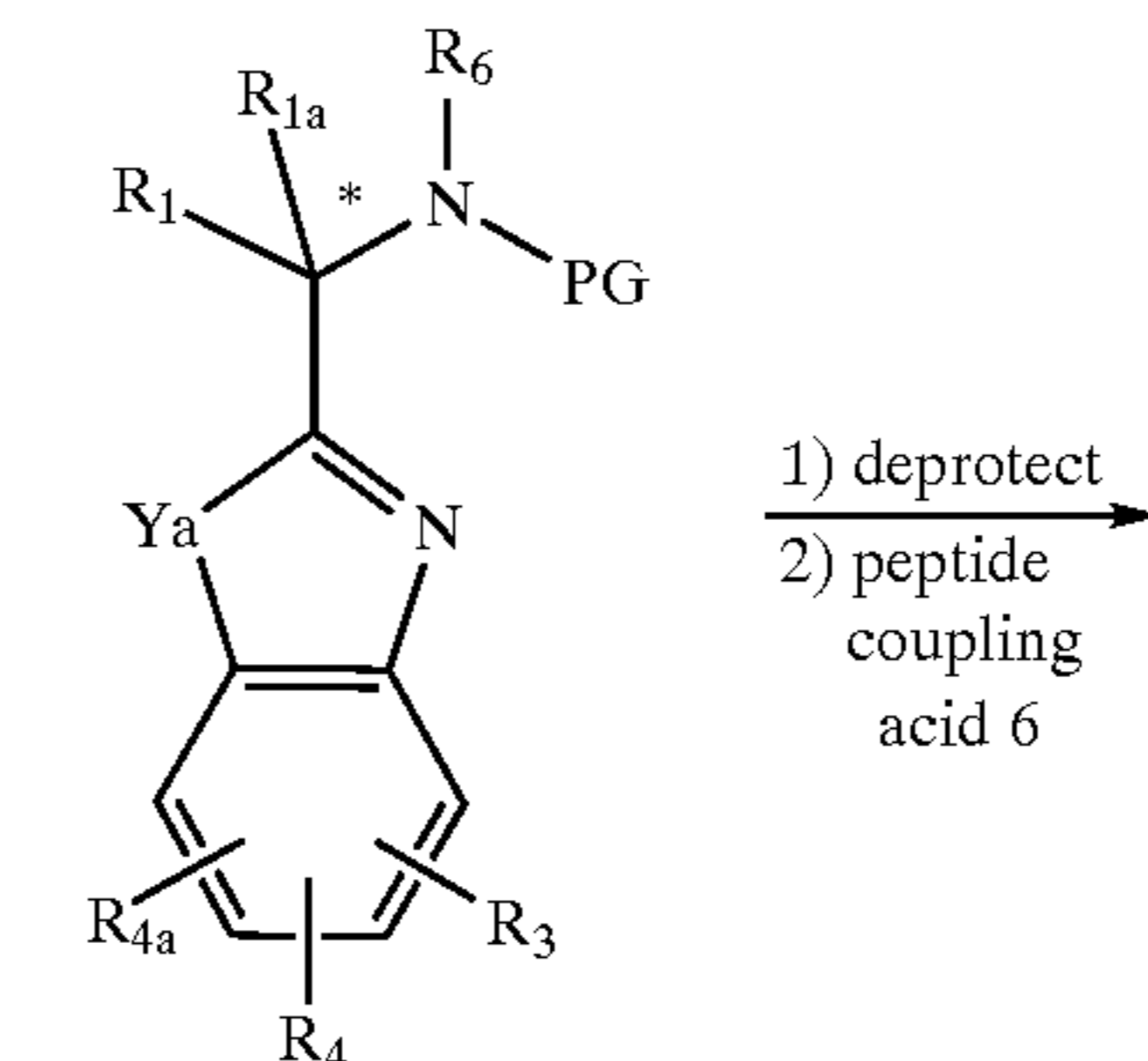
Scheme 1d
