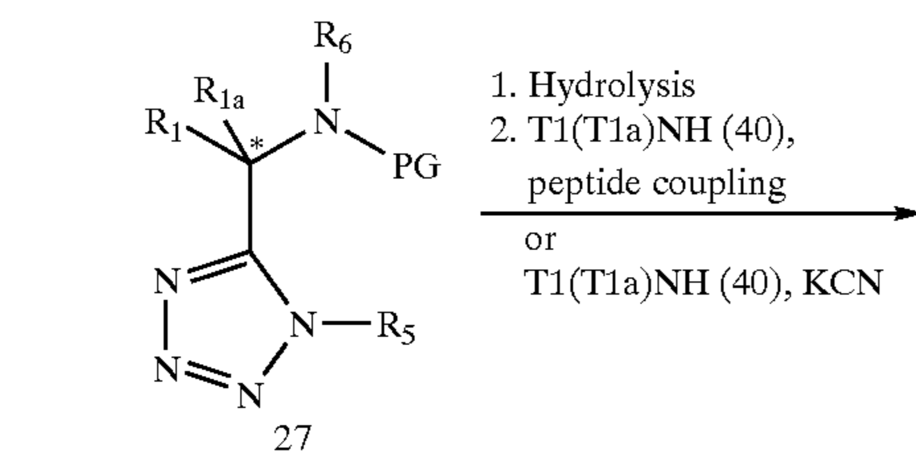
Scheme 3c
