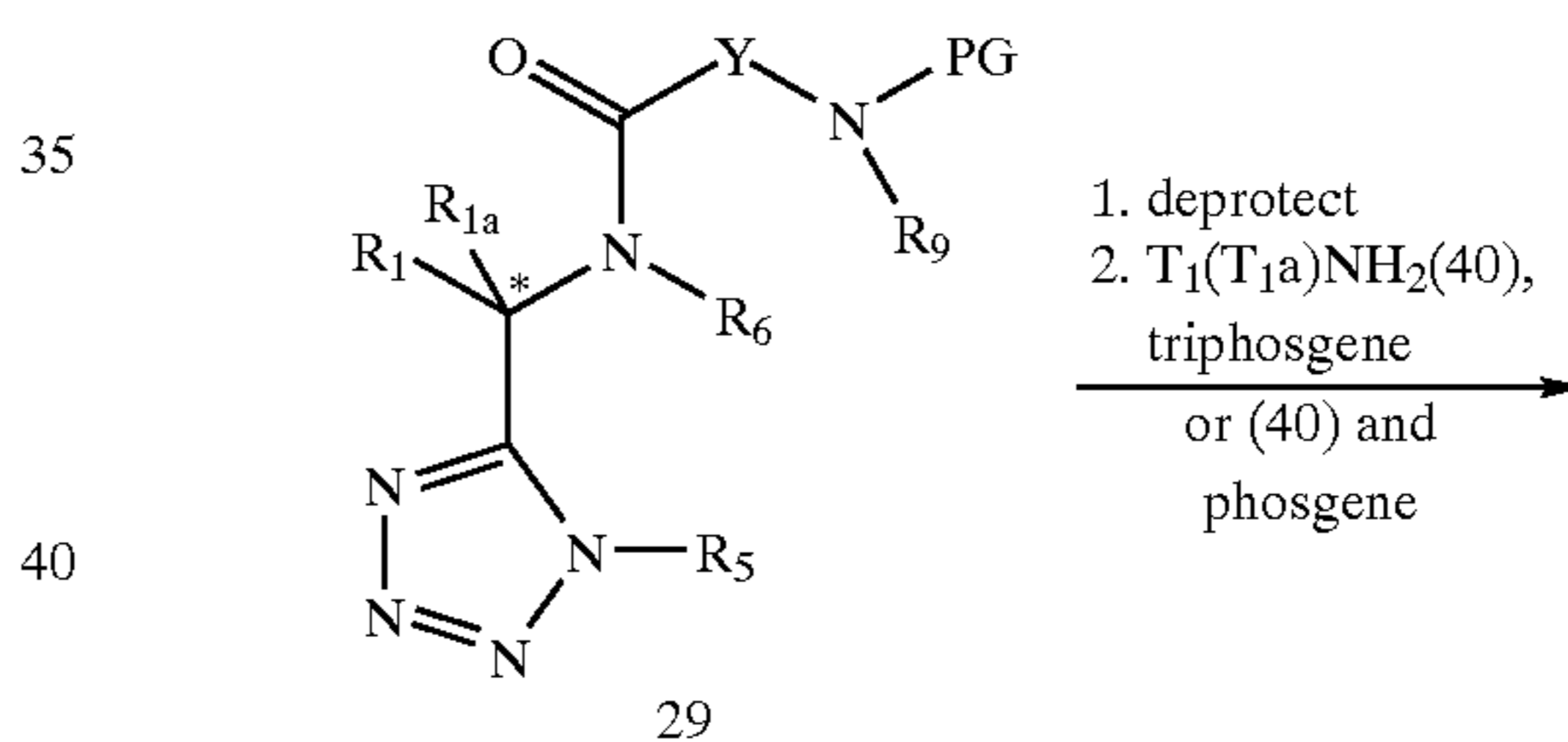
Scheme 3f
