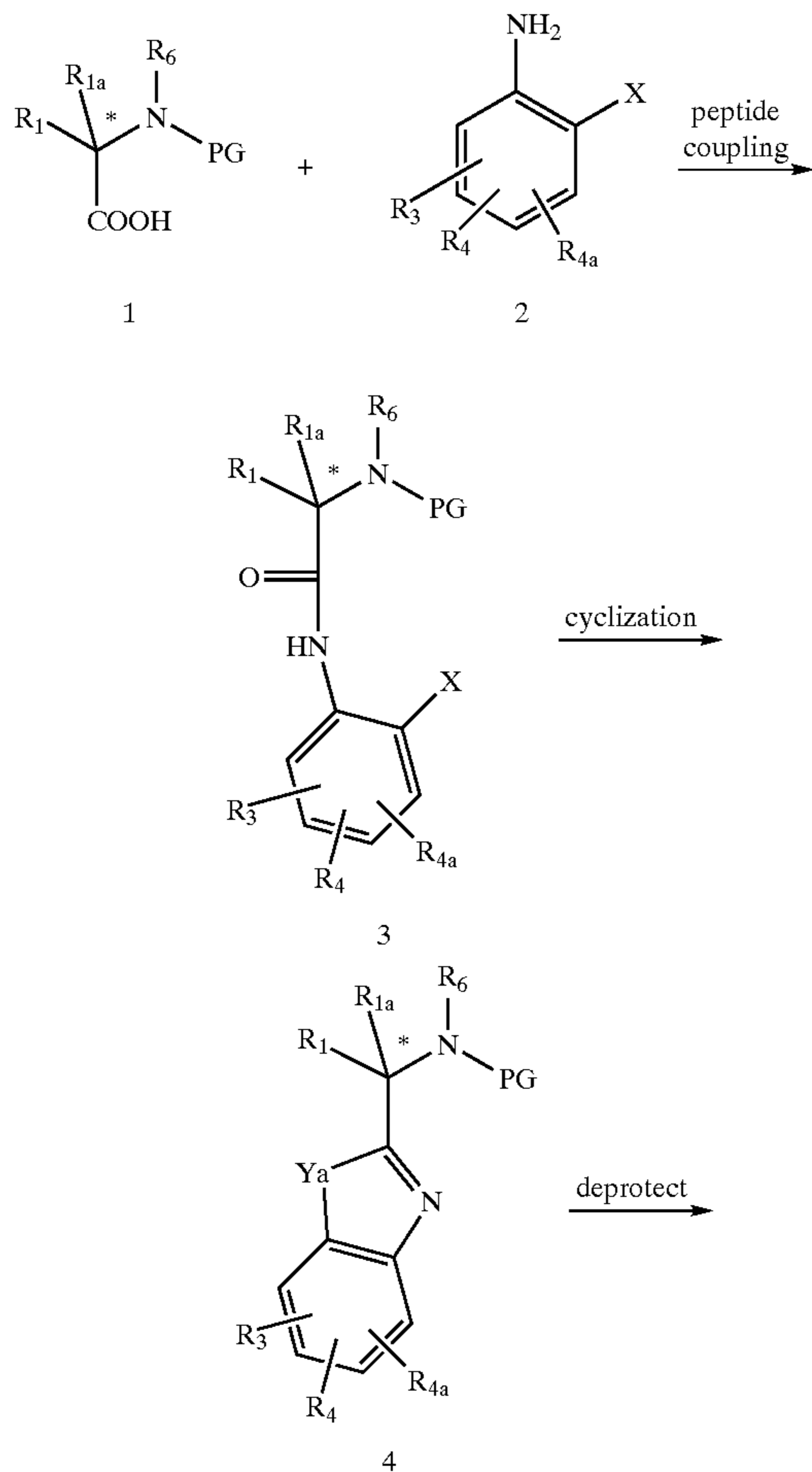
Scheme 1
