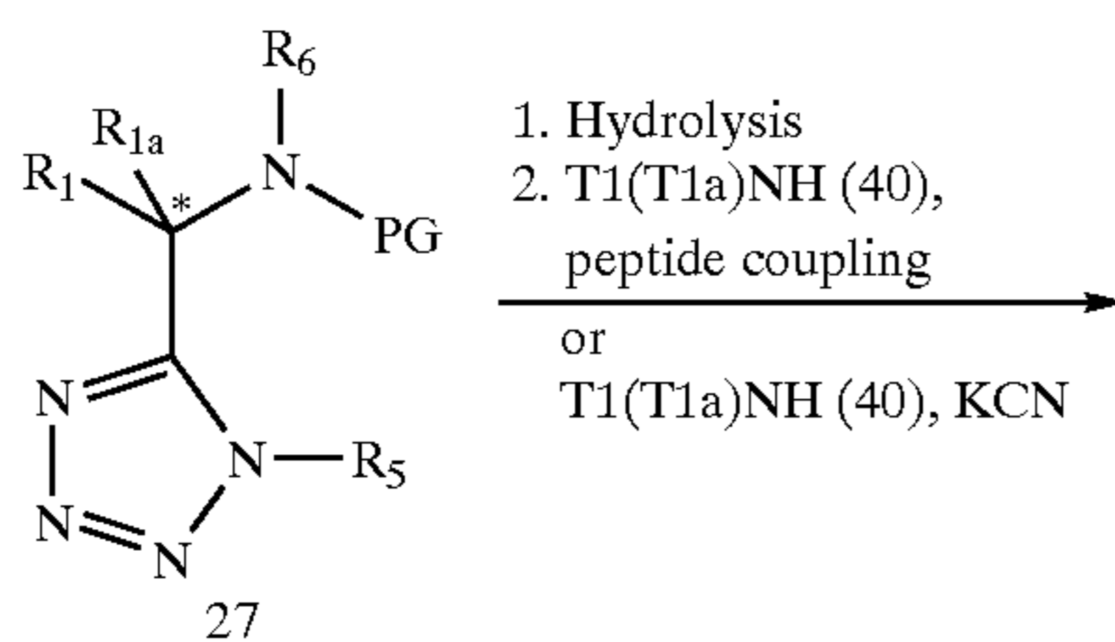
Scheme 3c
