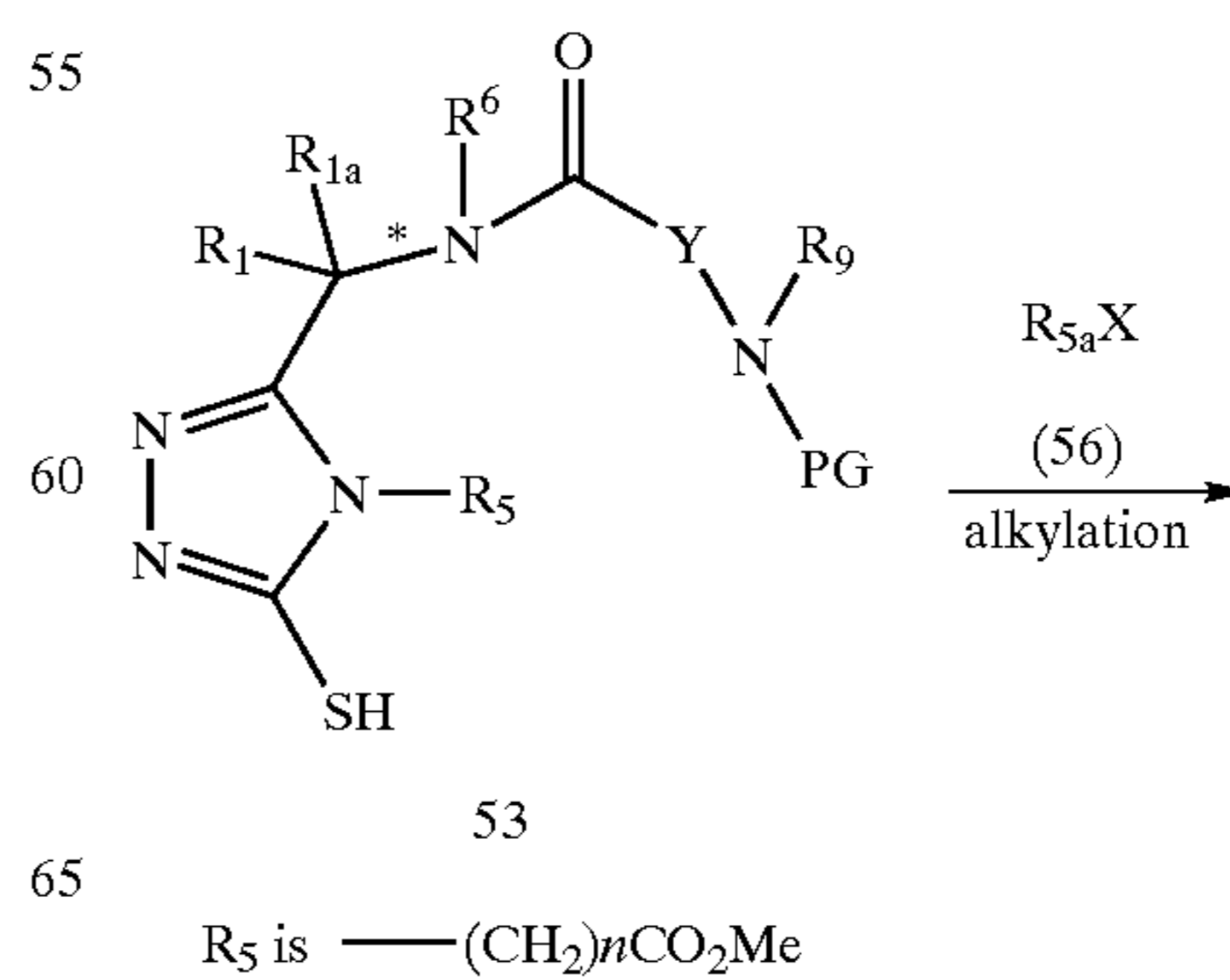
Scheme 4d
