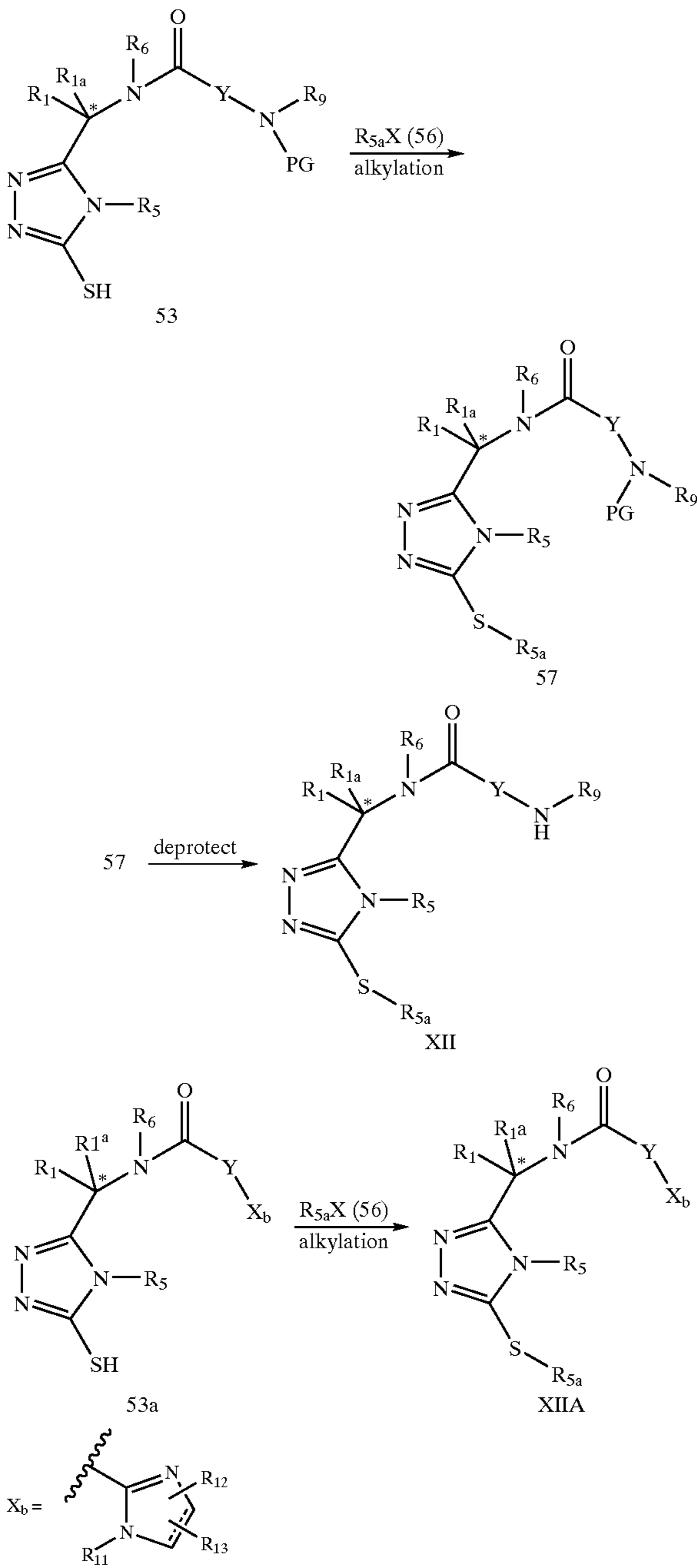
Scheme 4b
