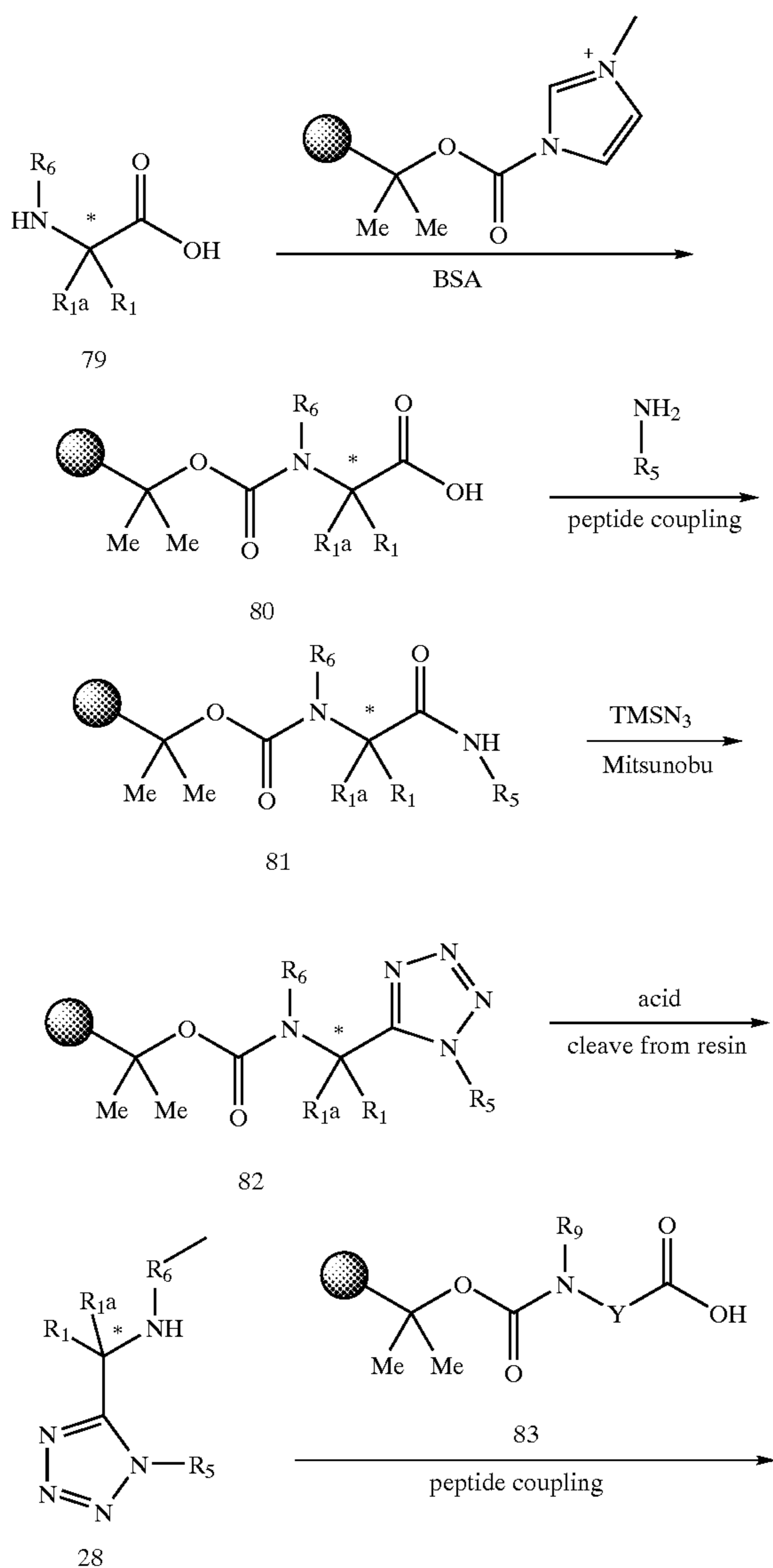
Scheme 6:
