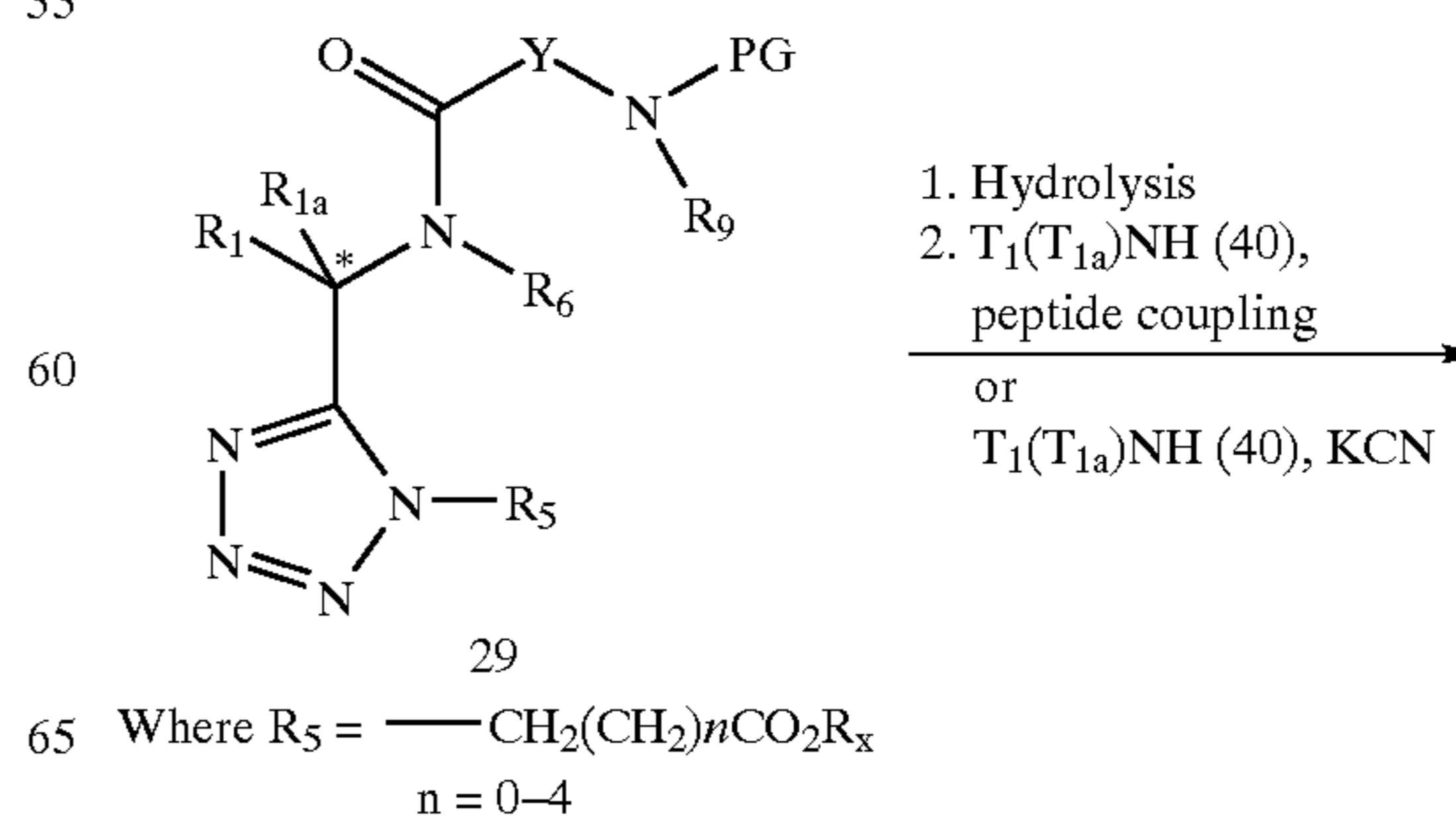
Scheme 3d
