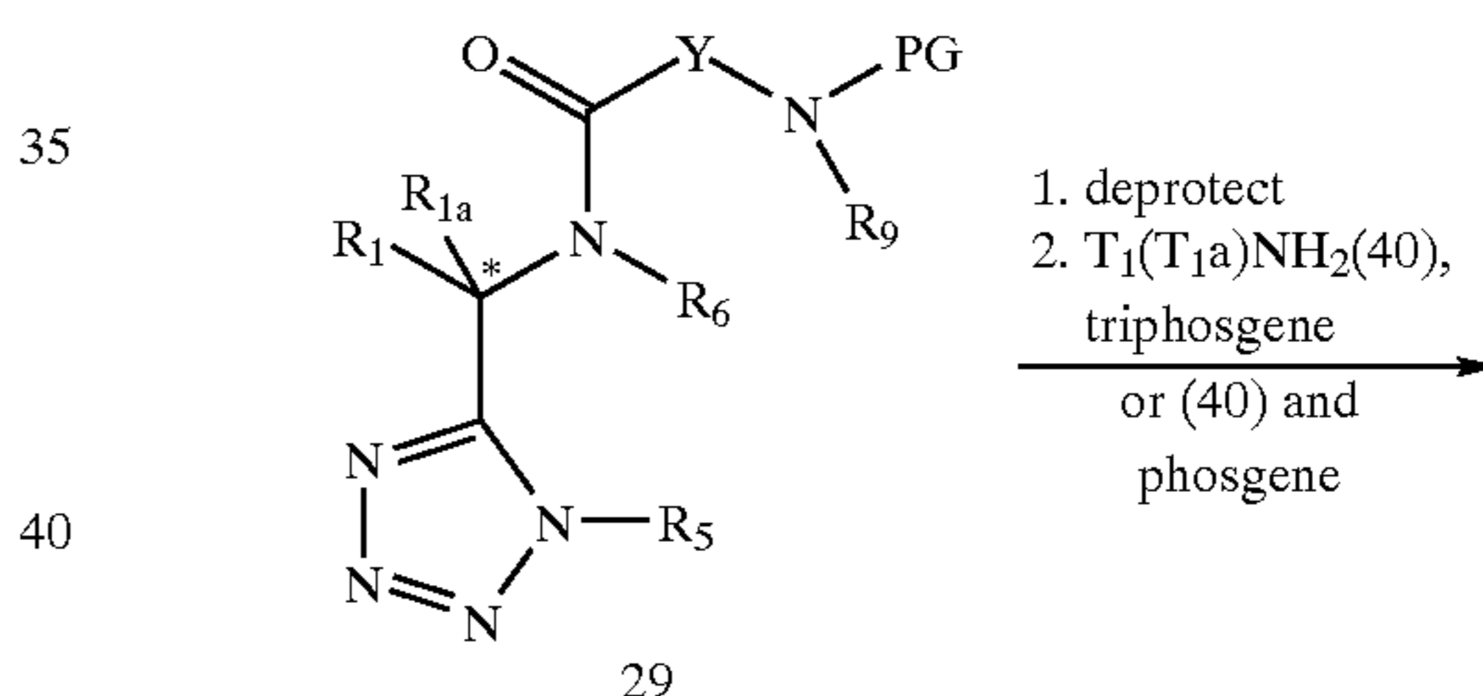
Scheme 3f
