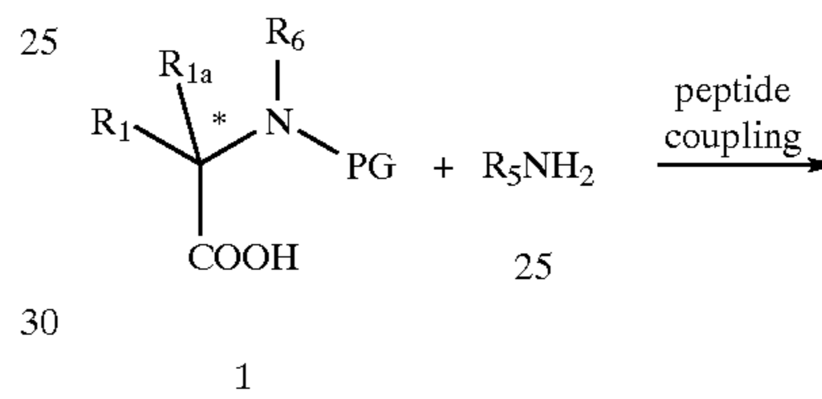
Scheme 3: Tetrazole
