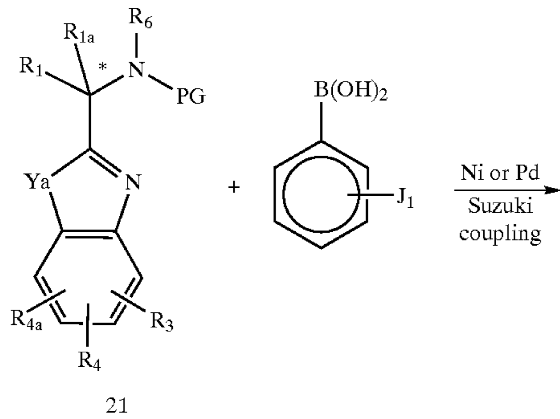
Scheme 2
