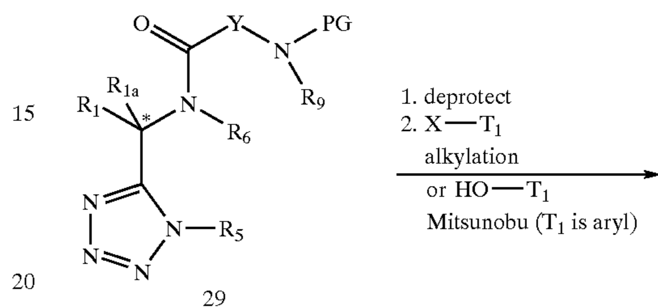
Scheme 3h
