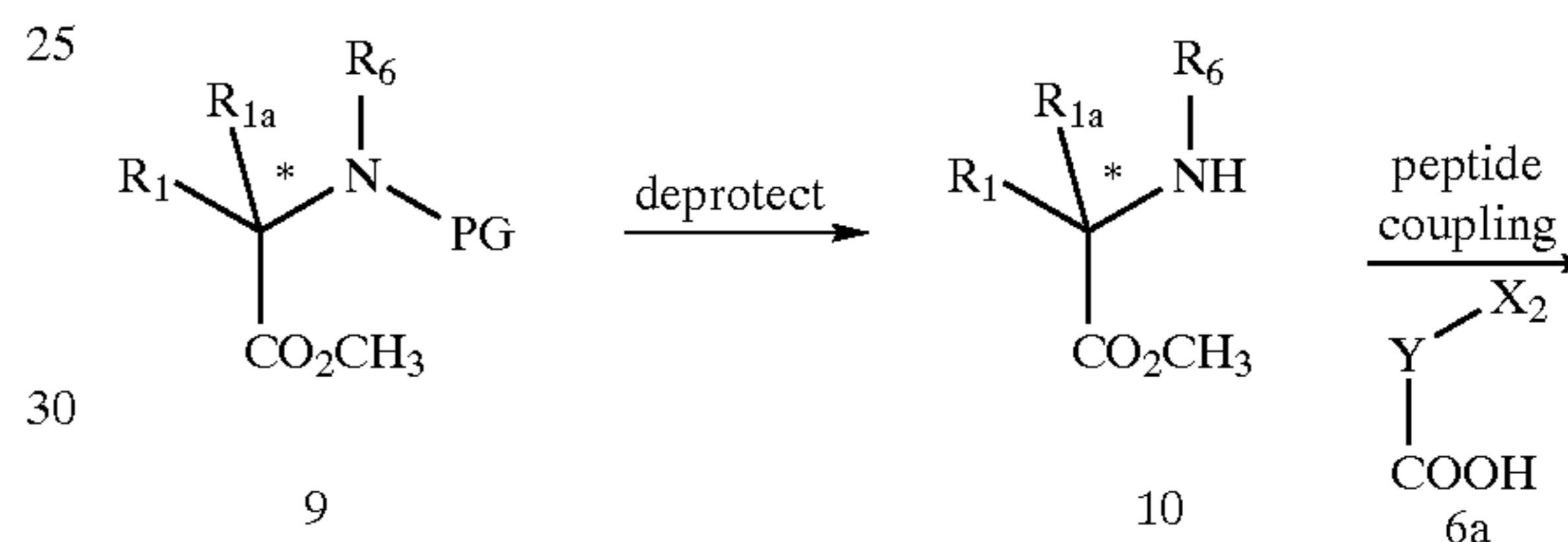
Scheme 1b
