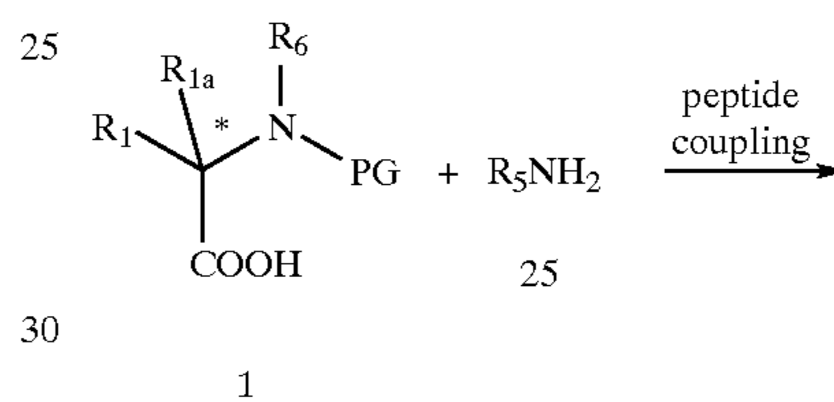
Scheme 3: Tetrazole
