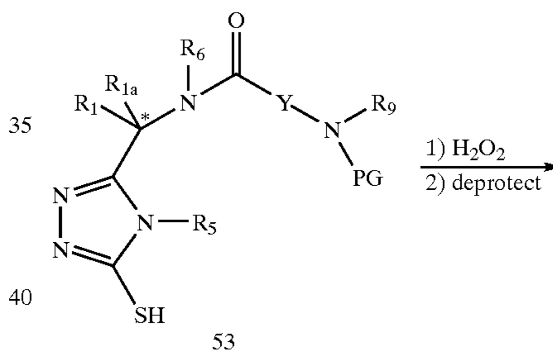
Scheme 4a
