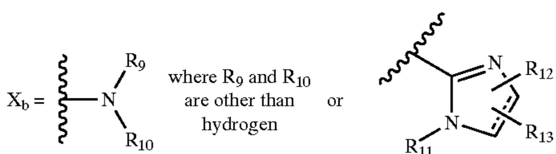
Scheme 3c
