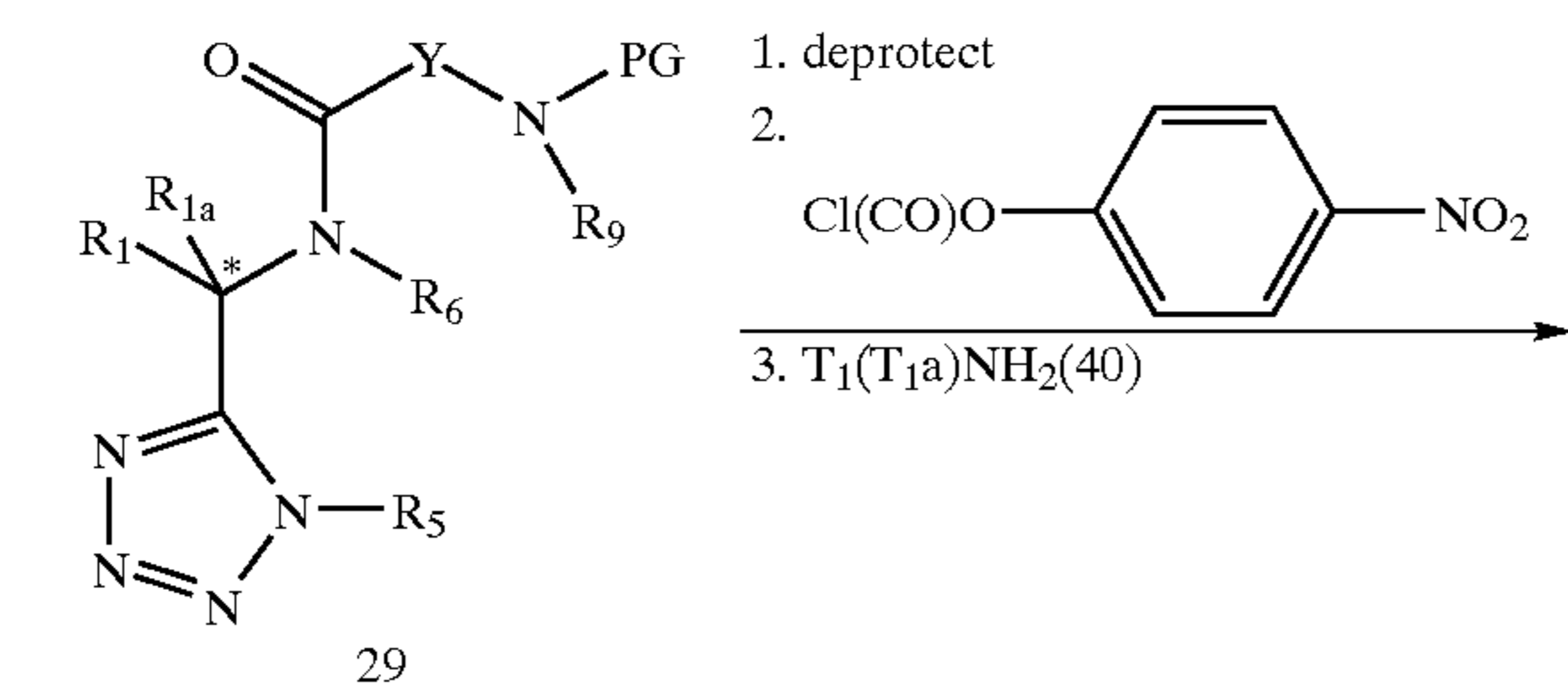
Scheme 3g
