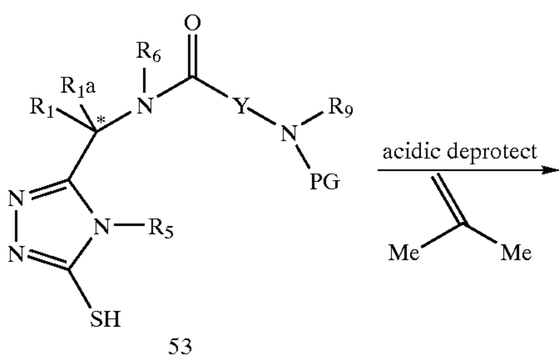
Scheme 4c
