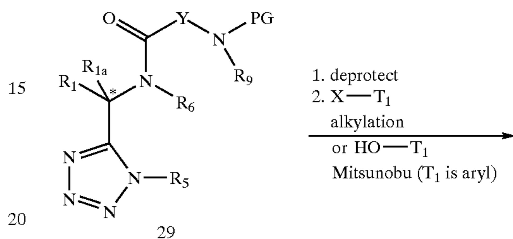
Scheme 3h
