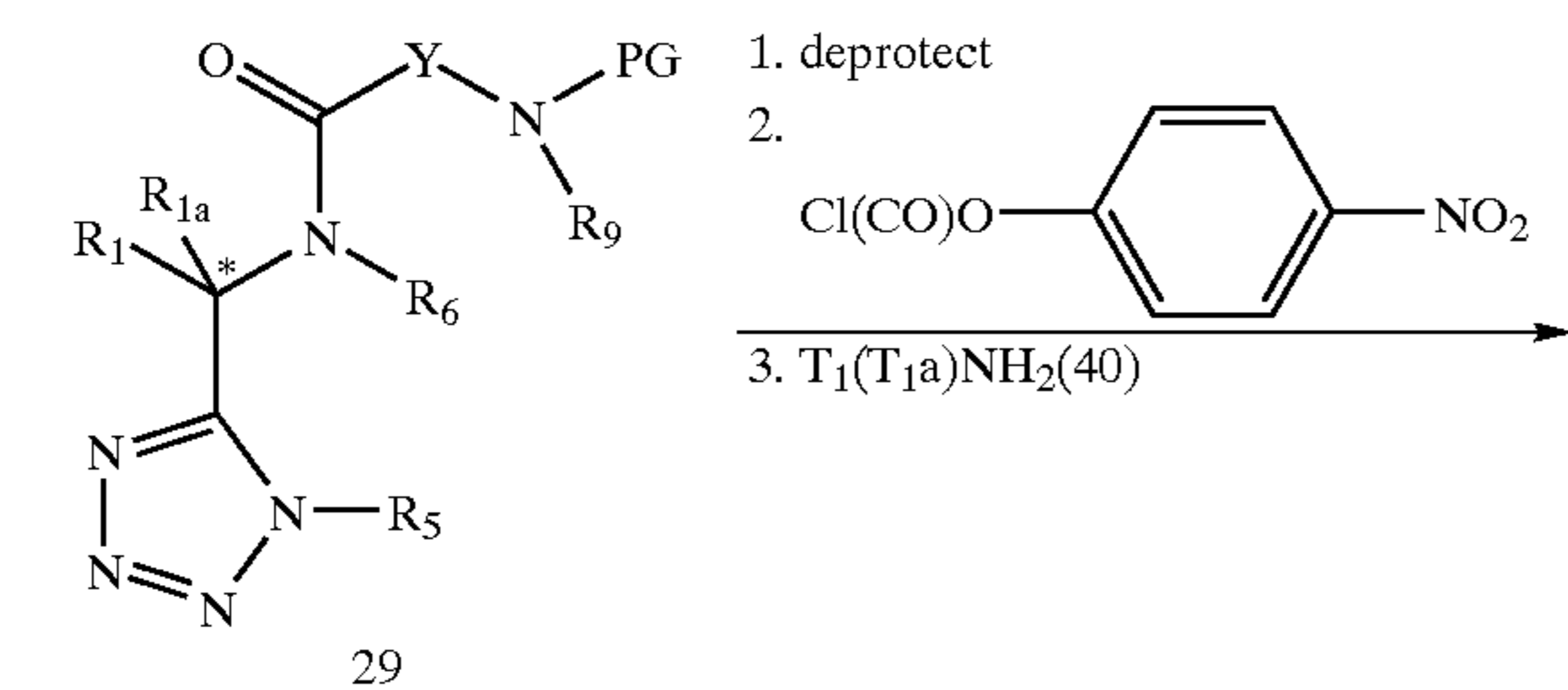
Scheme 3g
