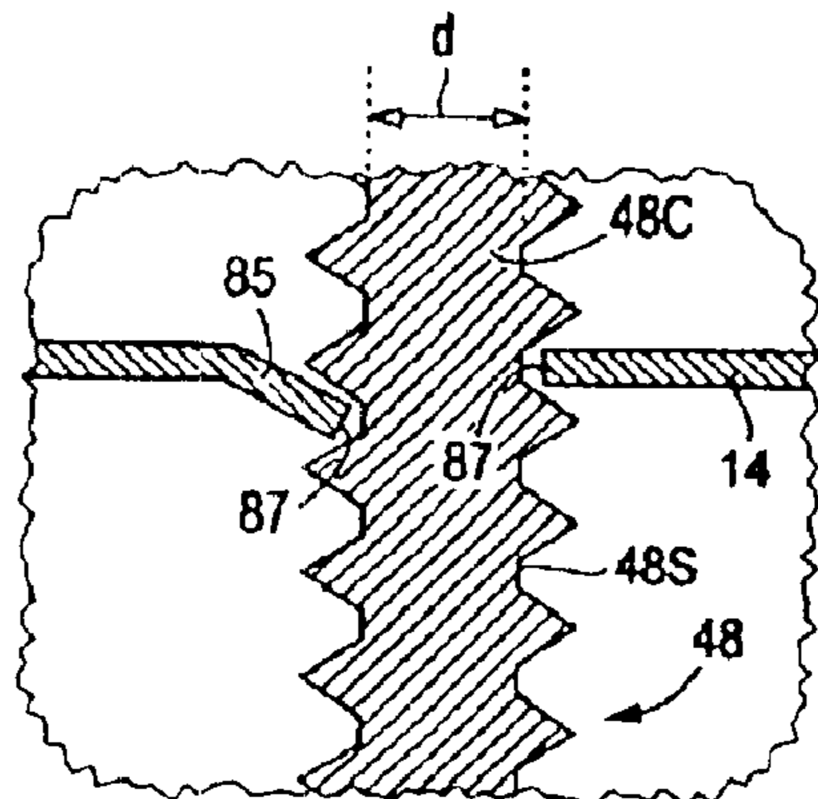
FIG. 18 PRIOR ART
