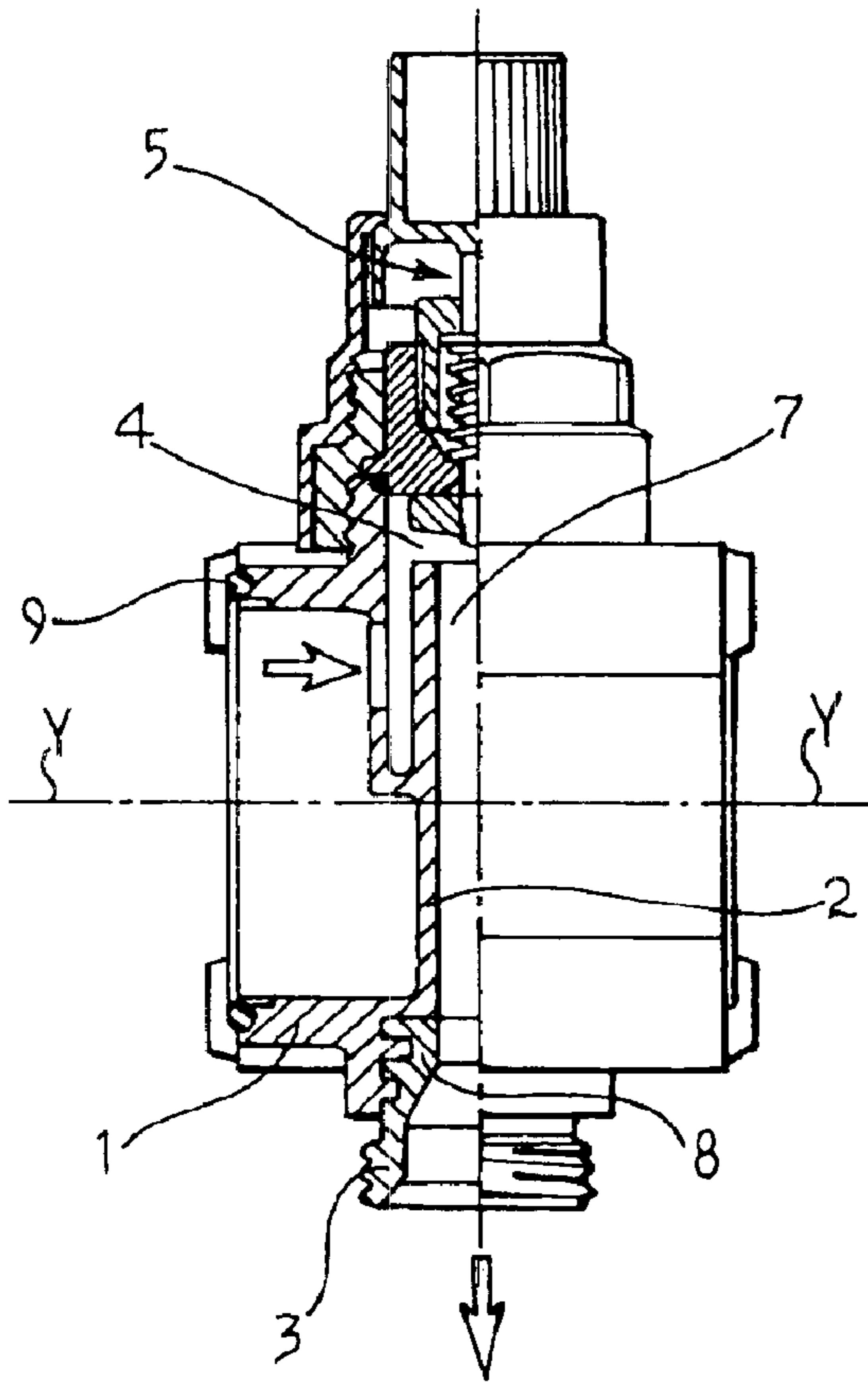
FIG. 1 (PRIOR ART)
