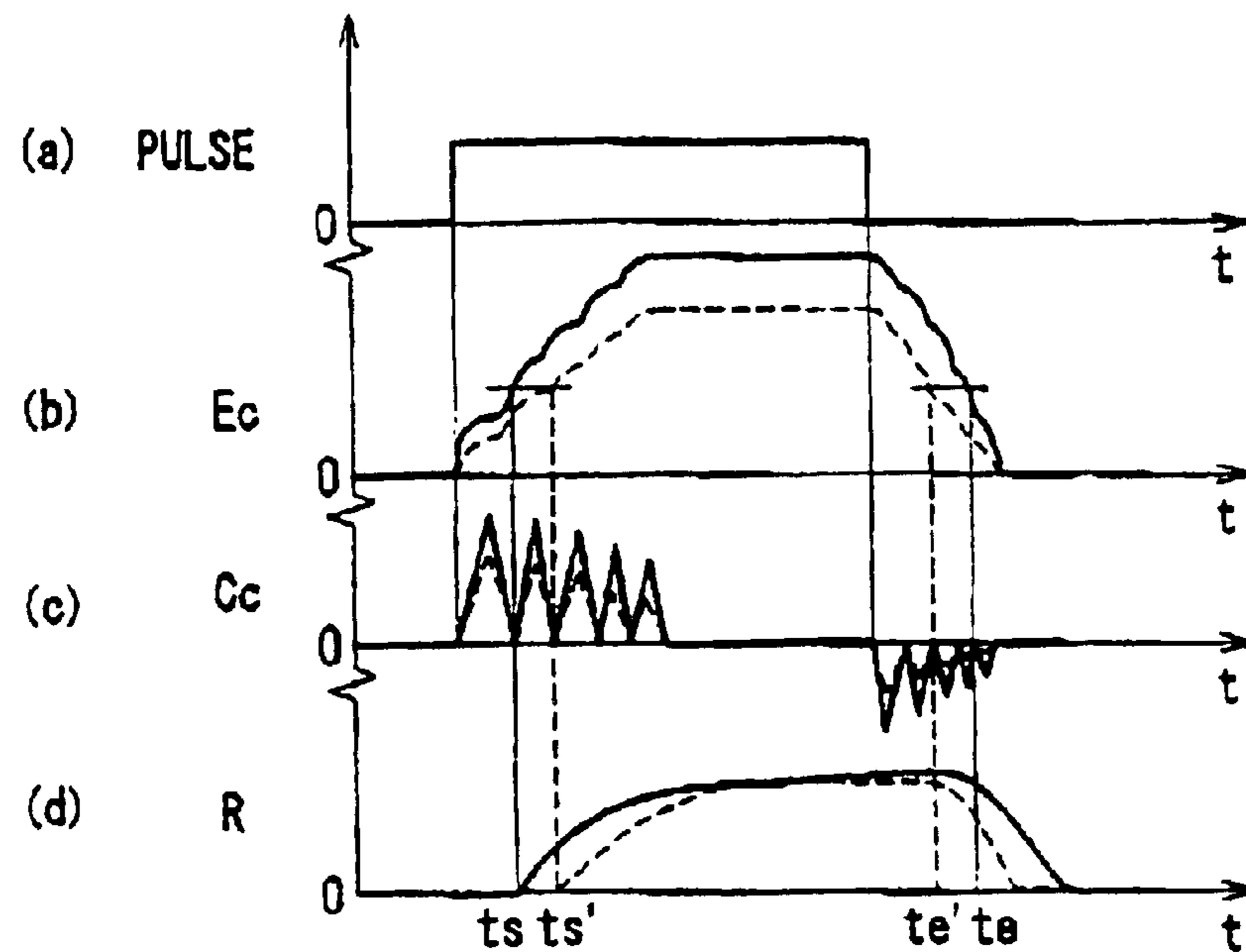
FIG. 9 RELATED ART
