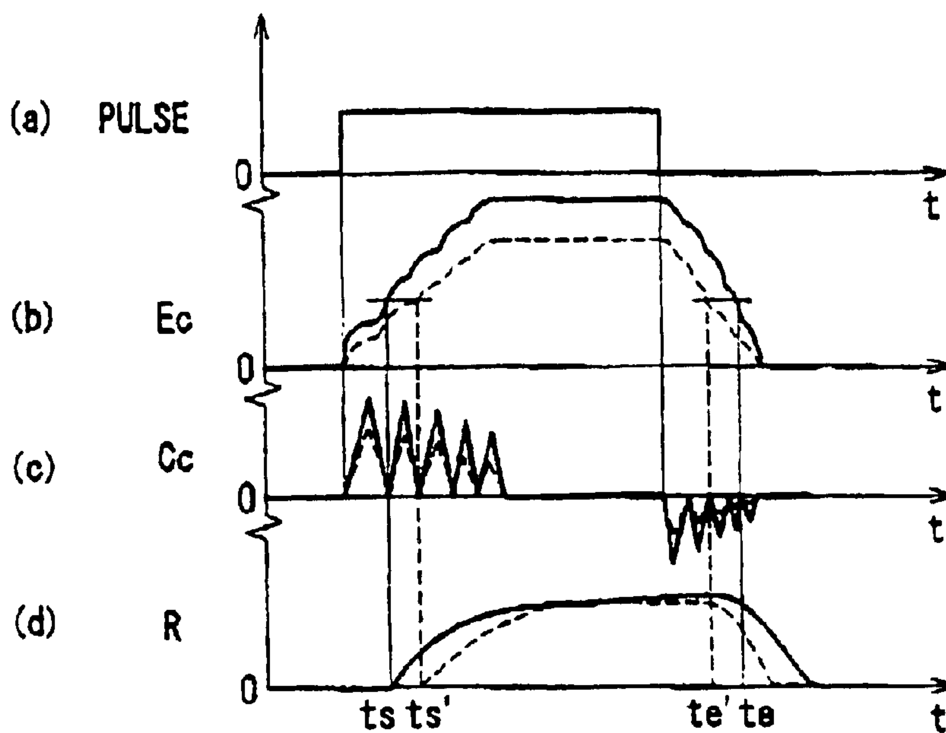
FIG. 9 RELATED ART
