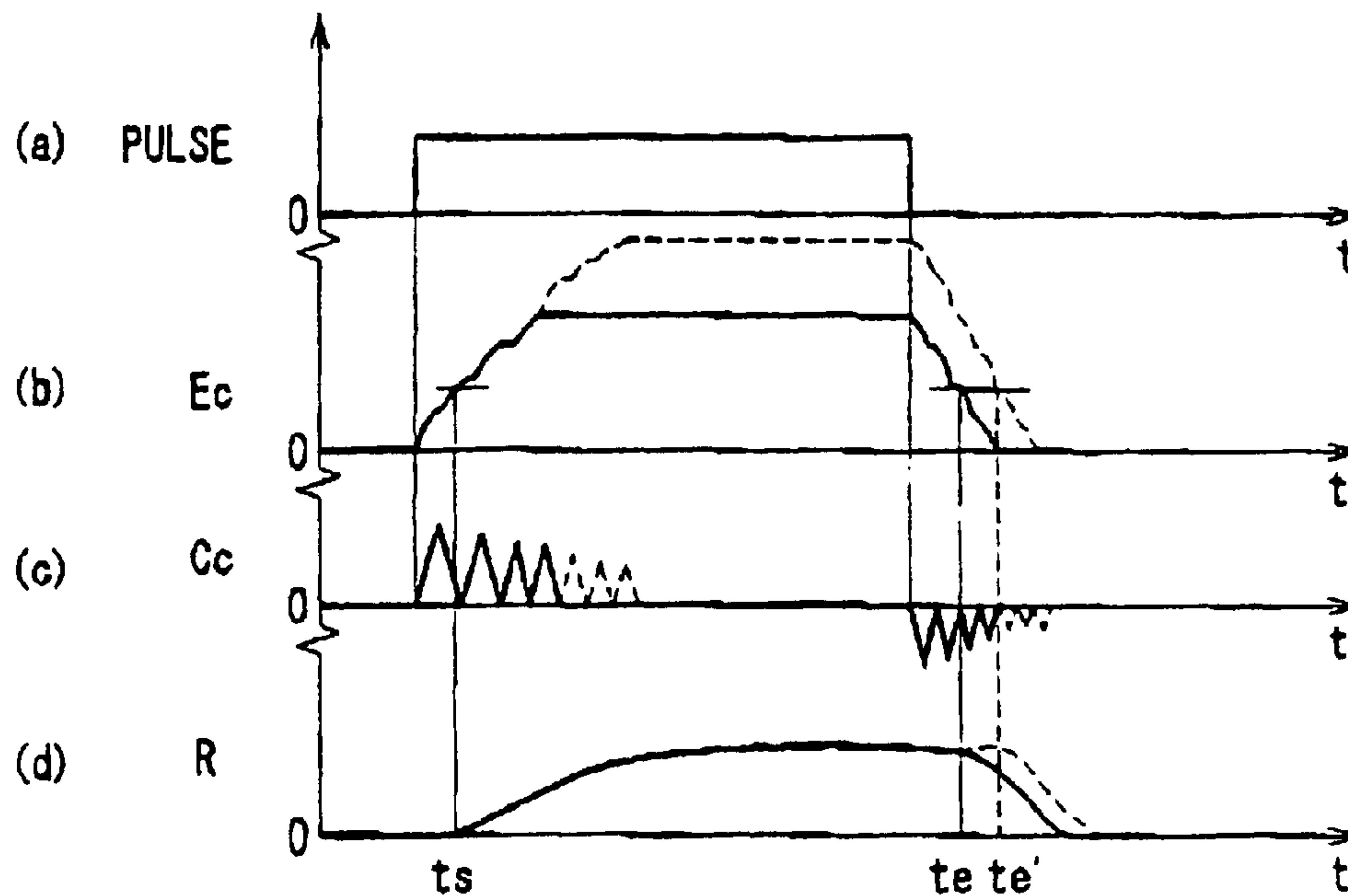
FIG. 8 RELATED ART
