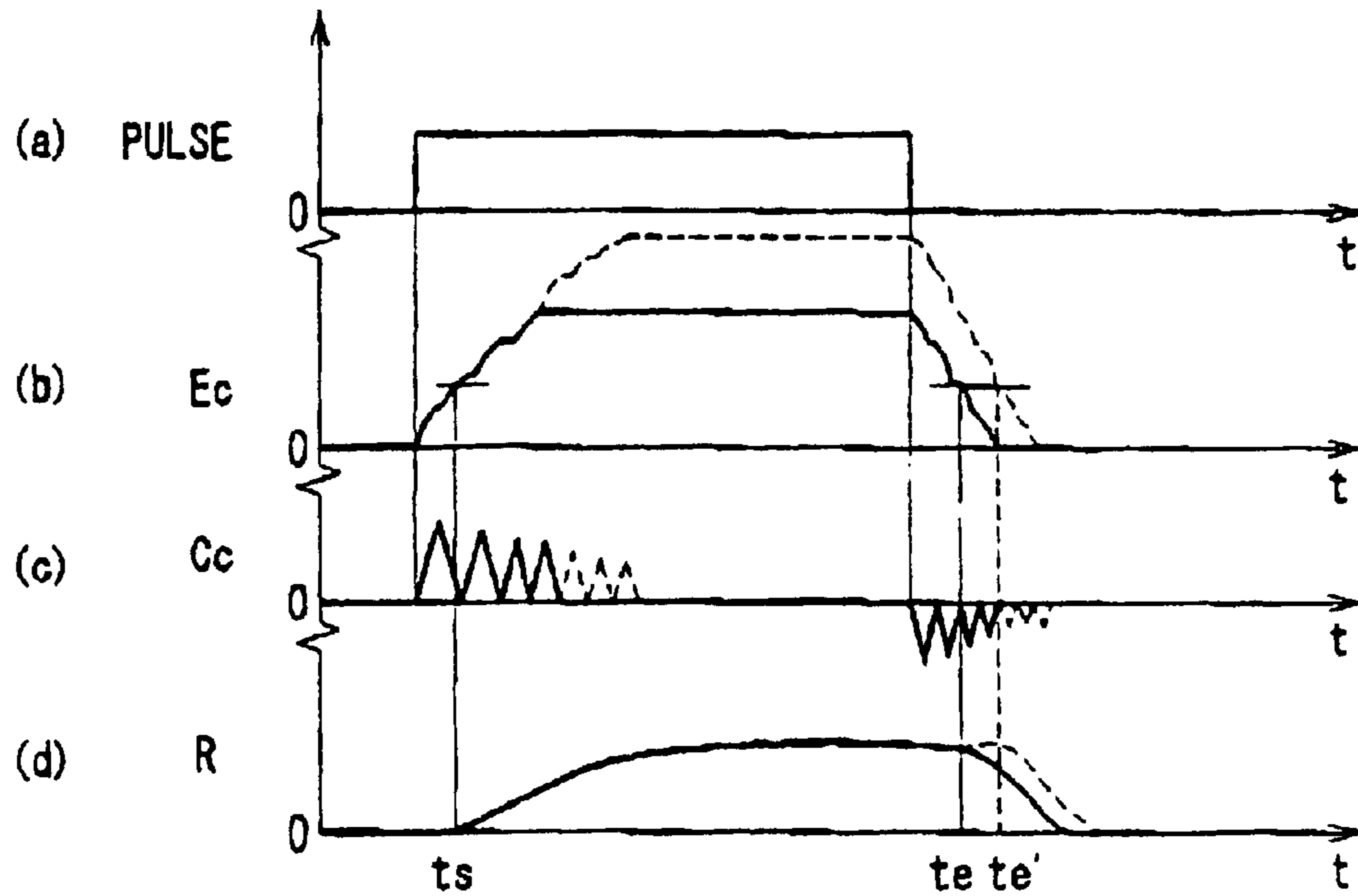
FIG. 8 RELATED ART
