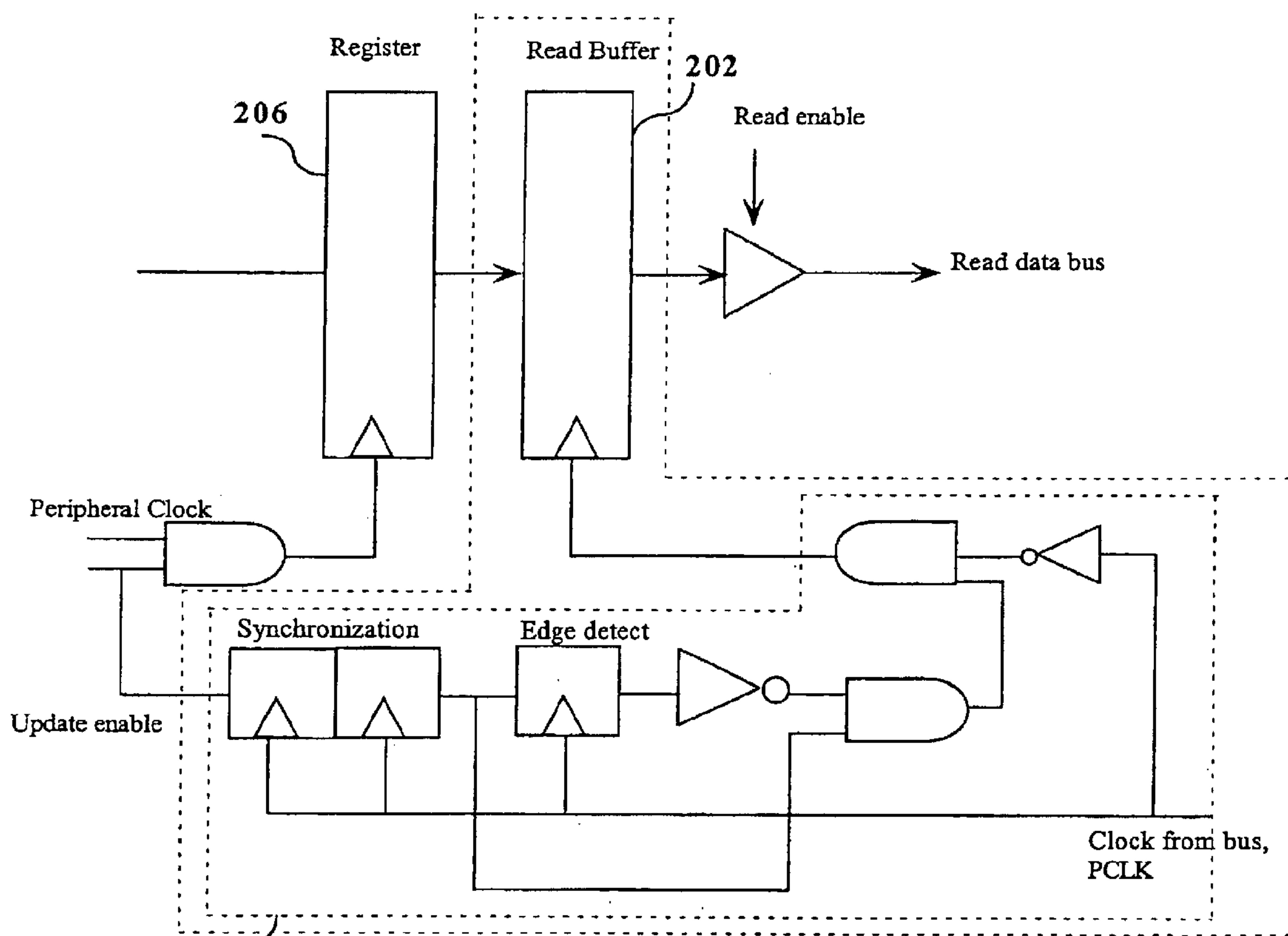
Figure 2 (Prior Art)
