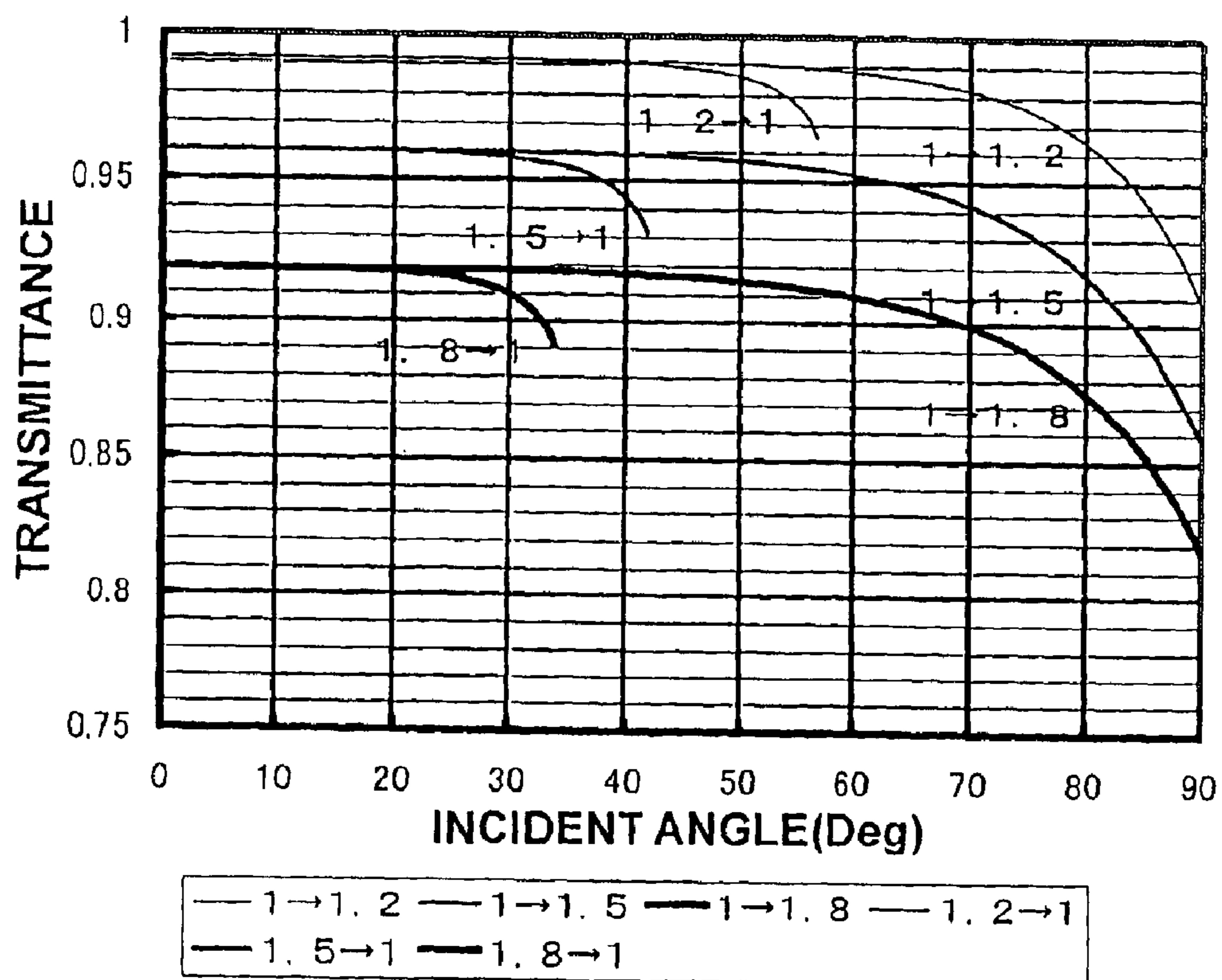
FRESNEL LOSS AT BOUNDARIES BETWEEN MEDIUMS HAVING DIFFERENT REFRACTIVE INDEXES
