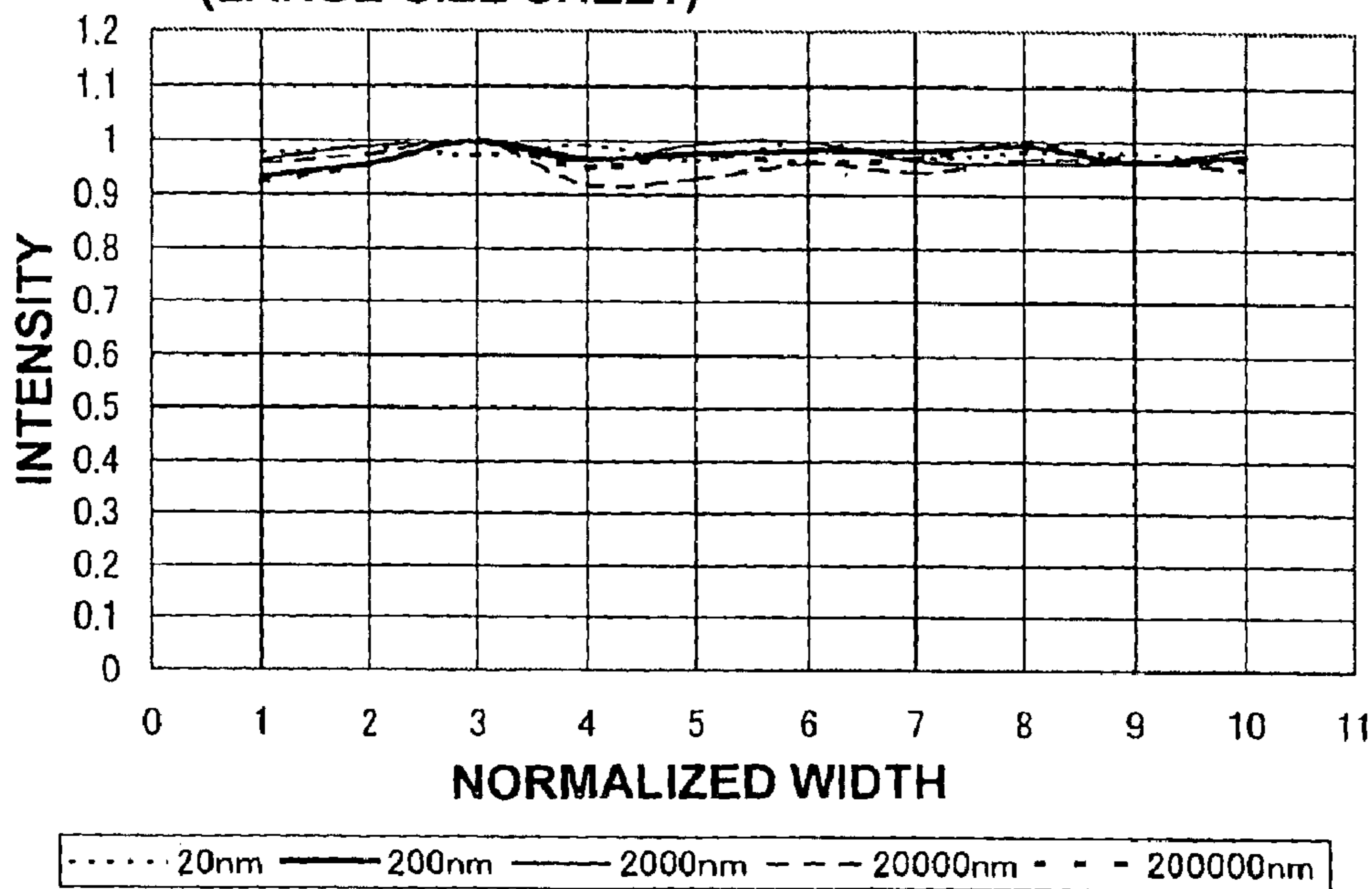
INTENSITY DISTRIBUTION OF EMITTED LIGHT (LARGE-SIZE SHEET)
