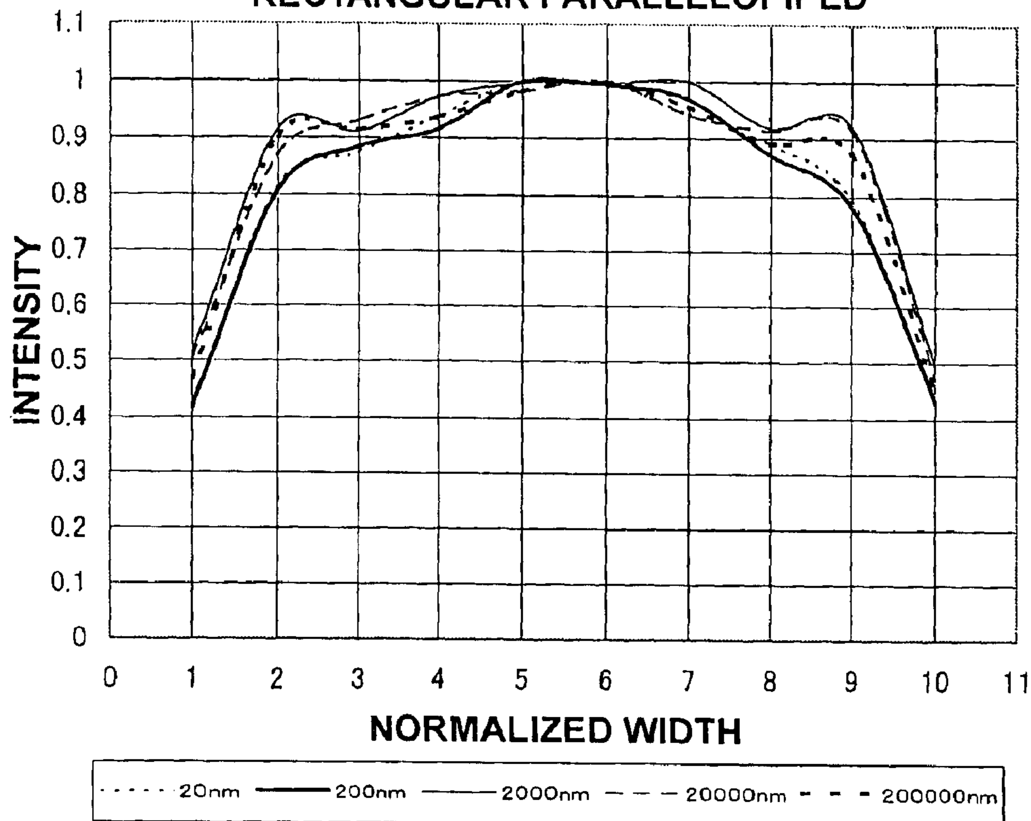
INTENSITY DISTRIBUTION OF EMITTED LIGHT (CENTRAL PORTION) RECTANGULAR PARALLELOPIPED
