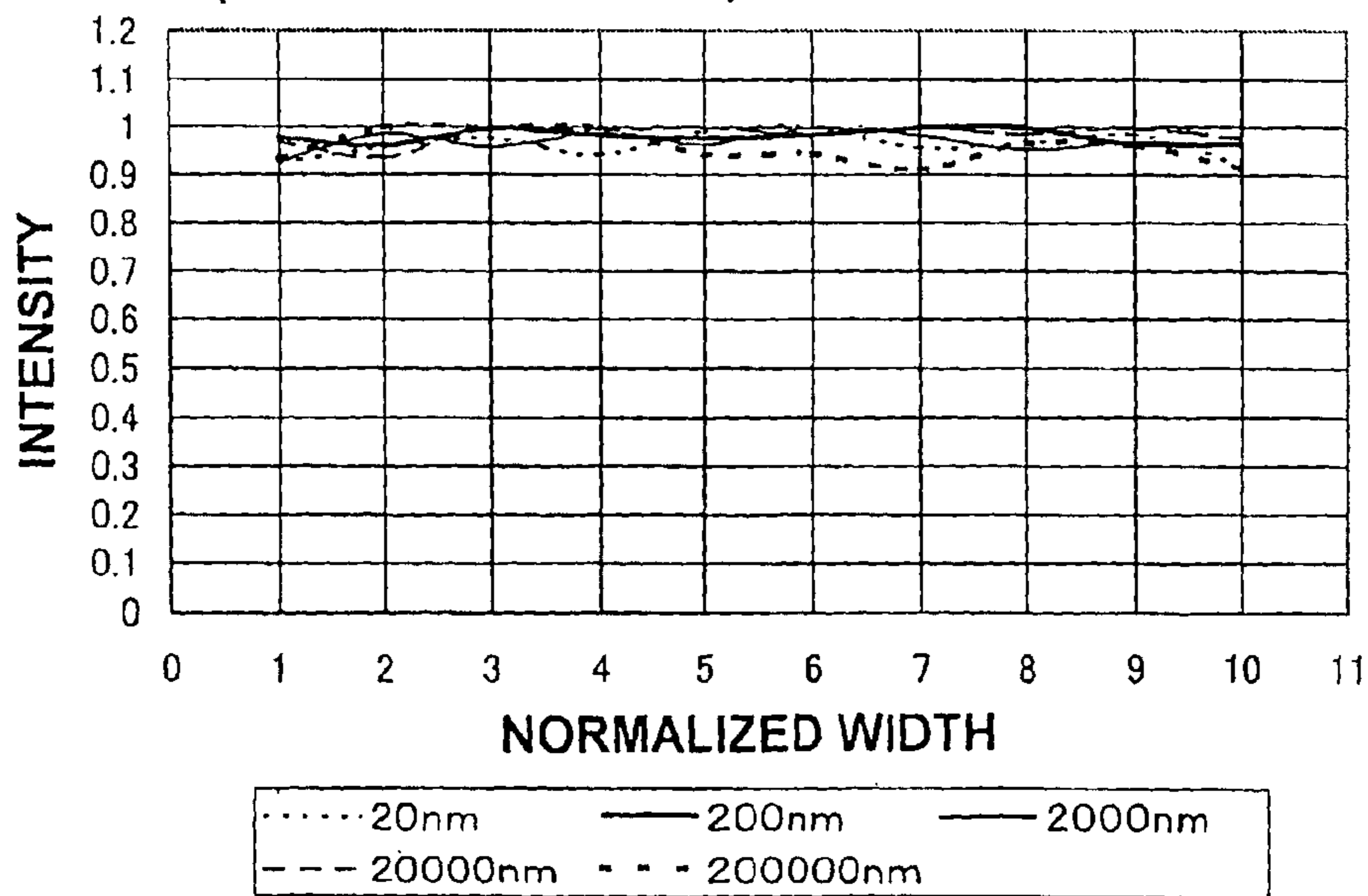
INTENSITY DISTRIBUTION OF EMITTED LIGHT (MEDIUM-SIZE SHEET)
