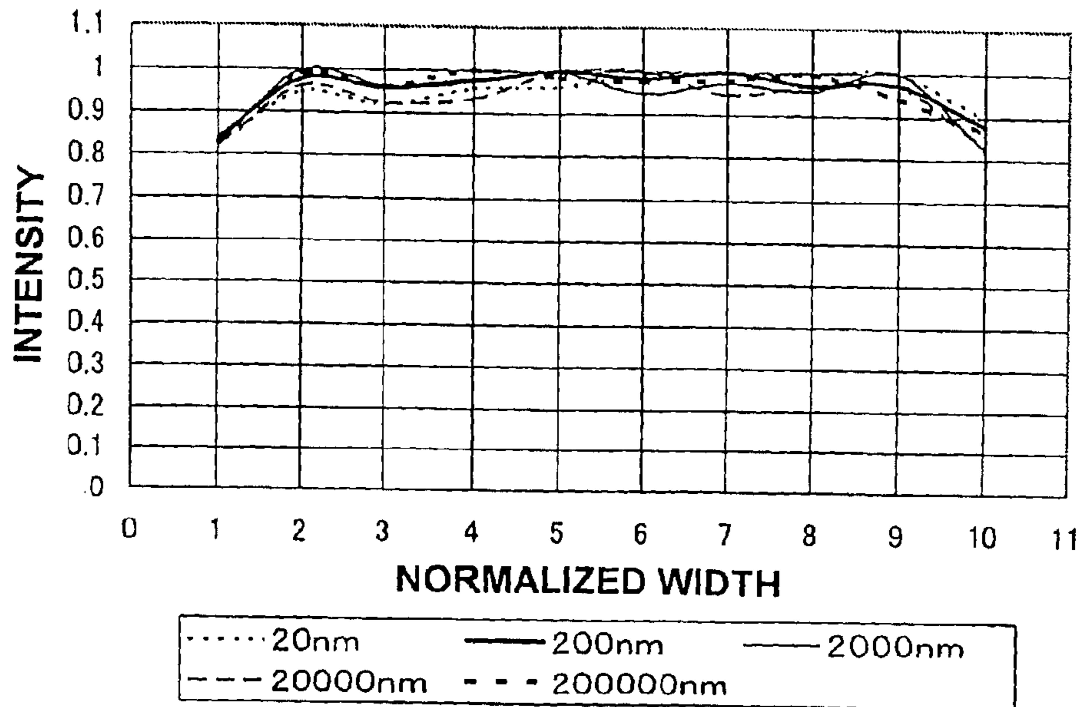
INTENSITY DISTRIBUTION OF EMITTED LIGHT (SMALL-SIZE SHEET)
