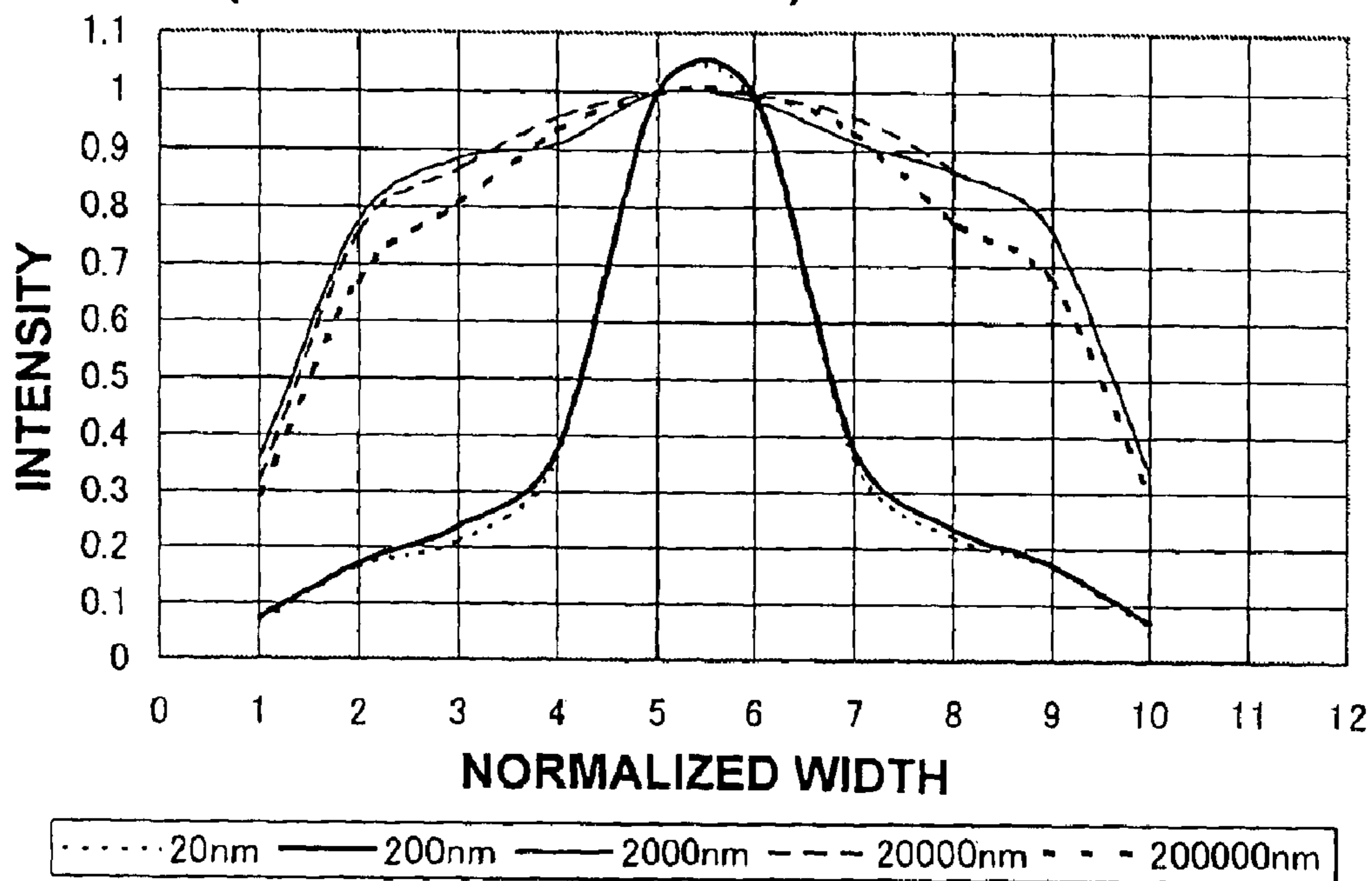
INTENSITY DISTRIBUTION OF EMITTED LIGHT (LARGE-SIZE CYLINDER)
