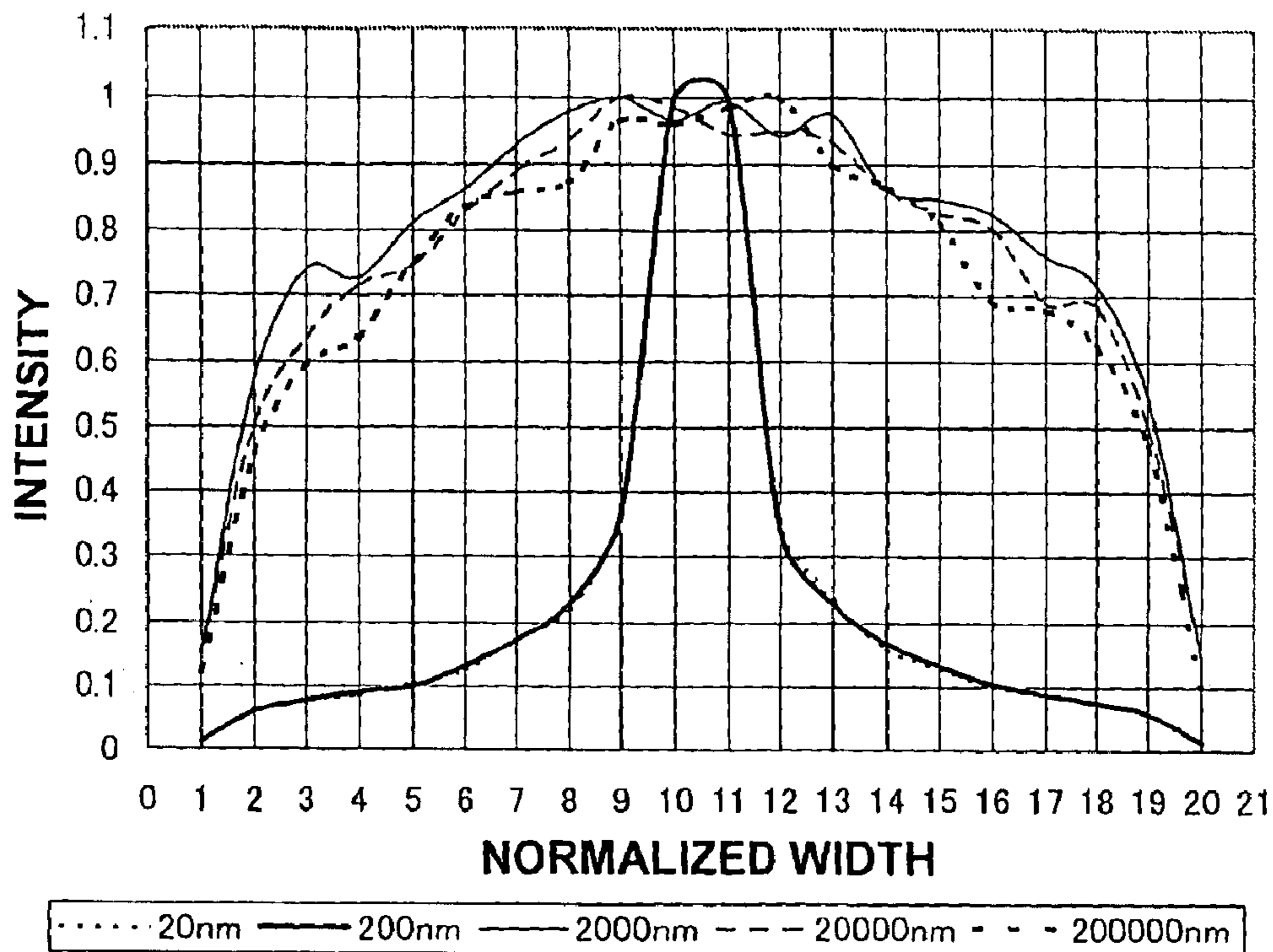
INTENSITY DISTRIBUTION OF EMITTED LIGHT (SMALL-SIZE CYLINDER)
