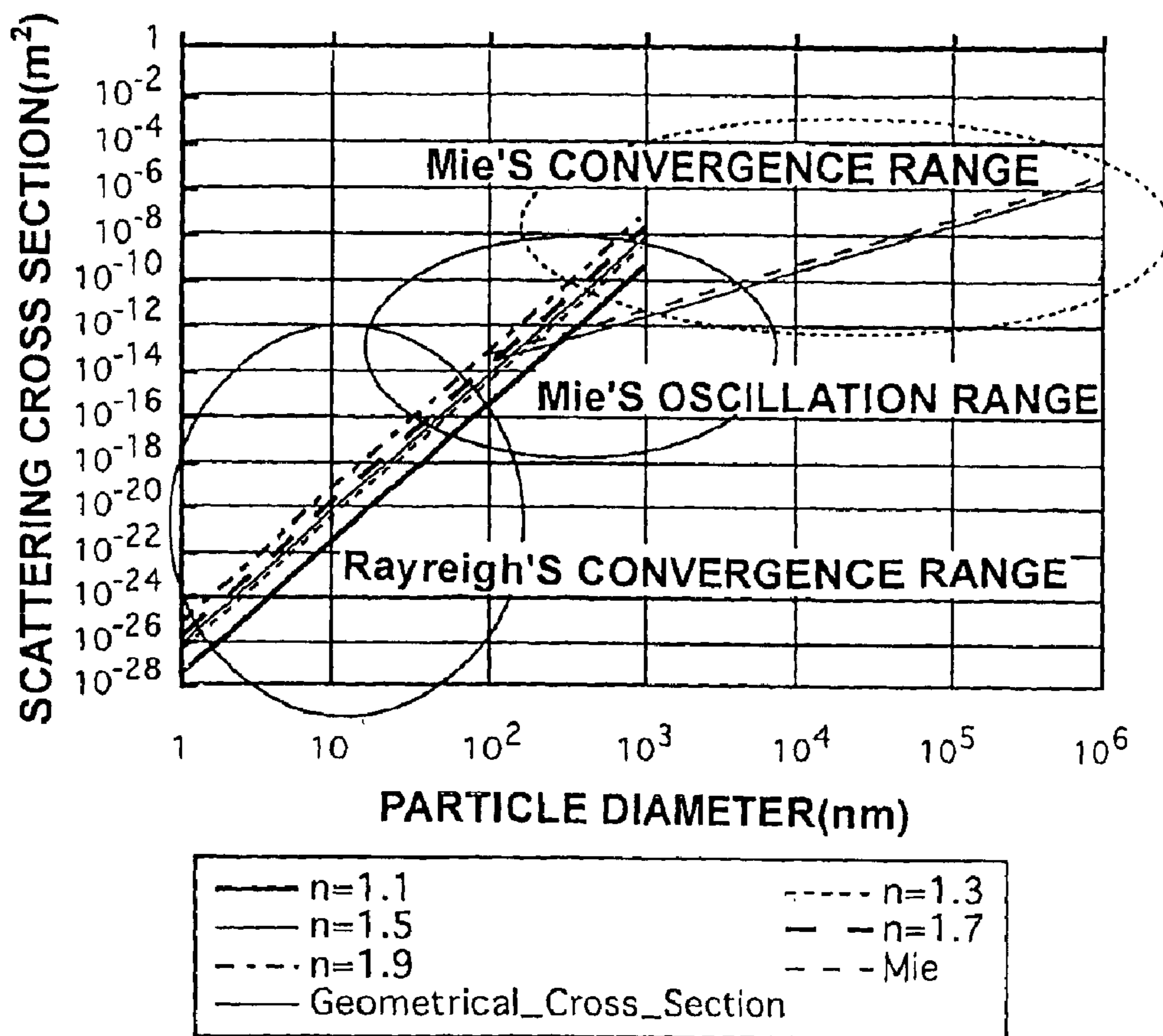
COMPARISON OF SCATTERING CROSS SECTIONS Rayreigh VS Fresnel(Mie'S CONVERGENCE RANGE)
