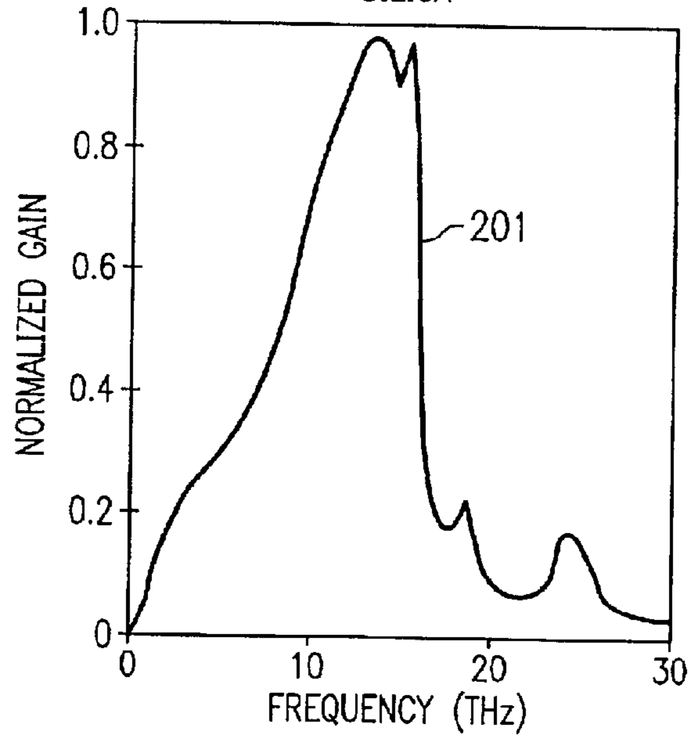
FIG. 2 (PRIOR ART) SILICA
