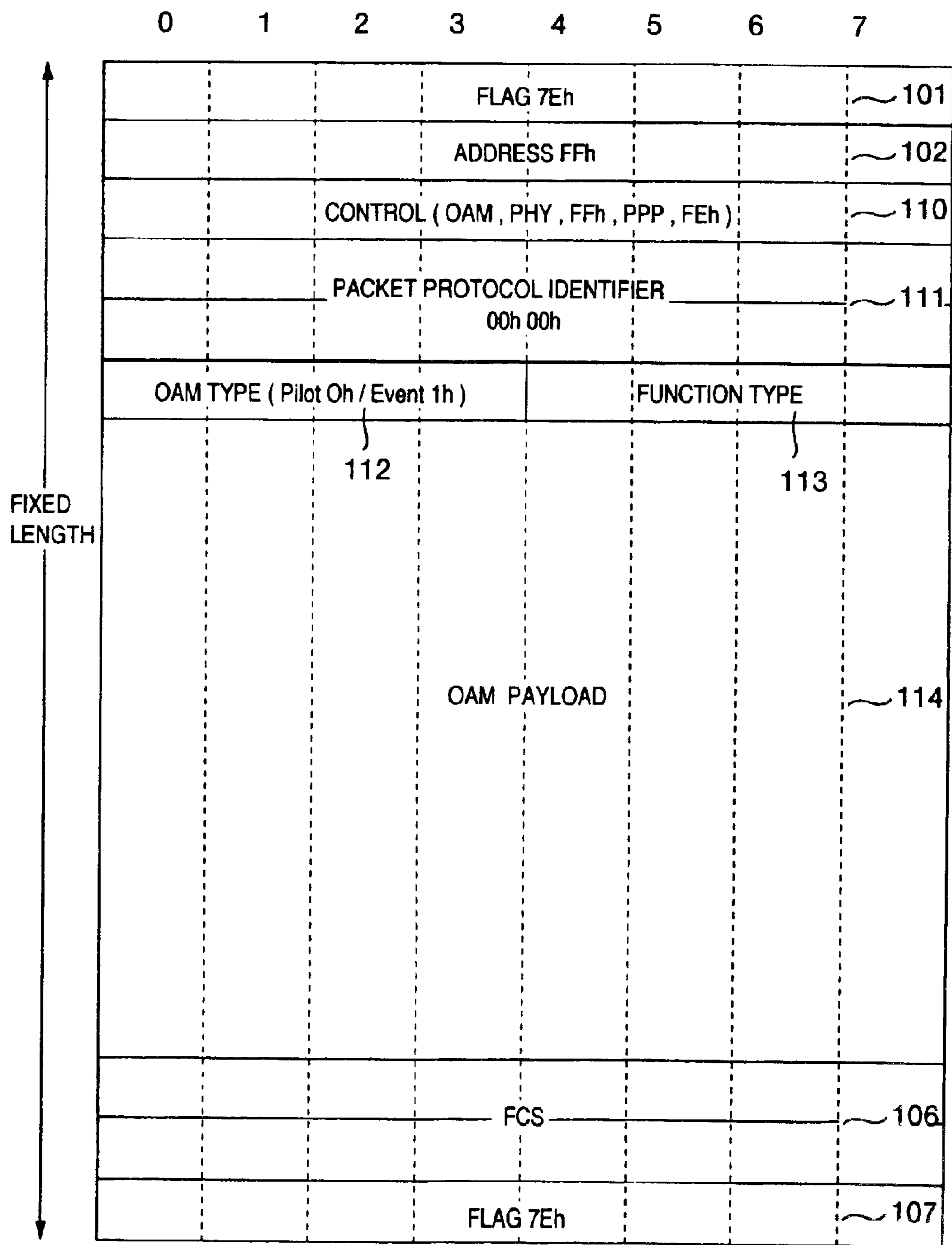
PPP OAM FRAME FORMAT
