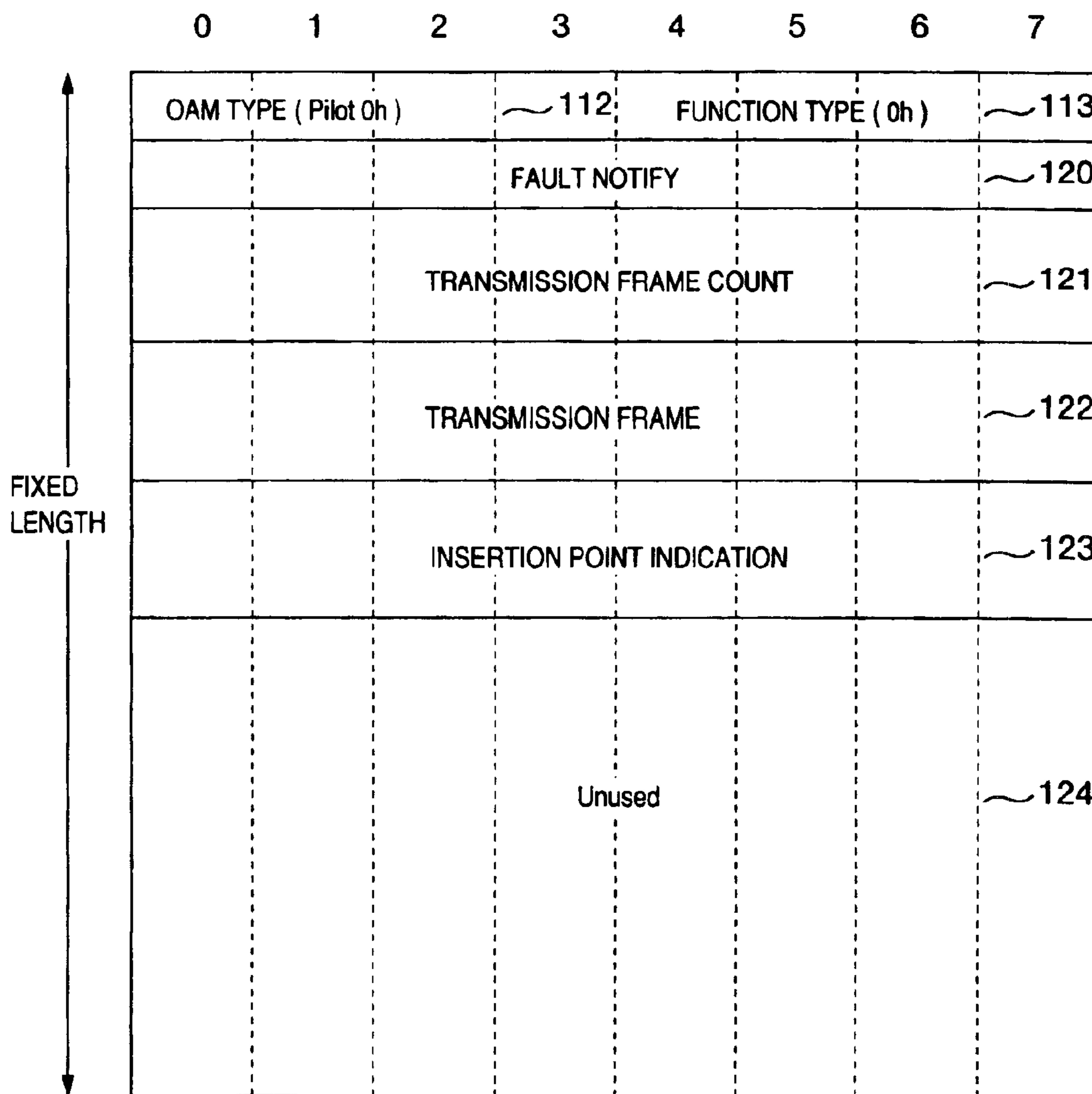
PPP OAM FRAME (Pilot) Payload
