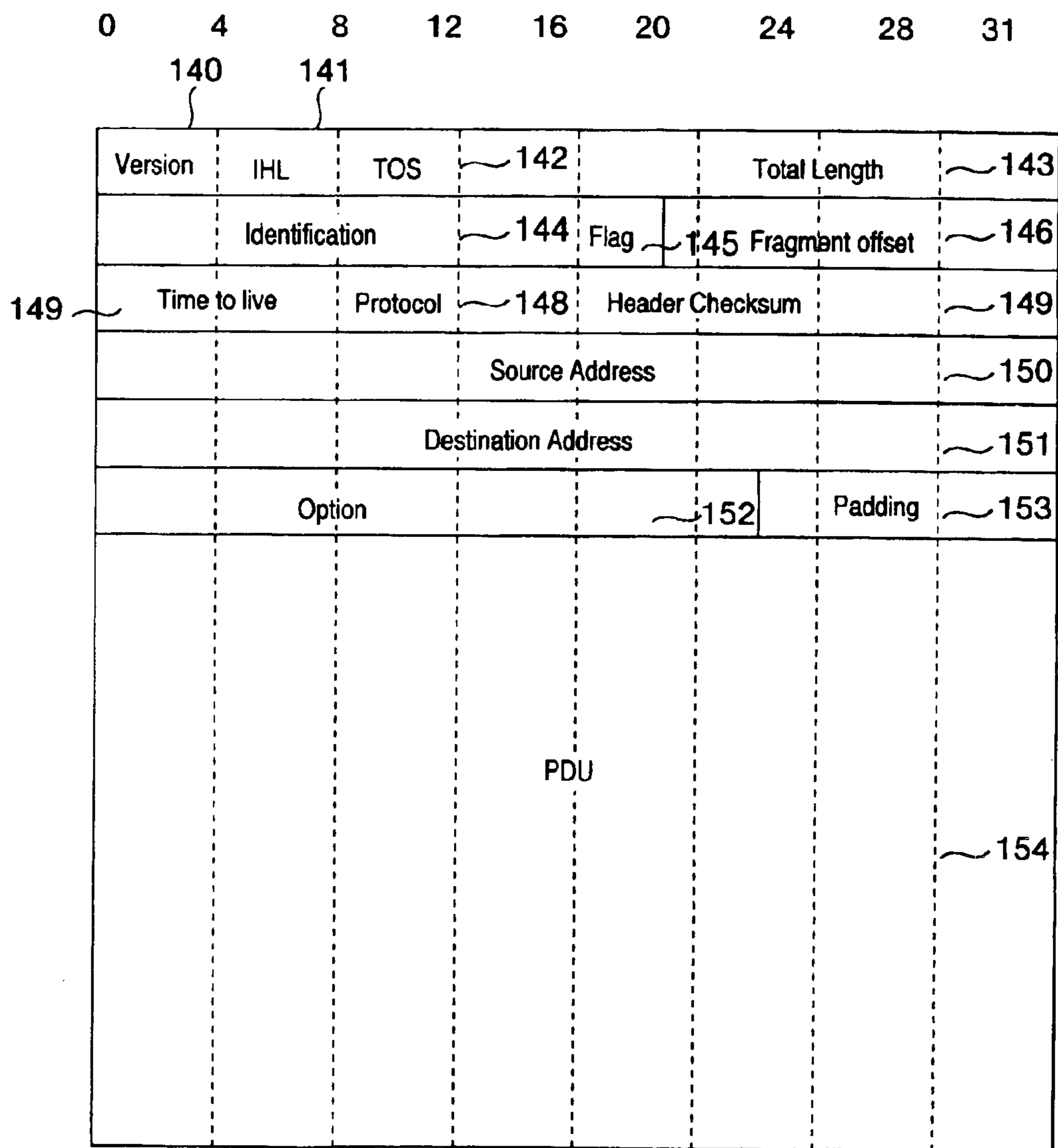
IPv4 FRAME FORMAT
