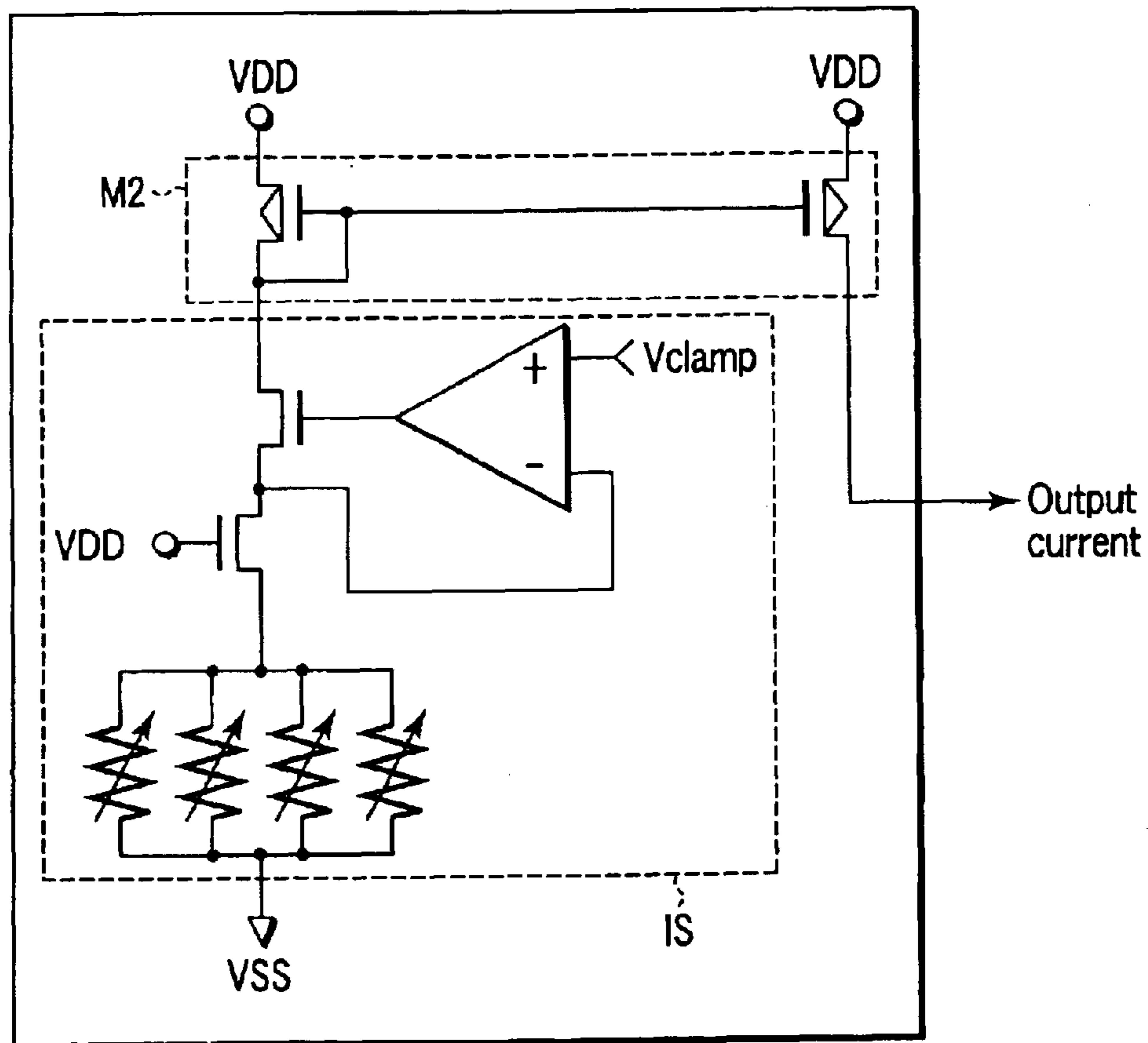
Additive current generating section 42
