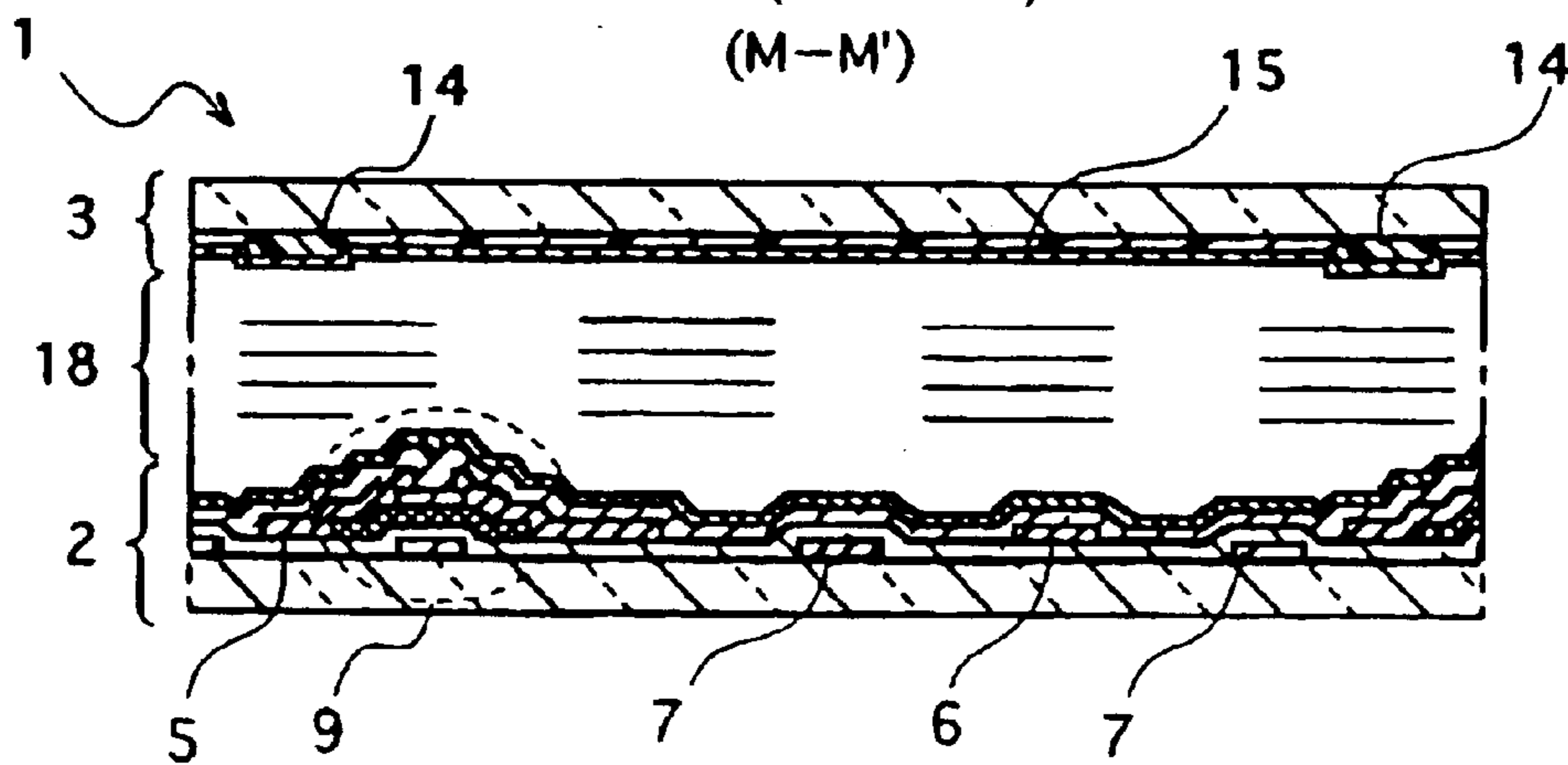
FIG. 18c (Prior Art)
