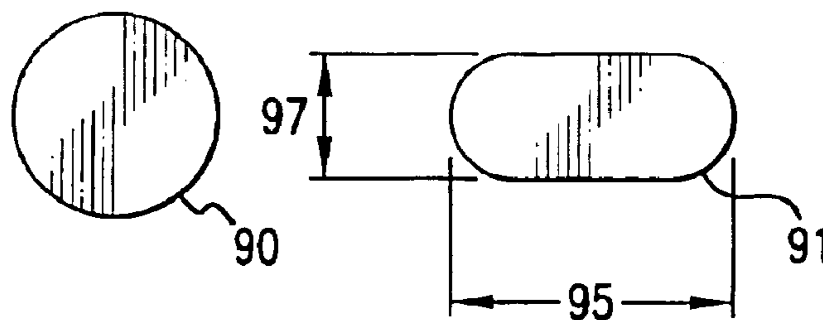
FIG. 9 PRIOR ART
