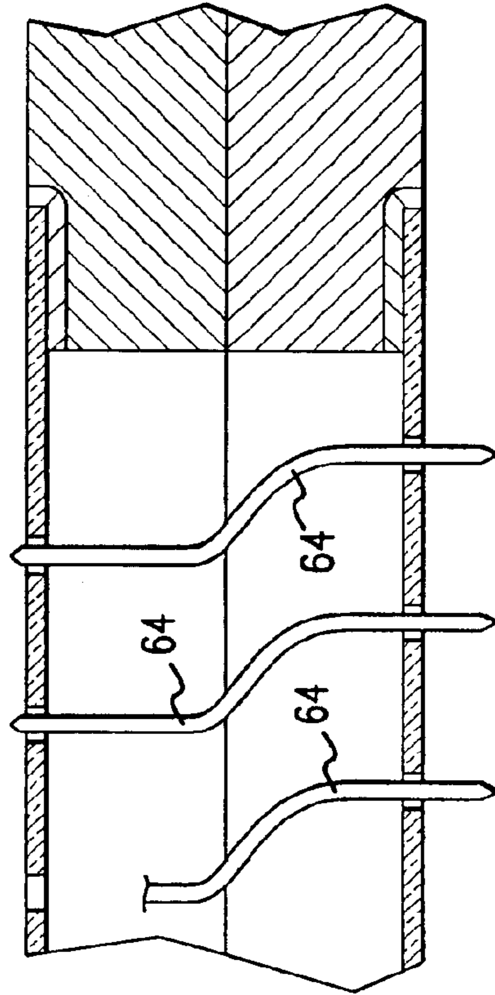
FIG. 3 (PRIOR ART)
