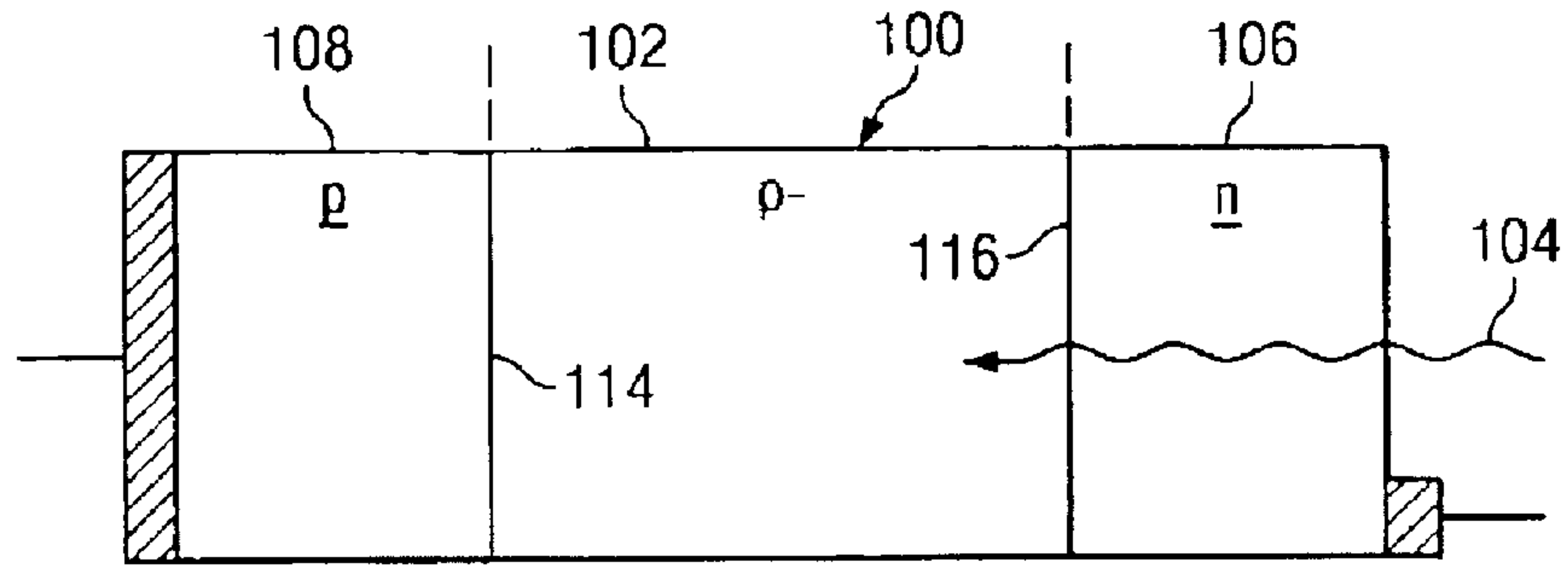
FIG. 1 (PRIOR ART)
