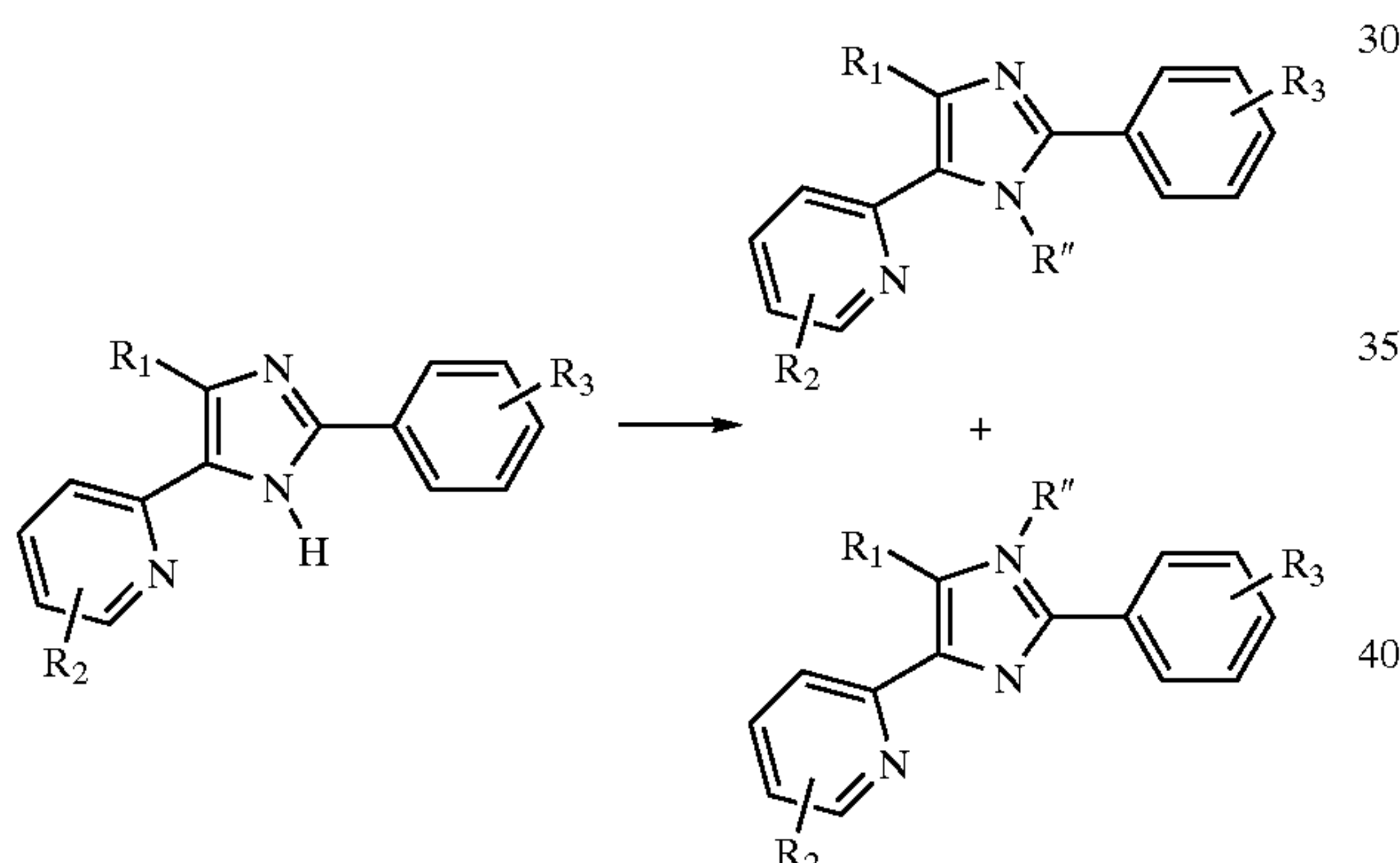
Scheme 3
