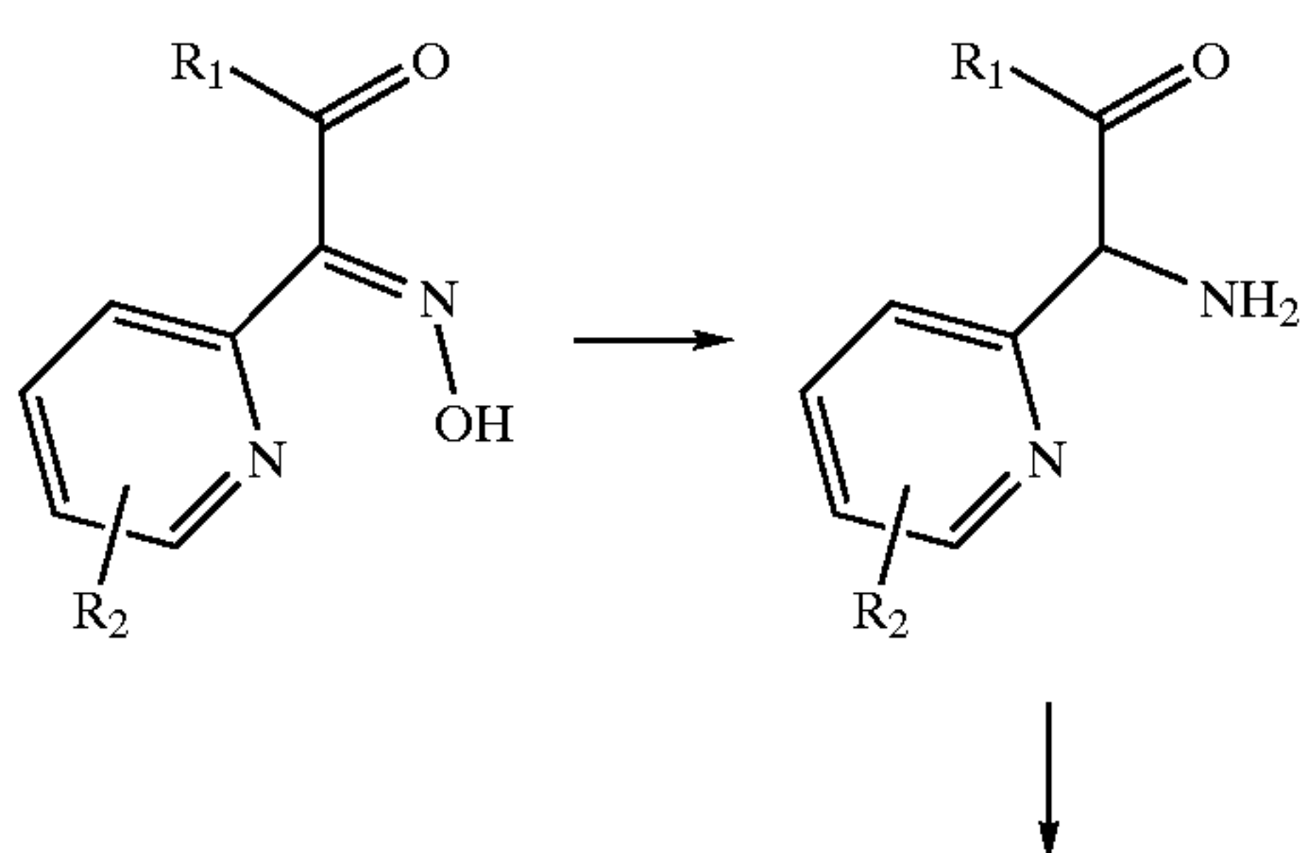
Scheme 4
