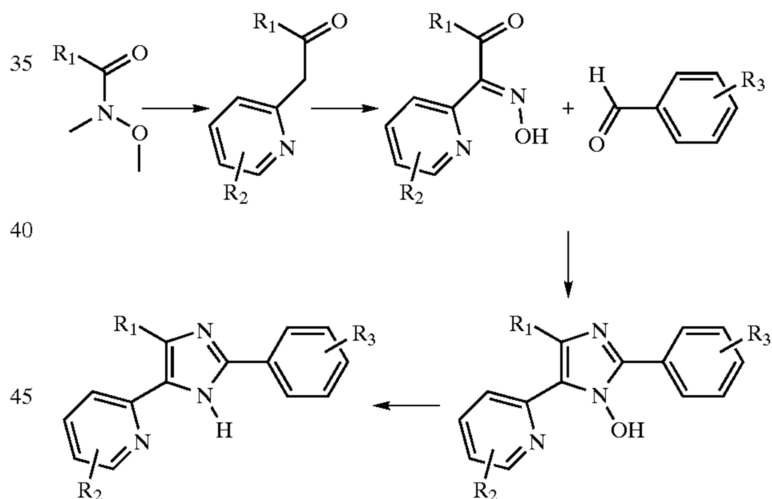
Scheme 1
