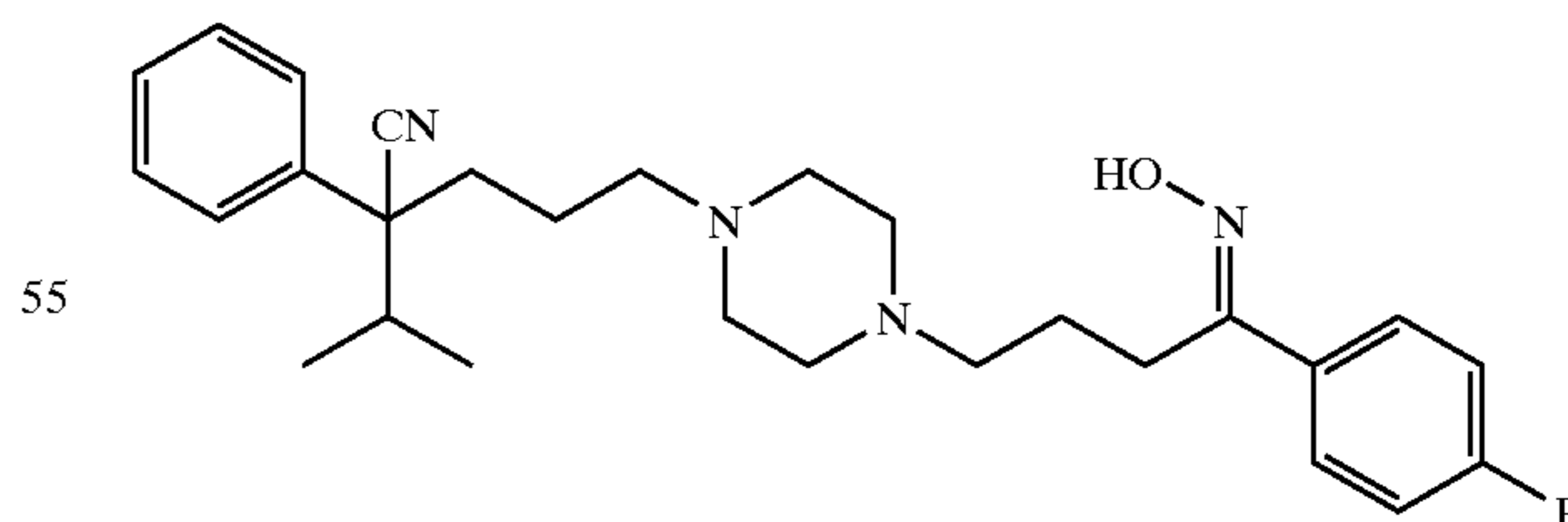
Example 51 1-[(4-Cyano-5-methyl-4-phenyl)hexyl]-4-[4-hydroxime-4-(4'-fluorophenyl)butyl]piperazine
