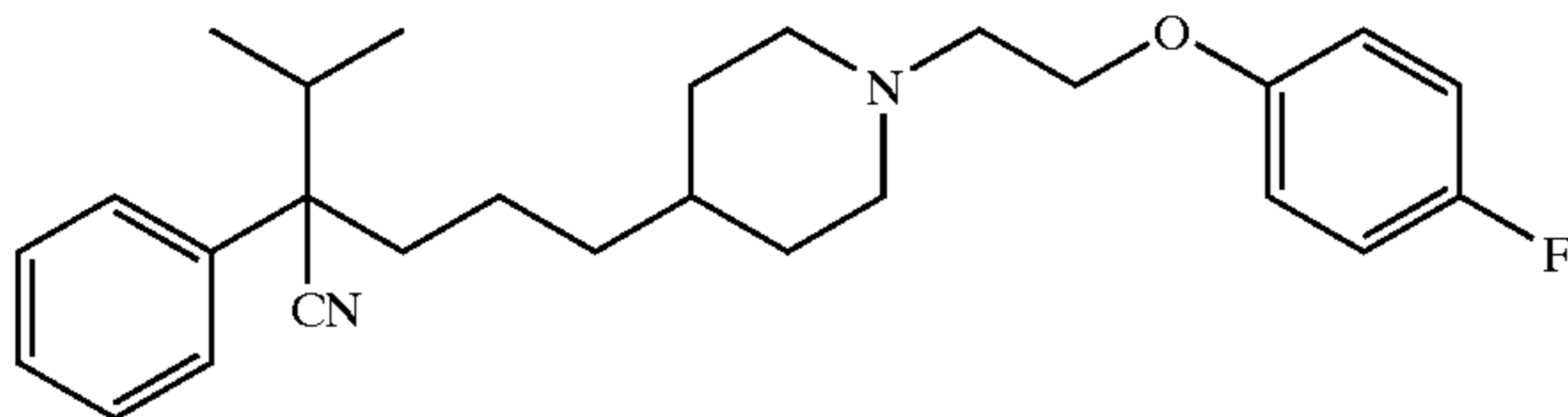
Example 48 1-[(2-(4-Fluorophenoxy)ethyl)-4-[(4-cyano-5-methyl-4-phenyl)hexyl]piperidine
