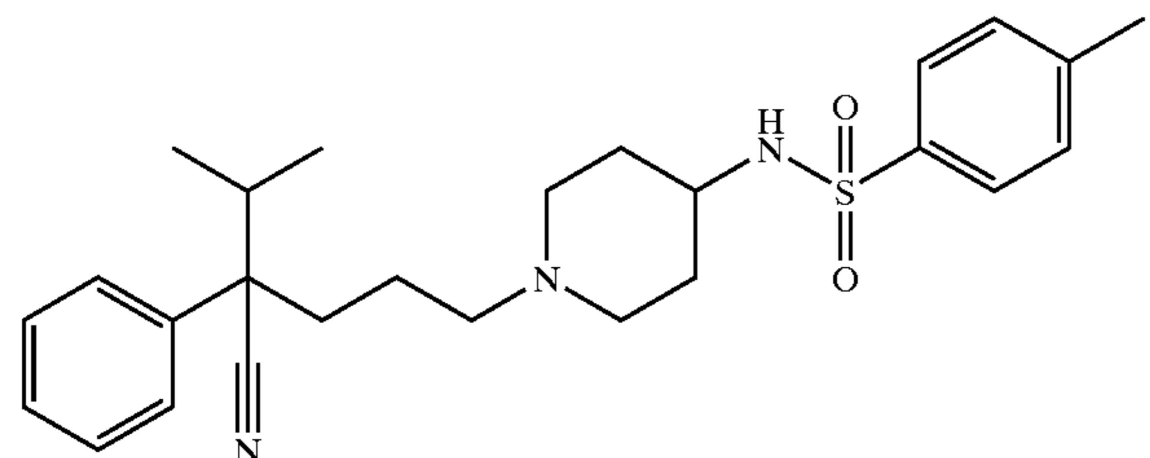
Example 229 N-[1-[4-cyano-5-methyl-4-phenyl)hexyl]piperidine-4-yl]p-toluenesulfonamide
