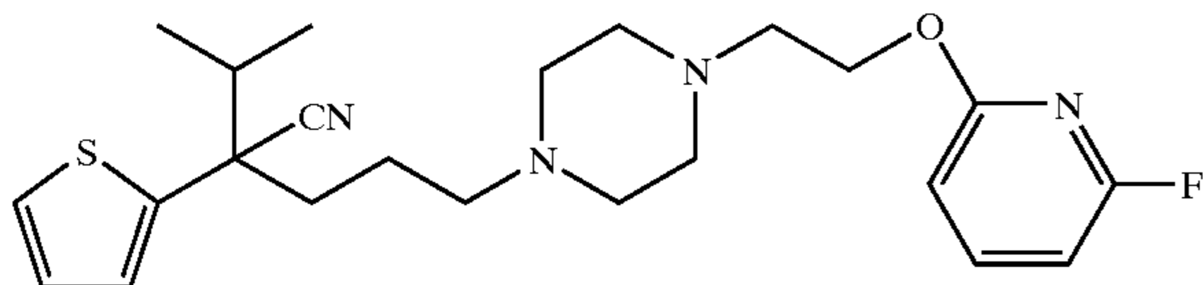
Example 193 1-[4-cyano-4-(2-thienyl)-5-methylhexyl]-4-[2-(6-fluoro-2-pyridyloxy)ethyl]piperazine
