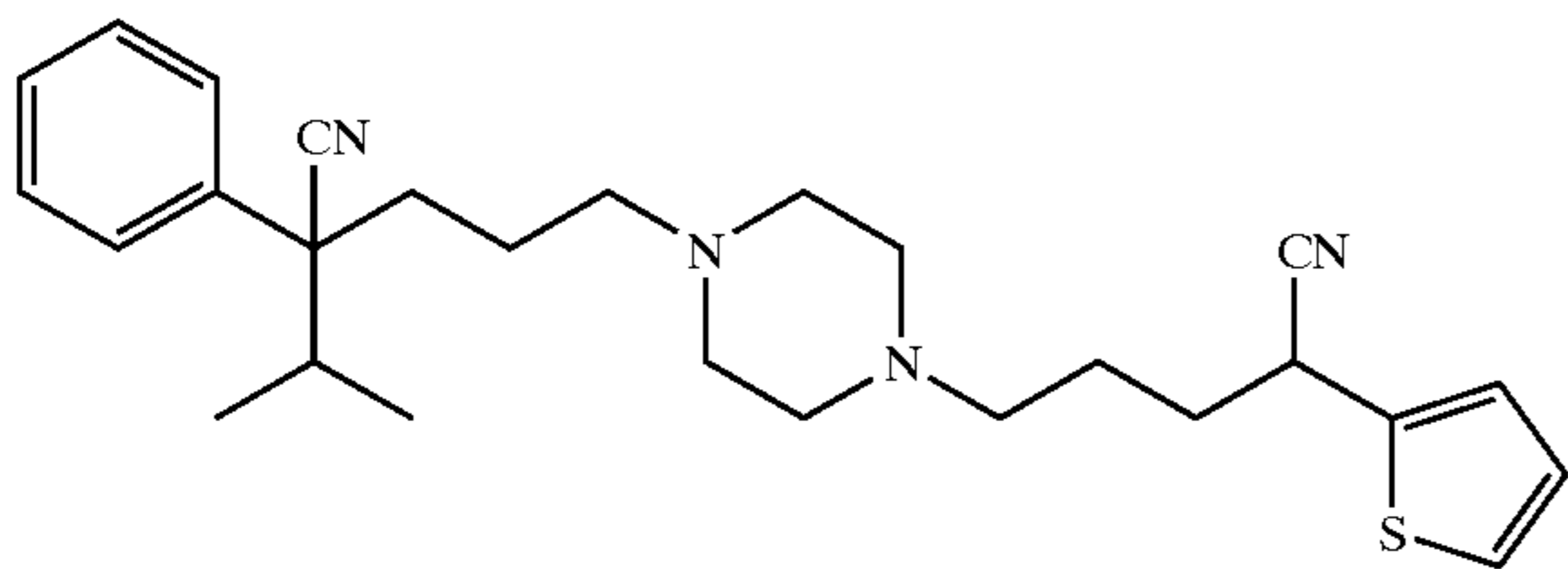
Example 49 1-[(4-cyano-5-methyl-4-phenyl)hexyl]-4-[3-cyano-3-(2-thienyl)propyl]piperazine
