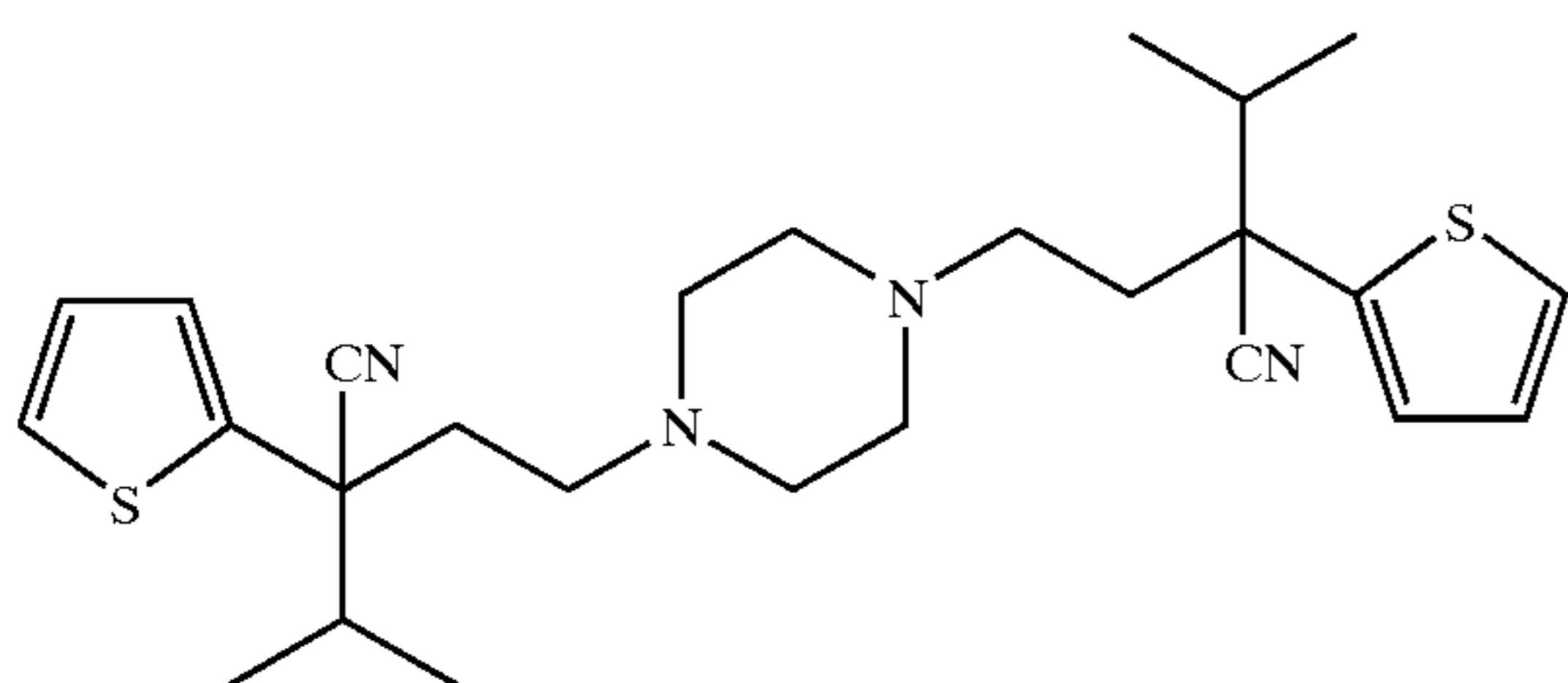
Example 126 Bis-1,4-[(3-cyano-4-methyl-3-(2-thienyl)pentyl)piperazine]
