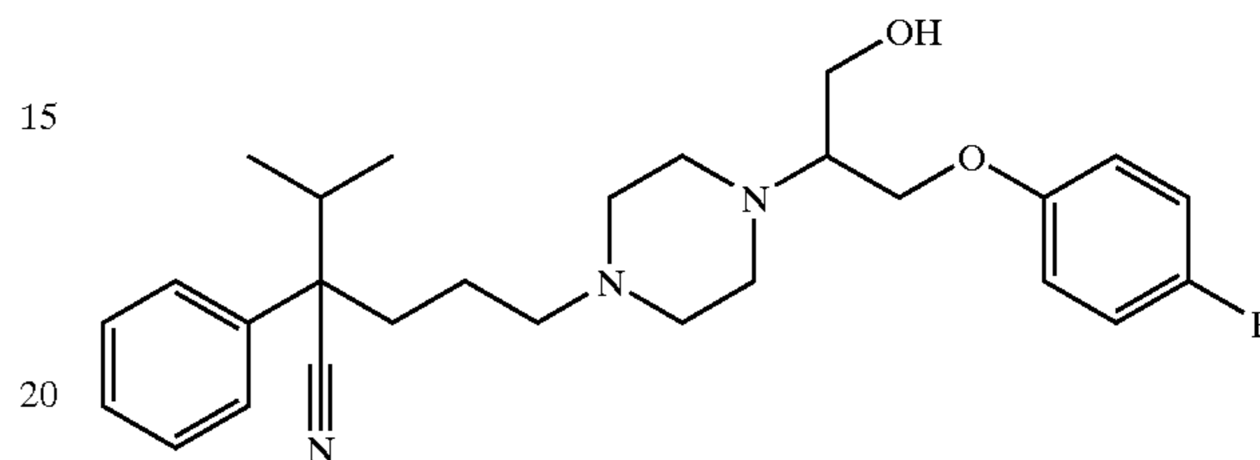
Example 230 1-[4-cyano-5-methyl-4-phenyl)hexyl]-4-[3-hydroxy-1-(4-fluorophenoxy)propane-2-yl]piperazine
