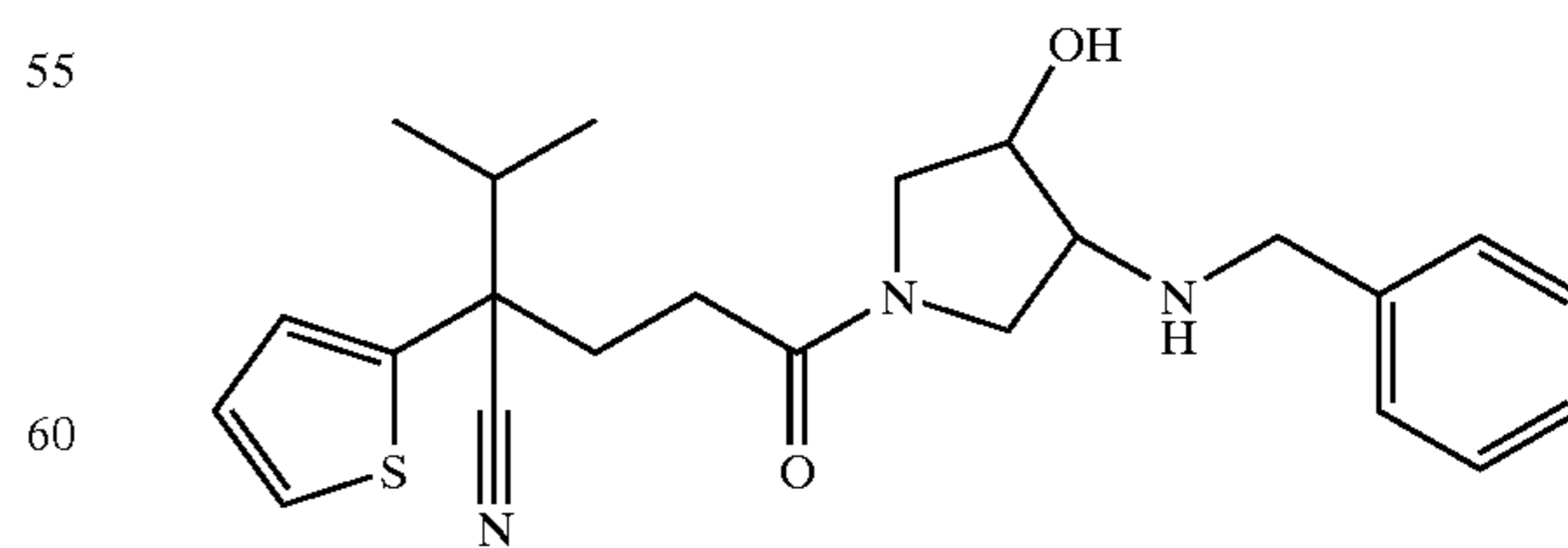
Example 130 5-[3-(Benzylamino)-4-hydroxytetrahydro-1H-1-pyrrolyl]-2-isopropyl-5-oxo-2-(2-thienyl)pentane Nitrile
