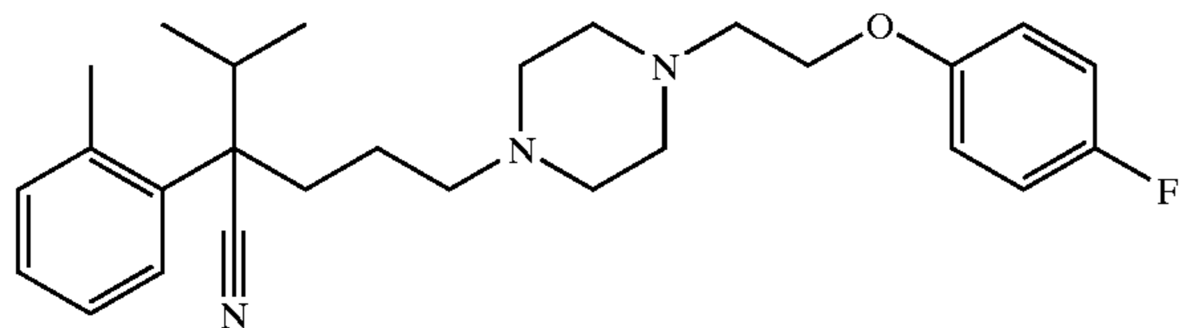
Example 227 1-[4-cyano-5-methyl-4-(O-tolyl)hexyl]-4-[2-(4-fluorophenoxy)ethyl]piperazine
