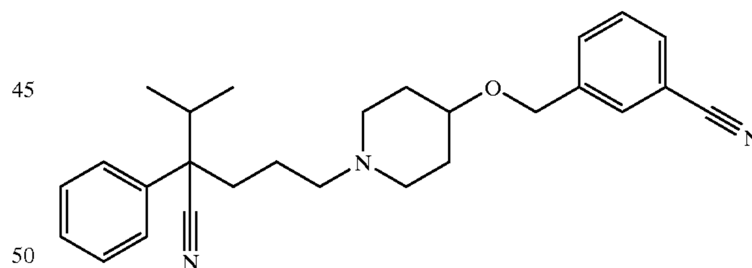
Example 231 1-[4-cyano-5-methyl-4-phenyl)hexyl]-4-(3-cyanobenzoyloxy)piperidine
