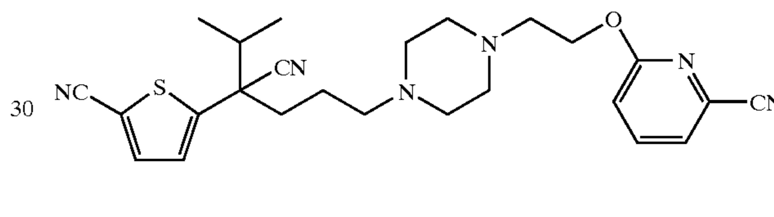
Example 197 1-[4-cyano-4-(5-cyano-2-thienyl)-5-methylhexyl]-4-[2-(6-cyano-2-pyridyloxy)ethyl]piperazine
