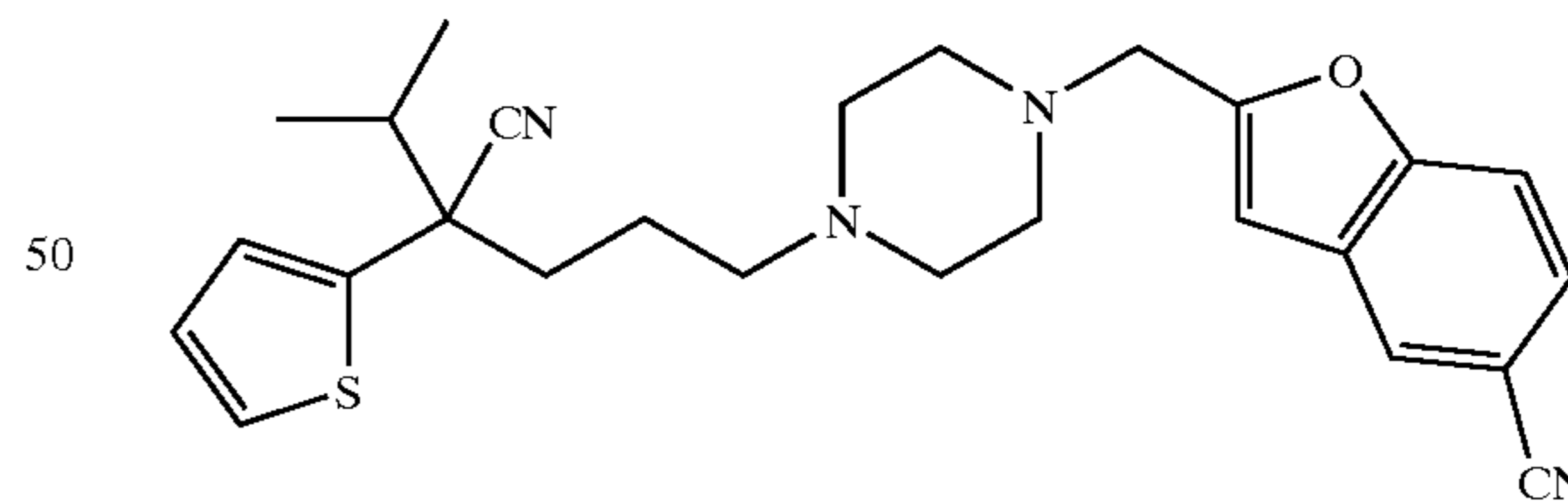
Example 106 1-[4-Cyano-5-methyl-4-(2-thienyl)hexyl]-4-[(2-(5-cyanobenzofuranyl)methyl] piperazine
