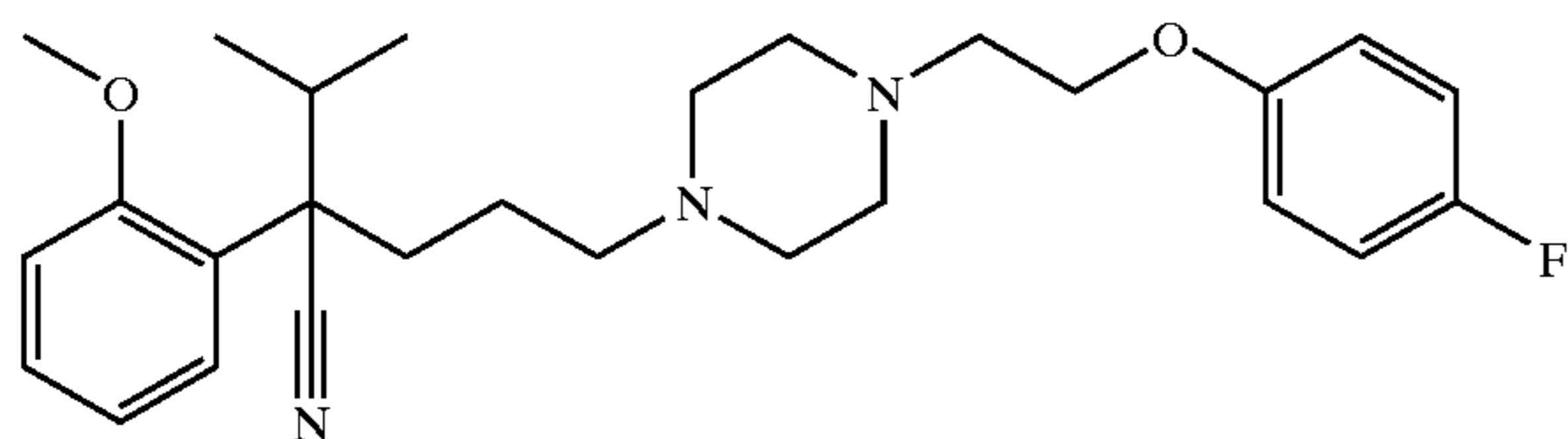
Example 228 1-[4-cyano-5-methyl-4-(2-methoxyphenyl)hexyl]-4-[2-(4-fluorophenoxy)ethyl]piperazine
