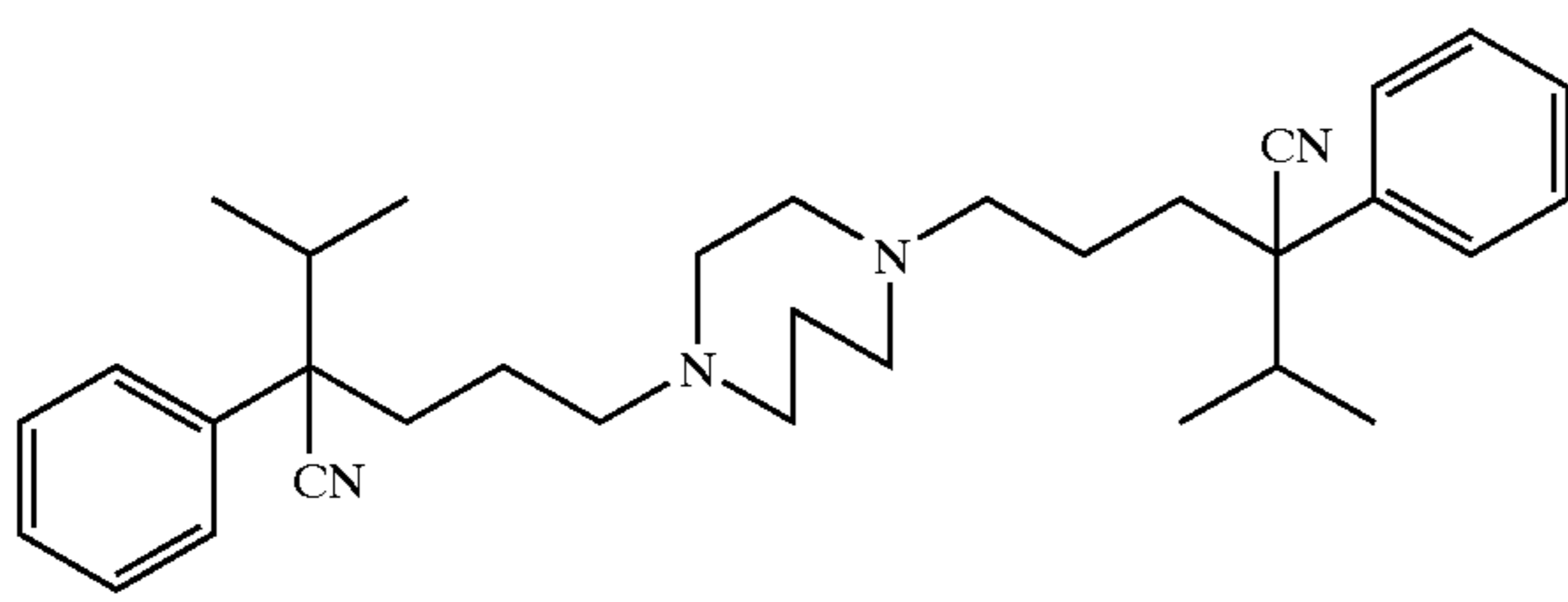
Example 125 Bis-1,4-[(3-cyano-4-methyl-3-phenyl)hexyl]homopiperazine
