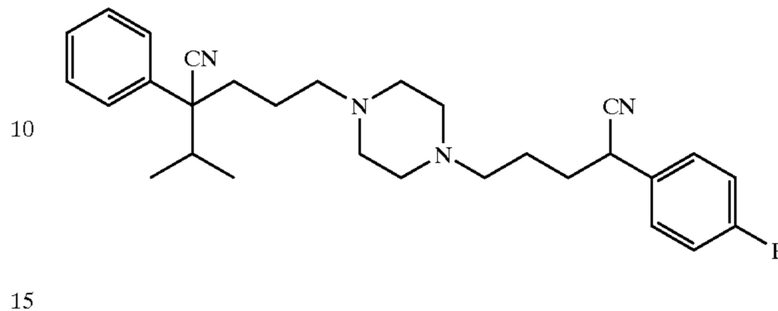
Example 50 1-[(4-Cyano-5-methyl-4-phenyl)hexyl]-4-[(4-cyano-4-(4'-fluorophenyl)butyl)piperazine
