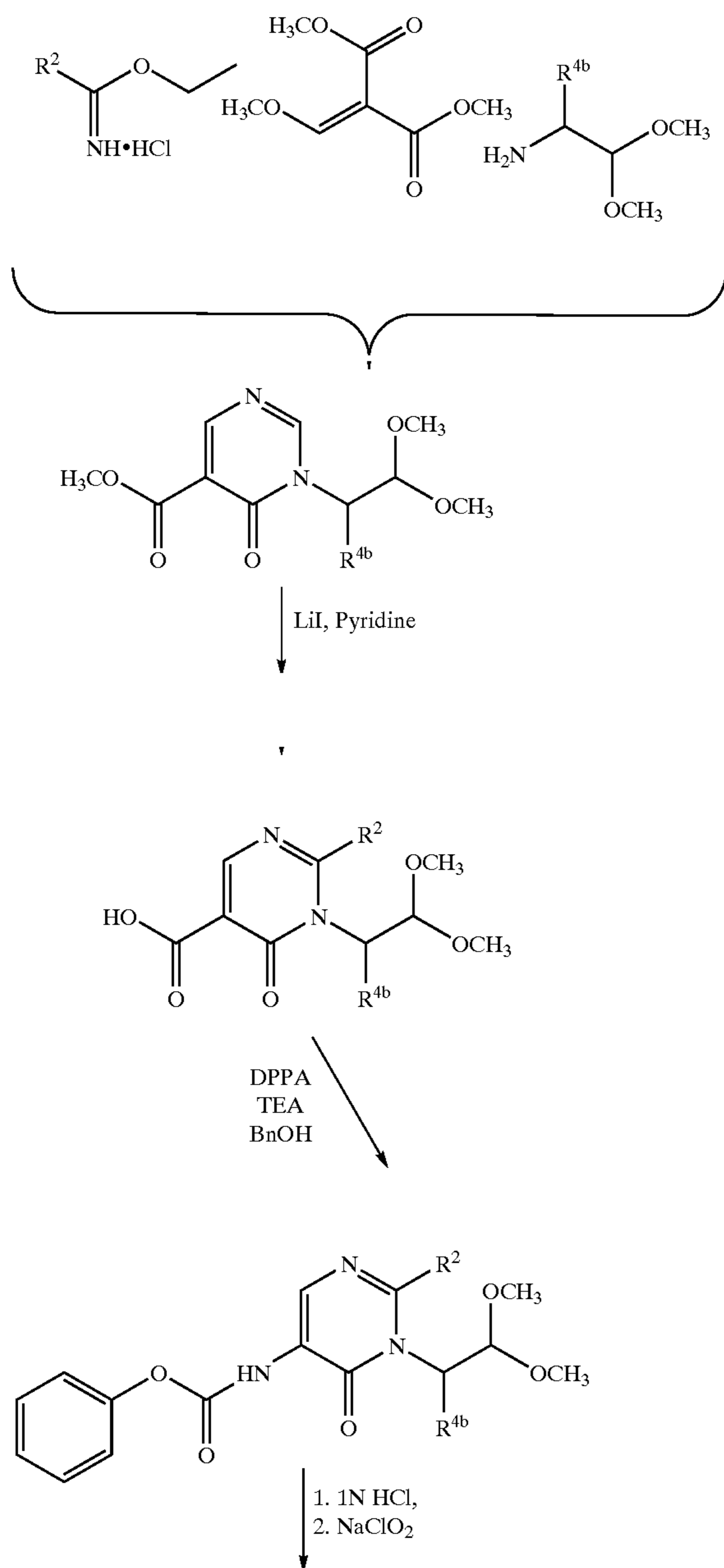
Scheme 1: General Pyrimidinone Synthesis-I
