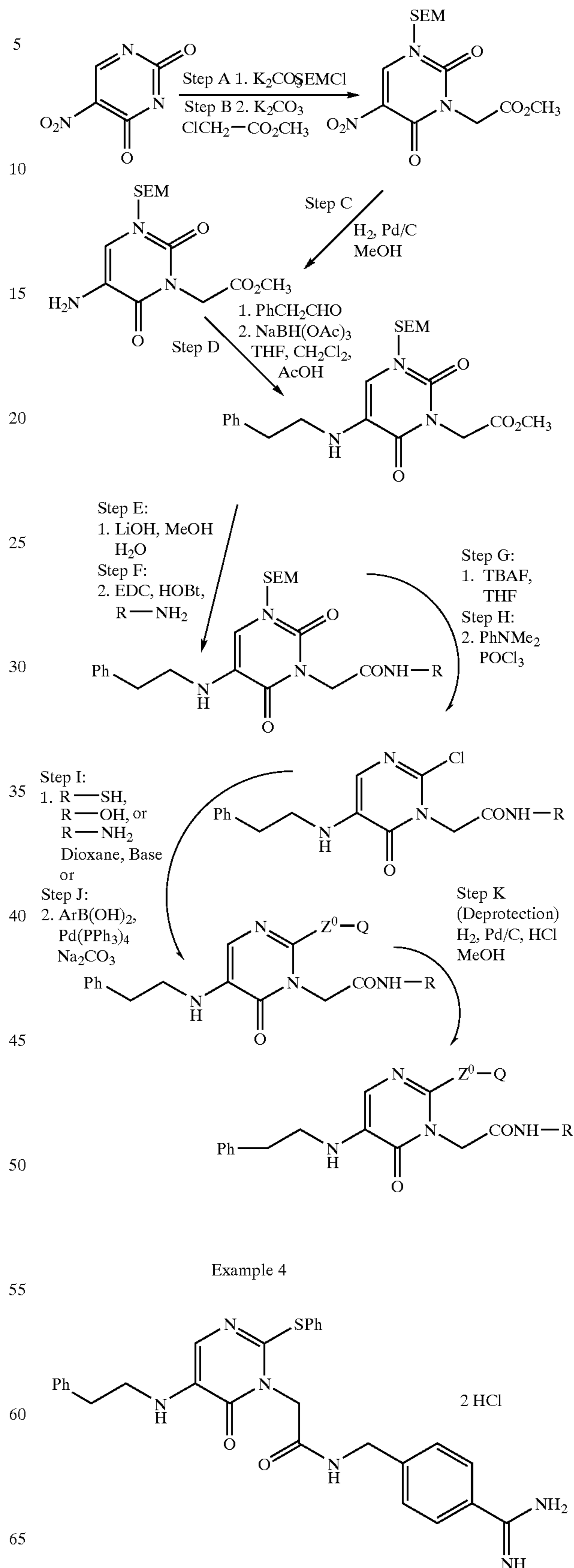
Scheme 6: Preparation of 2-Substituted Pyrimidinones
