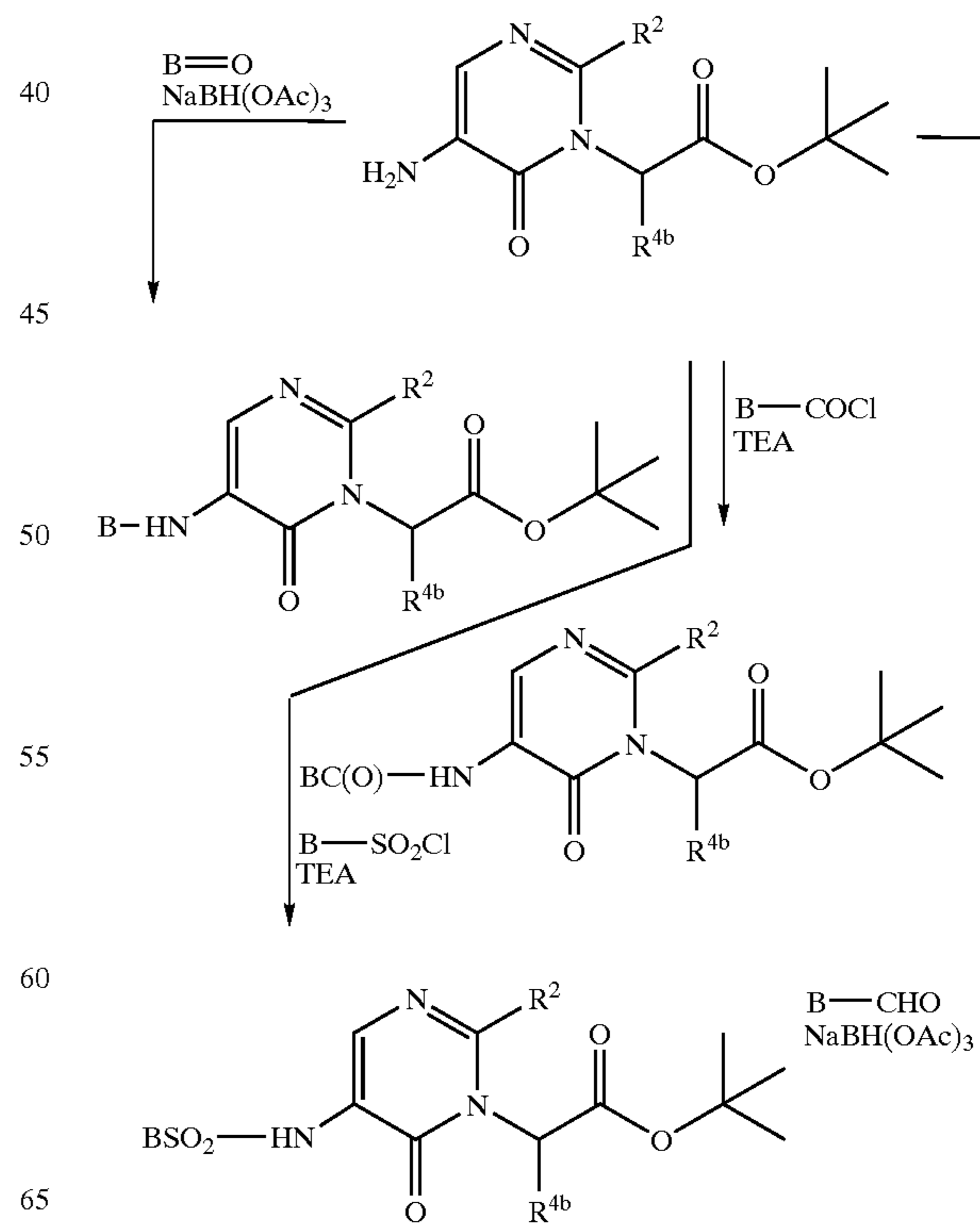
Scheme 3: General Pyrimidinone Synthesis-I (Continued)
