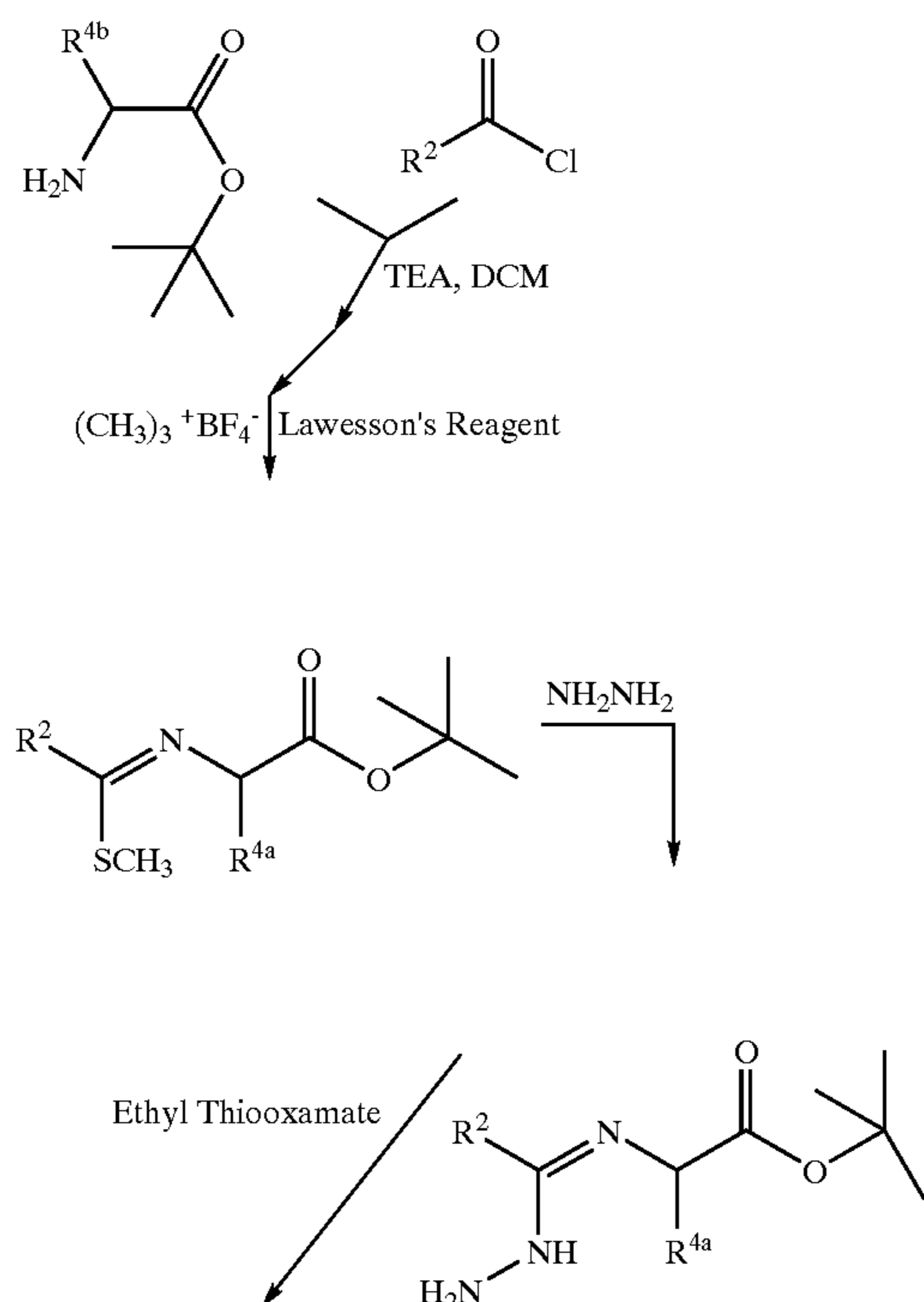
Scheme 9: General 4-AzaPyrimidinon Synthesis
