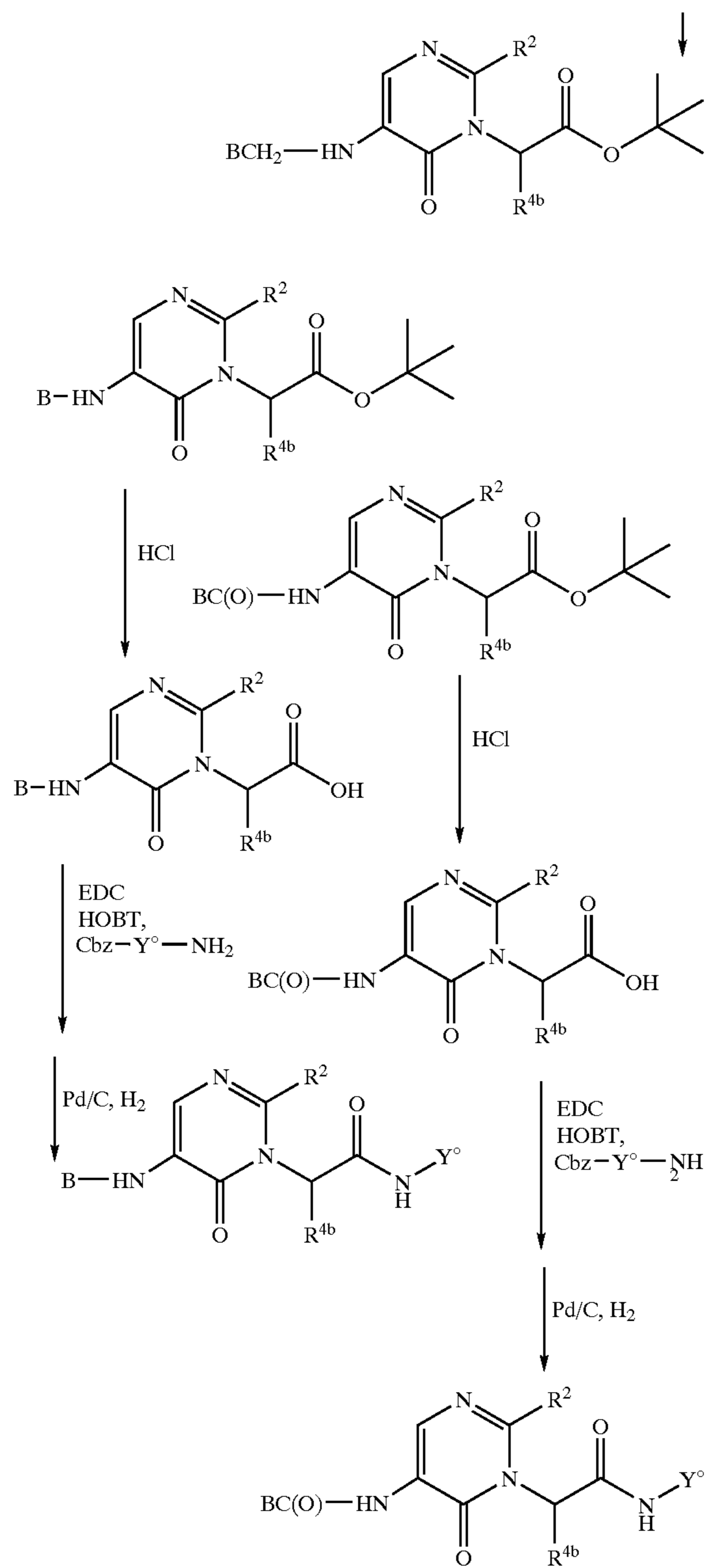
Scheme 5: General Pyrimidinone Synthesis-I (Concluded)
