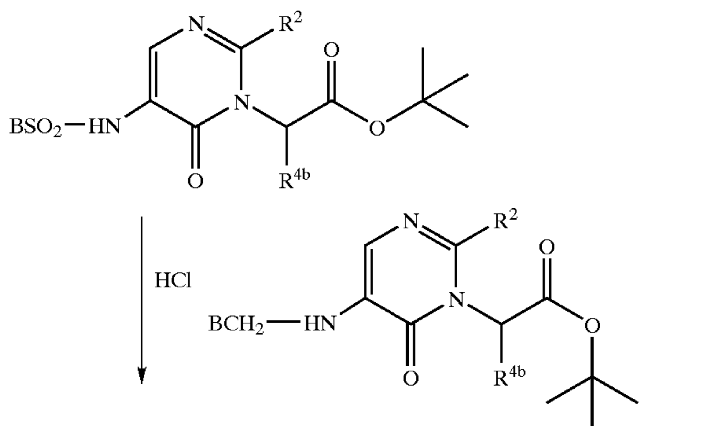
Scheme 5: General Pyrimidinone Synthesis-I (Concluded)
