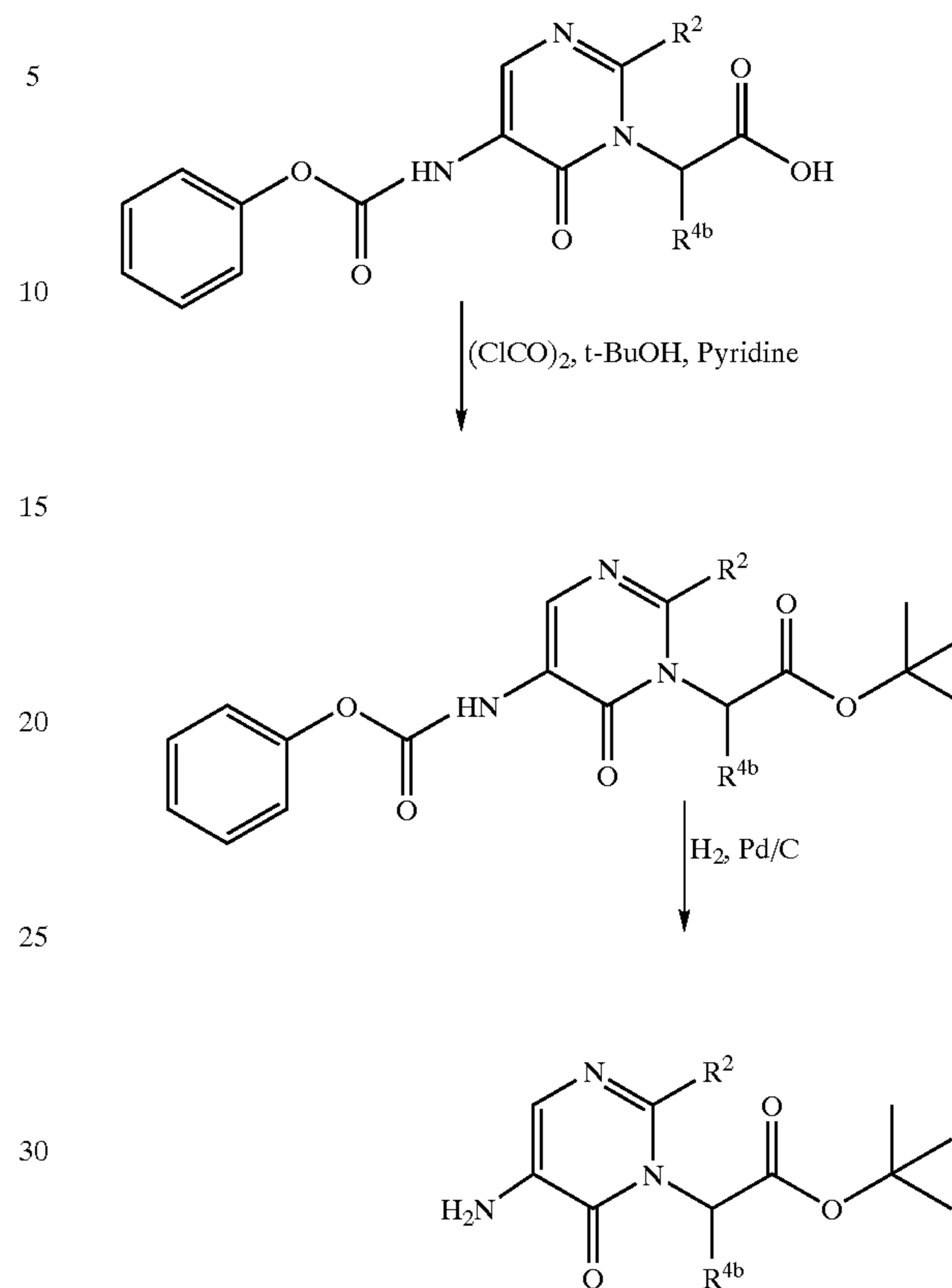
Scheme 2: General Pyrimidinone Synthesis-I (Continued)
