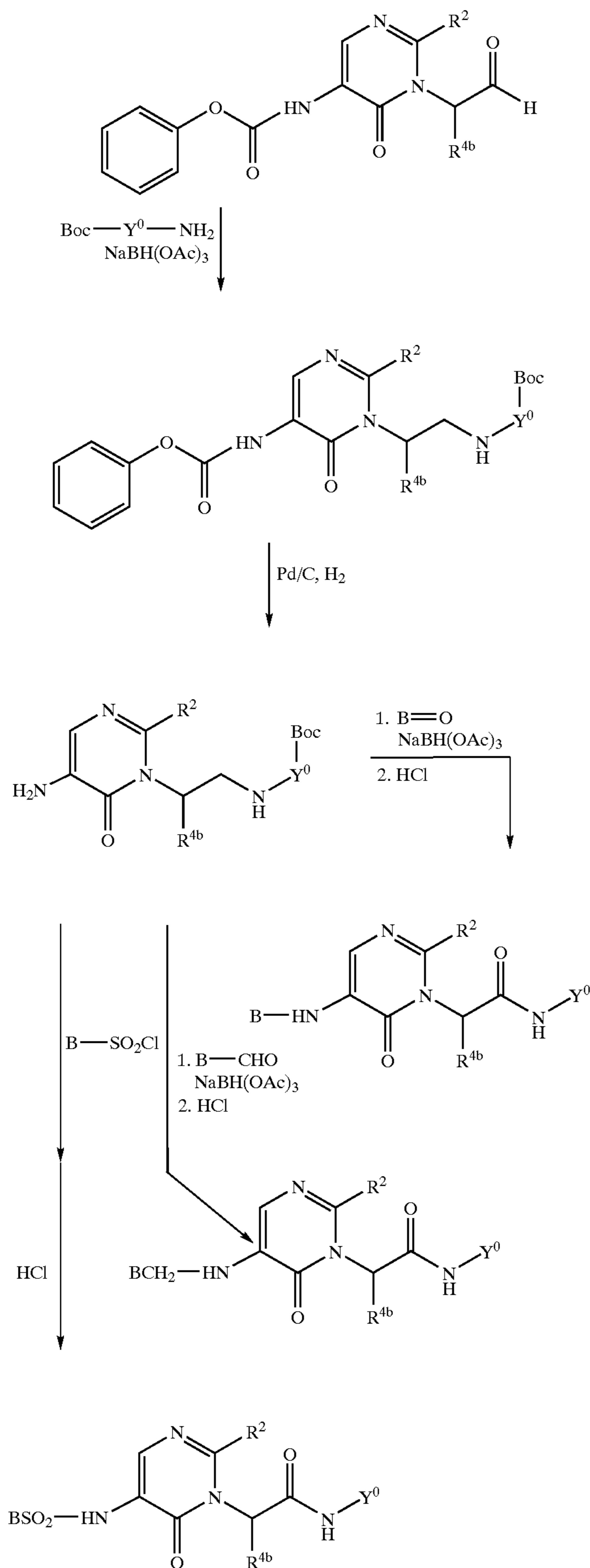
Scheme 8: General Methylene Pyrimidinone Synthesis
