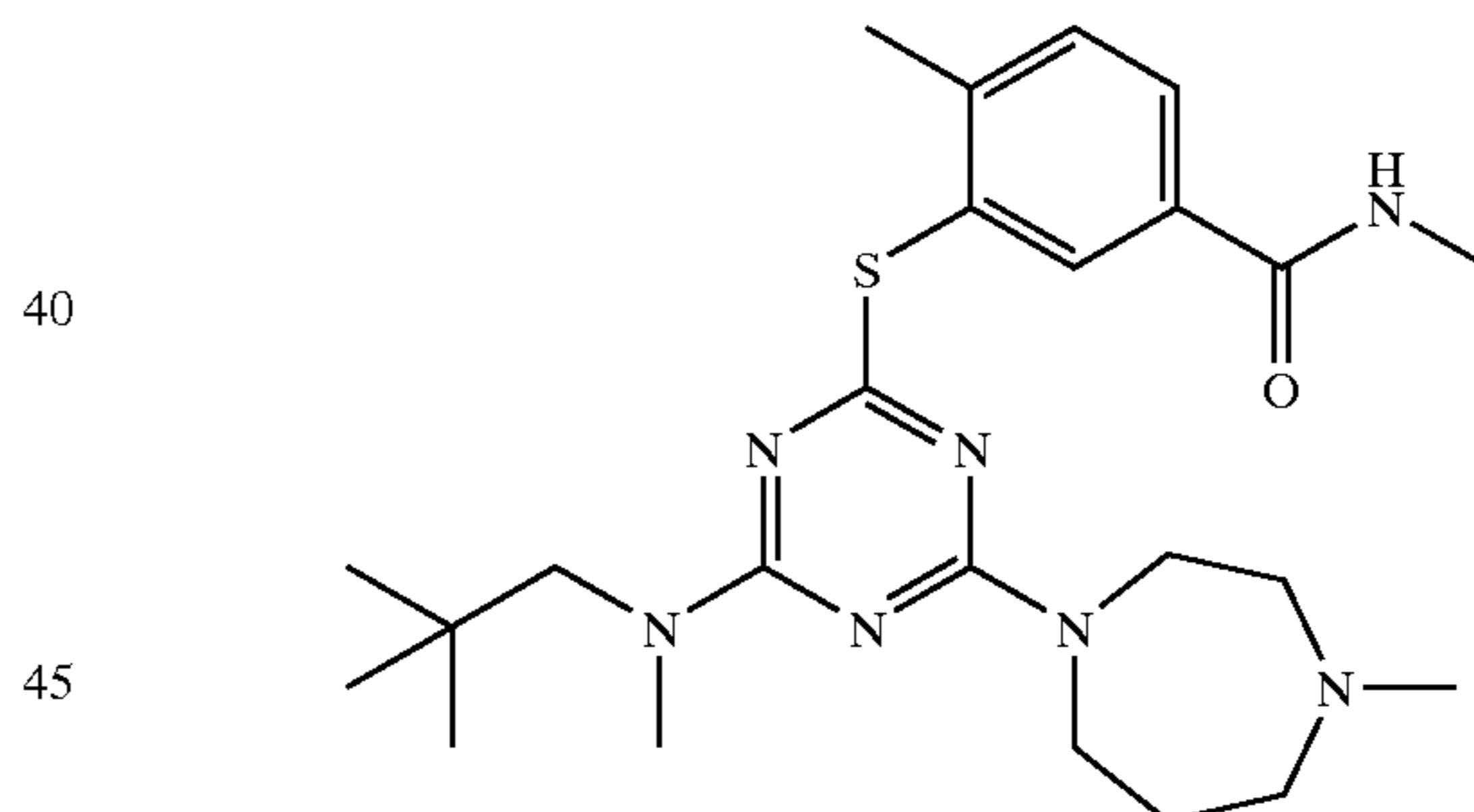
Compound N
