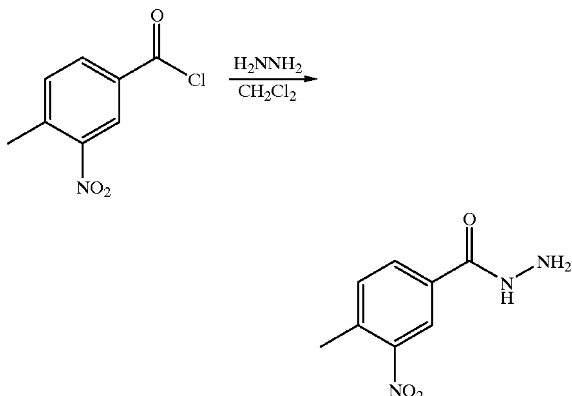
2-(4-Methyl-3-nitro-phenyl)-[1,3,4]oxadiazole
