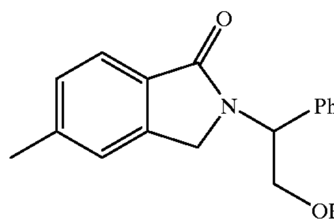
2-(2-Hydroxy-1-phenyl-ethyl)-5-methyl-2,3-dihydro-isoindol-1-one
