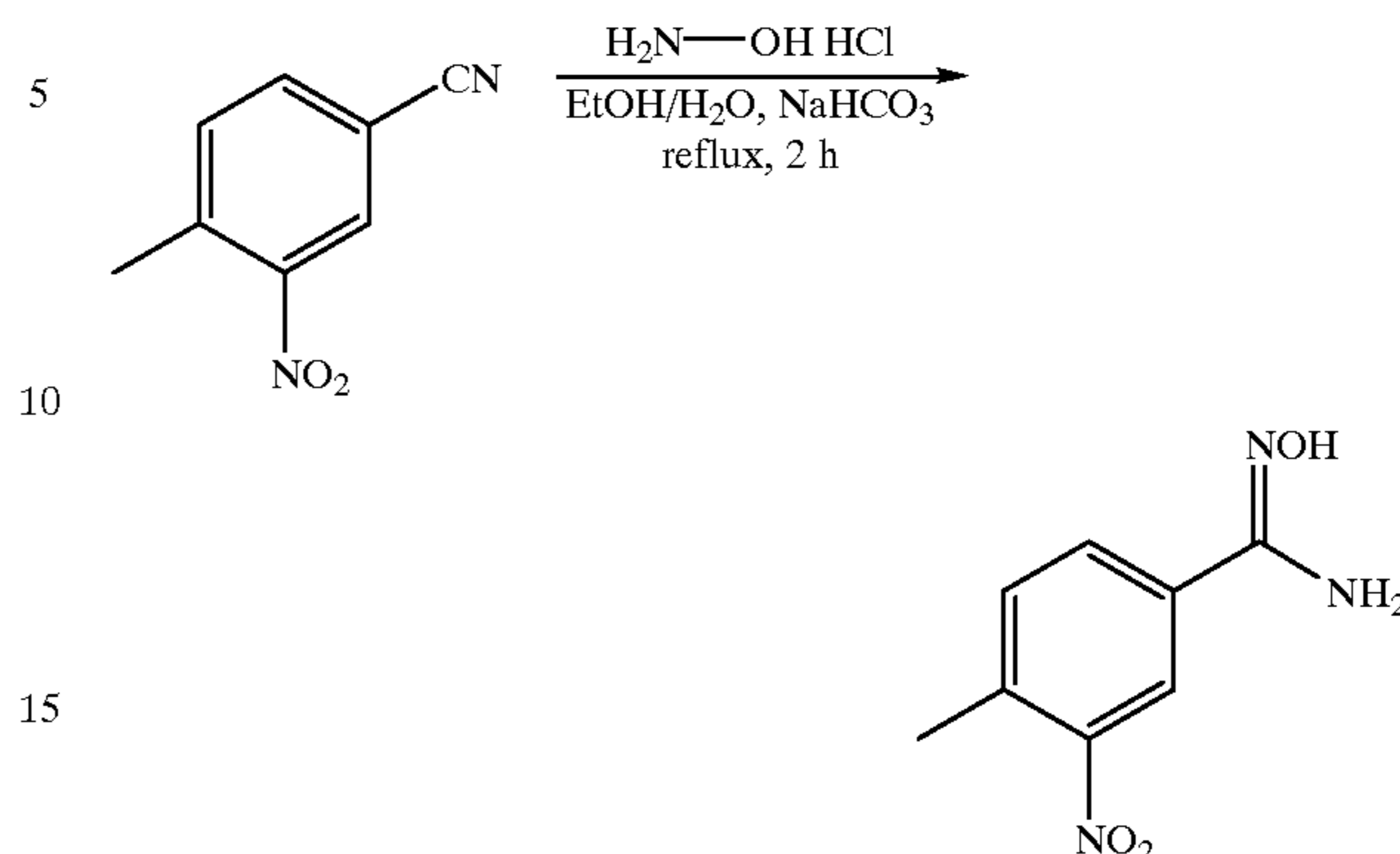
2-Methyl-5-(5-methyl-[1,2,4]oxadiazol-3-yl)-phenylamine
