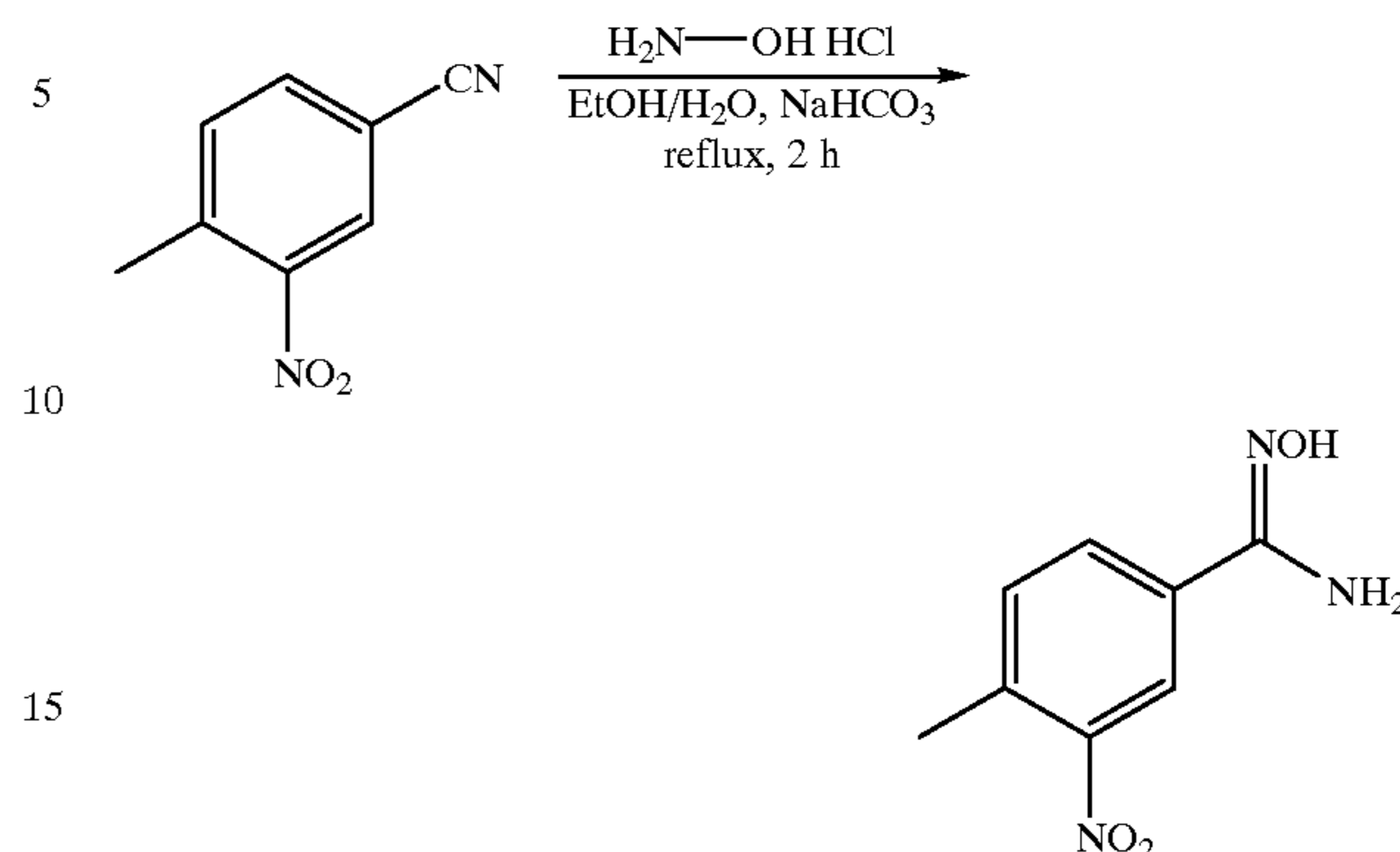
2-Methyl-5-(5-methyl-[1,2,4]oxadiazol-3-yl)-phenylamine
