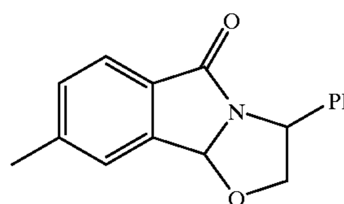
8-Methyl-3-phenyl-2,3-dihydro-9bH-oxazolo[2,3-α]isoindol-5-one
