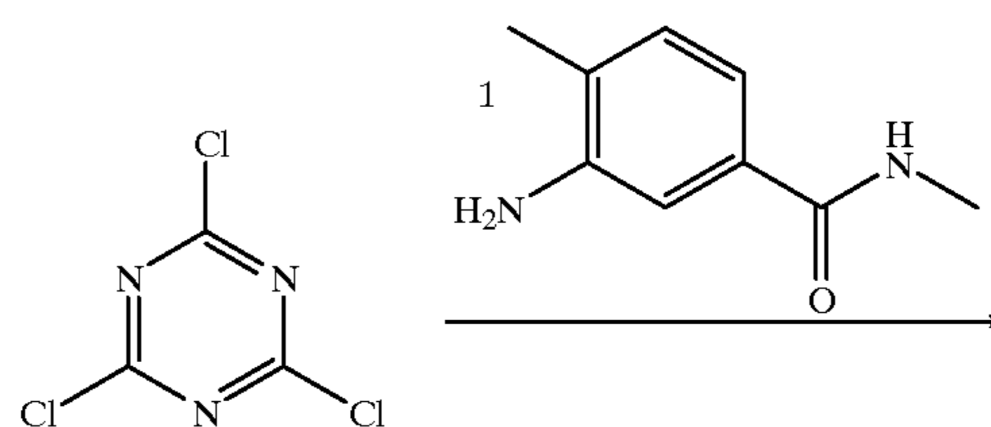
Scheme 1
