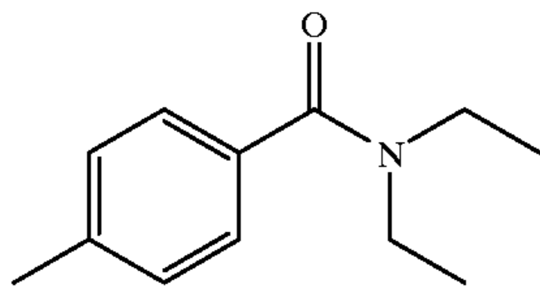
N,N-Diethyl-4-methyl-benzamide
