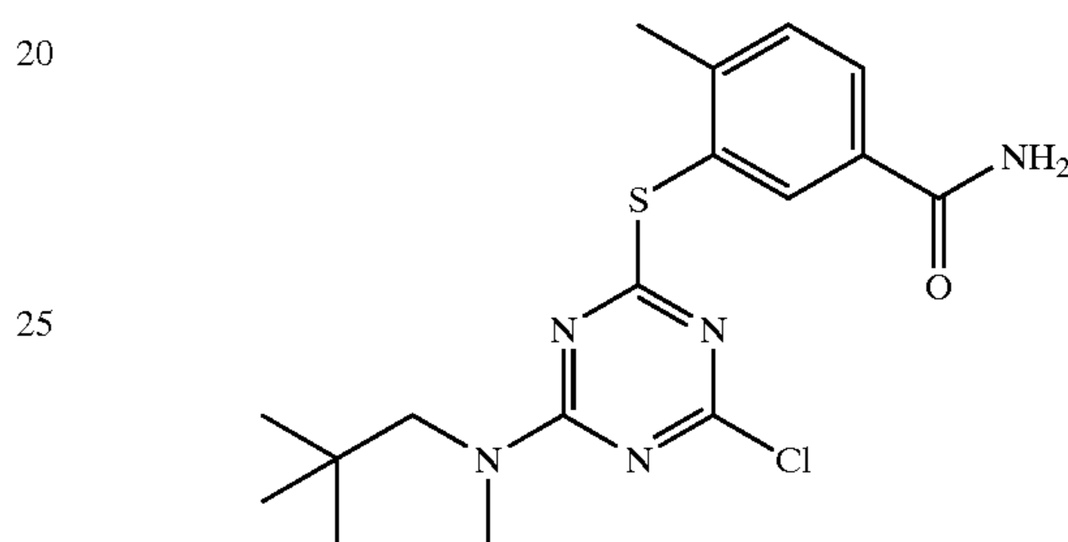
Compound M
