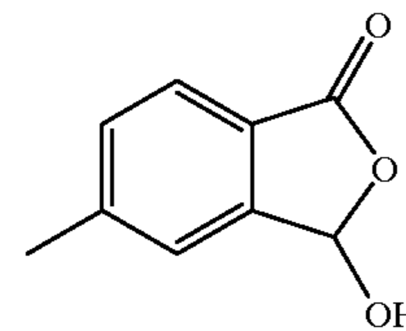
3-Hydroxy-5-methyl 3H-isobenzofuran-1-one
