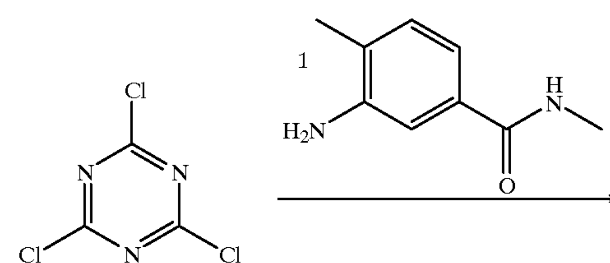
Scheme 1
