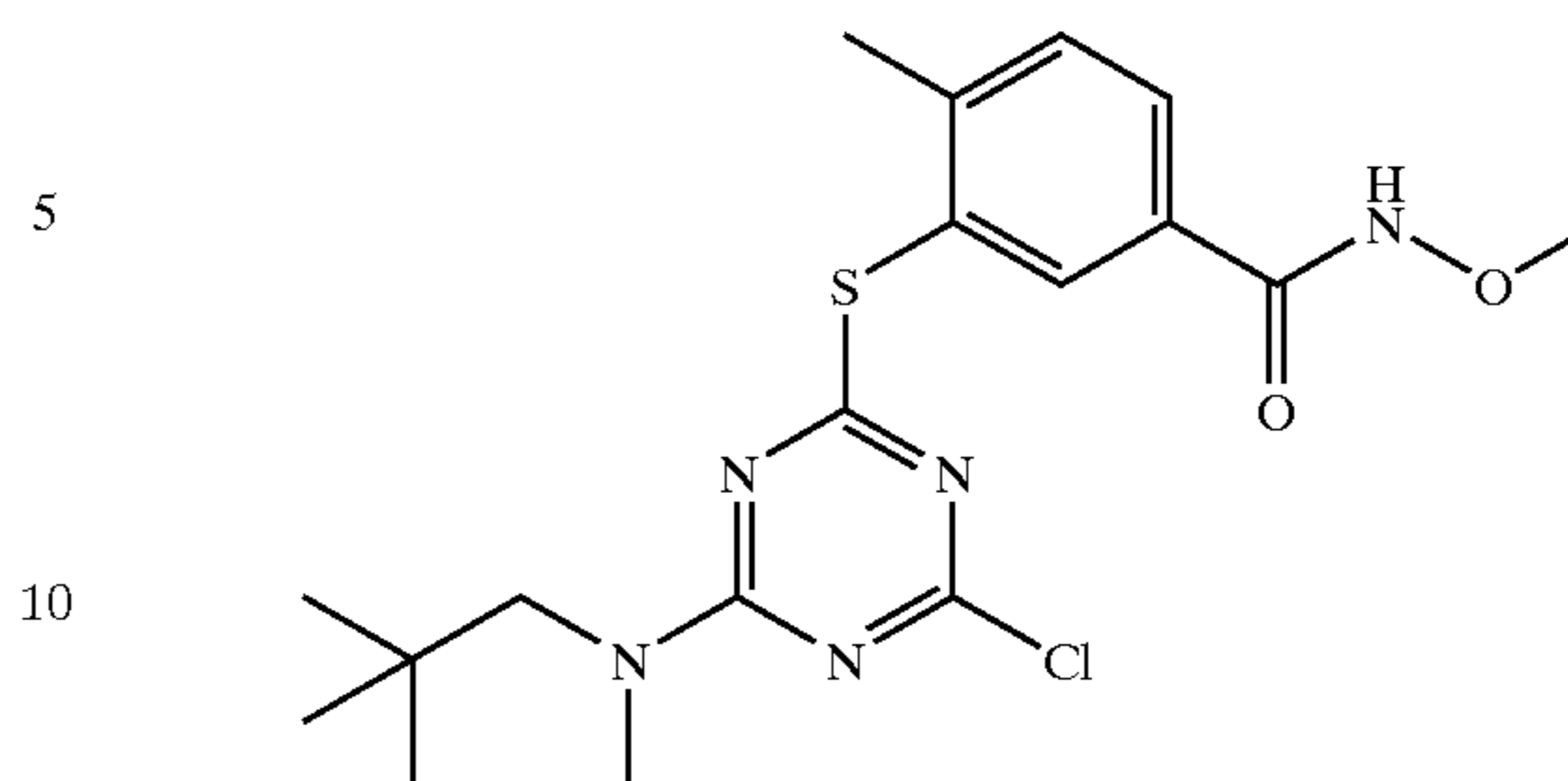
Compound L
