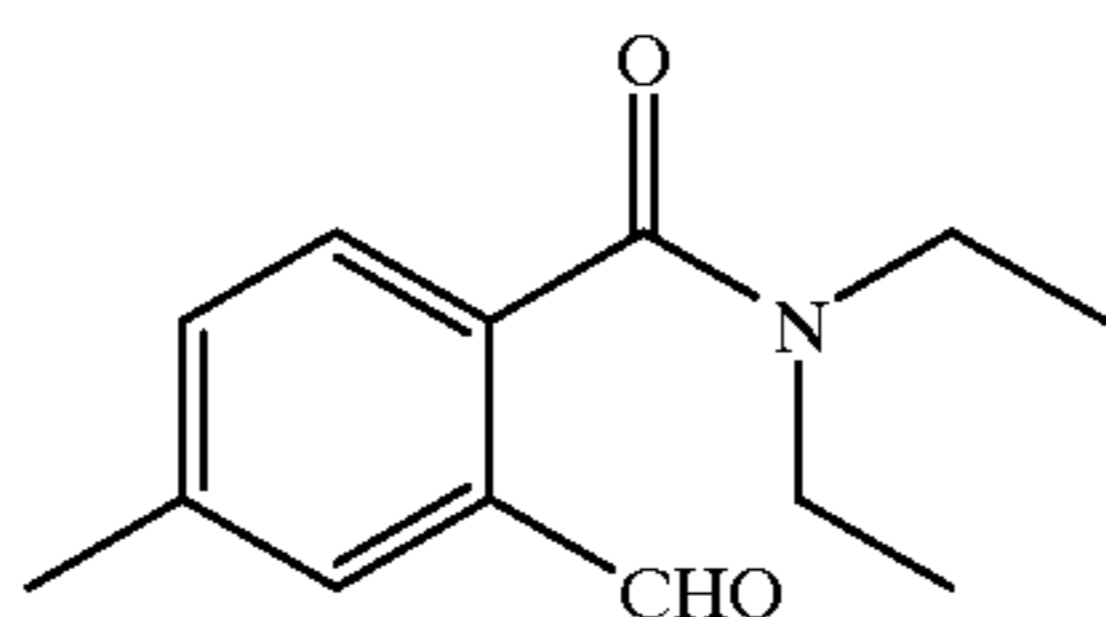
N,N-Diethyl-2-formyl-4-methyl-benzamide
