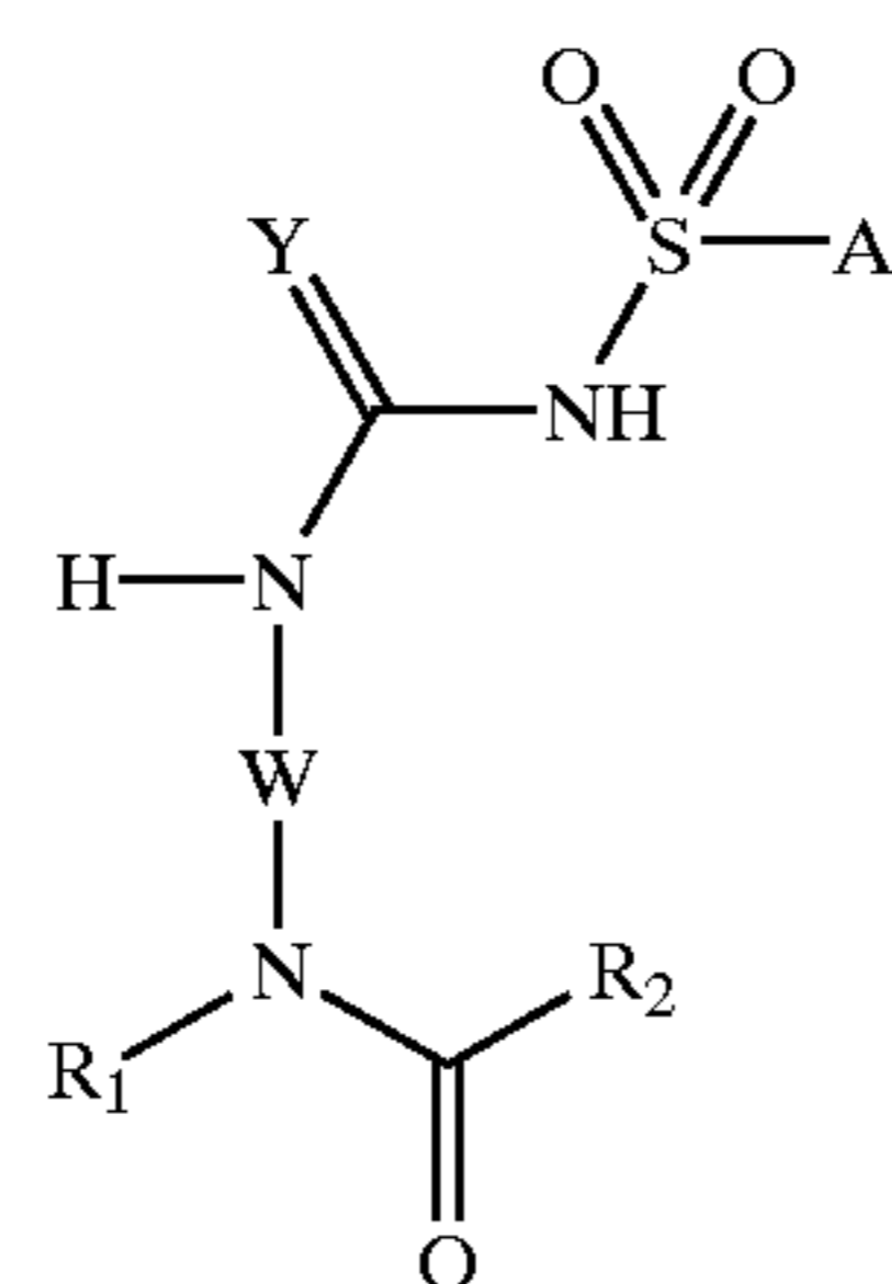
Formula Ia
