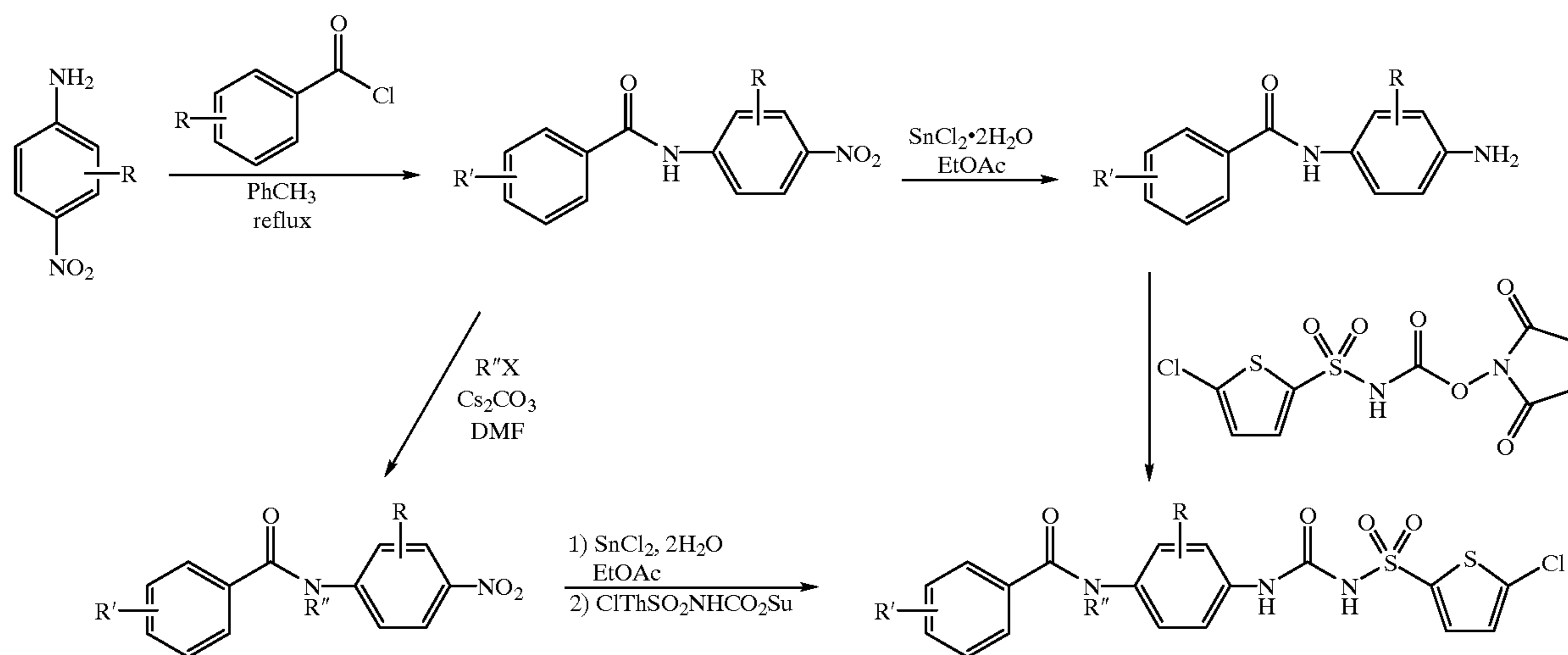
Scheme 3 Benzamide-containing Sulfonylureas
