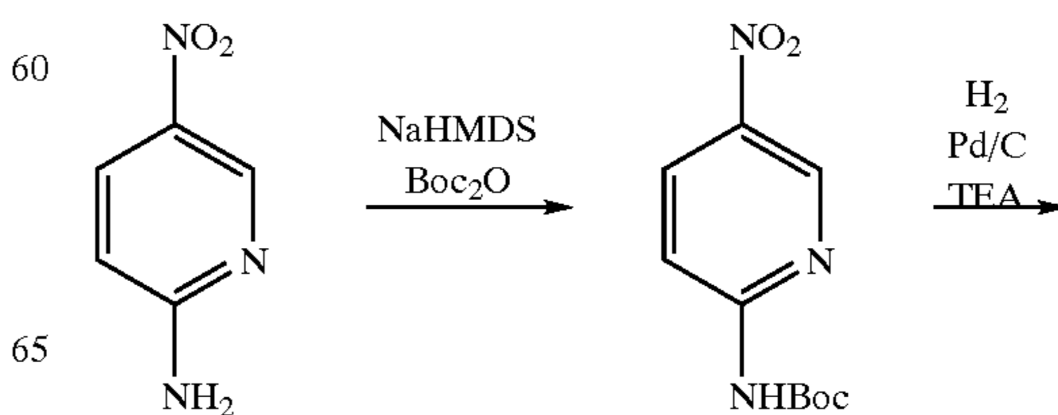
Scheme 2
