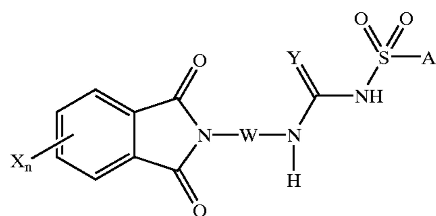
Formula Ib
