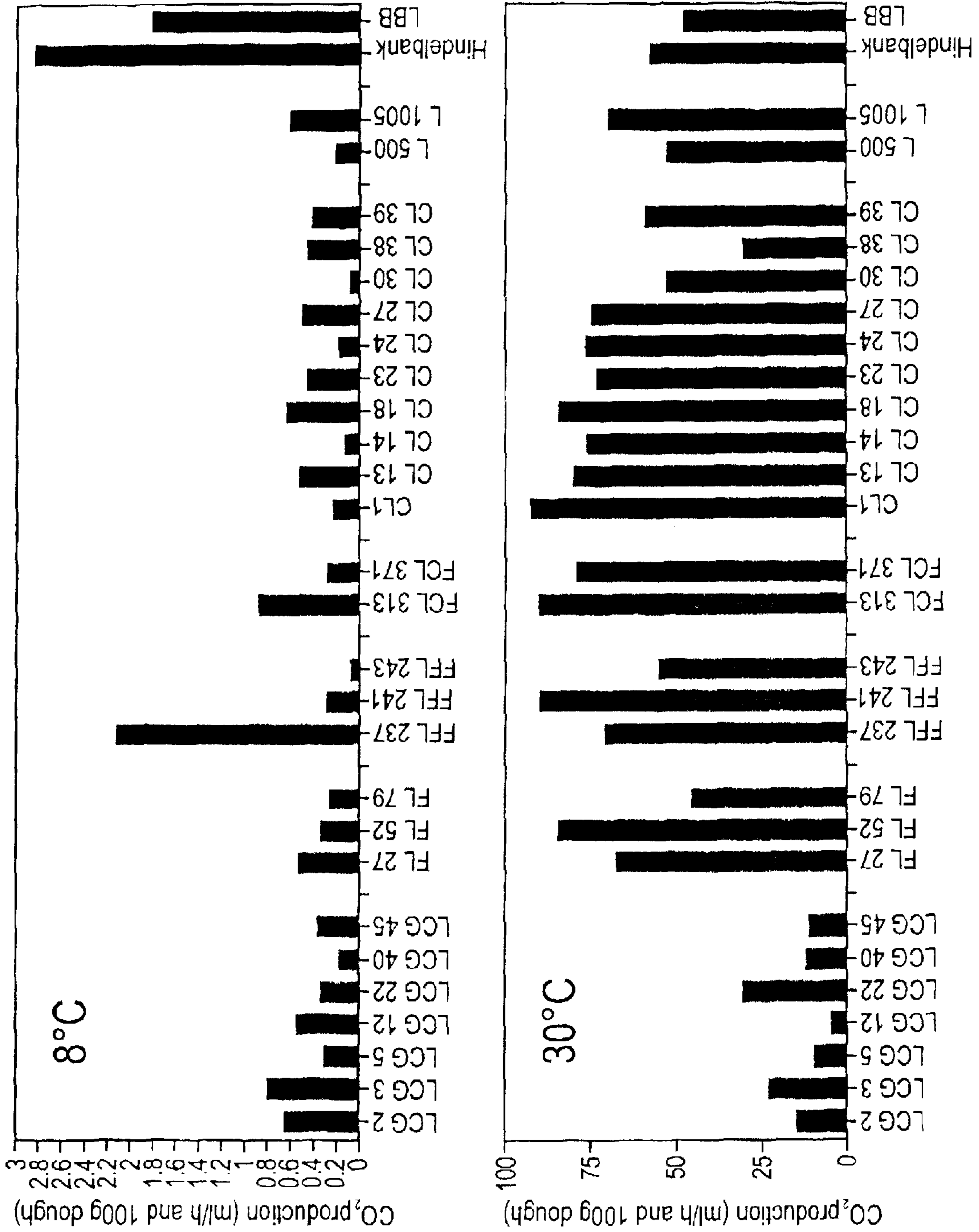
Figure 1: Initial CO 2 formation rates of LTI strains grown with the dough screening procedure
