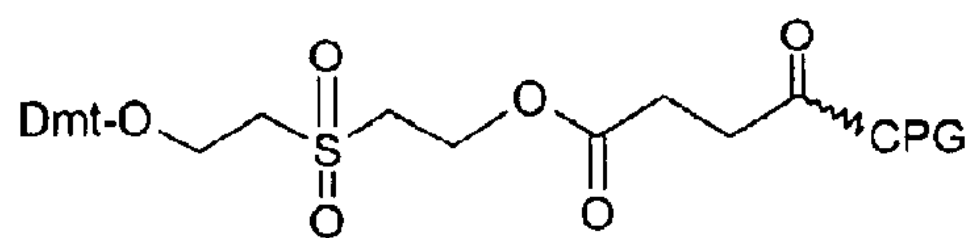
Bishydroxyethylsulfonyl support 1
