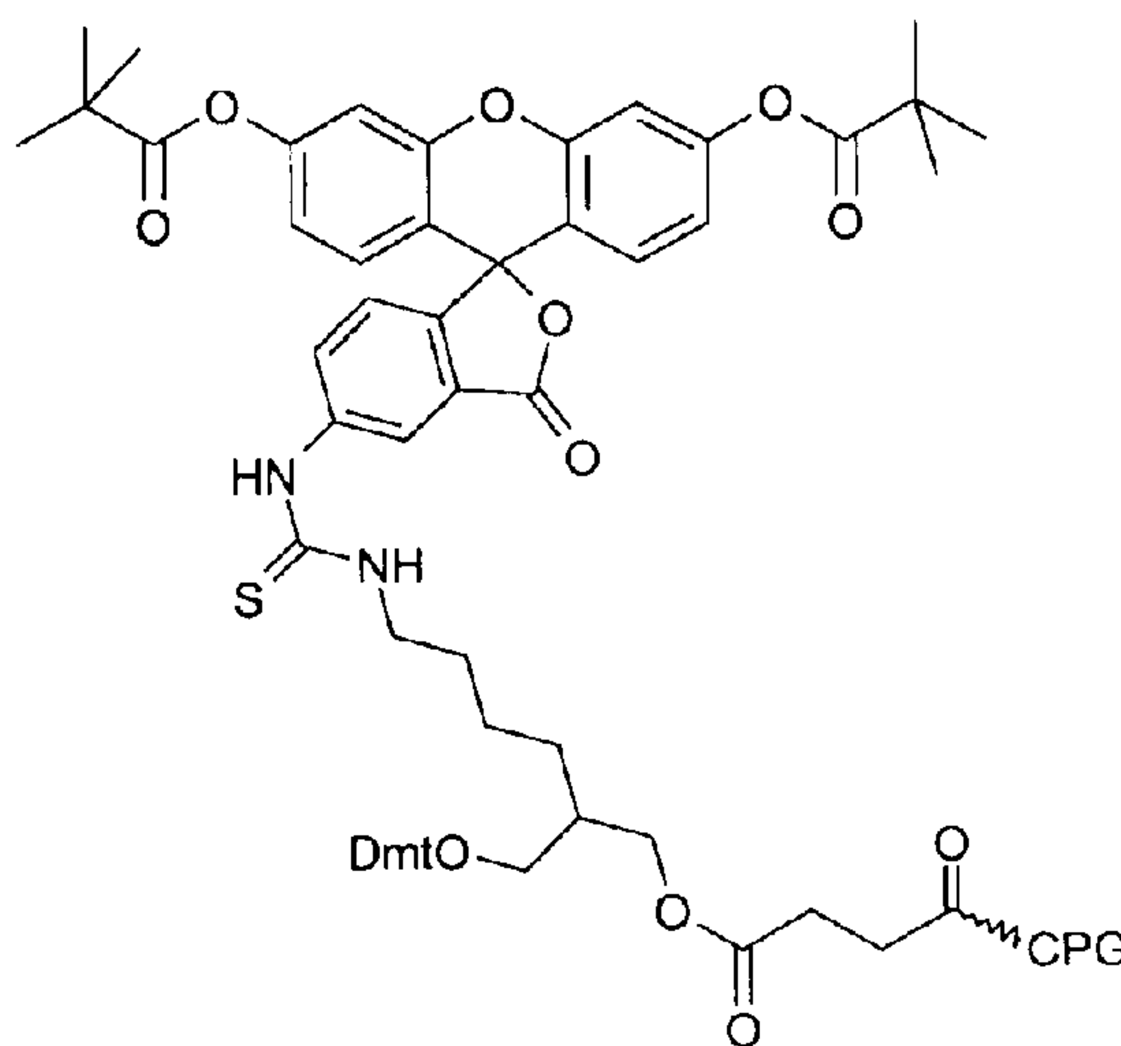
Fluorescein support 3
