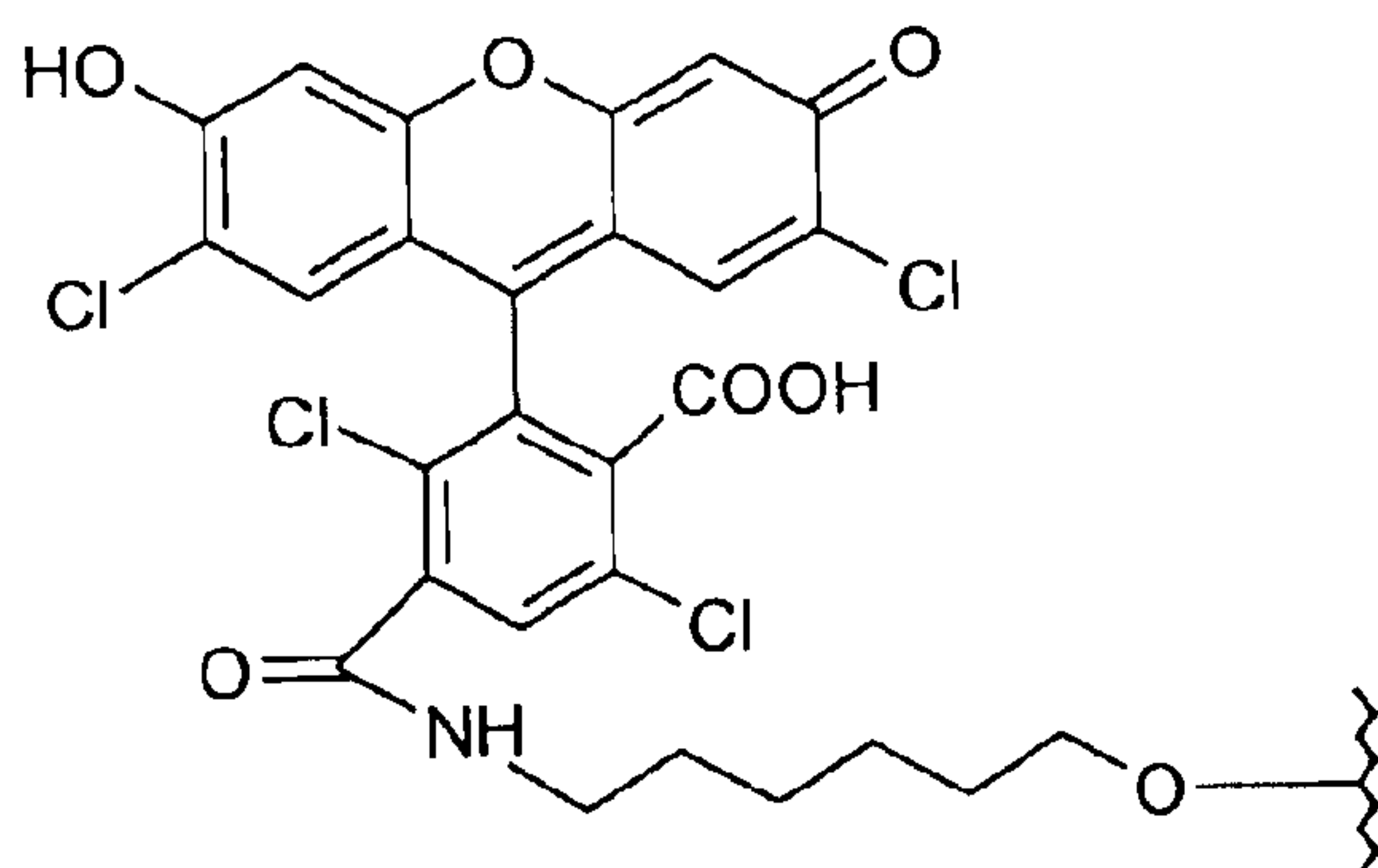
Tetrachlorofluorescein
