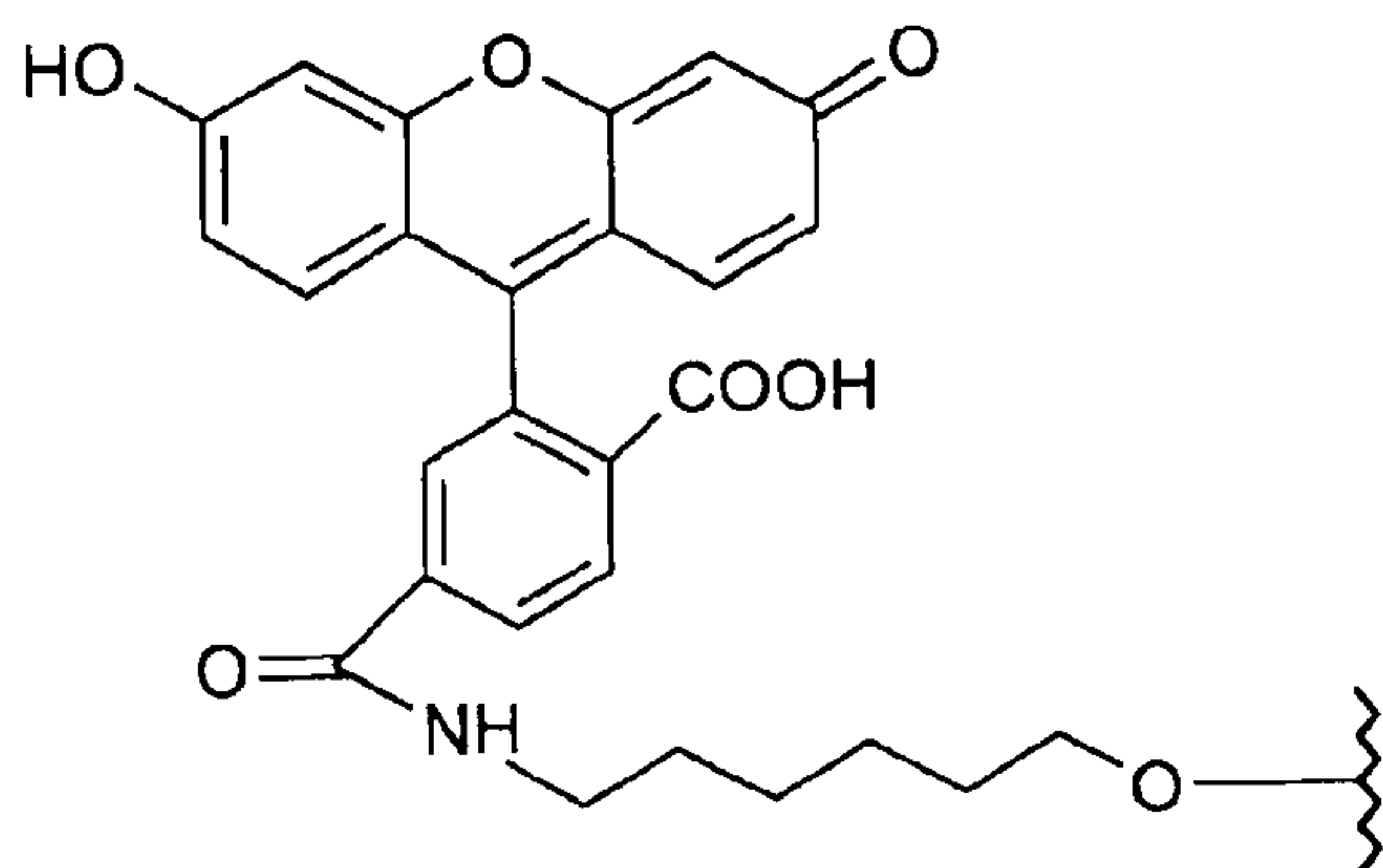
Fluorescein (Amide)
