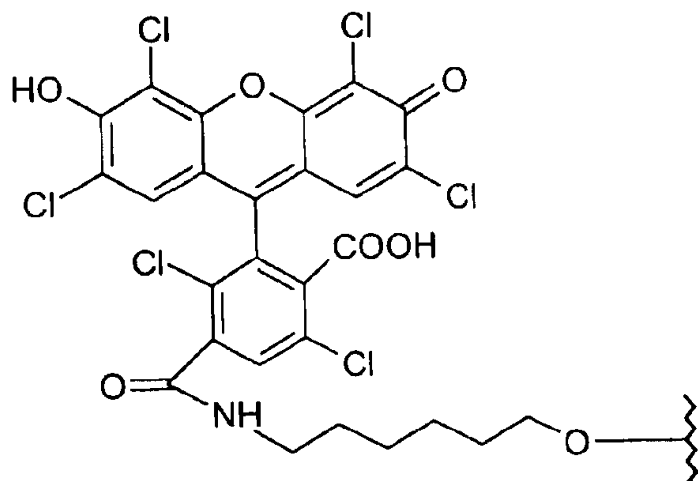
Hexachlorofluorescein
