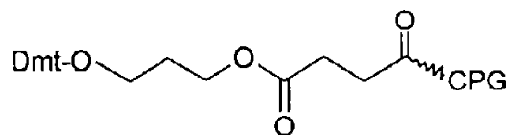
3'-Spacer-C3 support 2
