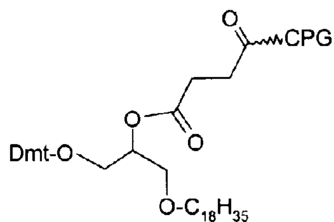
3'-BatyI support 4
