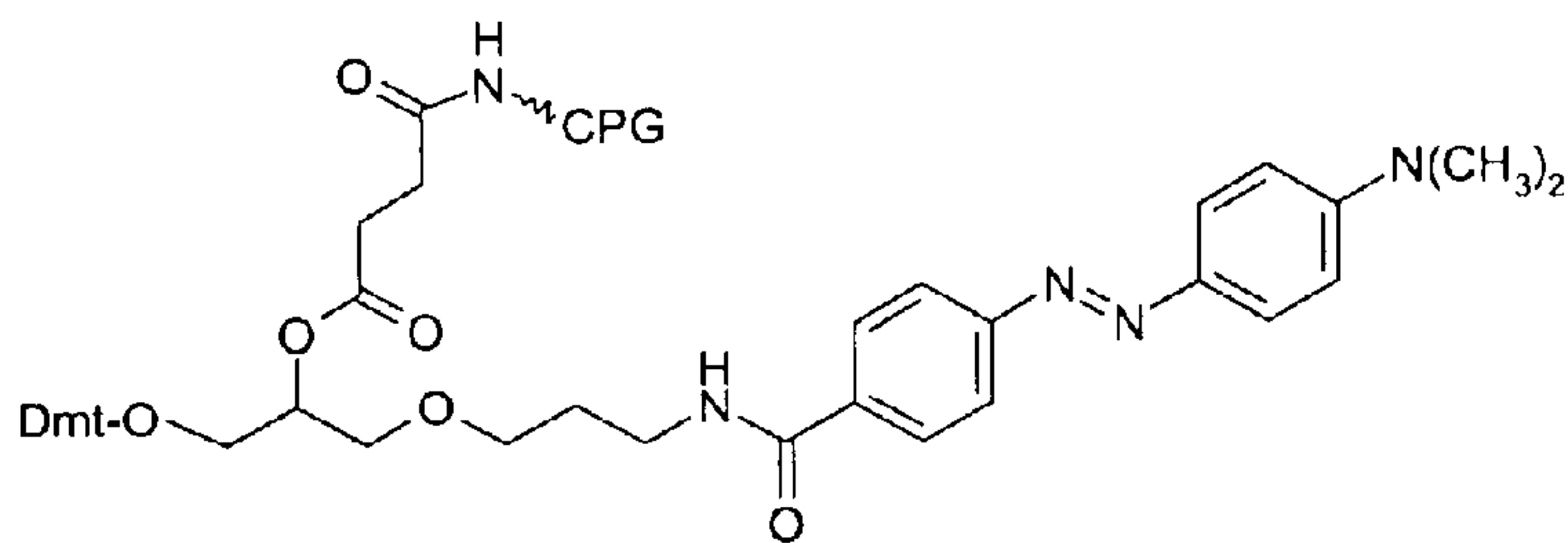
DABCYL support 6
