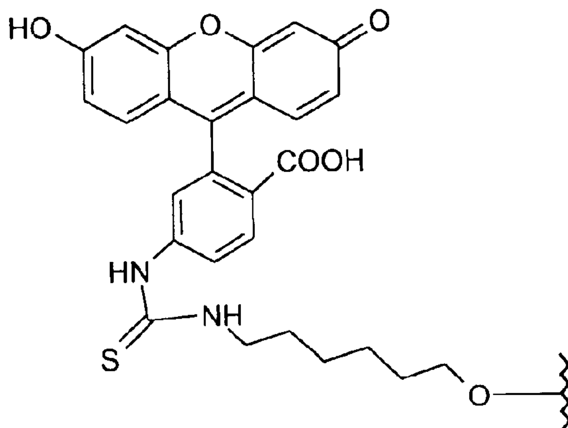
Fluorescein (Thiourea)
