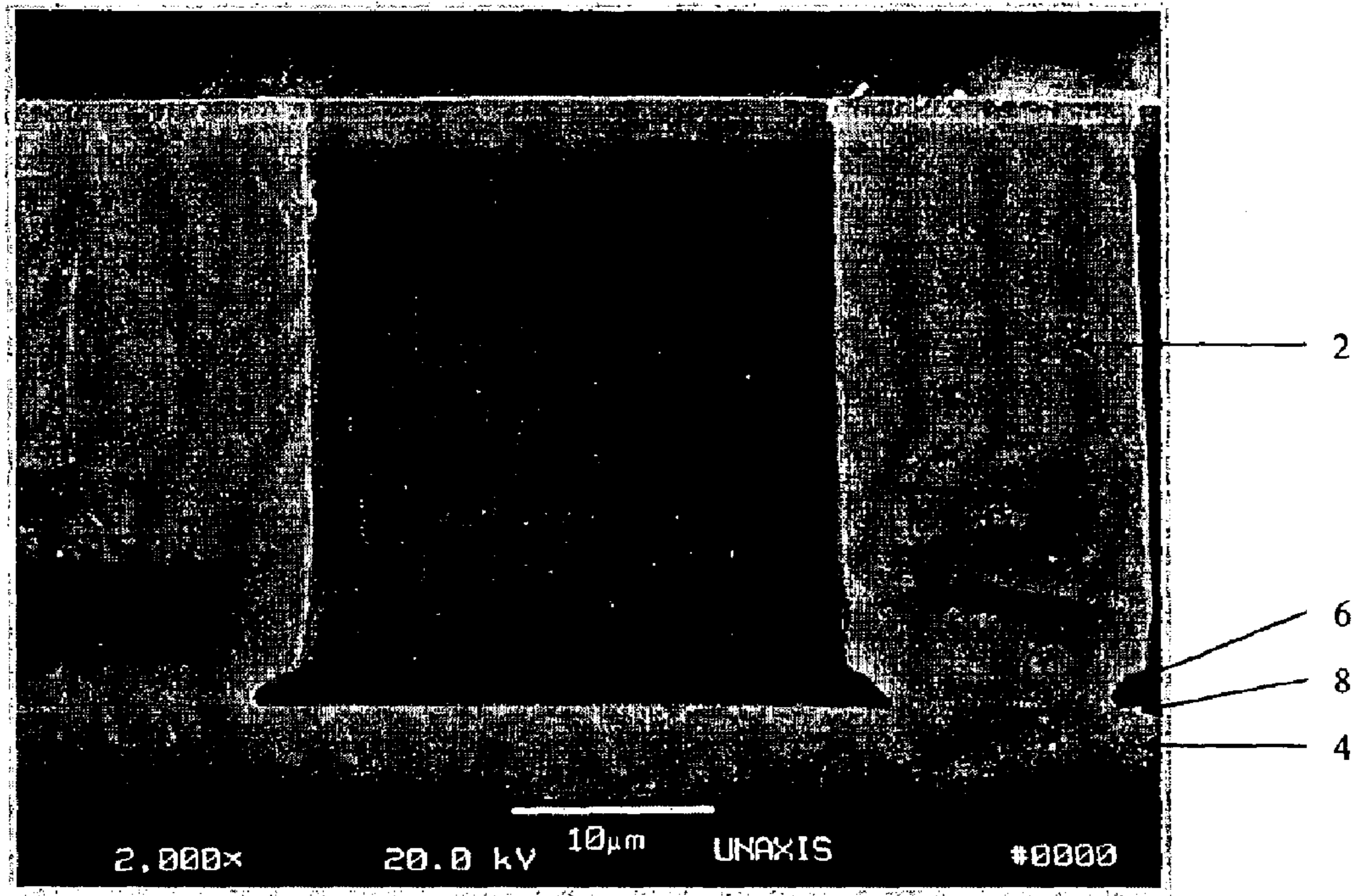
Figure 1 SOI feature etched using no pulsing (prior art)
