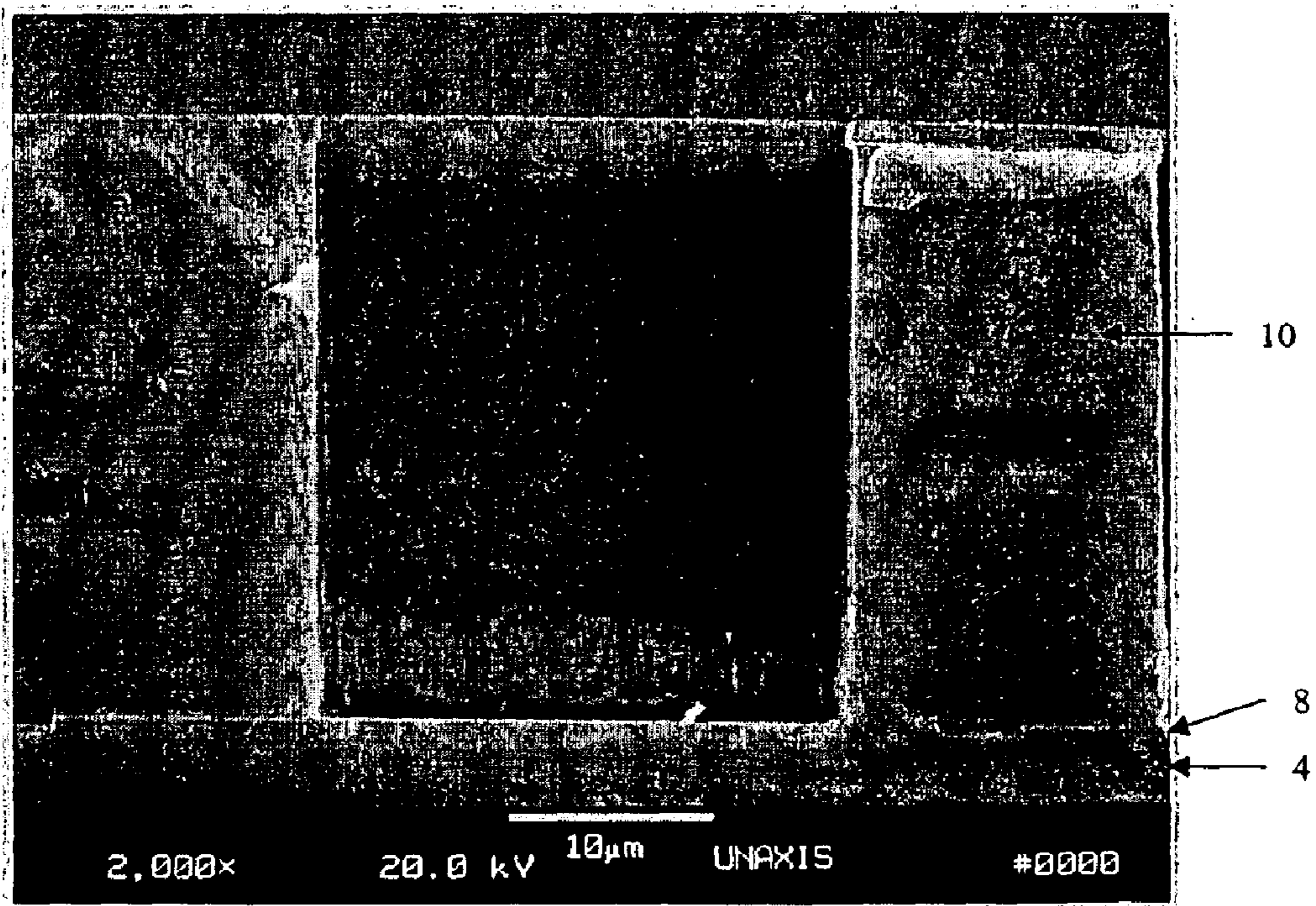
Figure 2 Same feature as Fig 1, using ICP pulsing
