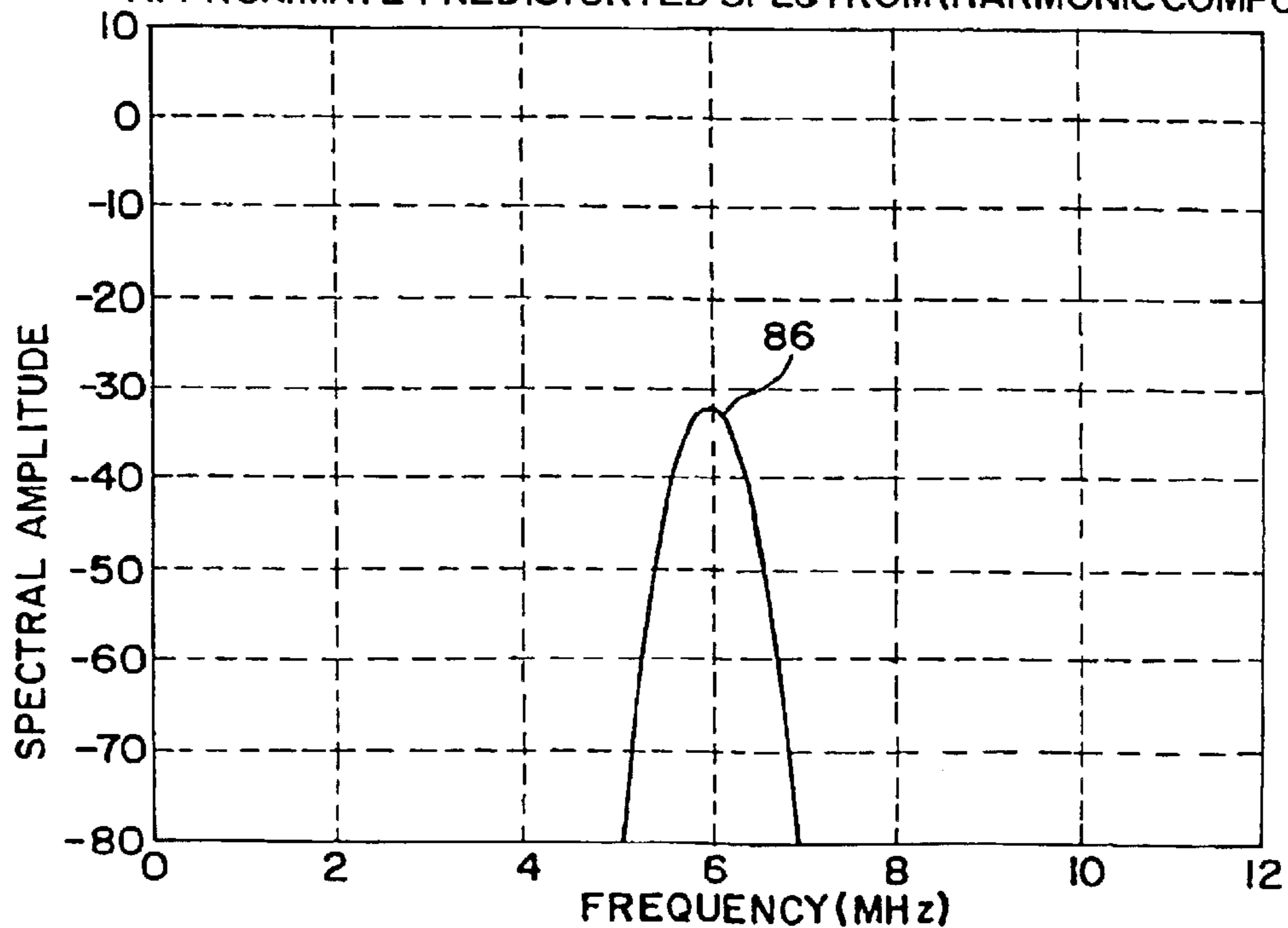
APPROXIMATE PREDISTORTED SPECTRUM (HARMONIC COMPONENT)
