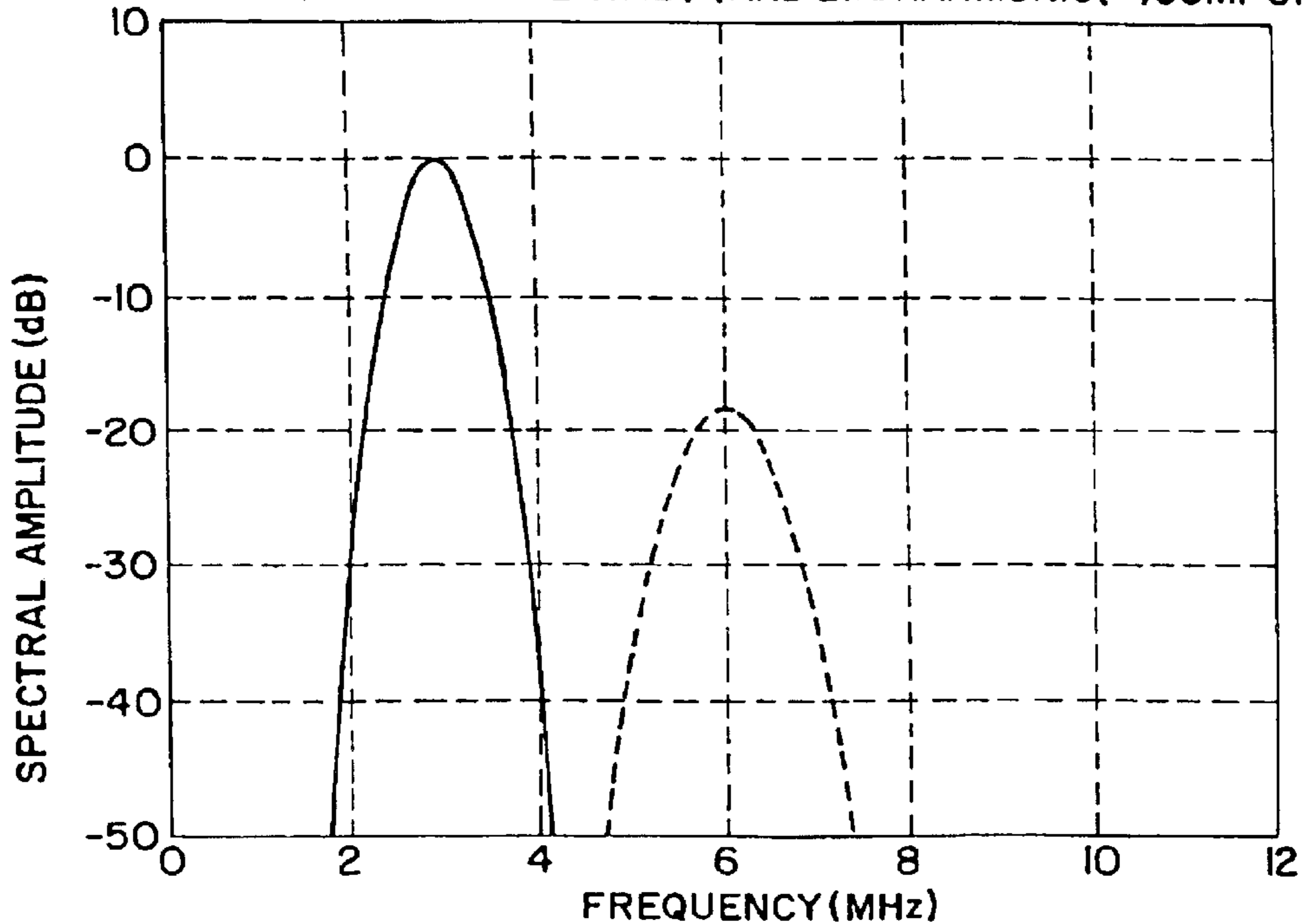
SOURCE SPECTRUM:FUNDAMENTAL (-)AND 2nd HARMONIC(--)-COMPONENTS
