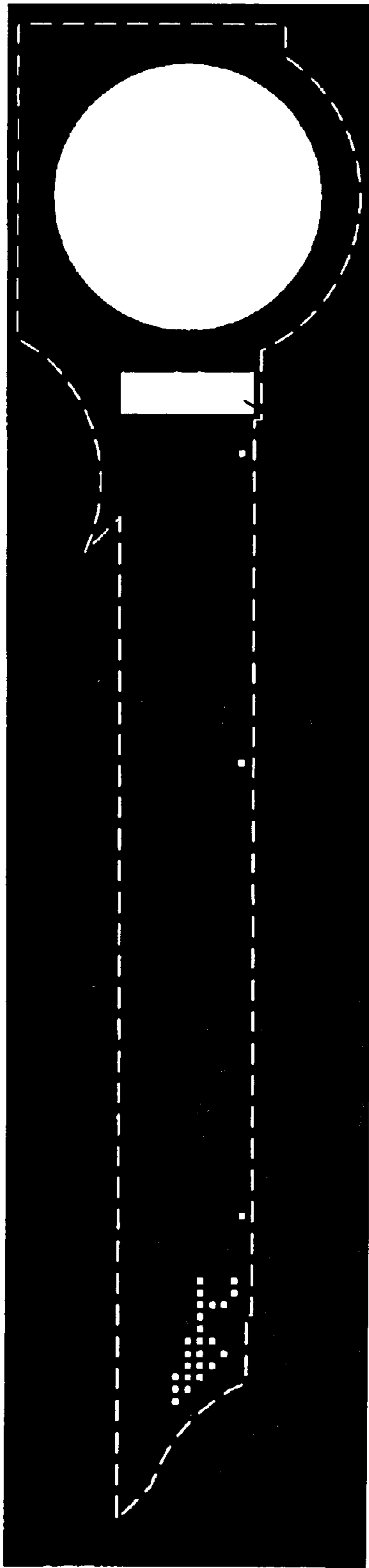
Via 2 mask
