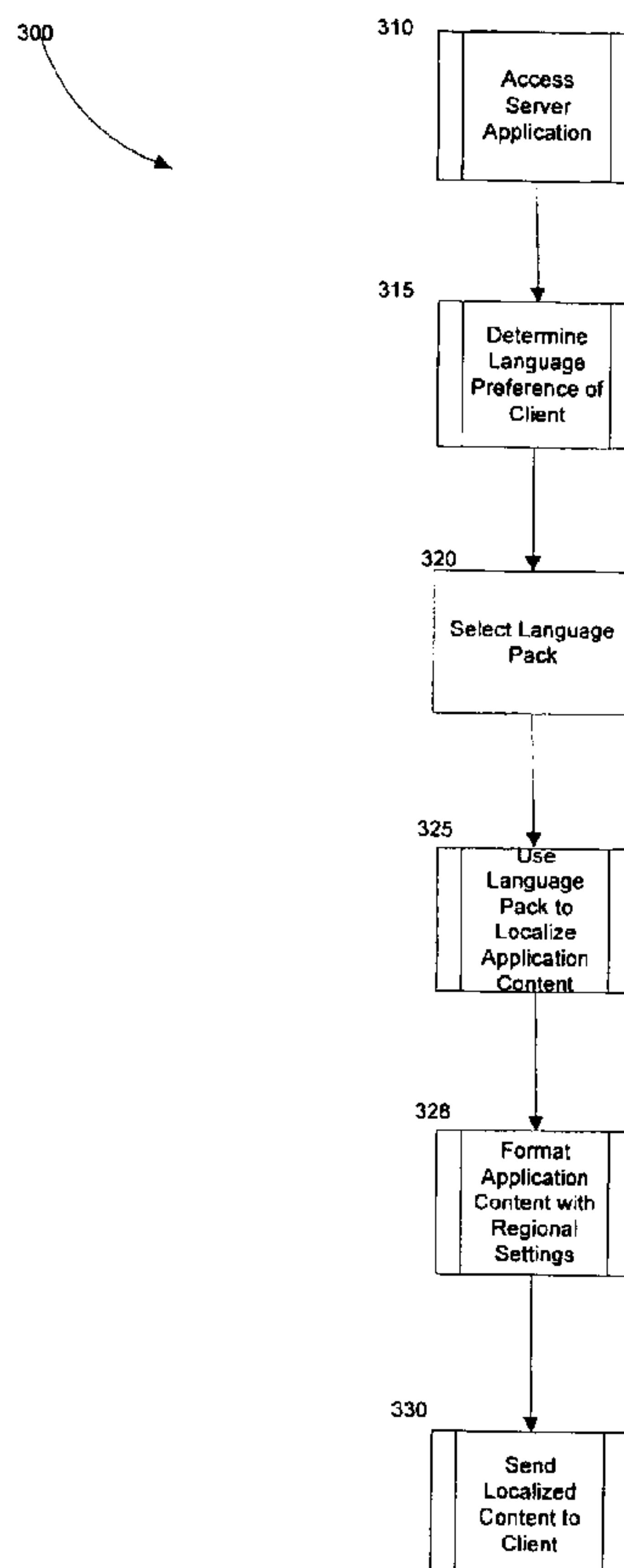
Overview of Language Localization Process with Regional Settings
