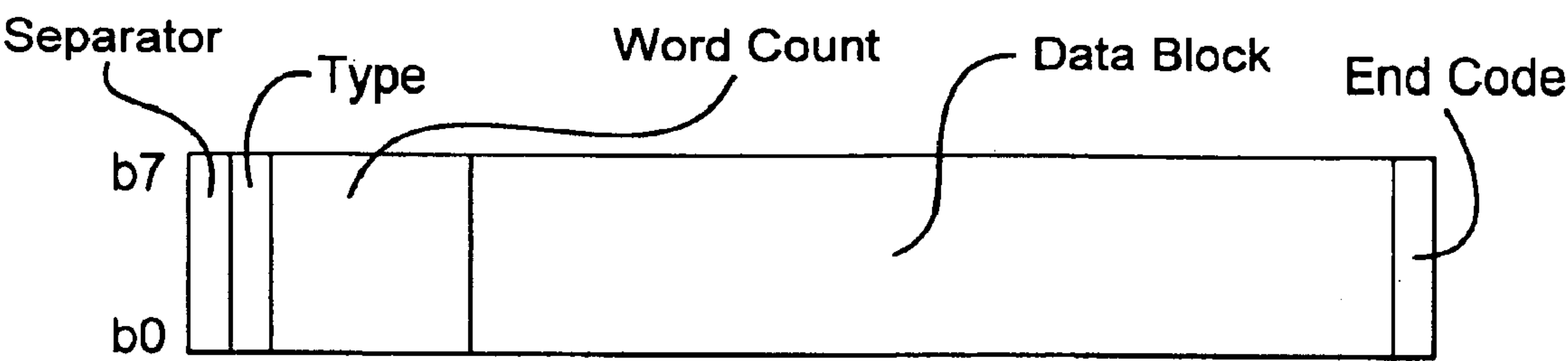
Fig. 10 : Format of the SDTI Variable Block
