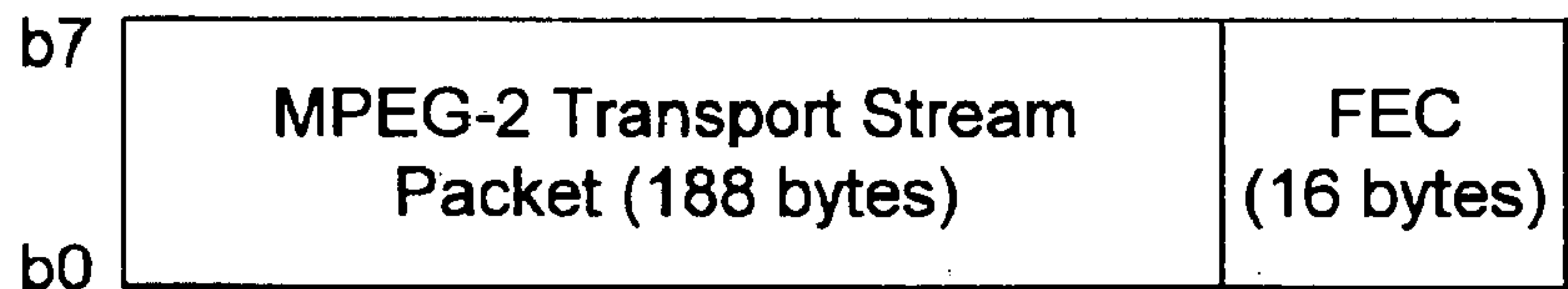
Fig. 2b : MPEG-2 Transport Stream Packet with Active 16 bytes FEC
