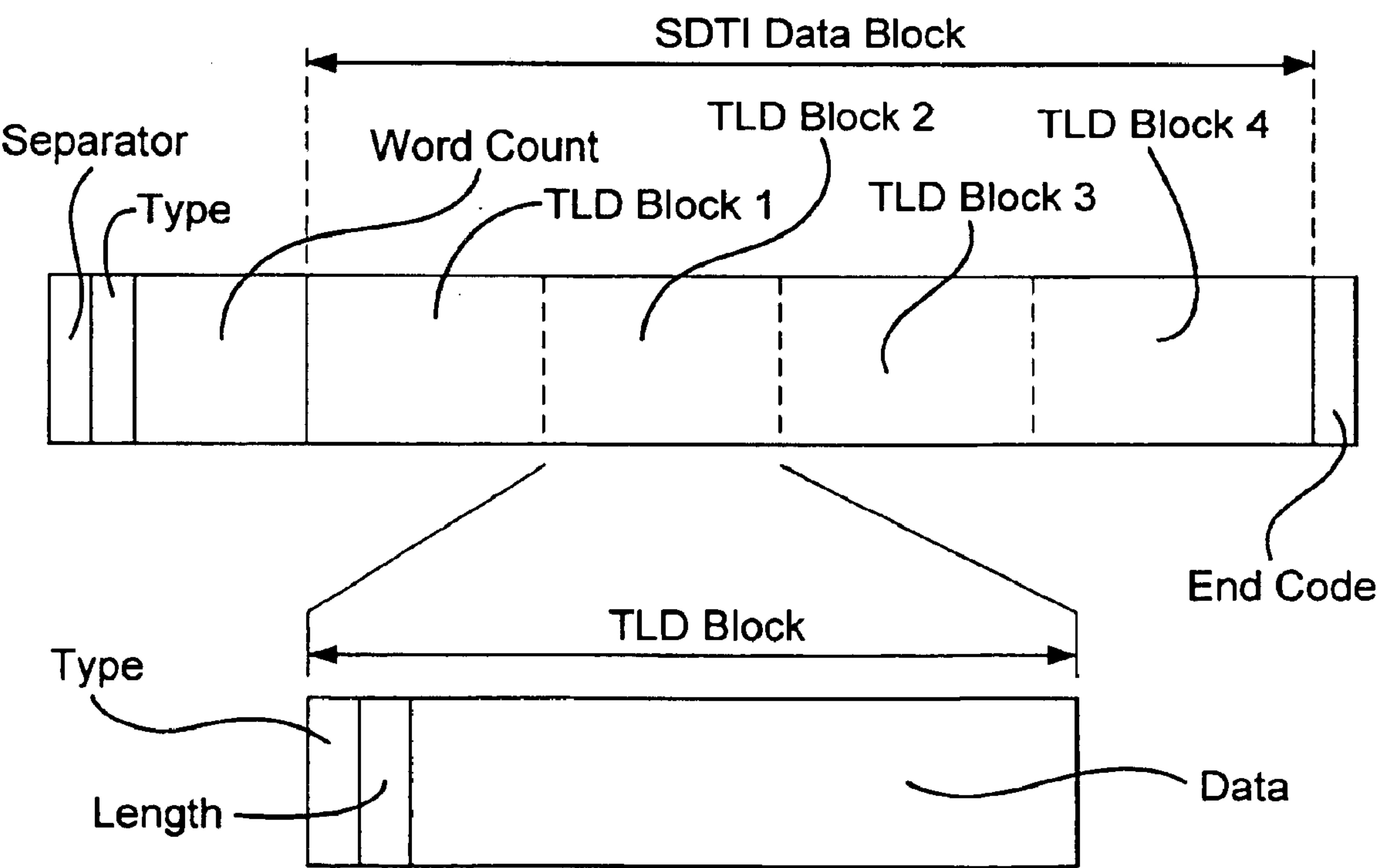
Fig. 12 : Hierarchy of SDTI Variable Blocks and TLD Blocks
