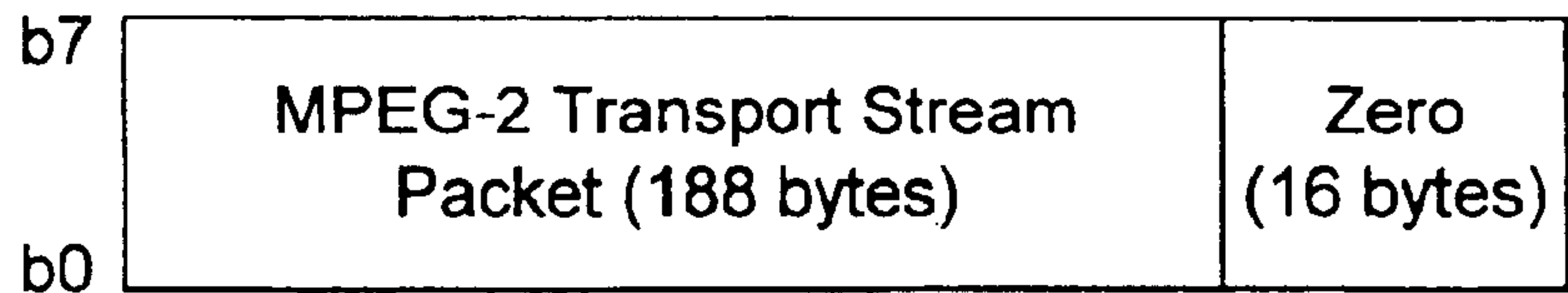
Fig. 2c : MPEG-2 Transport Stream Packet with Null FEC Space
