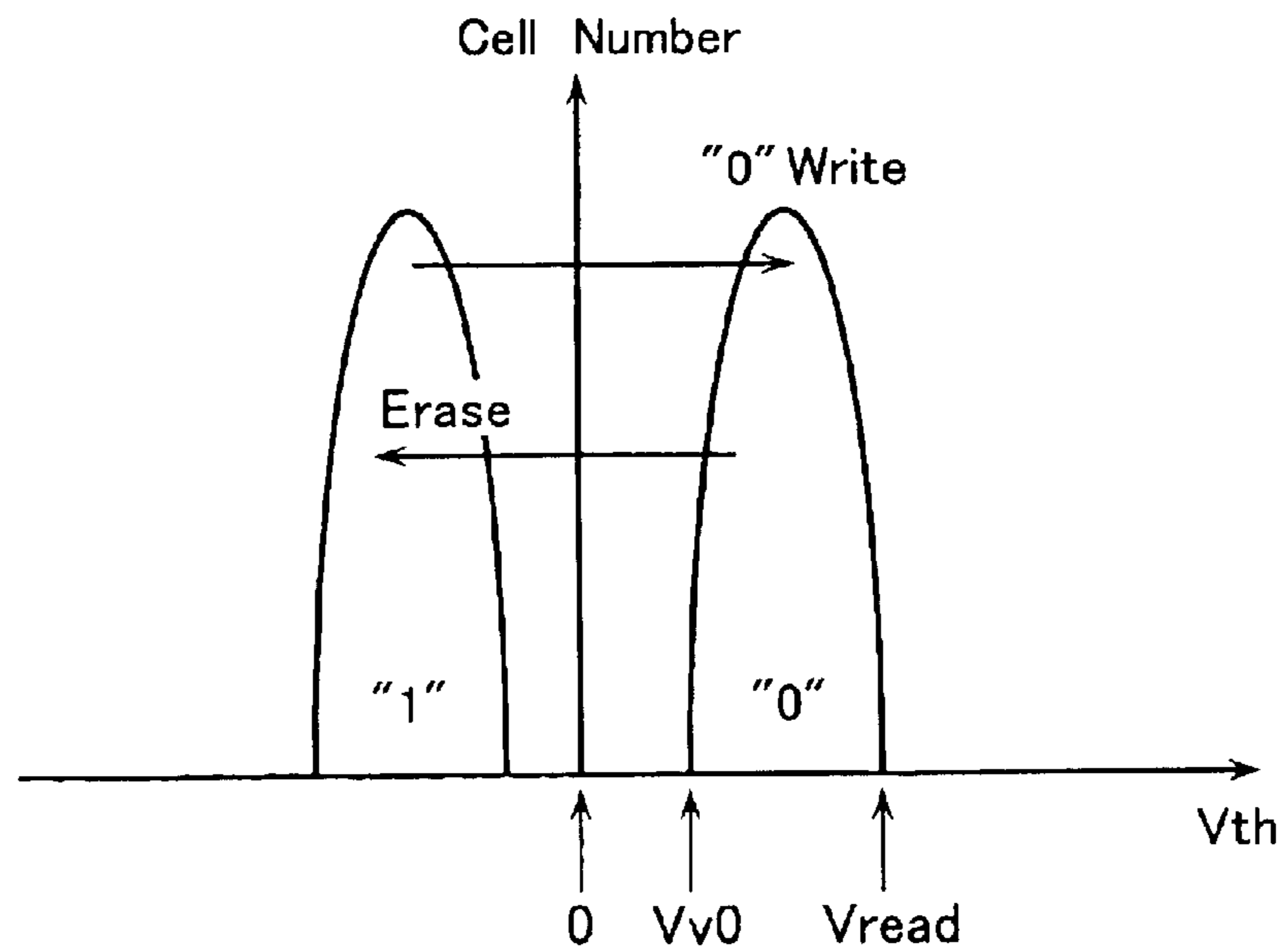
[Cell Array Threshold Voltage Distribution]
