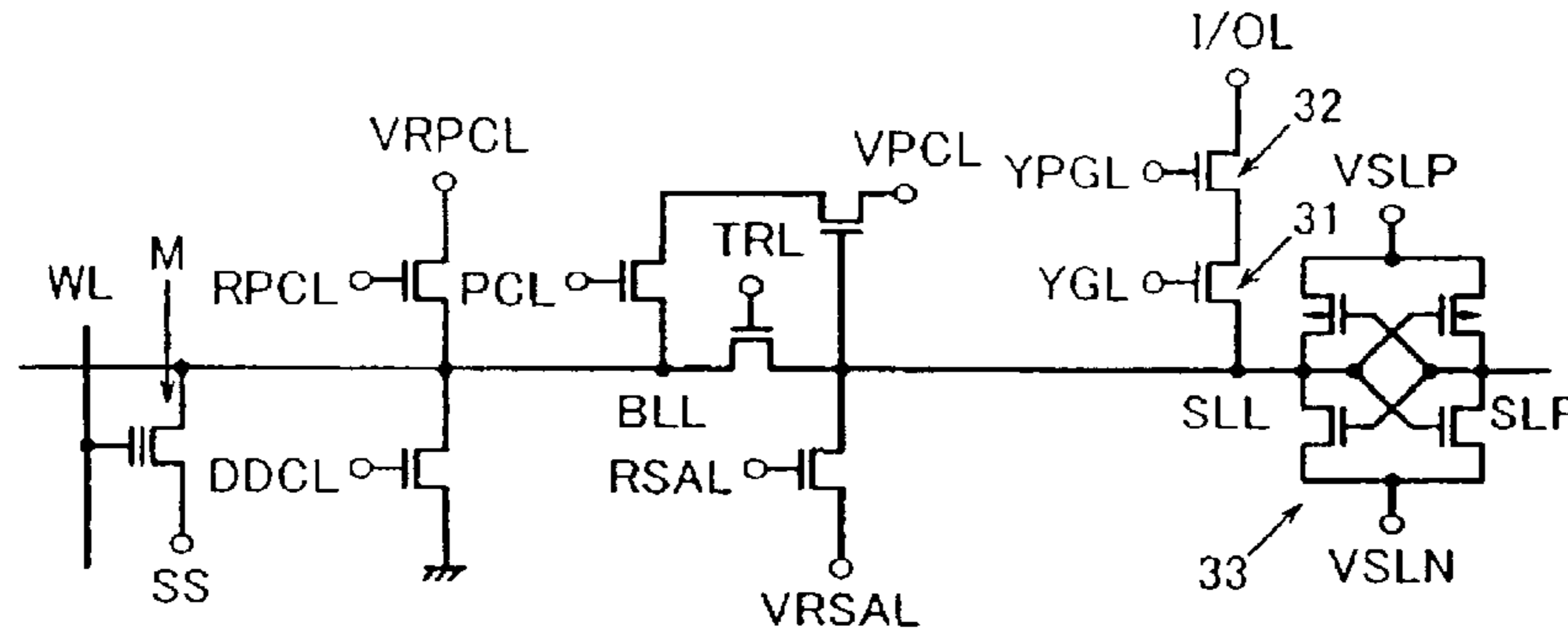
CIRCUIT DIAGRAM
