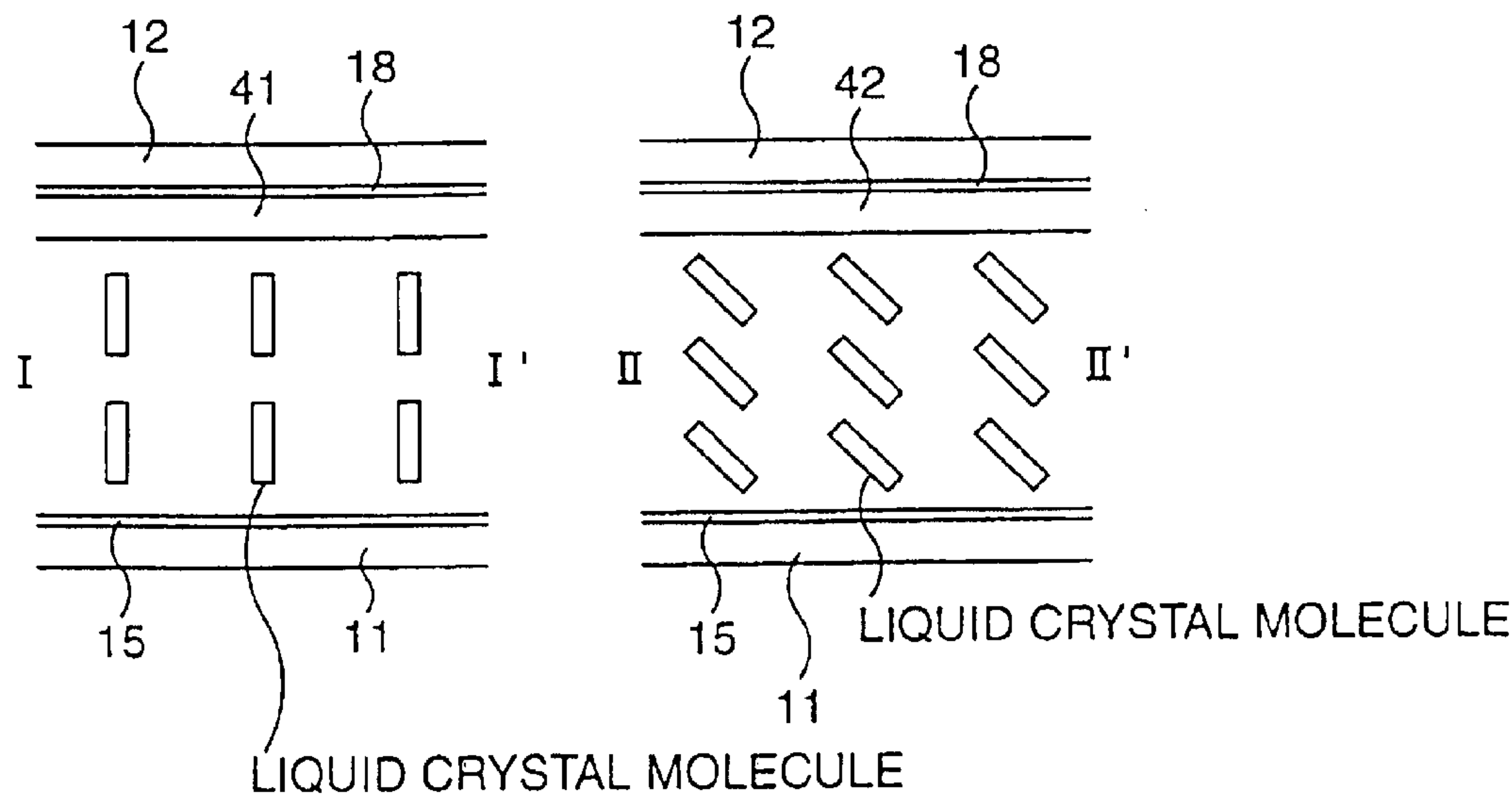
SECTIONAL VIEW
