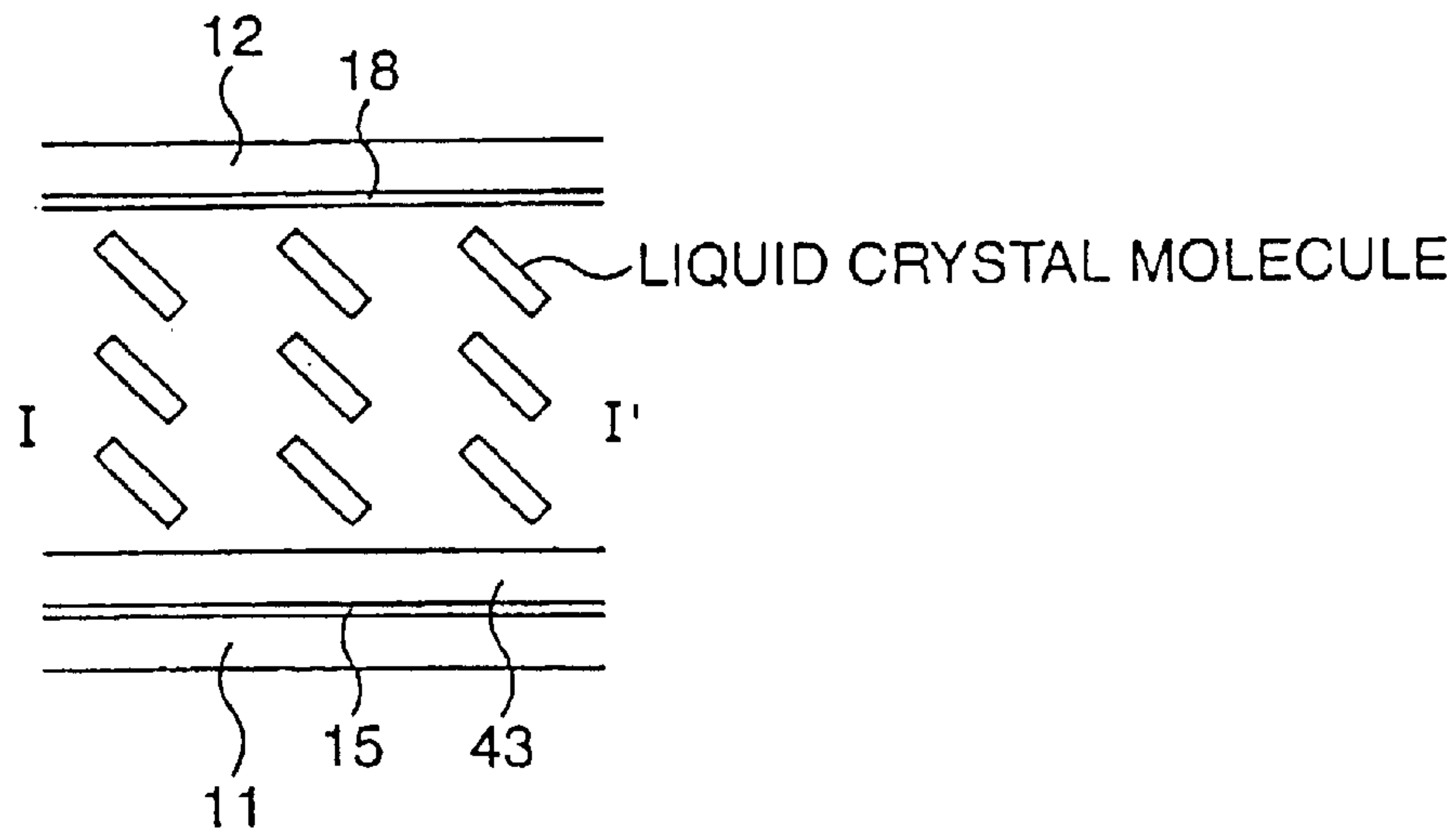
SECTIONAL VIEW
