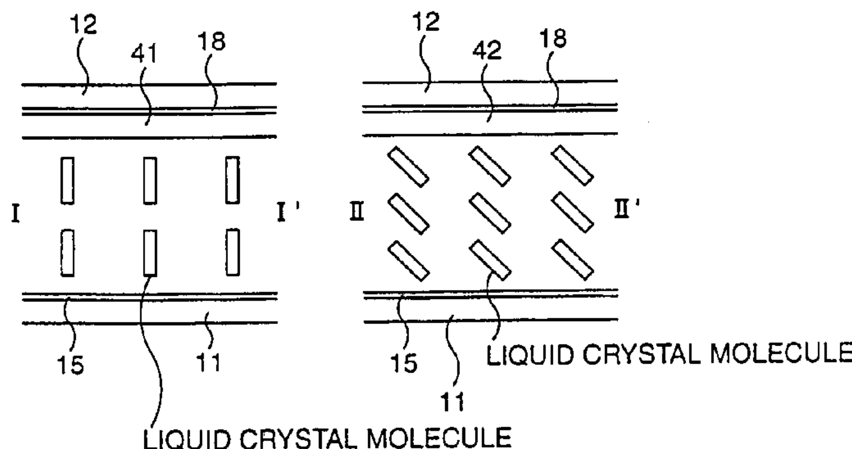
SECTIONAL VIEW
