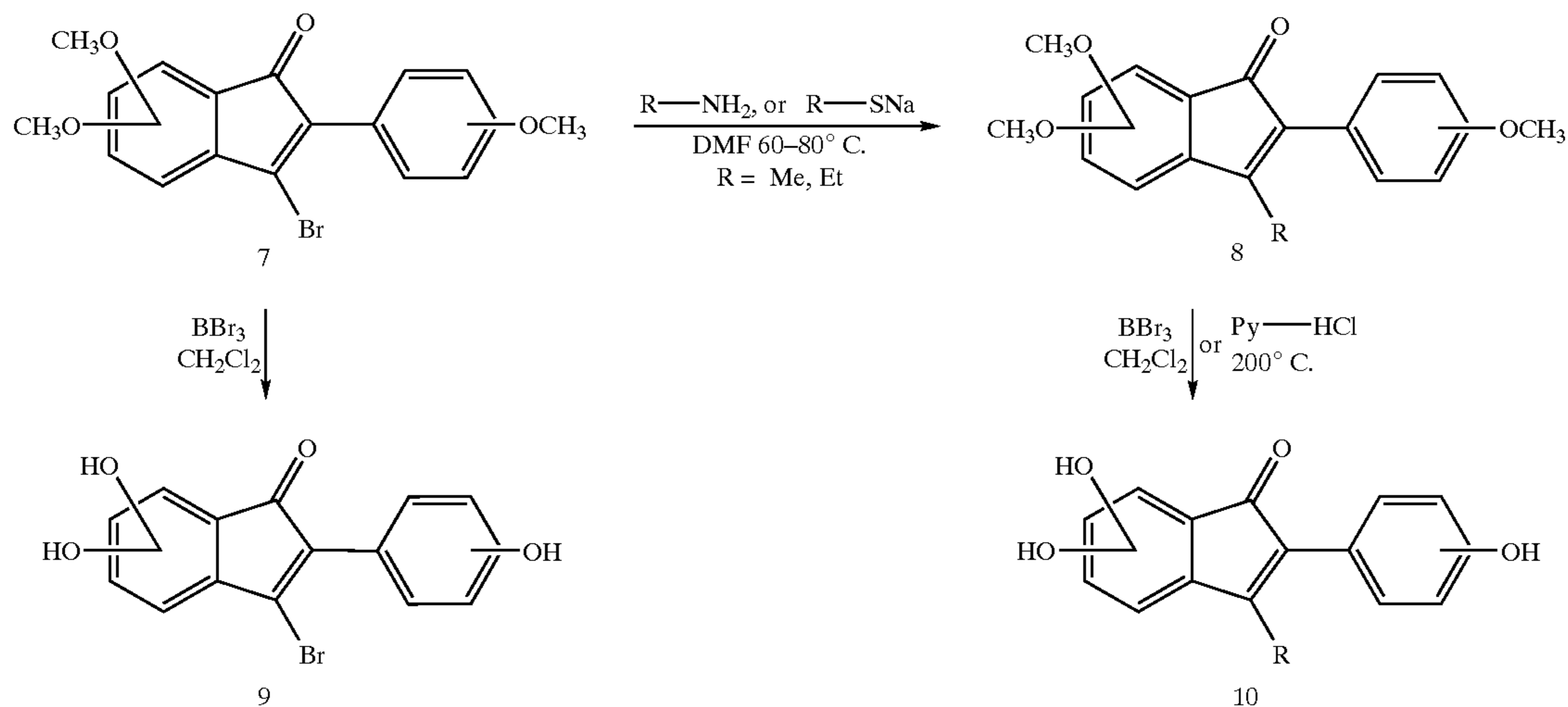
Scheme II
