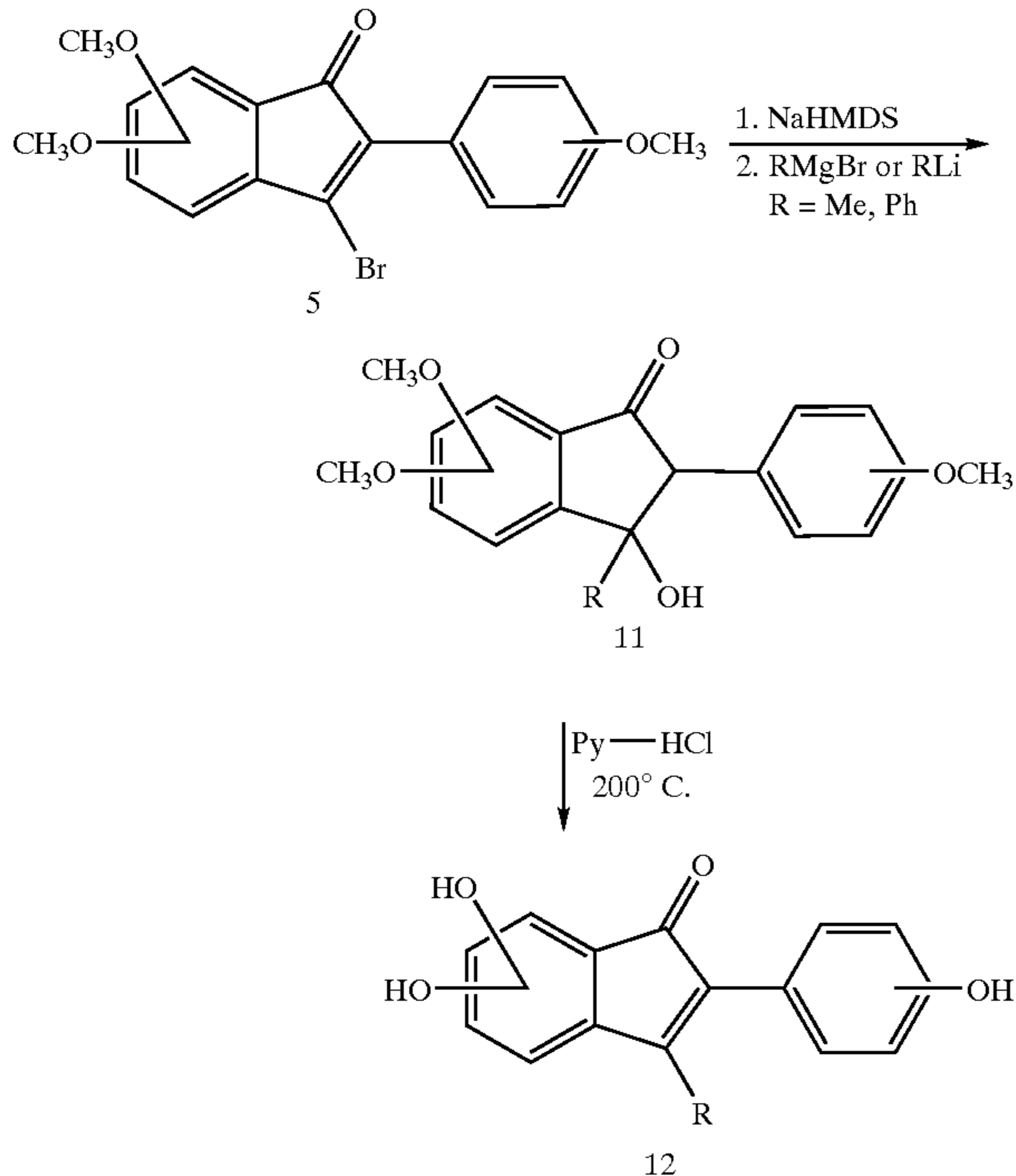
Scheme III
