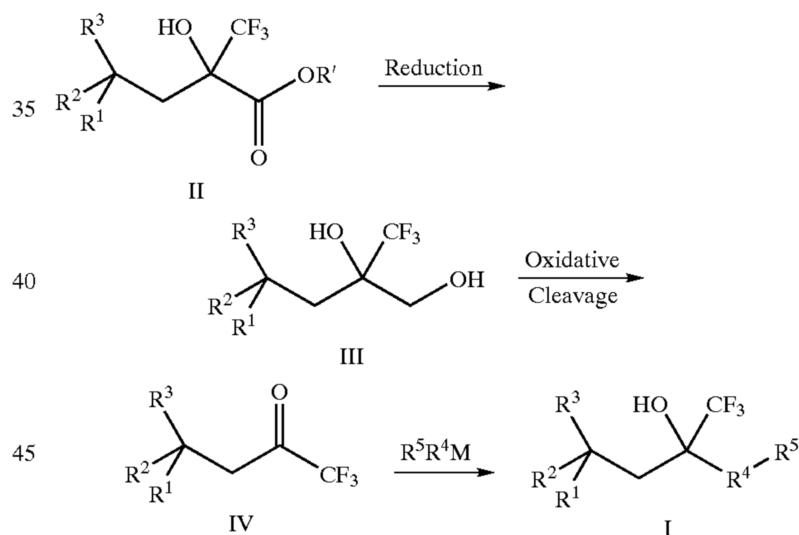
Scheme I
