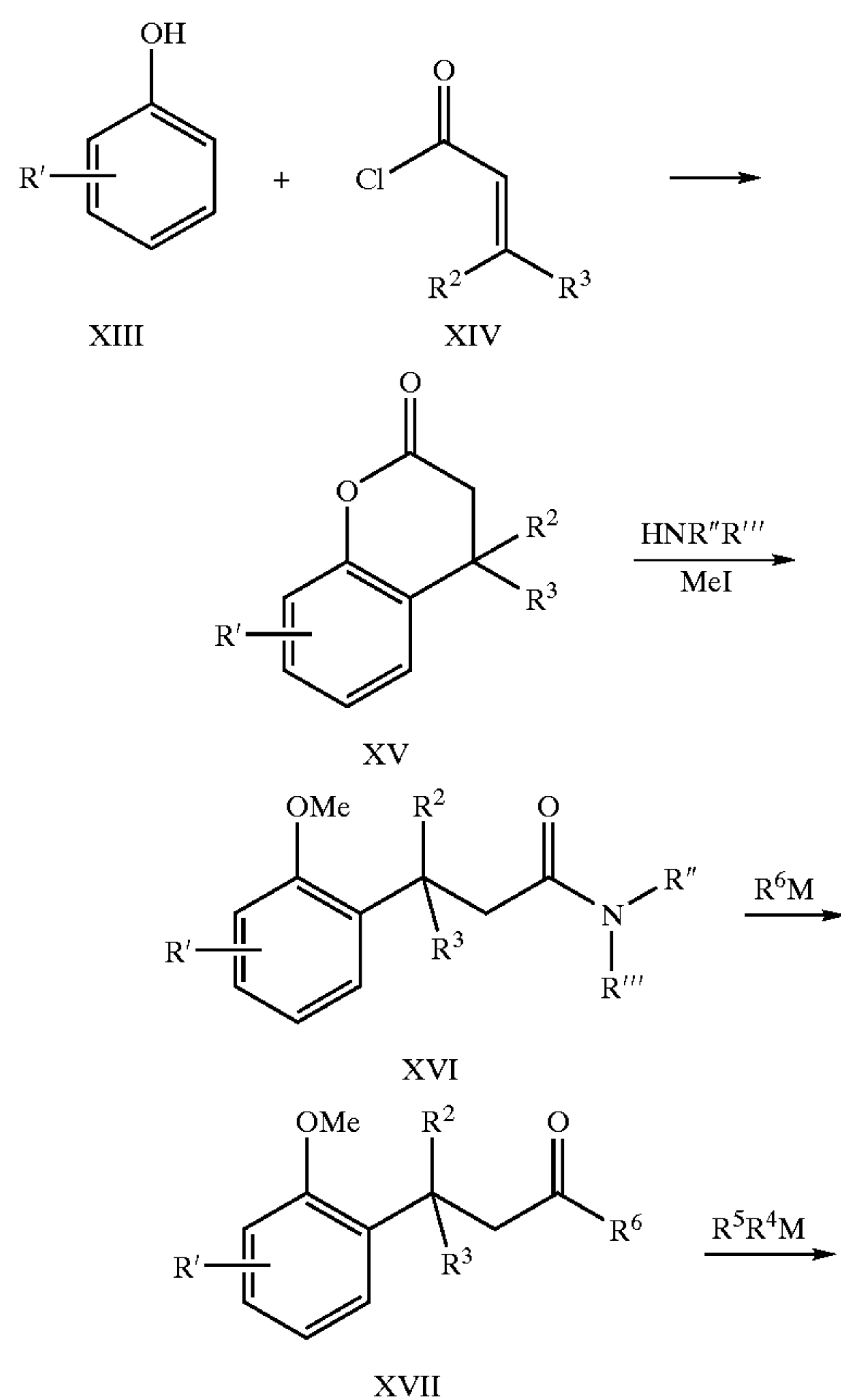
Scheme V
