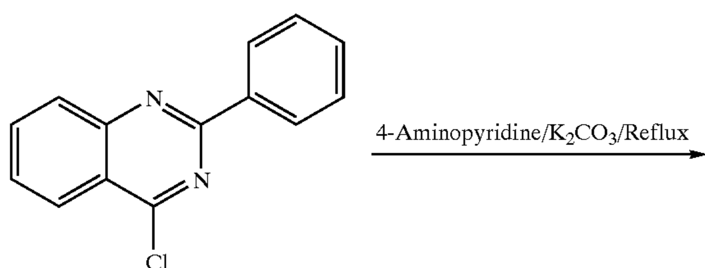
Reaction Scheme 1
