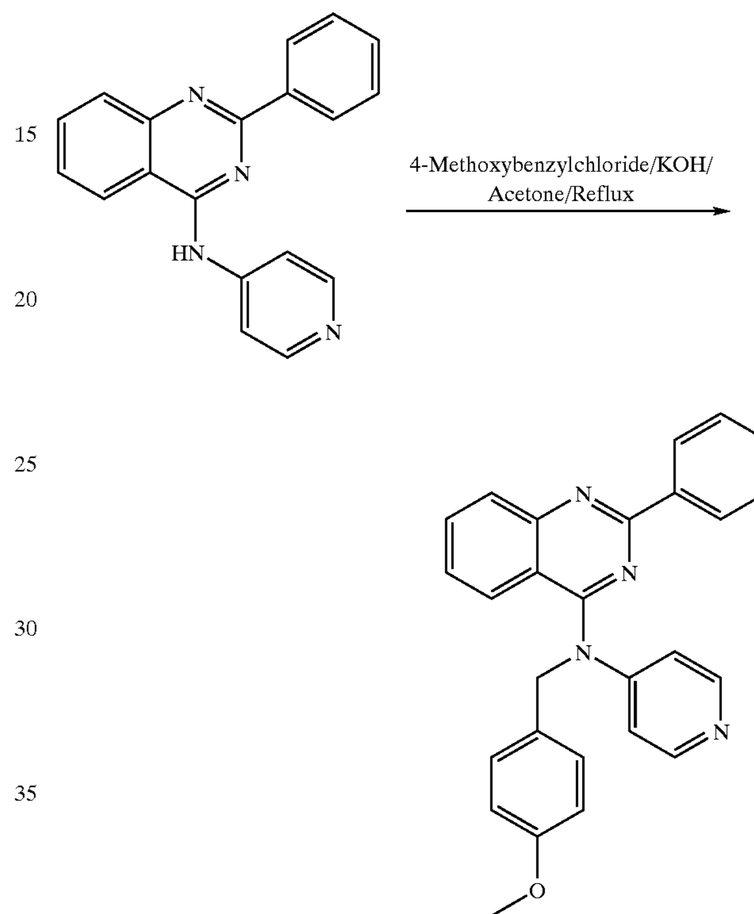
Reaction Scheme 7
