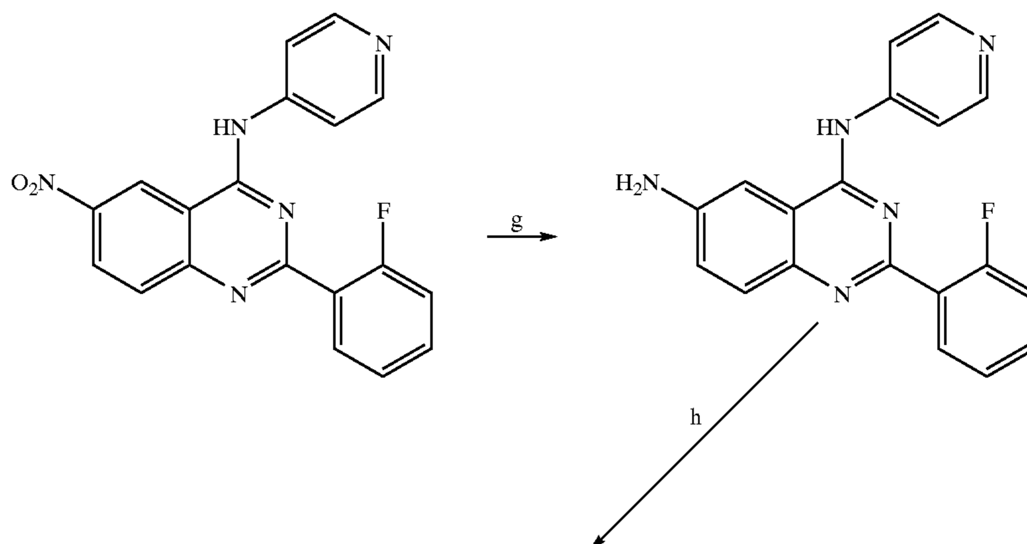
Reaction Scheme 9
