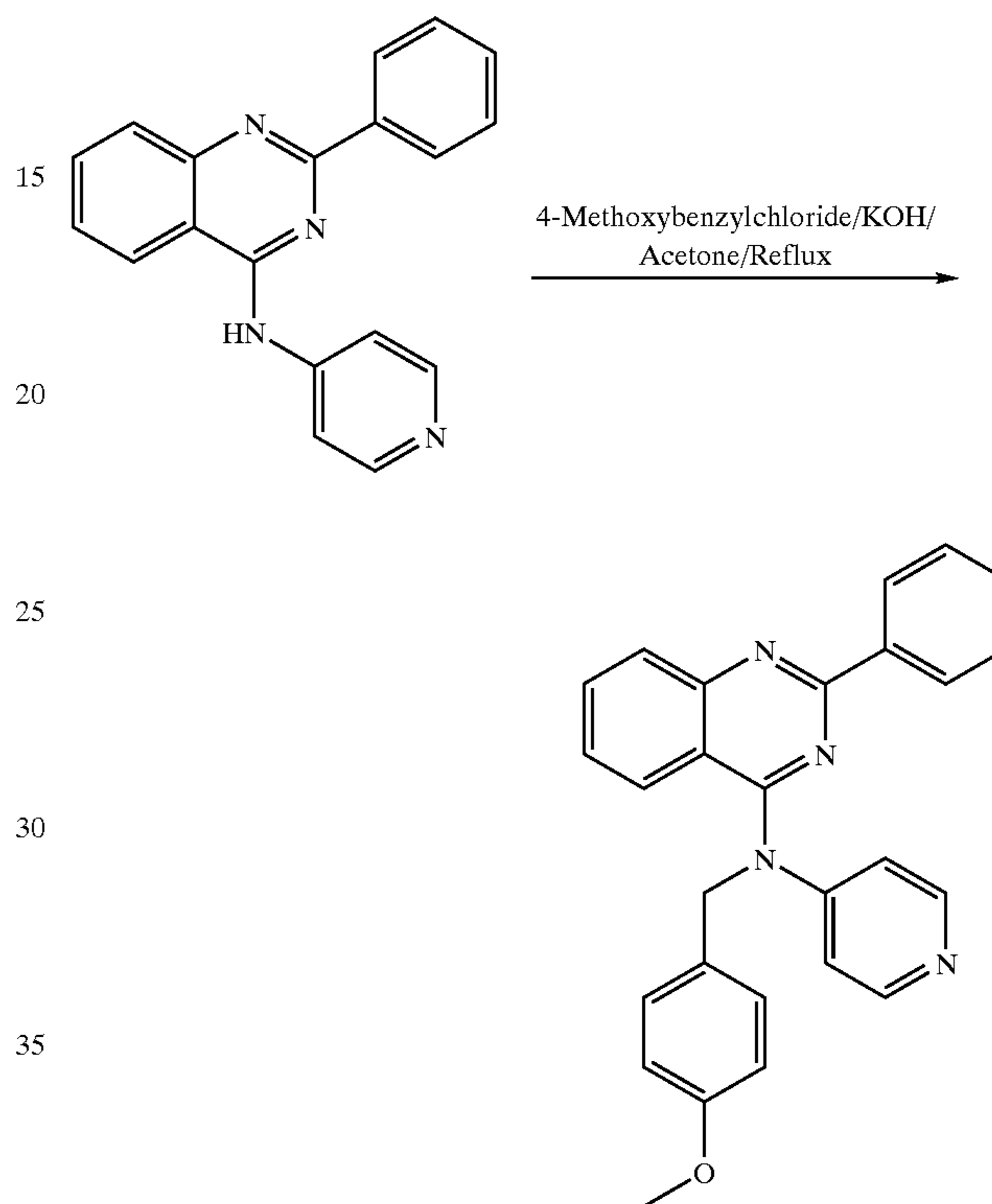
Reaction Scheme 7
