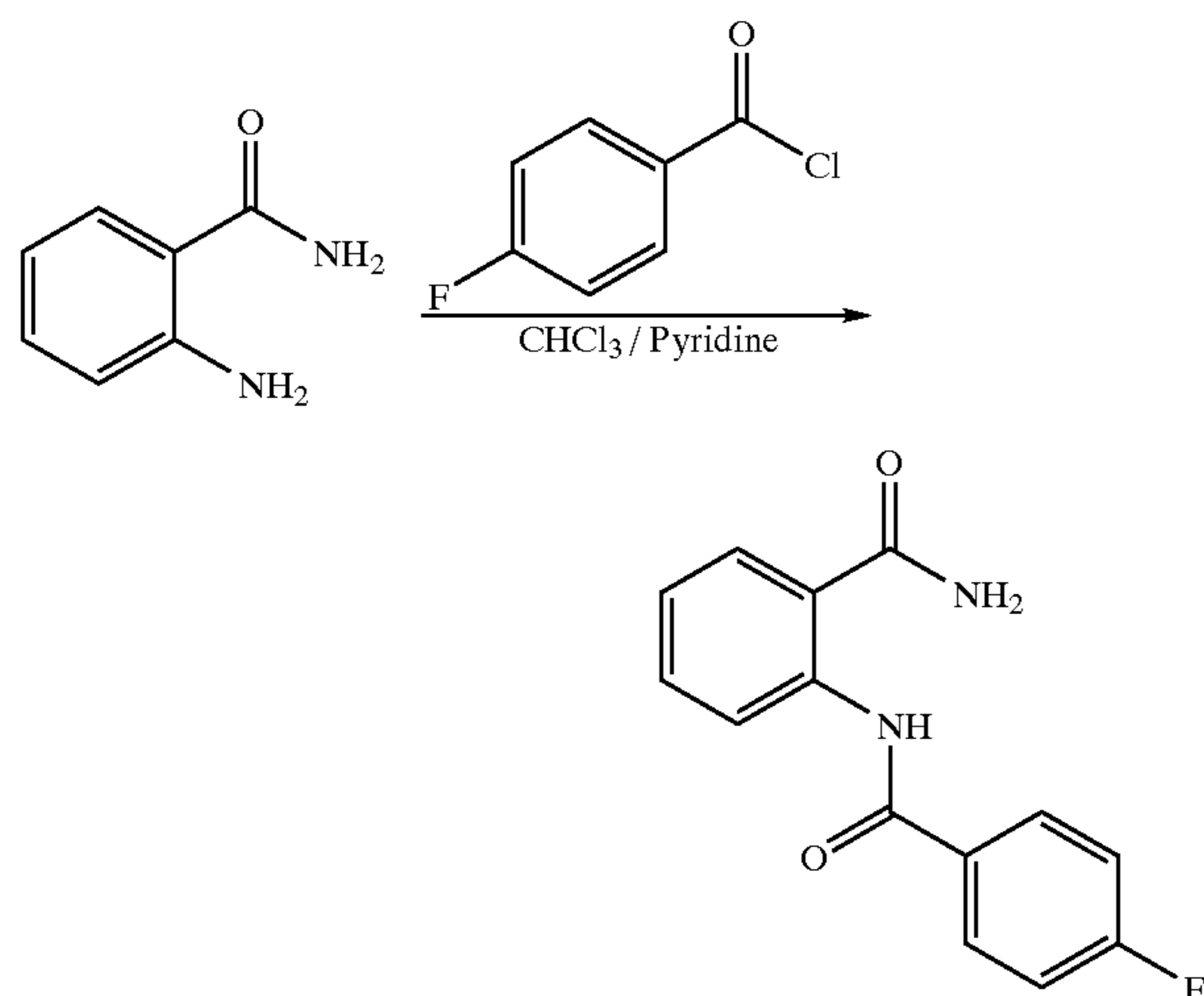
Reaction Scheme 3
