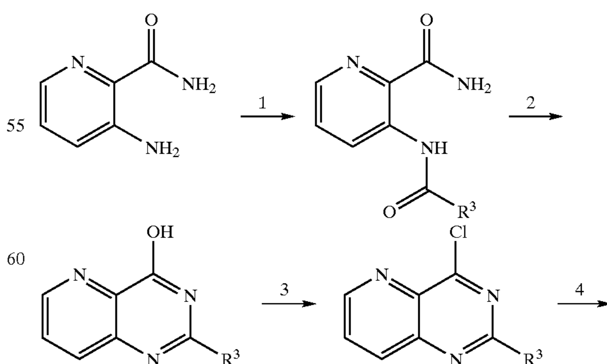
Reaction Scheme 5
