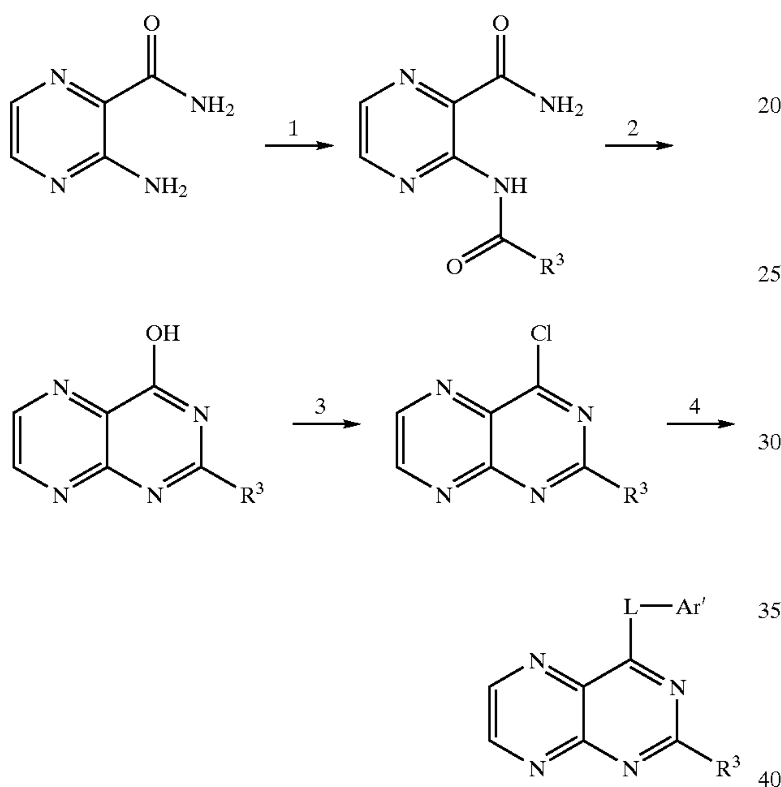
Reaction Scheme 6
