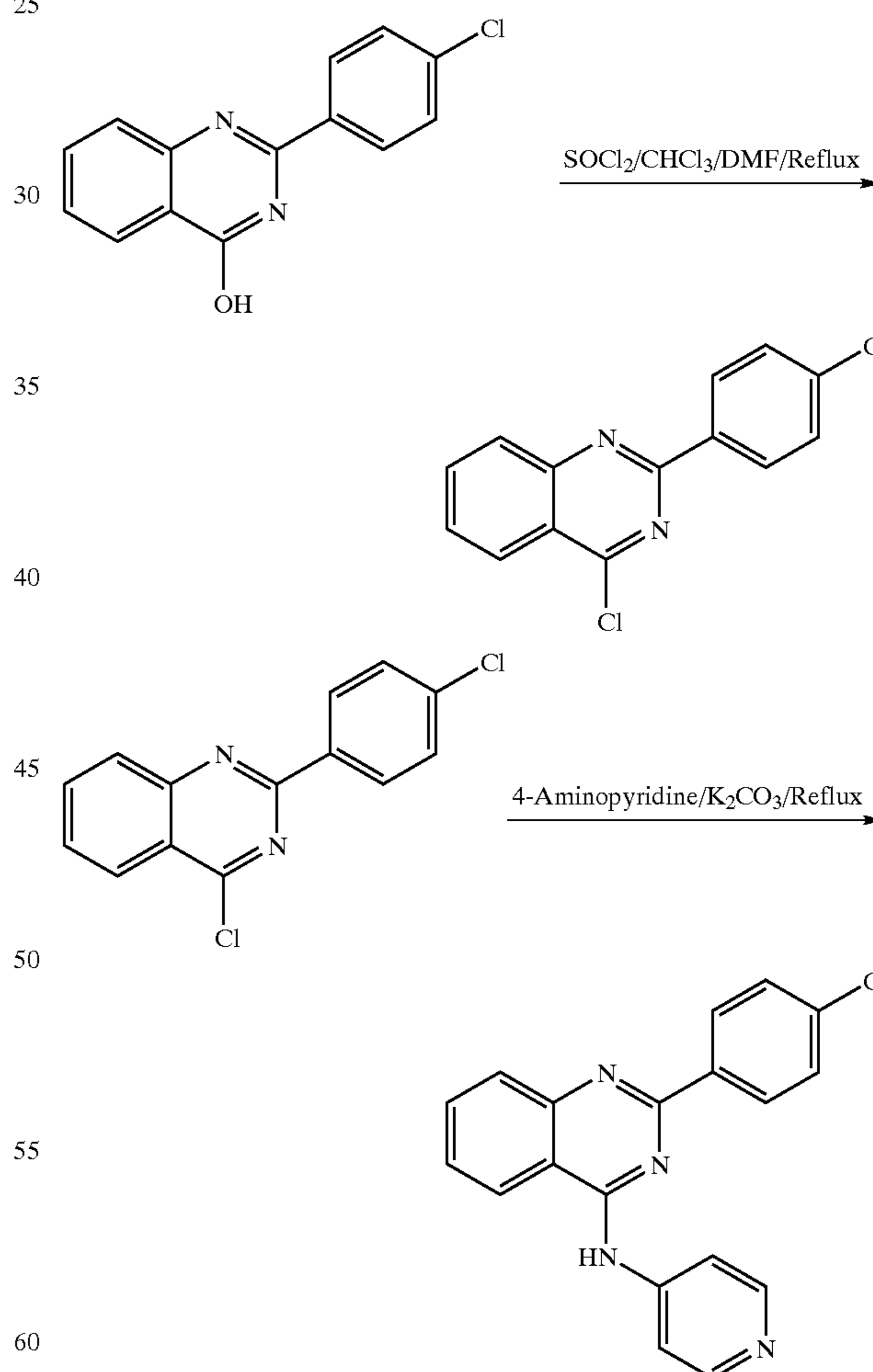
Reaction Scheme 2
