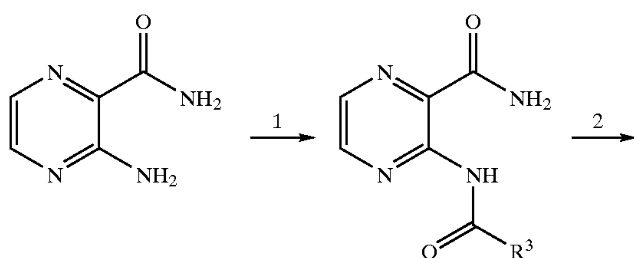
Reaction Scheme 6
