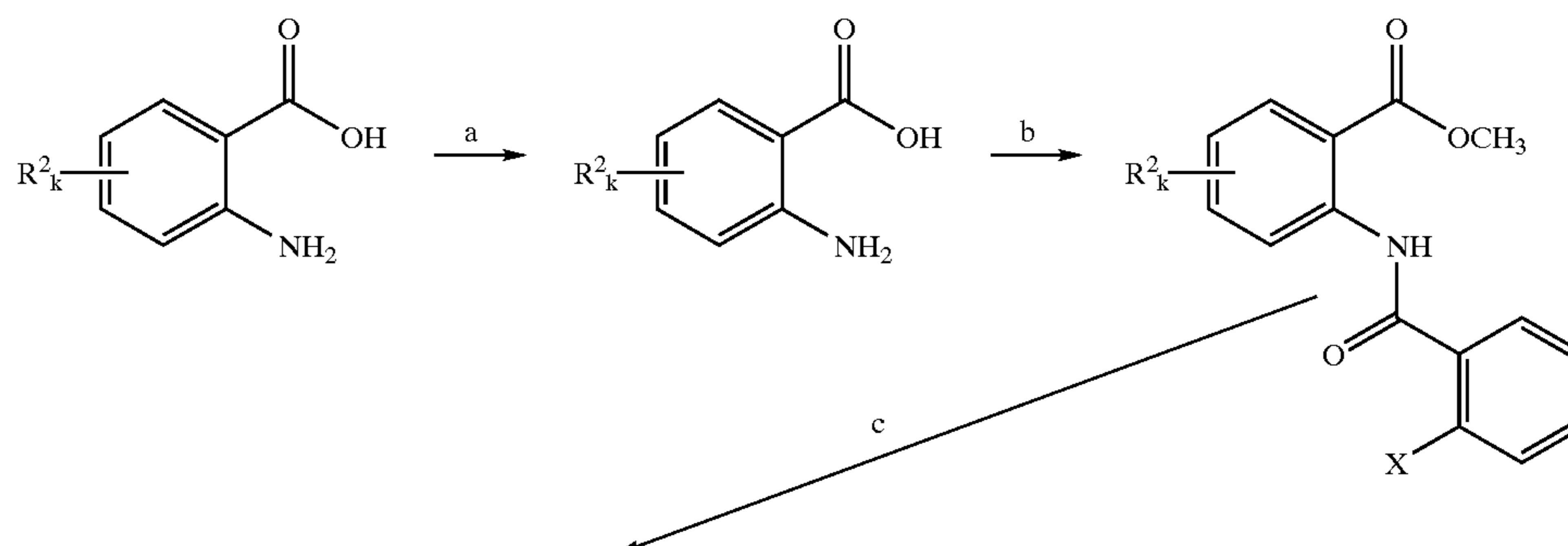
Reaction Scheme 8
