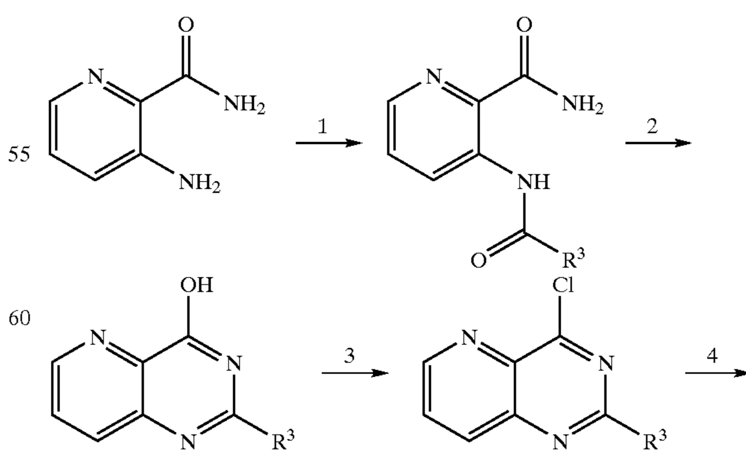
Reaction Scheme 5
