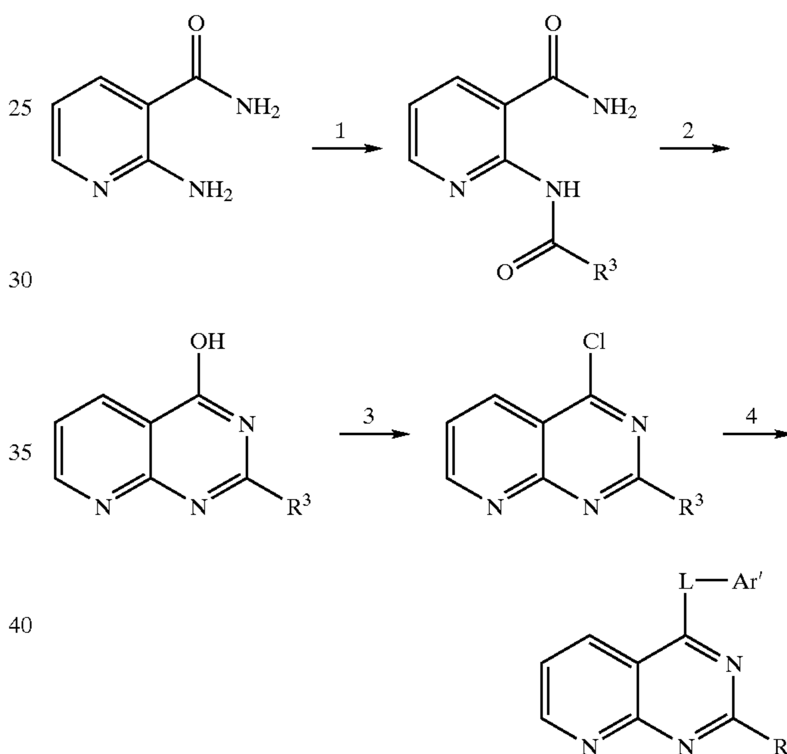
Reaction Scheme 4
