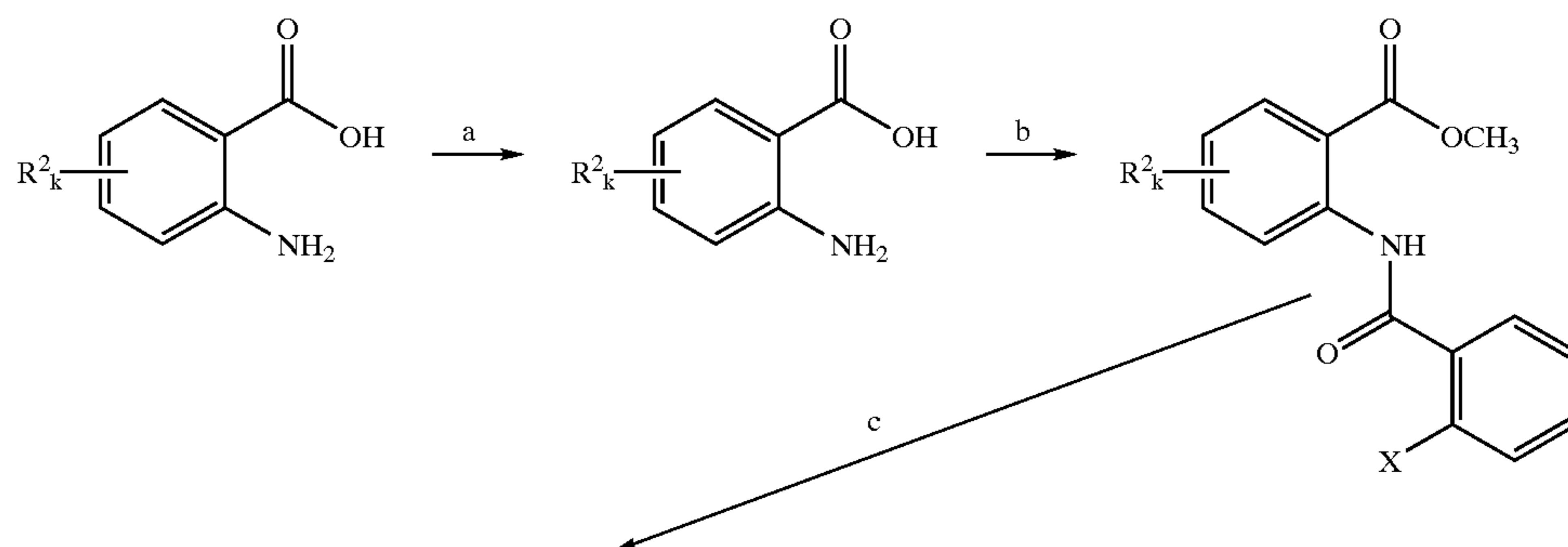
Reaction Scheme 8
