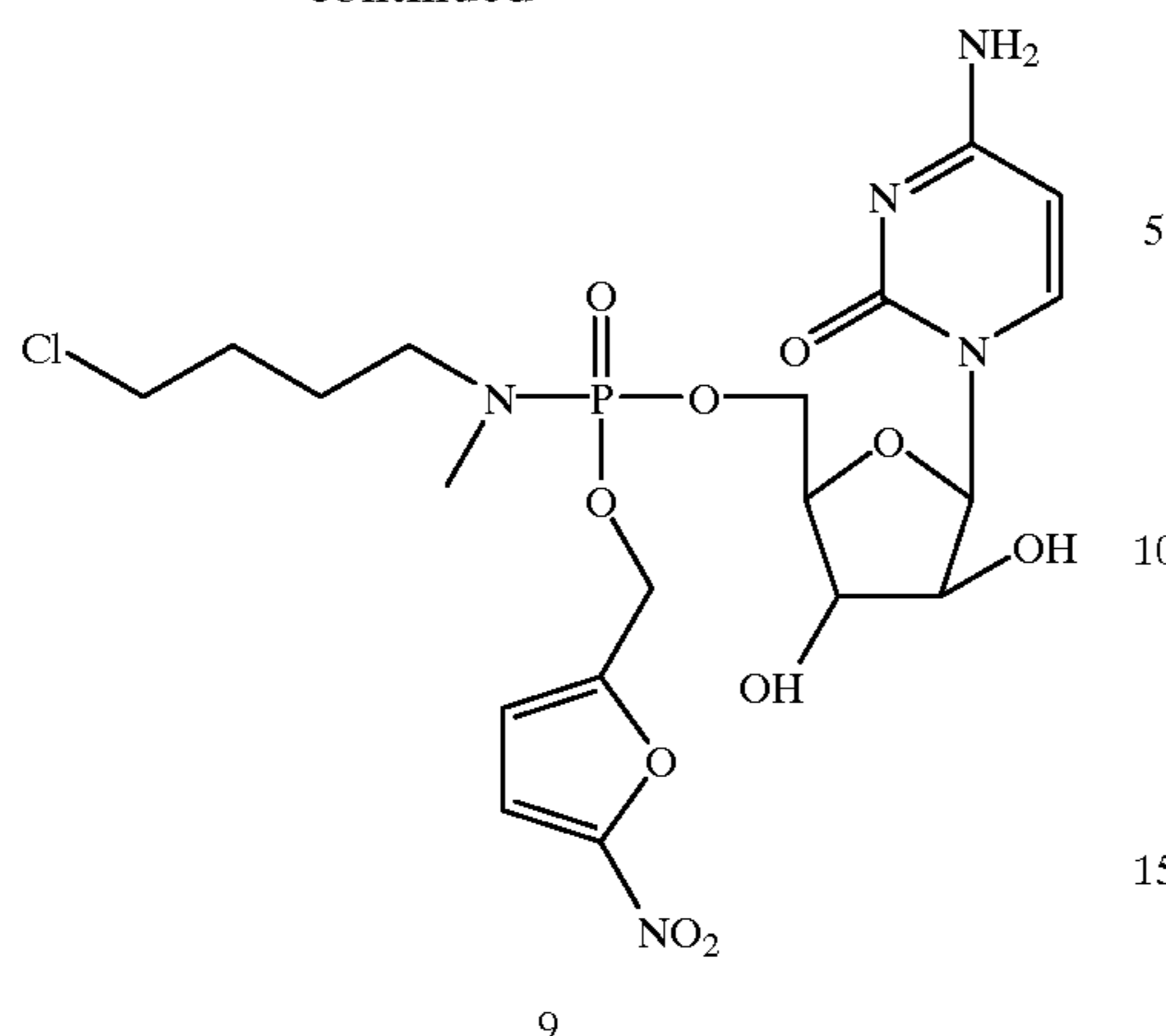
Arabinosylcytosyl 5-nitrofurfuryl N-methyl-N-(4-chlorobutyl)phosphoramidate
