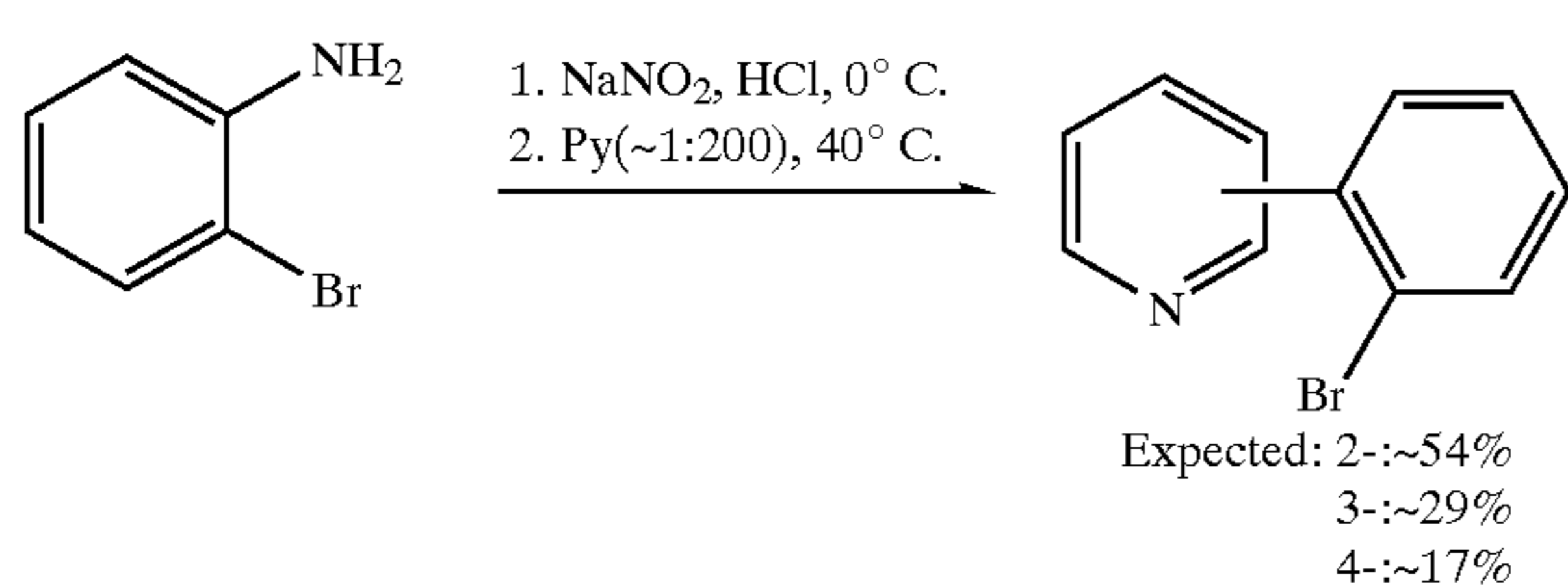
Scheme 4 Synthesis of n-(2'-bromophenyl)pyridines
