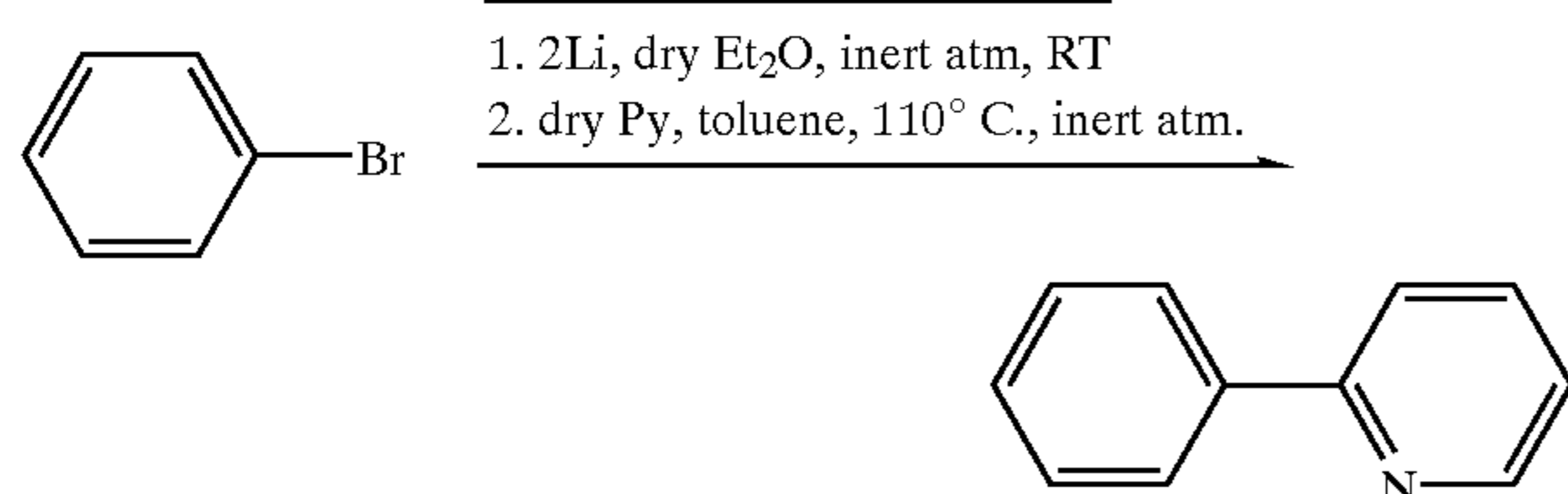
Scheme 5 Synthesis of 2-phenylpyridines
