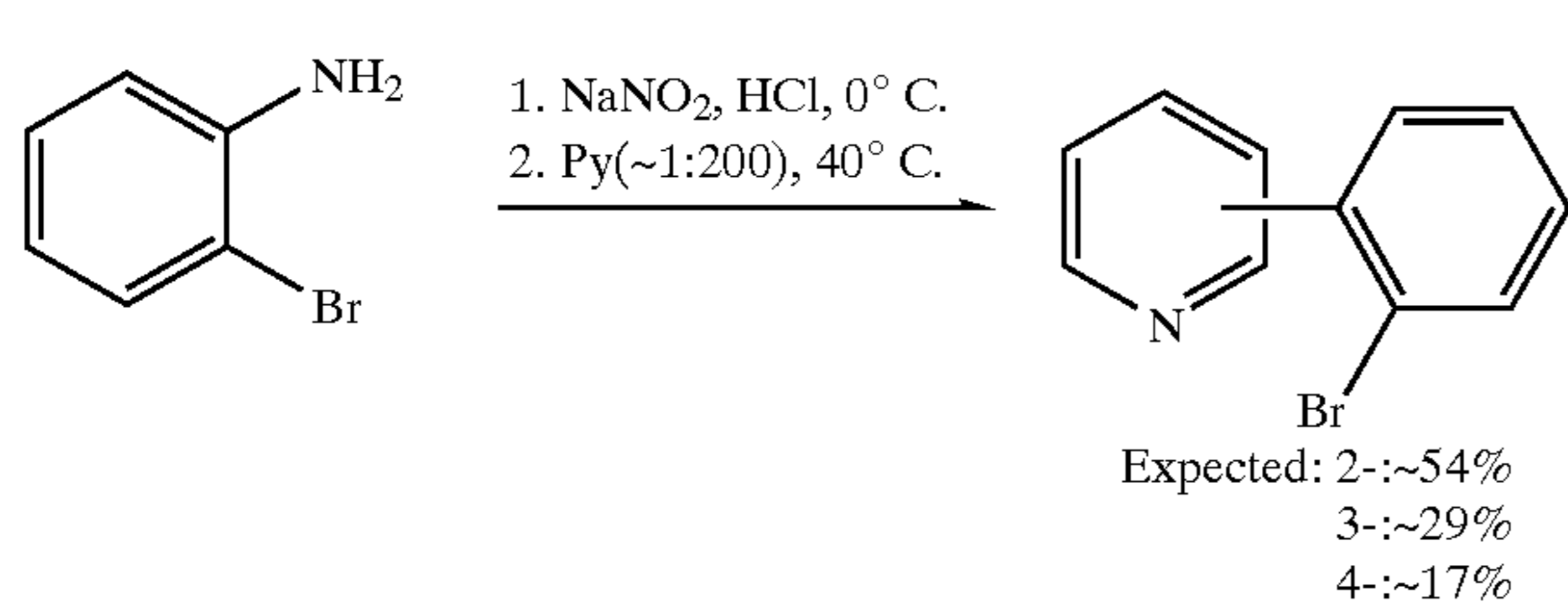
Scheme 4 Synthesis of n-(2'-bromophenyl)pyridines
