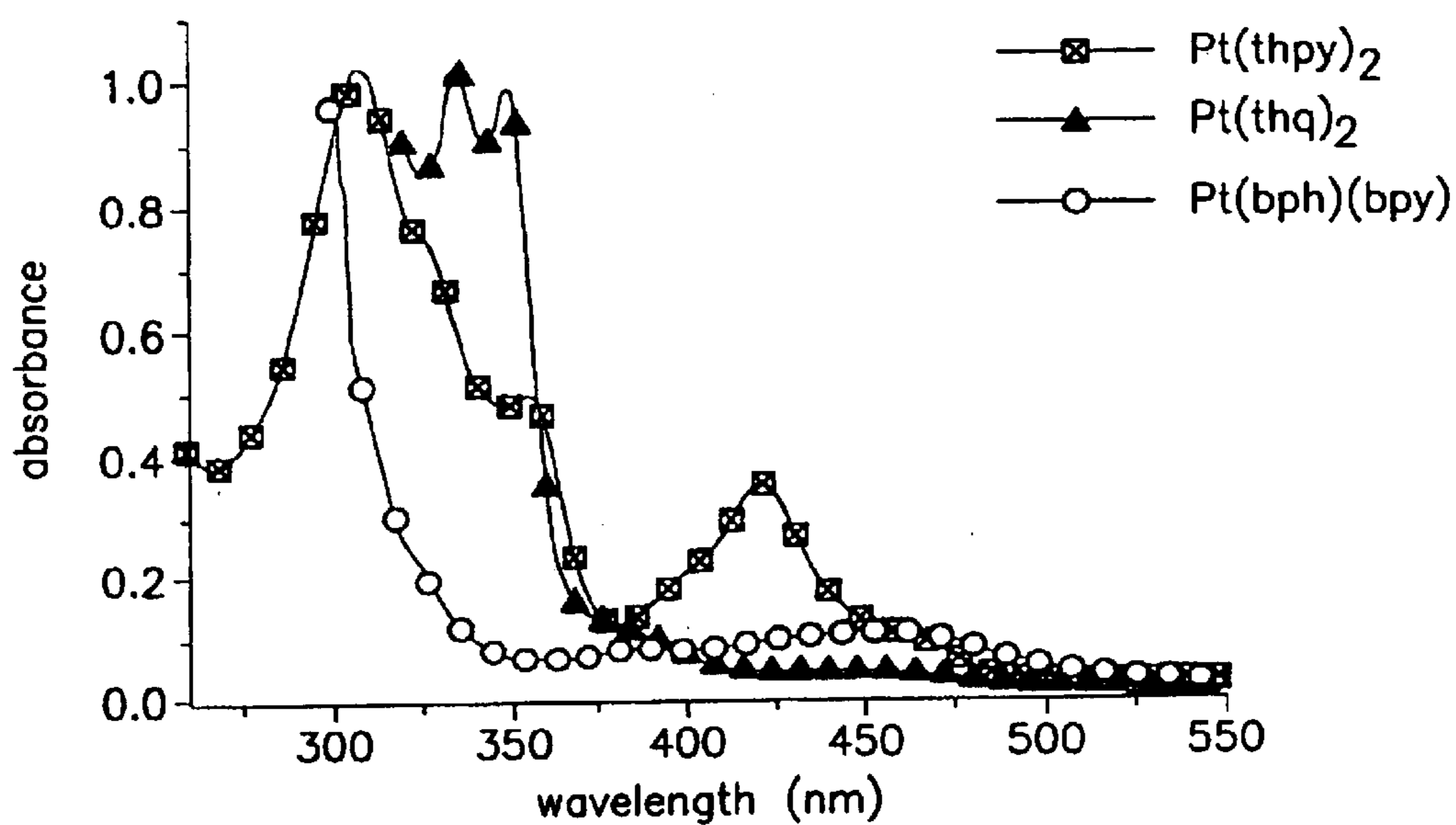
Electronic absorbance spectra of Pt(thpy) 2 , Pt(thq) 2 , Pt(bph)(bpy).
