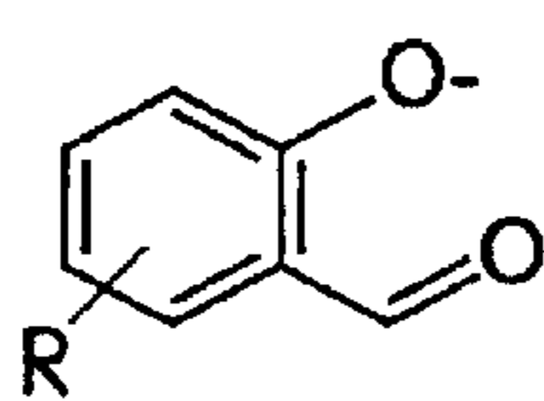
salicylaldehydes
