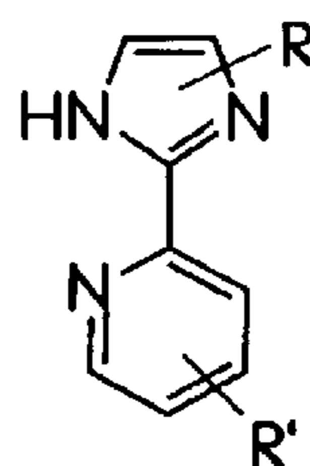
pyridylimidazoles
