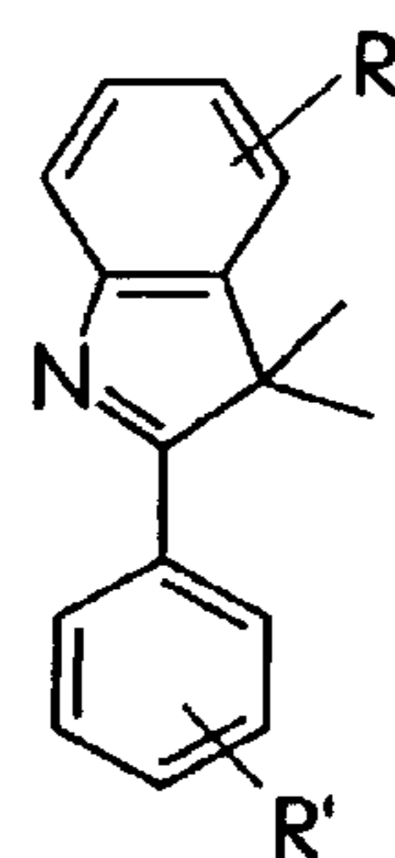
phenylindoles
