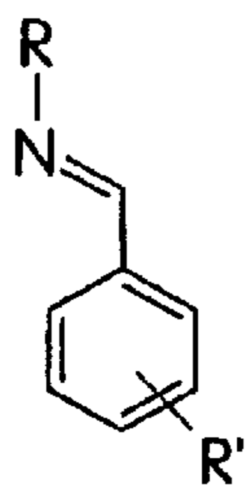
phenylimines
