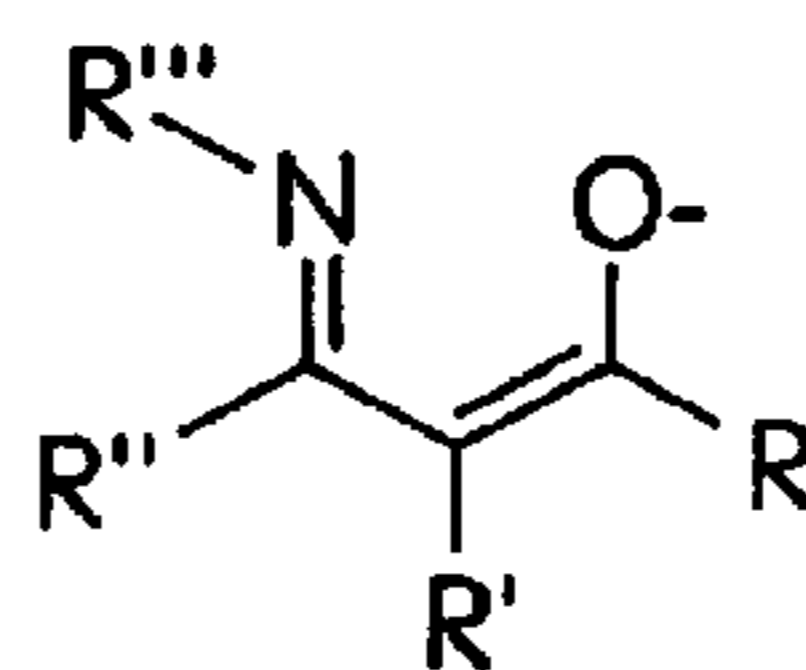
iminoacetates
