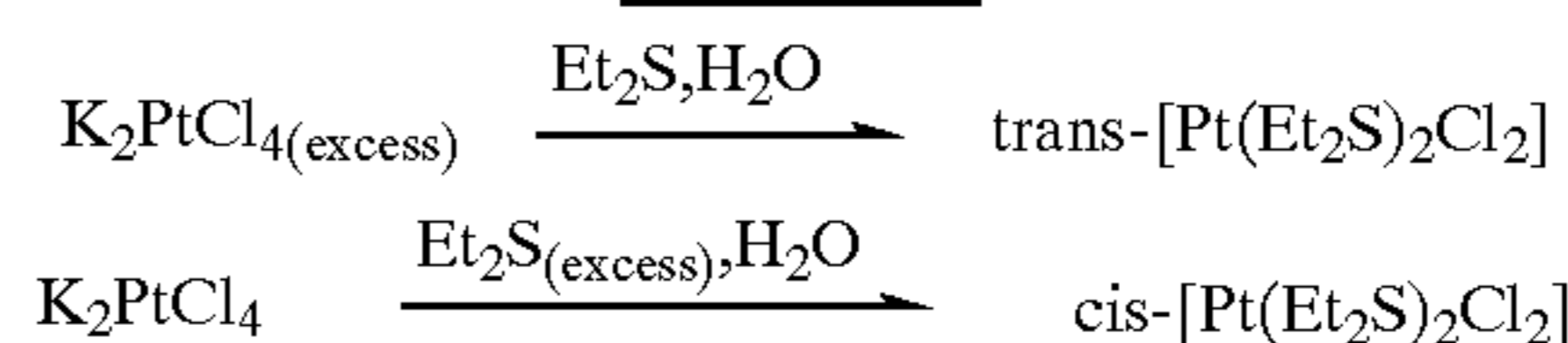
Scheme 8 Syntheses of cis- and trans-Dichloro-bis-(diethyl sulfide) platinum (II)
