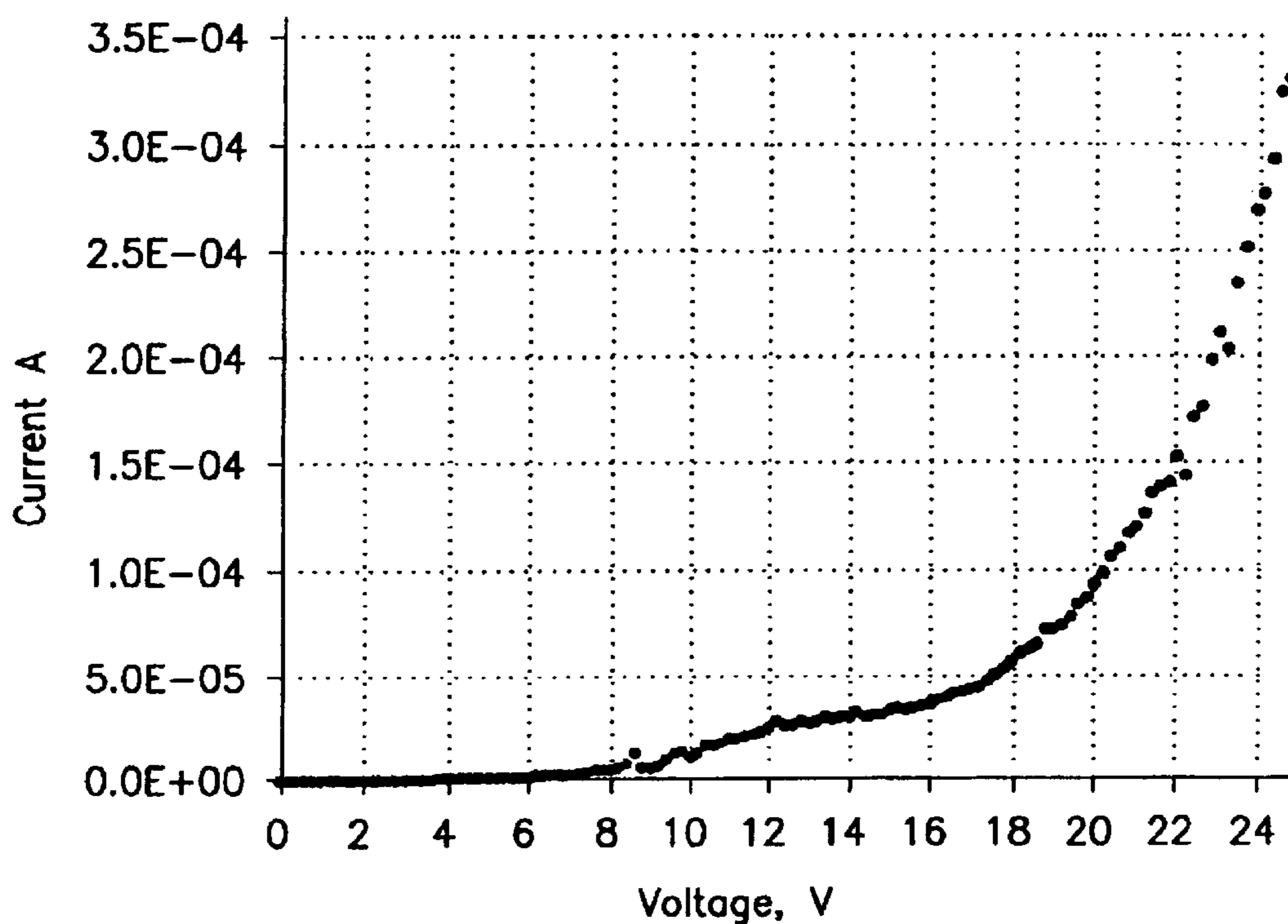
I-V characteristic of the device.
