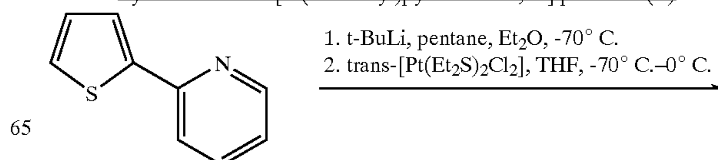
Scheme 9 Synthesis of cis-bis[2-(2'-thienyl)pyridinato- \text{N}, \text{C}^3 ] platinum (II)
