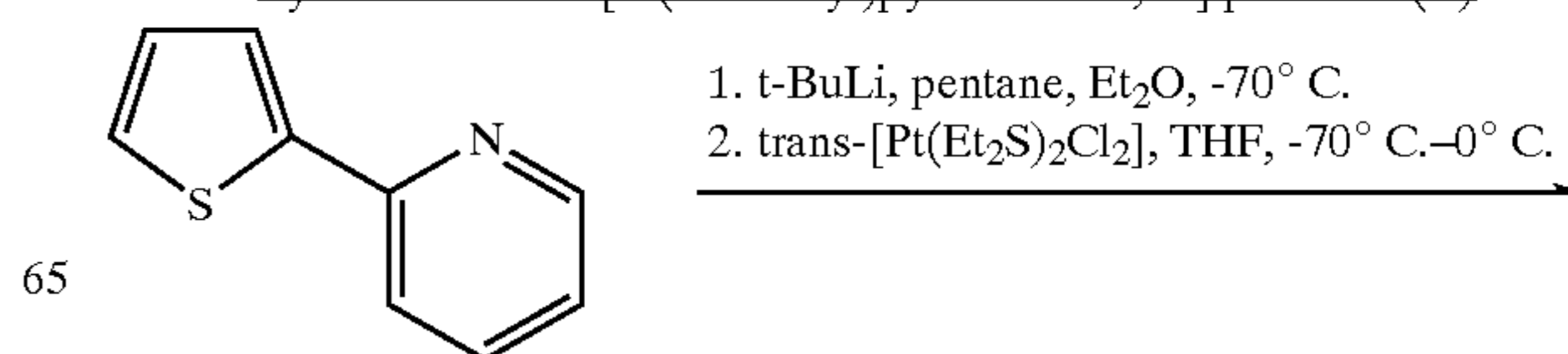
Scheme 9 Synthesis of cis-bis[2-(2'-thienyl)pyridinato- \text{N}, \text{C}^3 ] platinum (II)
