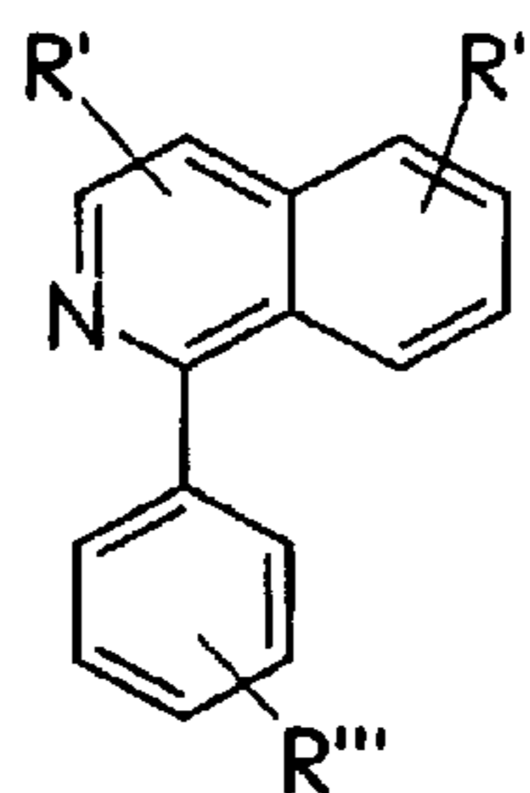
arylquinolines
