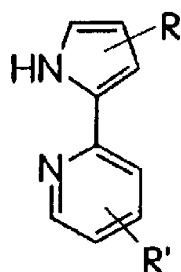
pyridylpyroles
