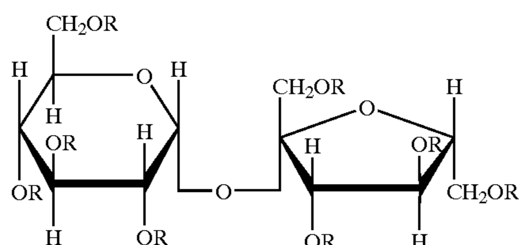
\alpha -D-glucopyranoside, \beta -D-fructofuranosyl-oktakakis (Hydrogen Sulfate) Bismuth Complex
