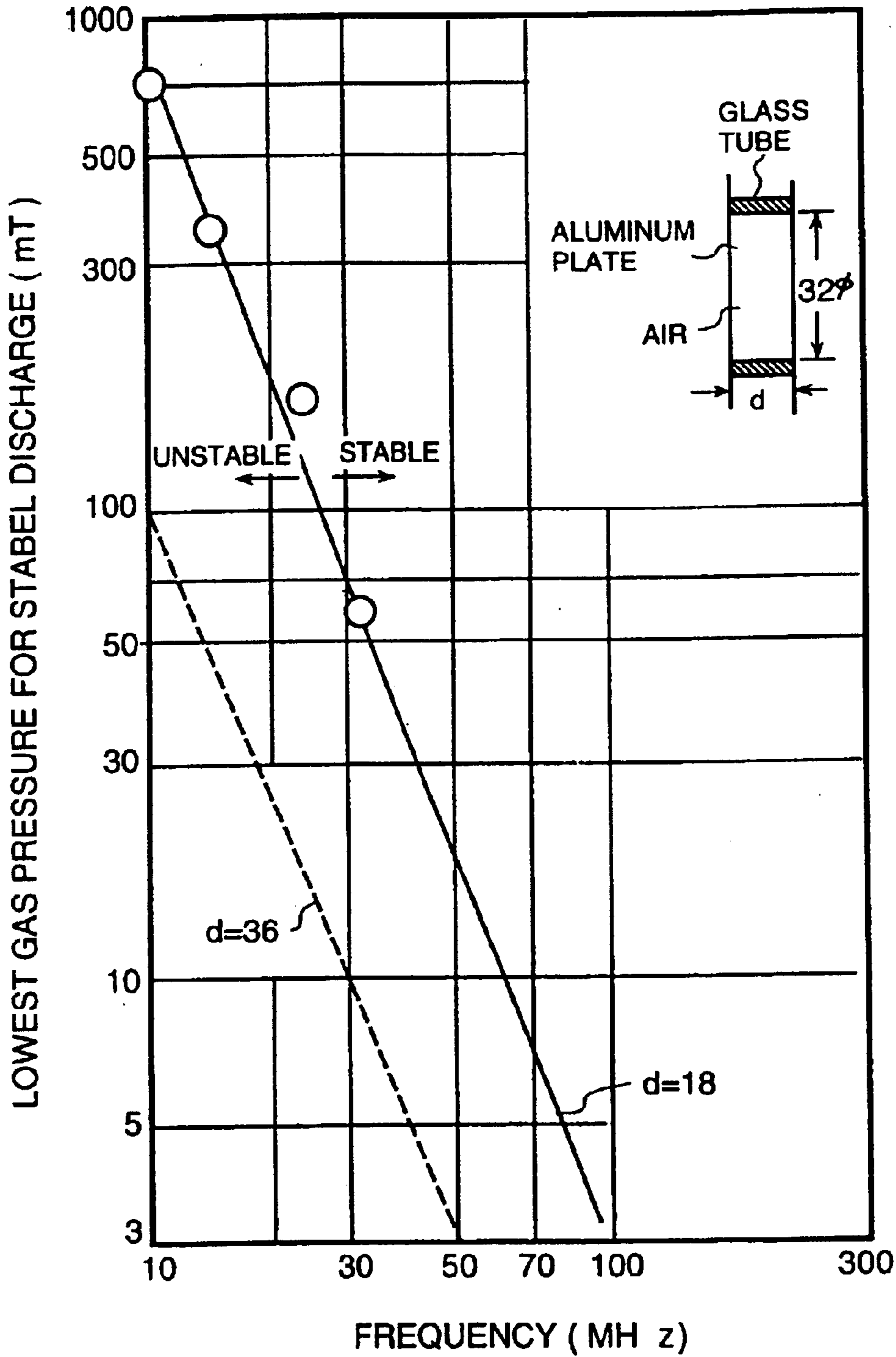
FREQUENCY-LOWEST GAS PRESSURE FOR STABLE DISCHARGE CHARACTERISTIC
