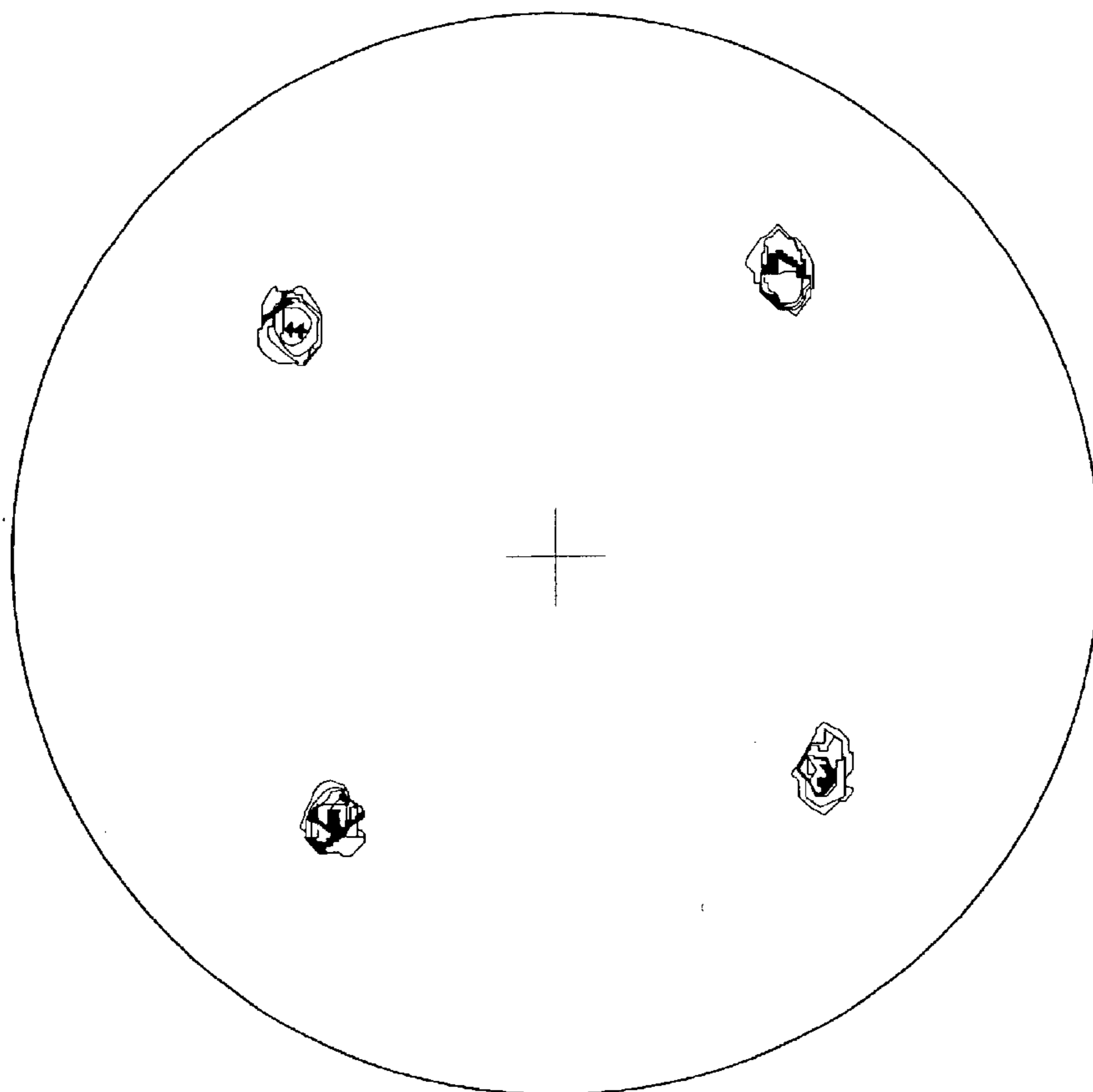
Ni-13at%Cr alloy Annealing Temperature = 1400°C
