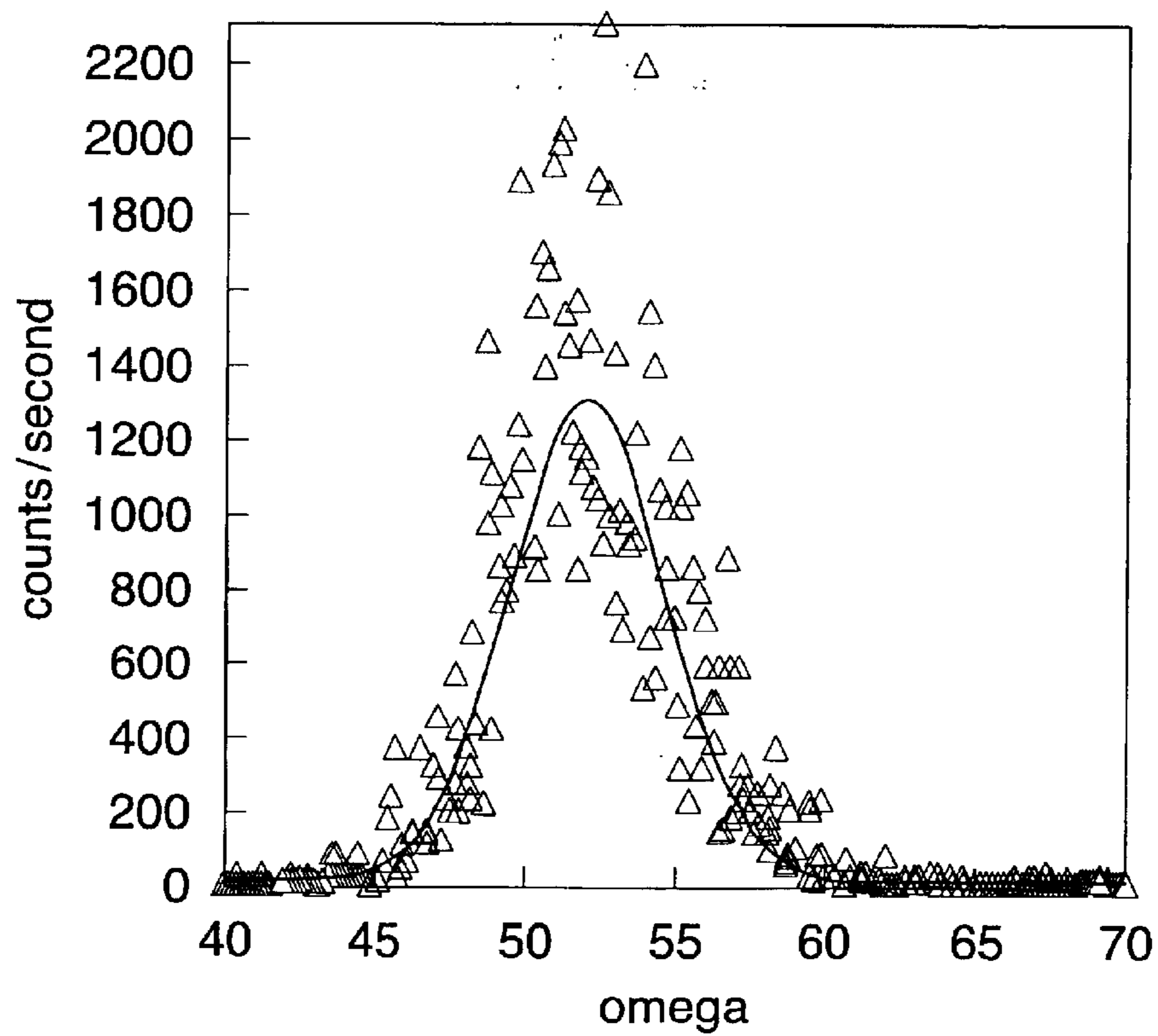
Ni-0.03at%Mg alloy Annealing Temperature = 1200°C
