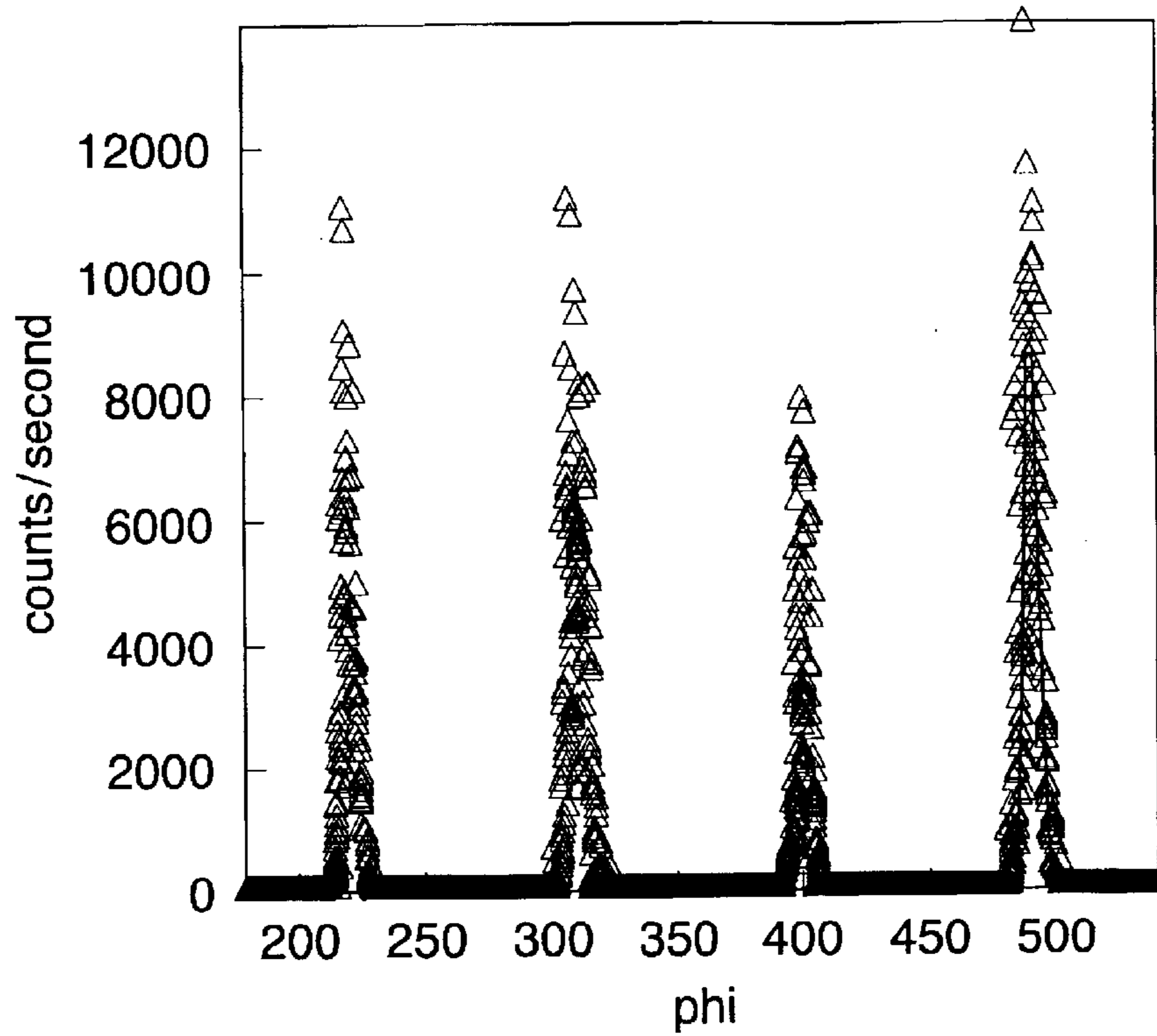
Ni-13at%Cr-0.03at%Mg alloy Annealing Temperature = 1400°C
