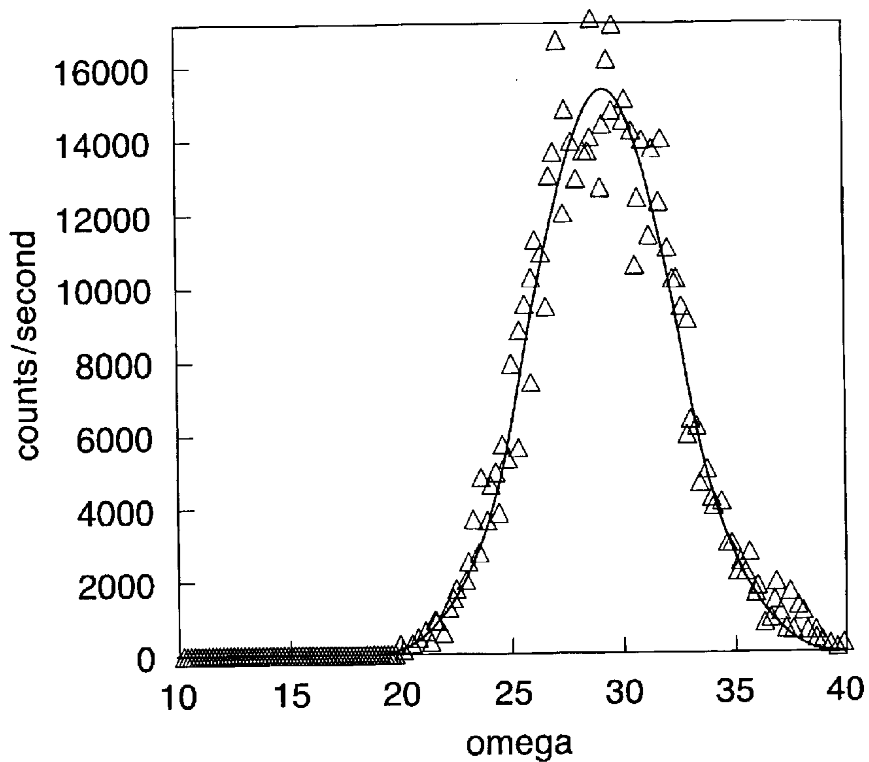
Ni-9at%W alloy Annealing Temperature = 1400°C
