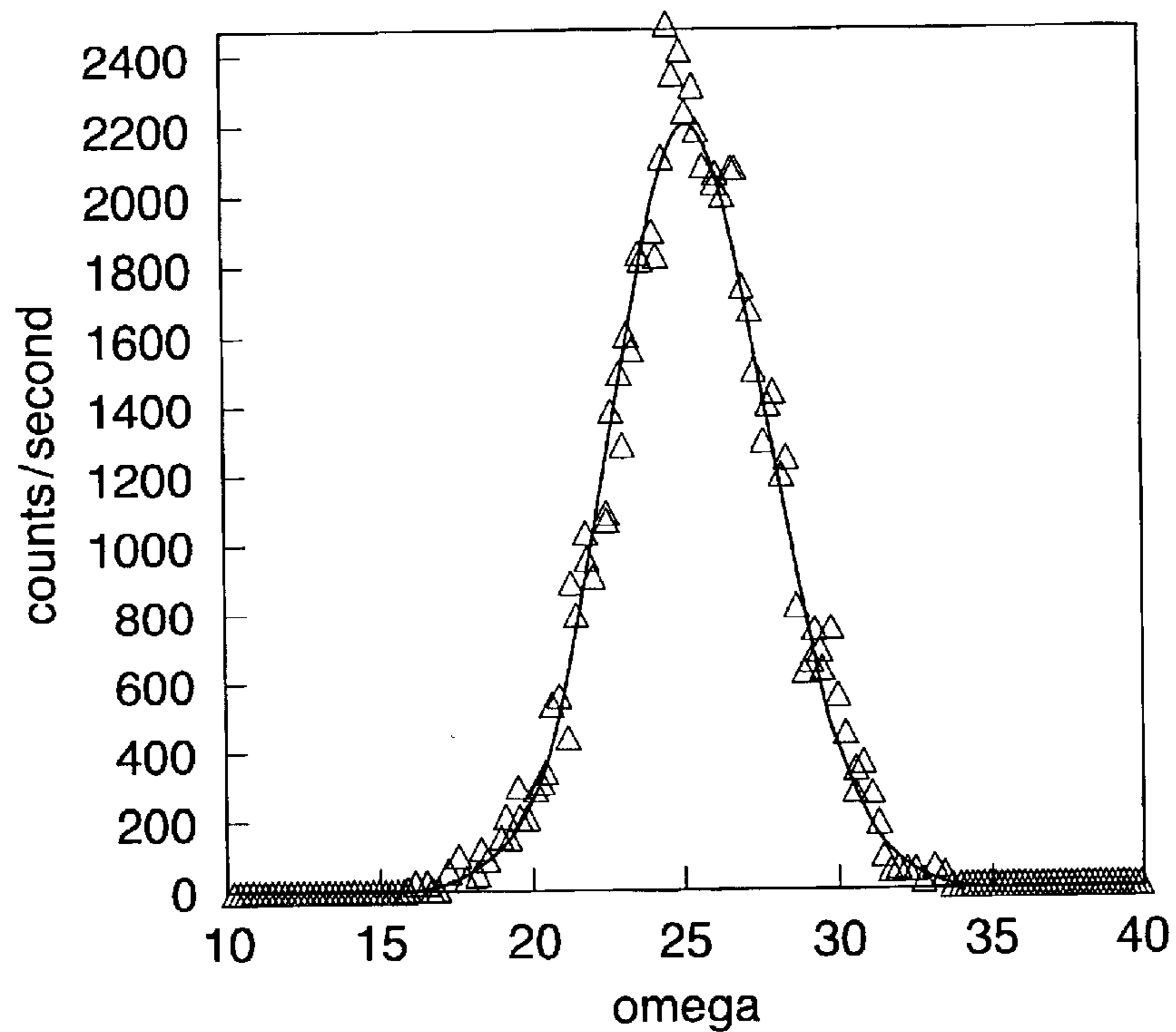
Ni-9at%W alloy Annealing Temperature = 1200°C
