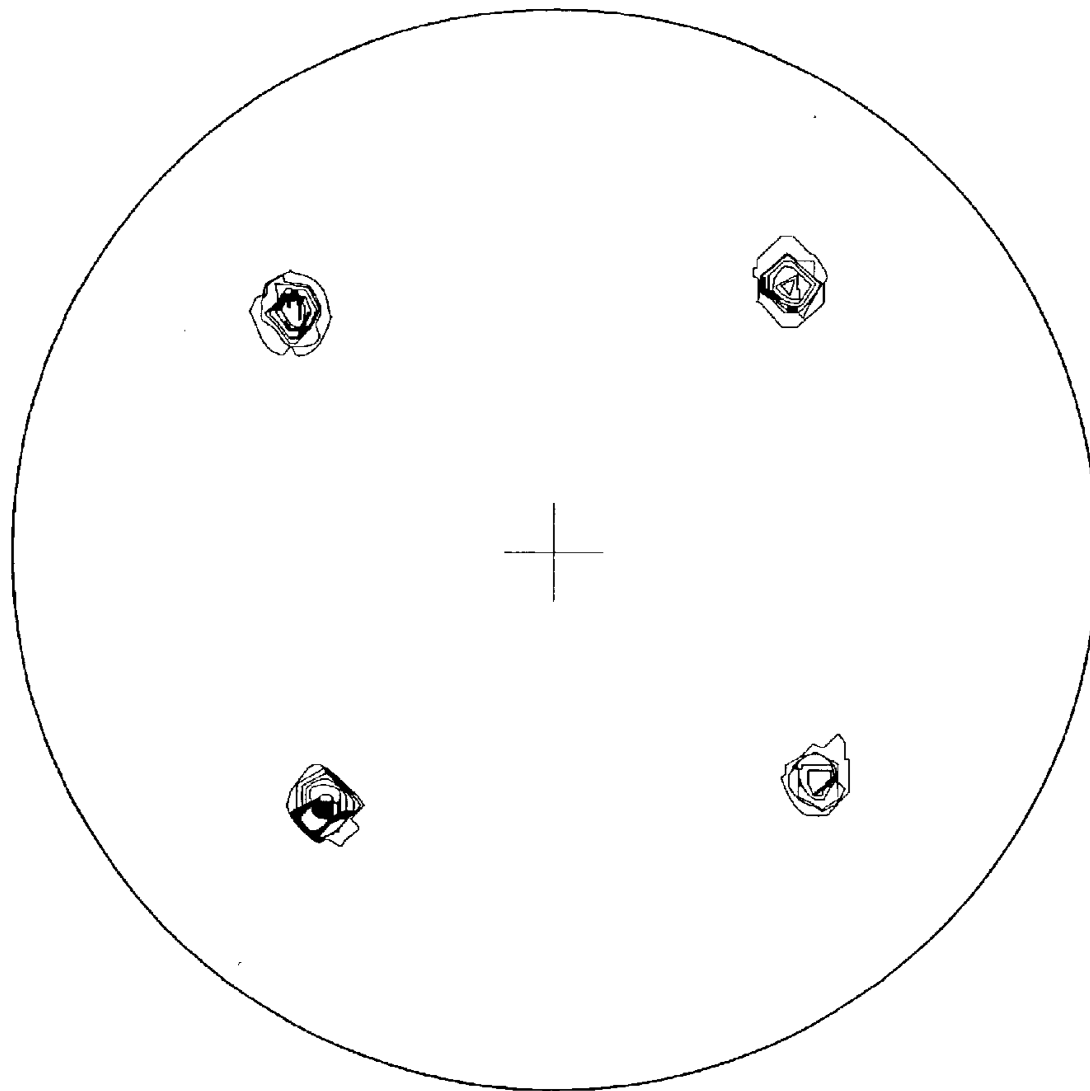
Ni-9at%W-0.03at%Mg alloy Annealing Temperature = 1400°C
