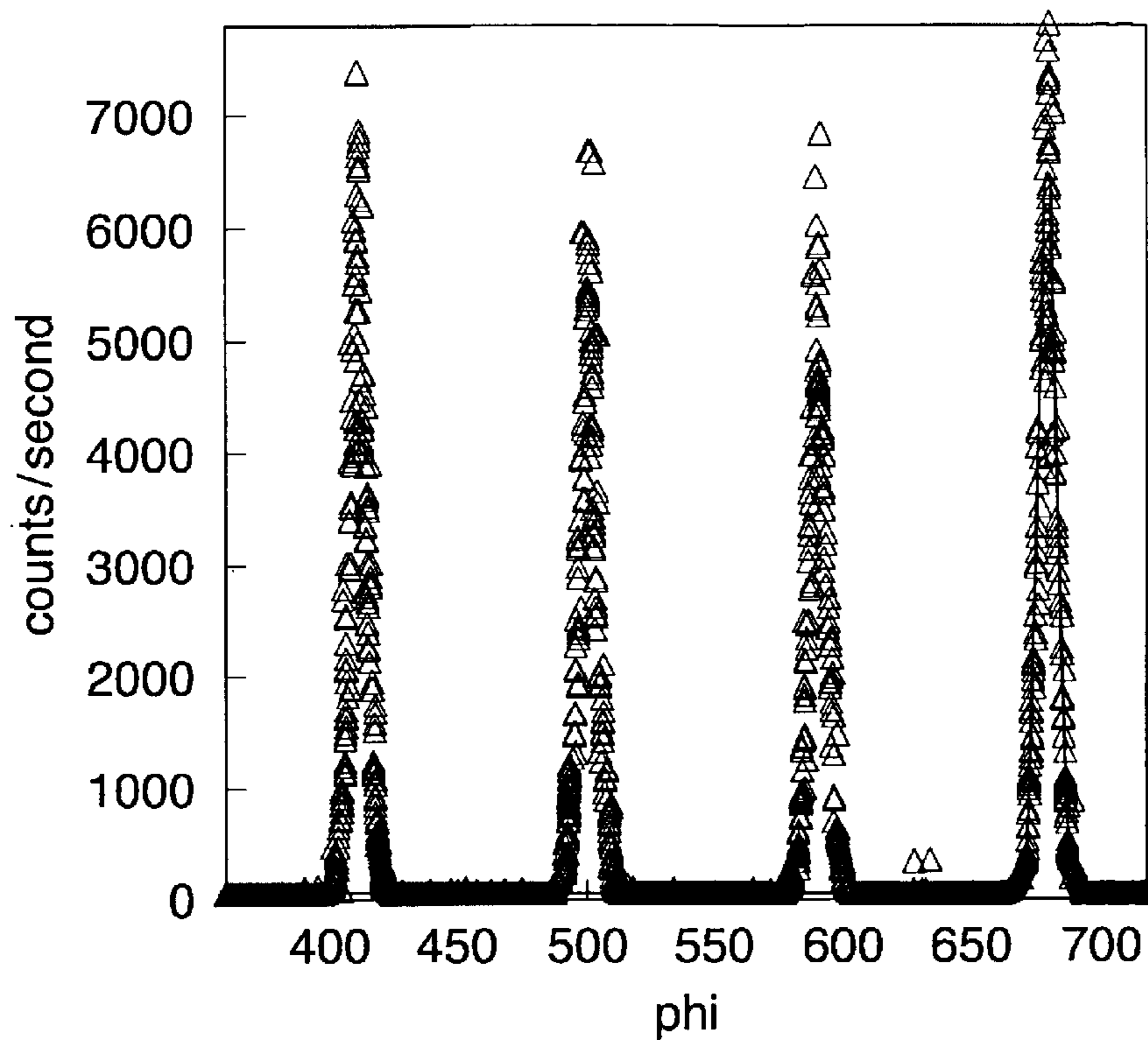
Ni-13at%Cr-0.03at%Mg alloy Annealing Temperature = 1200°C
