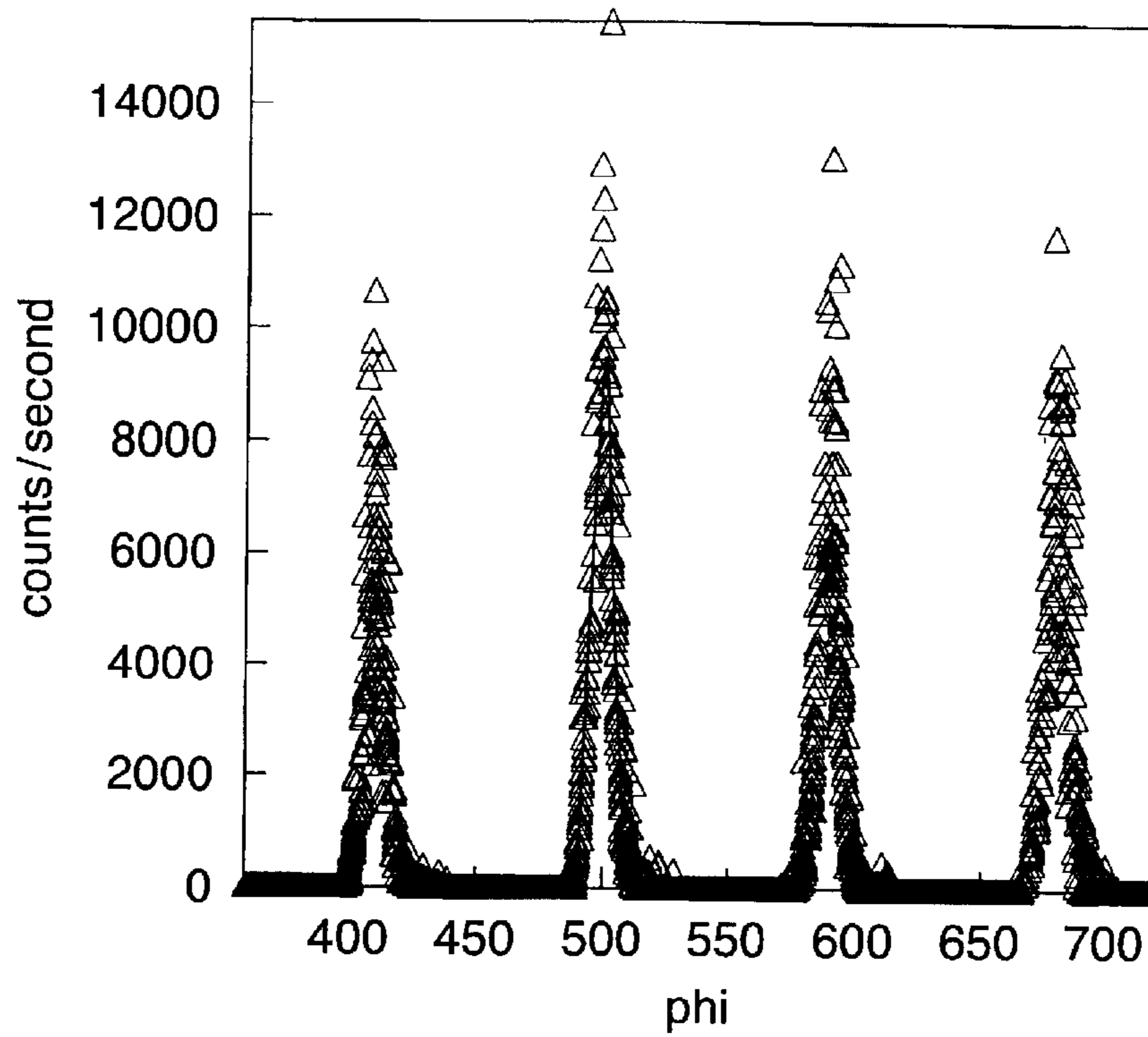
Ni-9at%W-0.03at%Mg alloy Annealing Temperature = 1200°C
