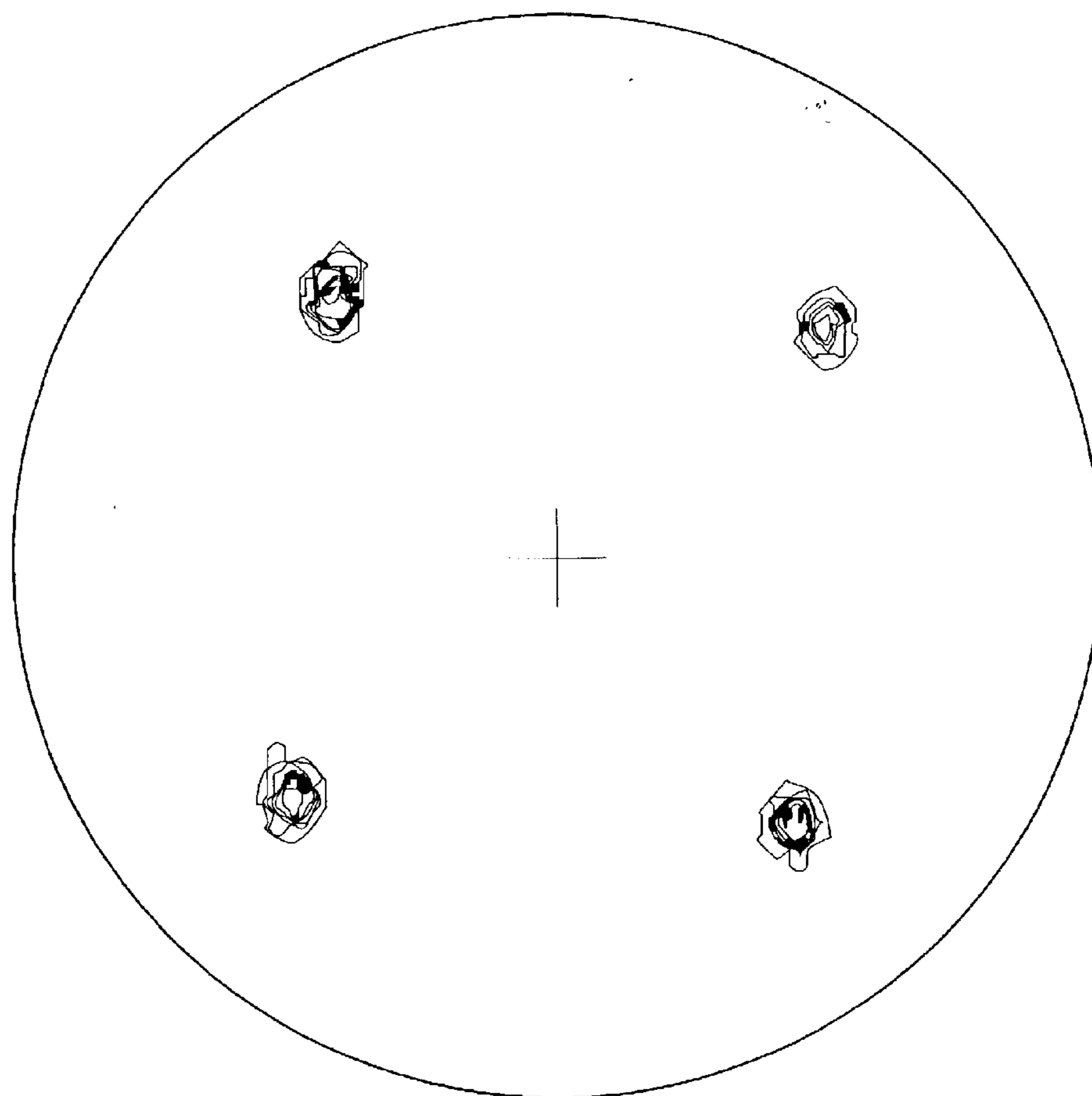
Ni-13at%Cr-0.03at%Mg alloy Annealing Temperature = 1200°C
