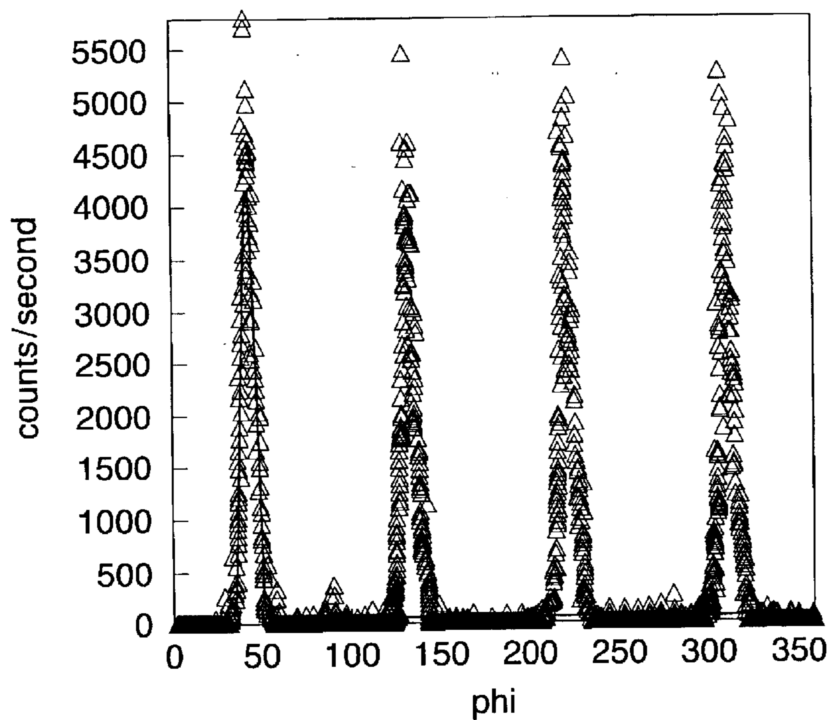
Ni-13at%Cr alloy Annealing Temperature = 1200°C
