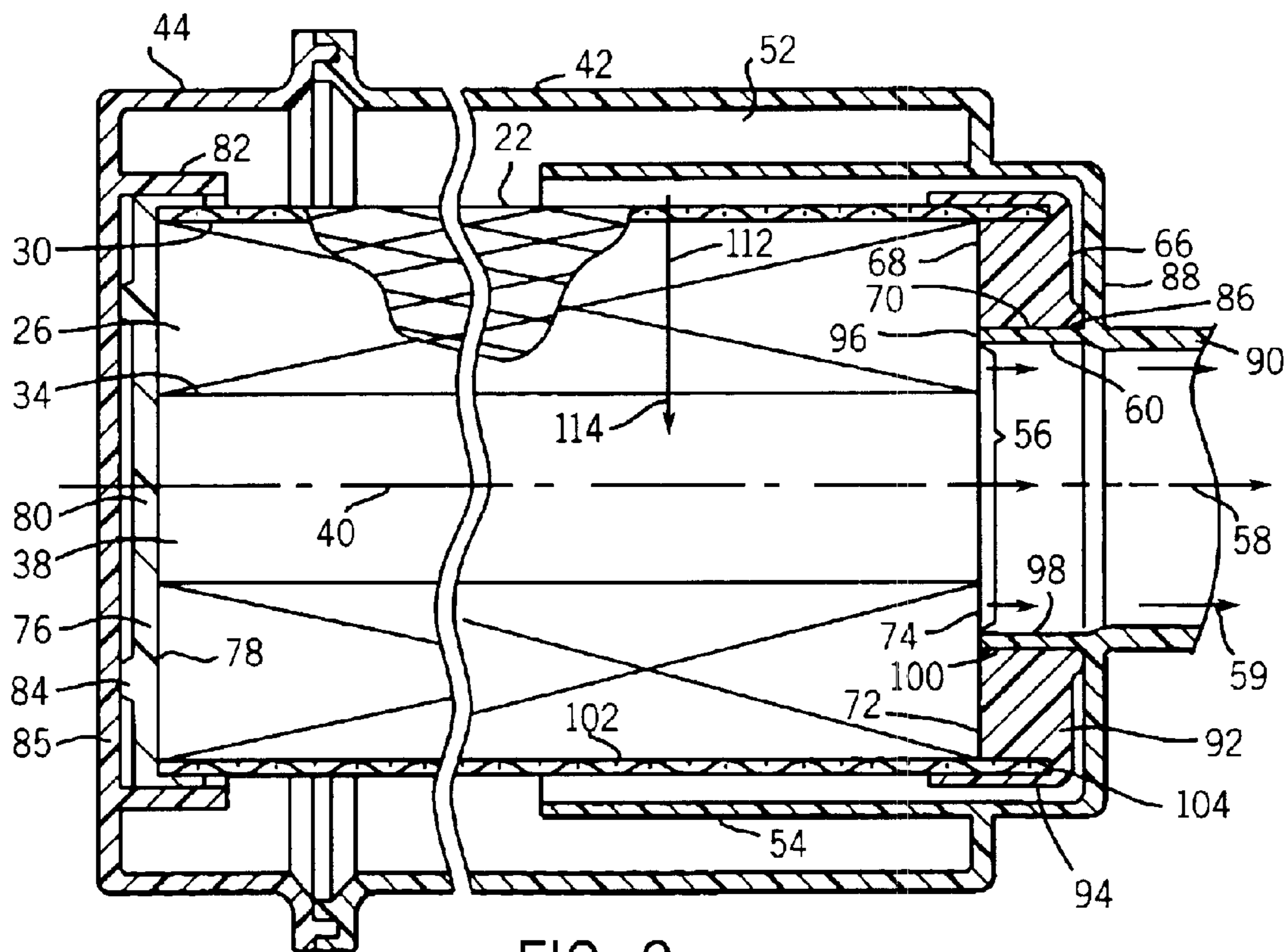
FIG. 2 PRIOR ART
