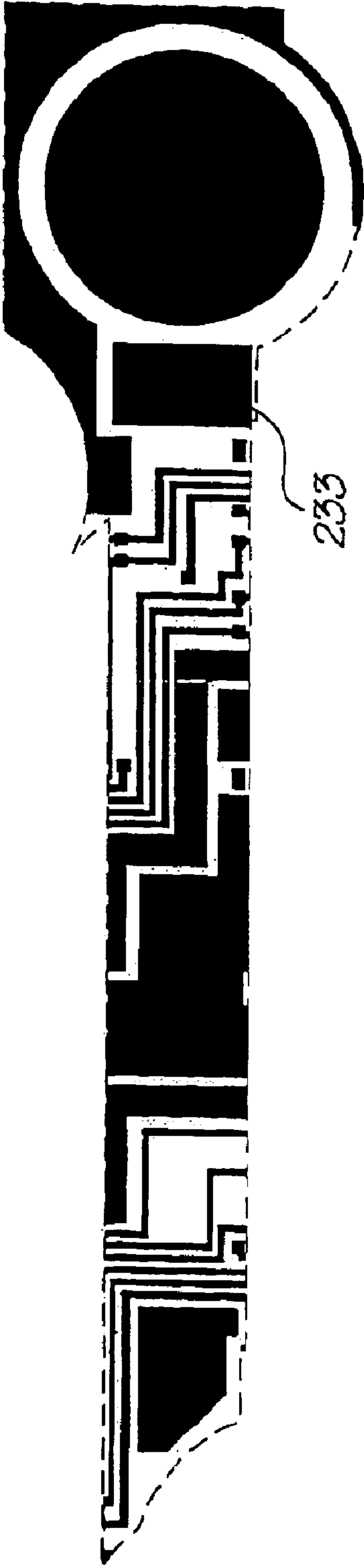
Metal 2 mask
