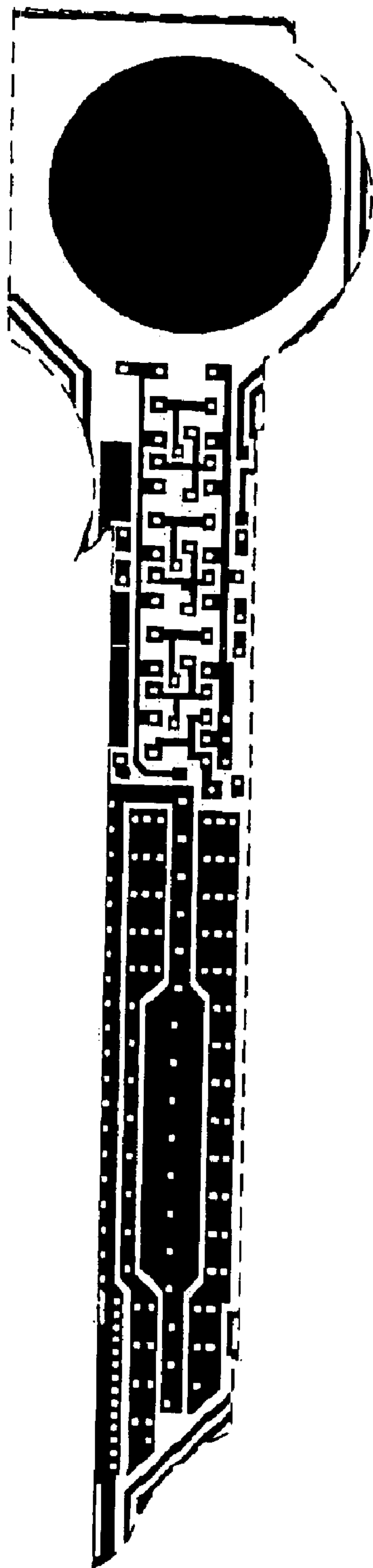
Metal 1 mask
