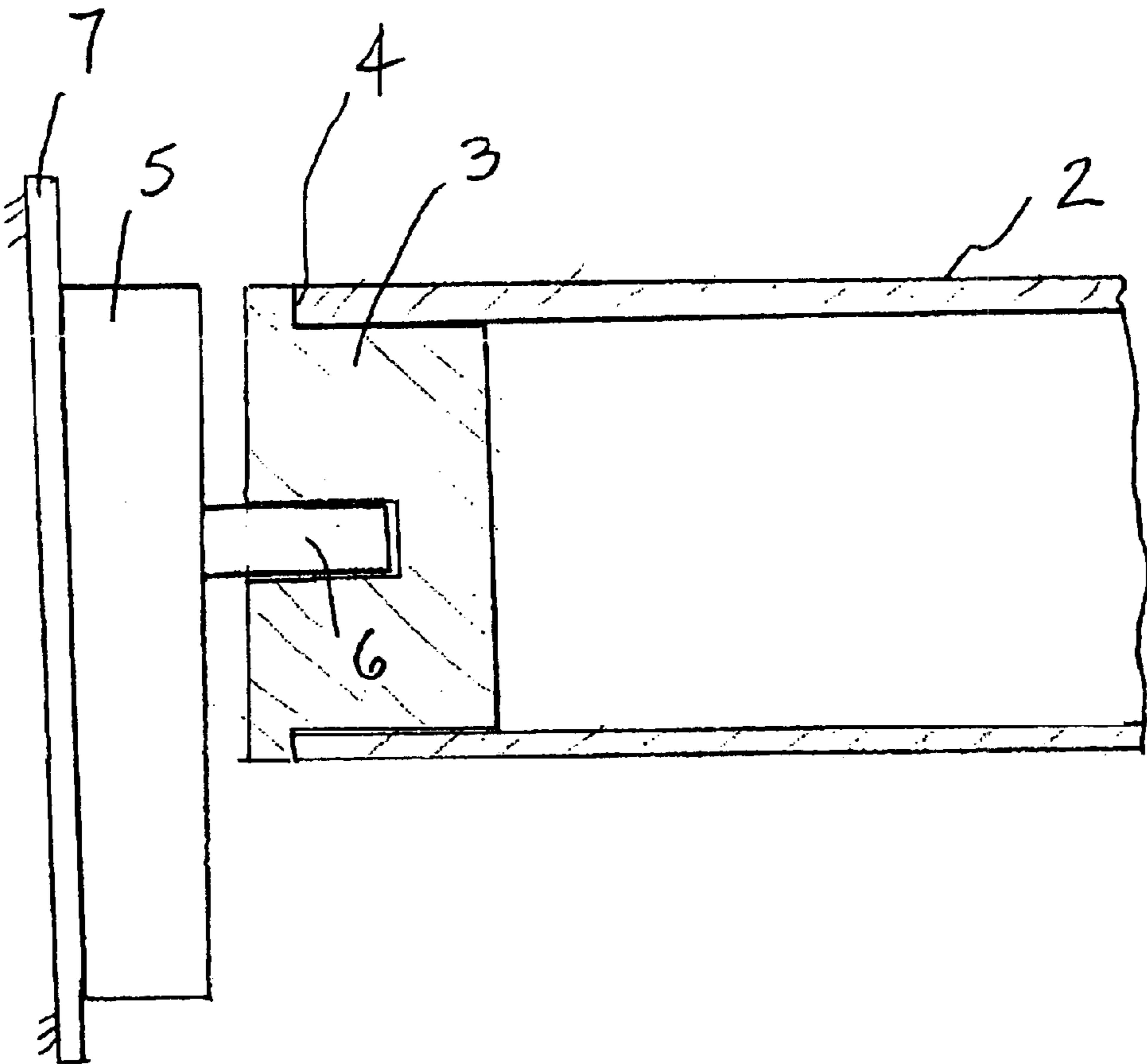
FIG. 1 (Prior Art)
