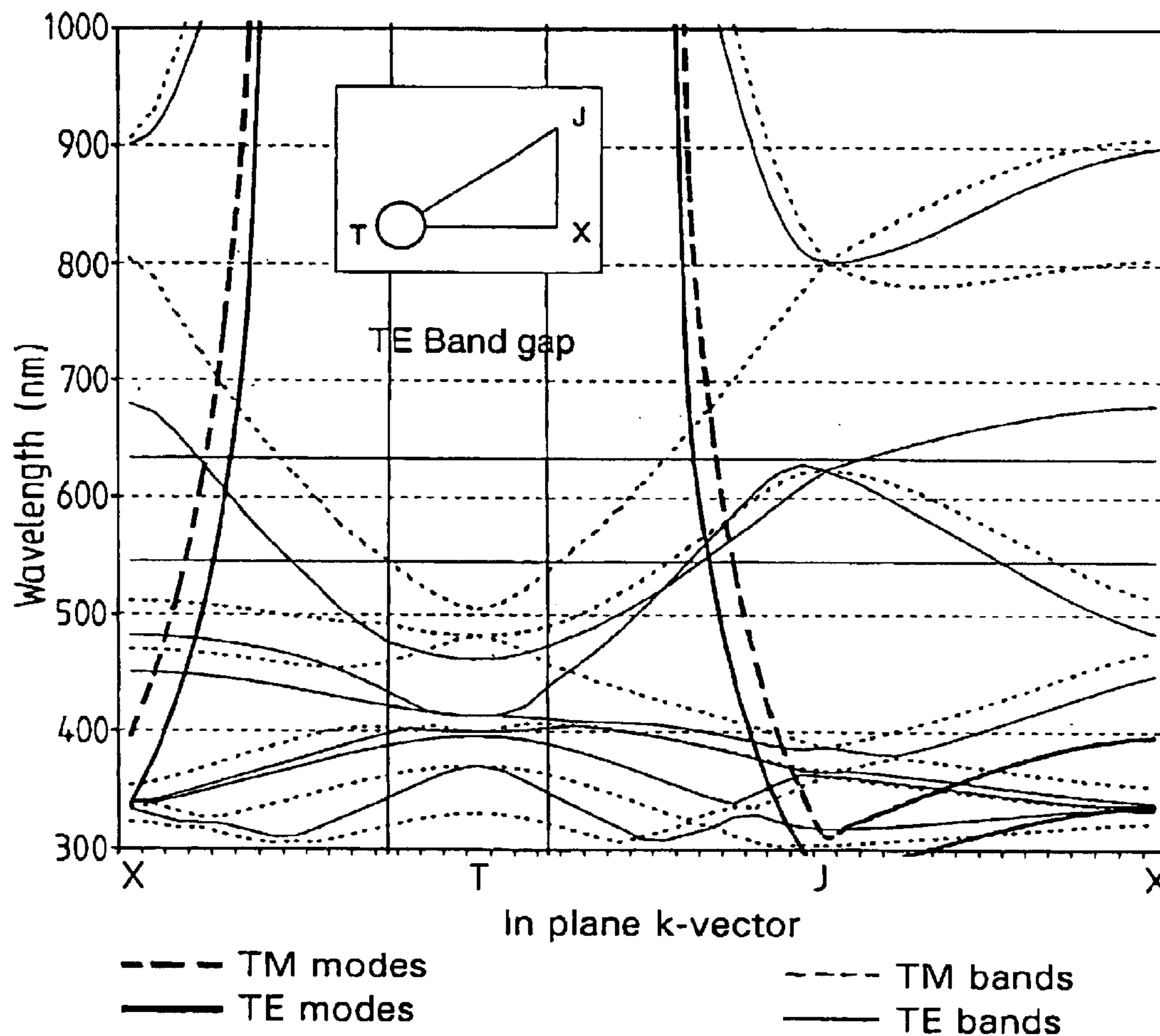
Guided modes in Nitride PBG waveguide f = 40\% , pitch = 300nm, core = 250nm, k_z = 1.2
