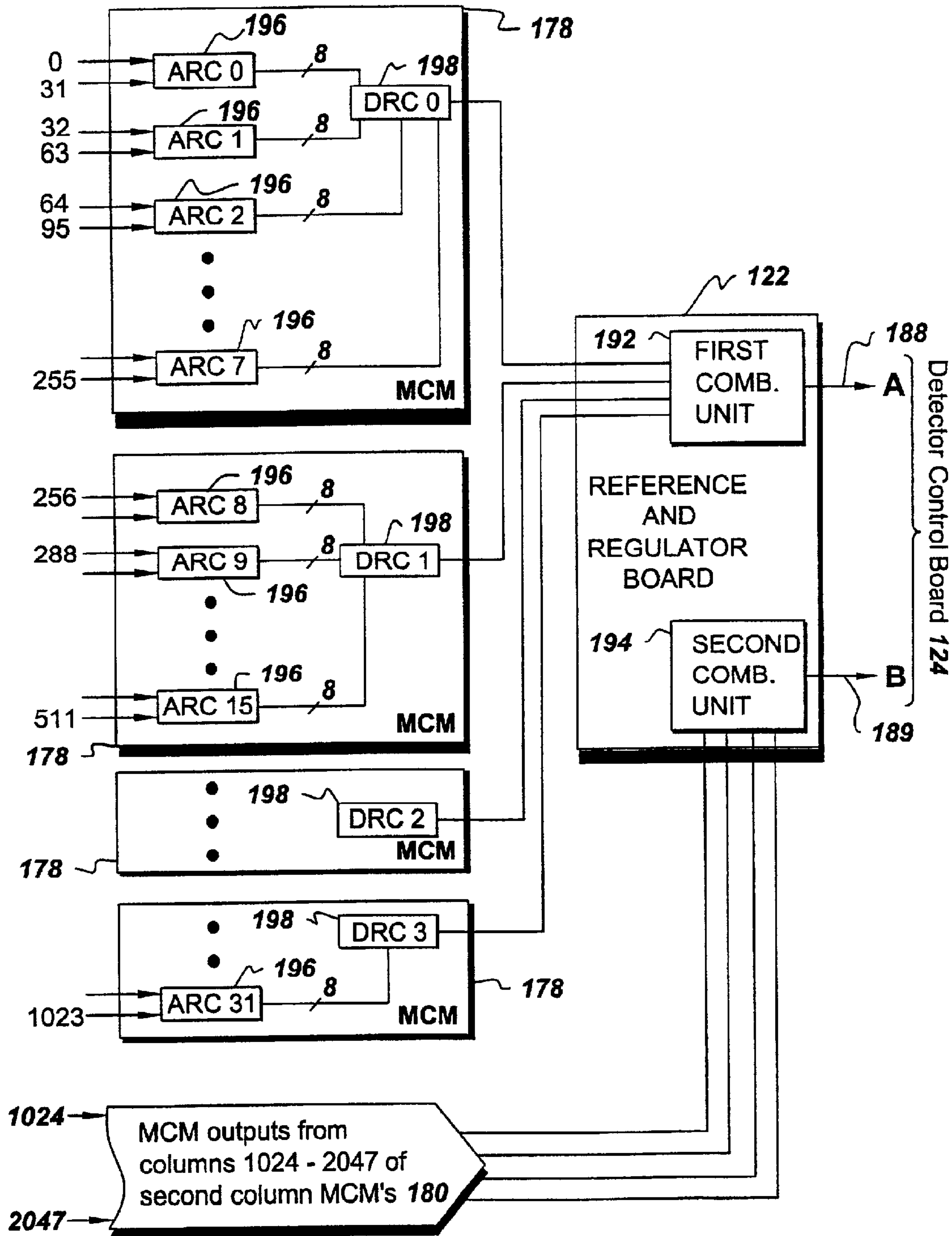
fig. 9 (PRIOR ART)
