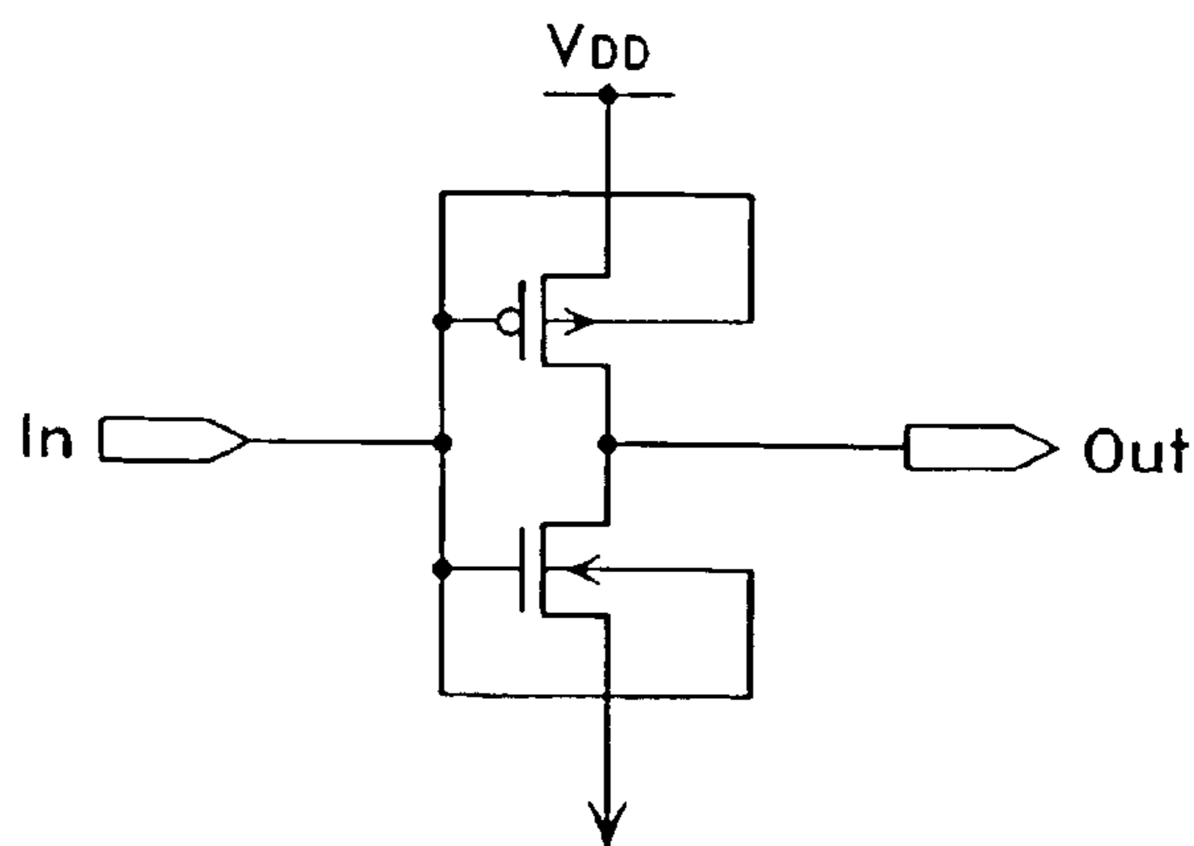
Fig. 3 (PRIOR ART)
