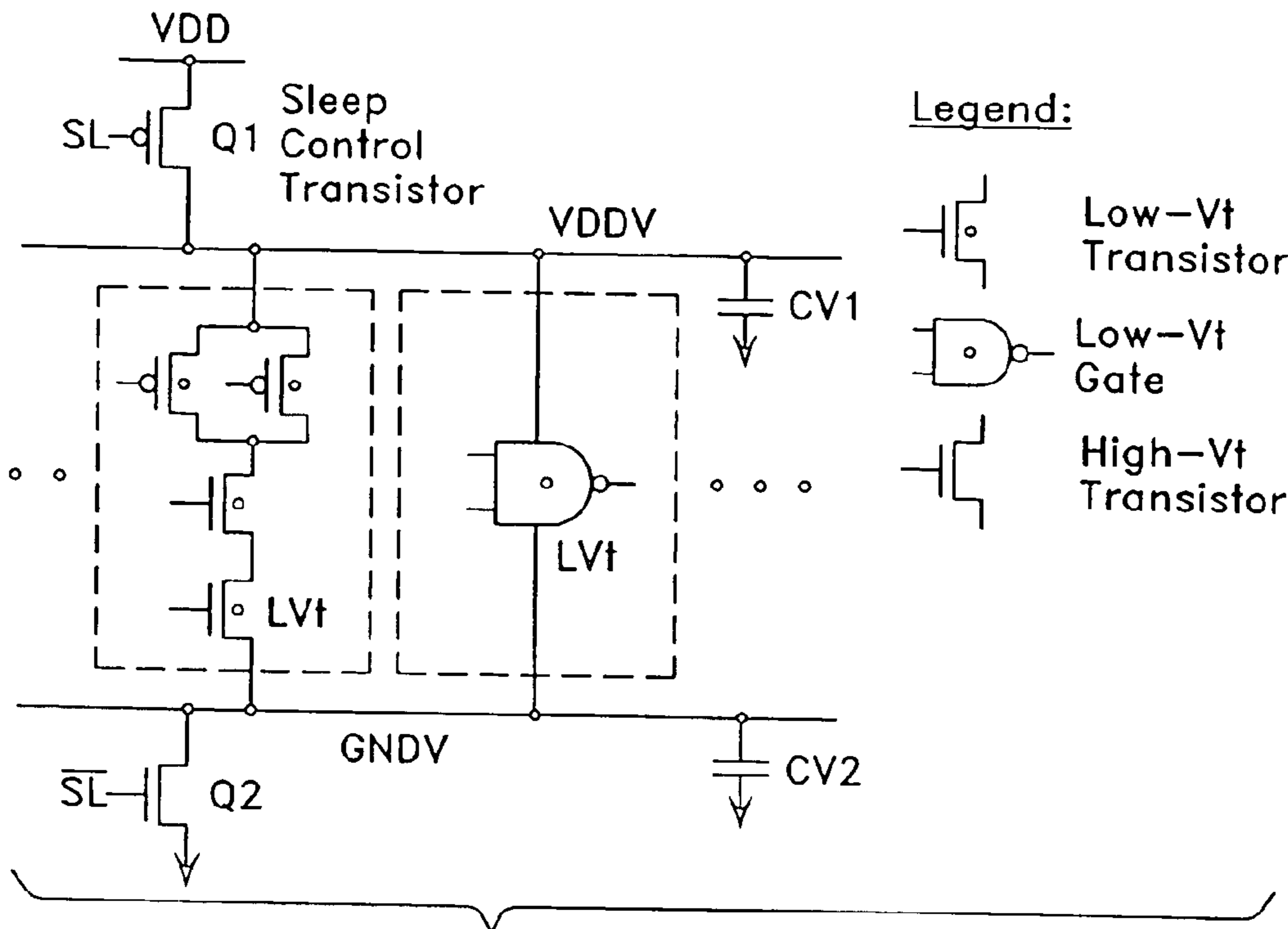
Fig. 1 (PRIOR ART)
