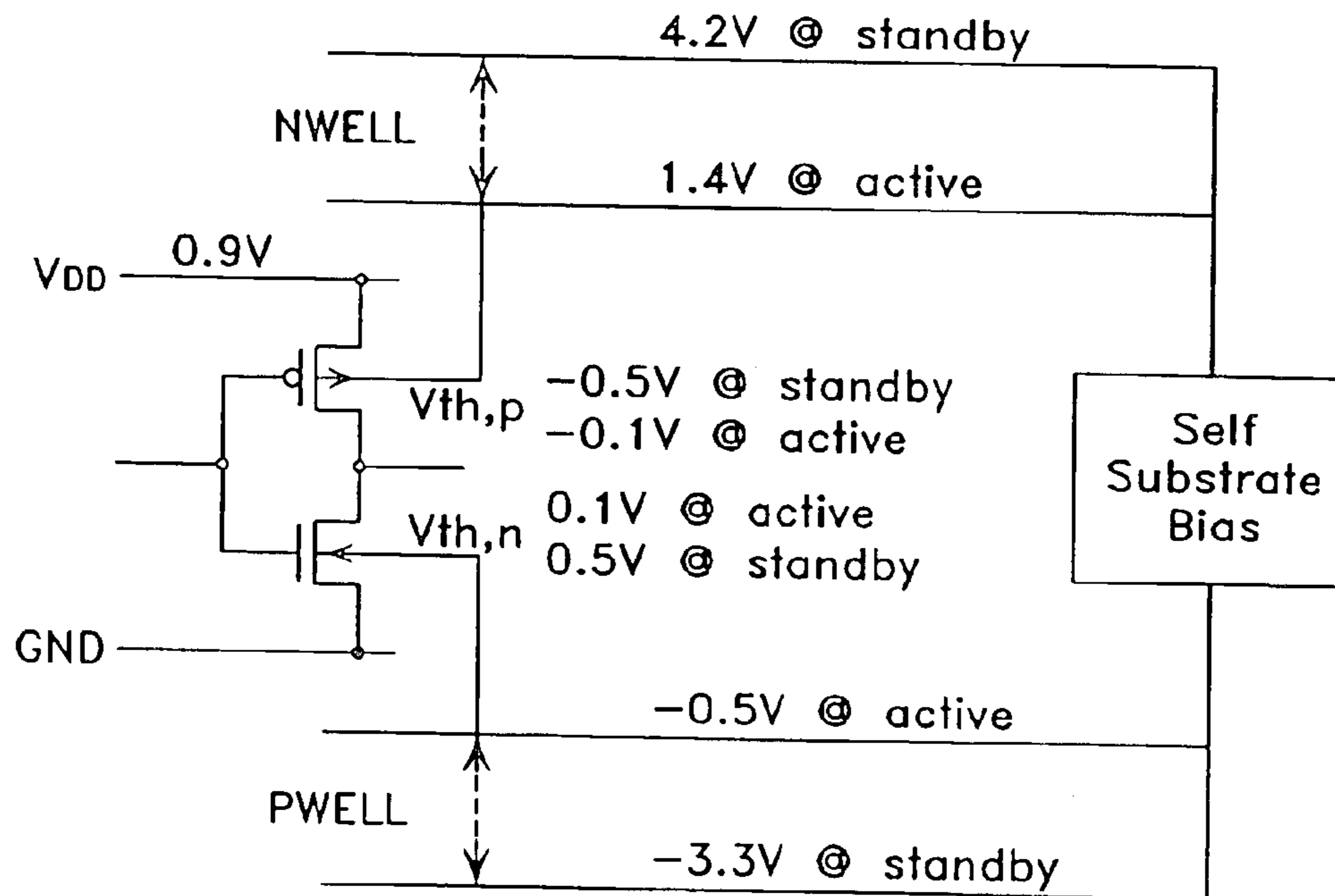
Fig. 2 (PRIOR ART)
