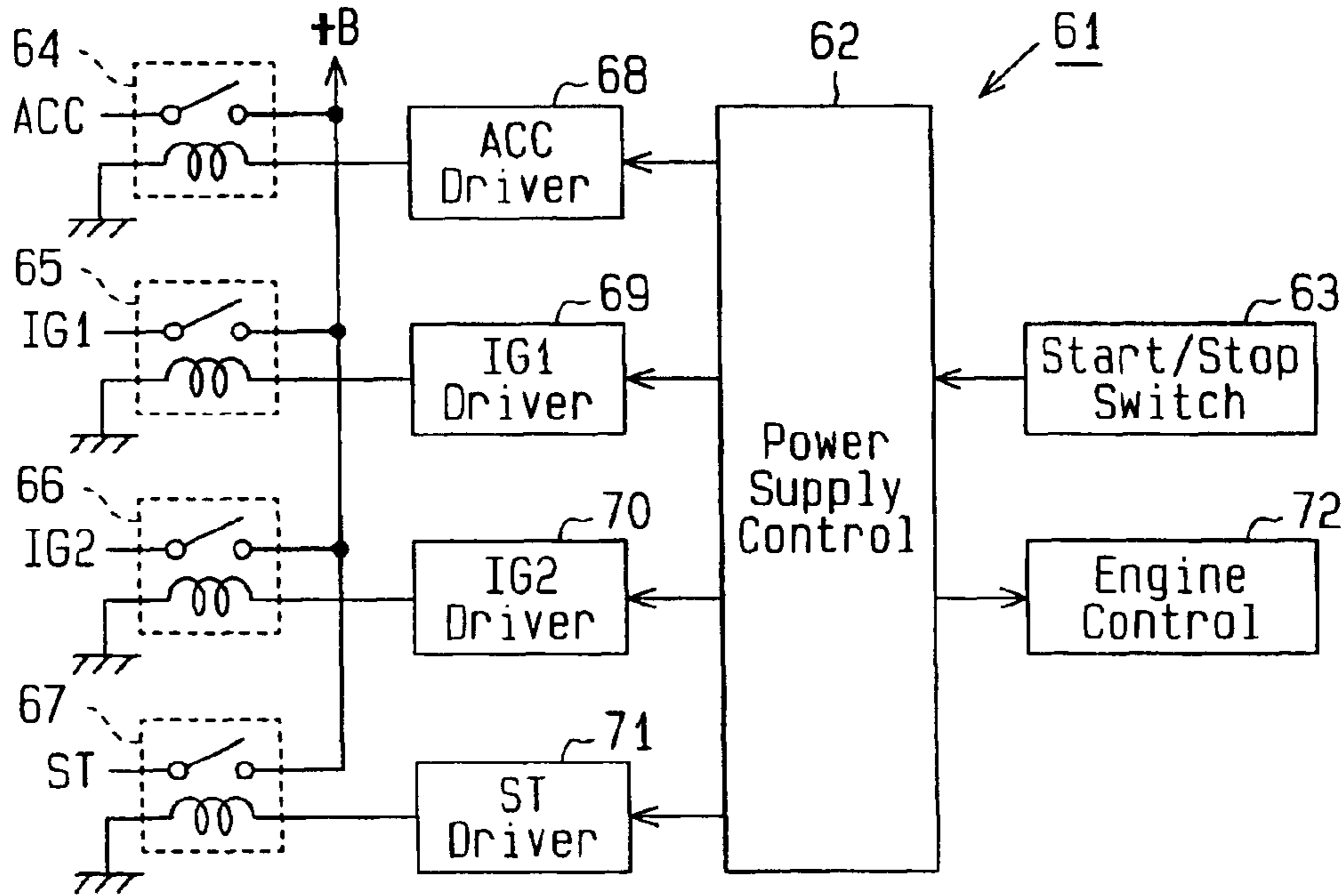
Fig. 6 (Prior Art)
