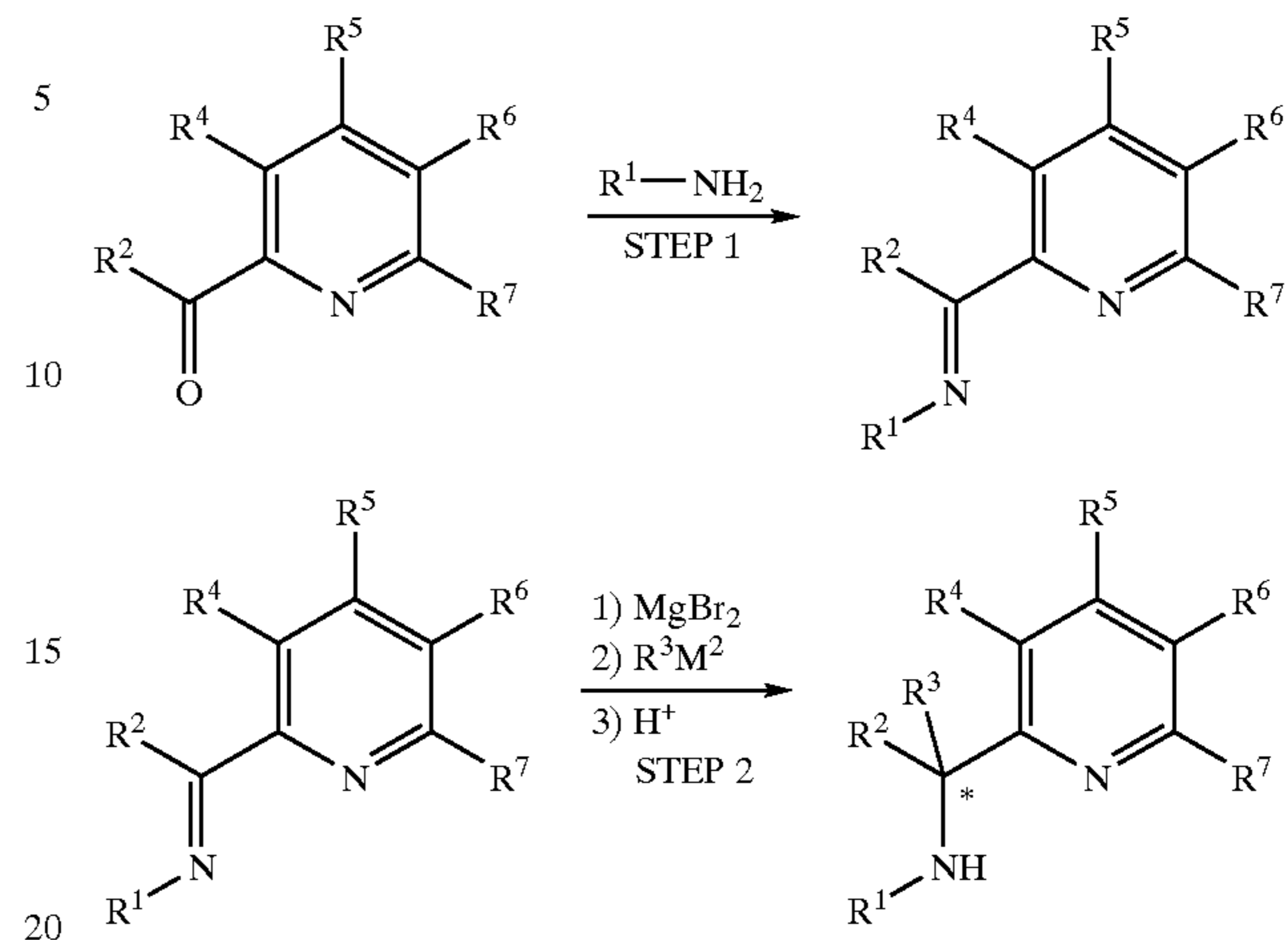
Scheme 1
