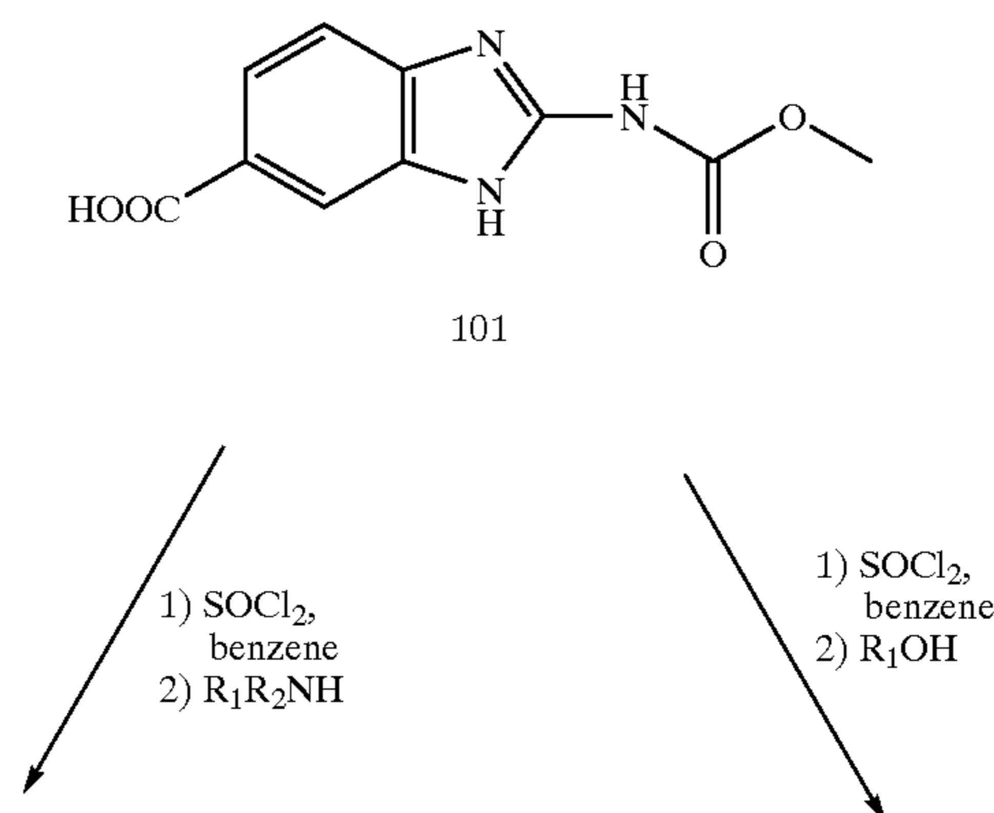
Reaction Scheme 1:
