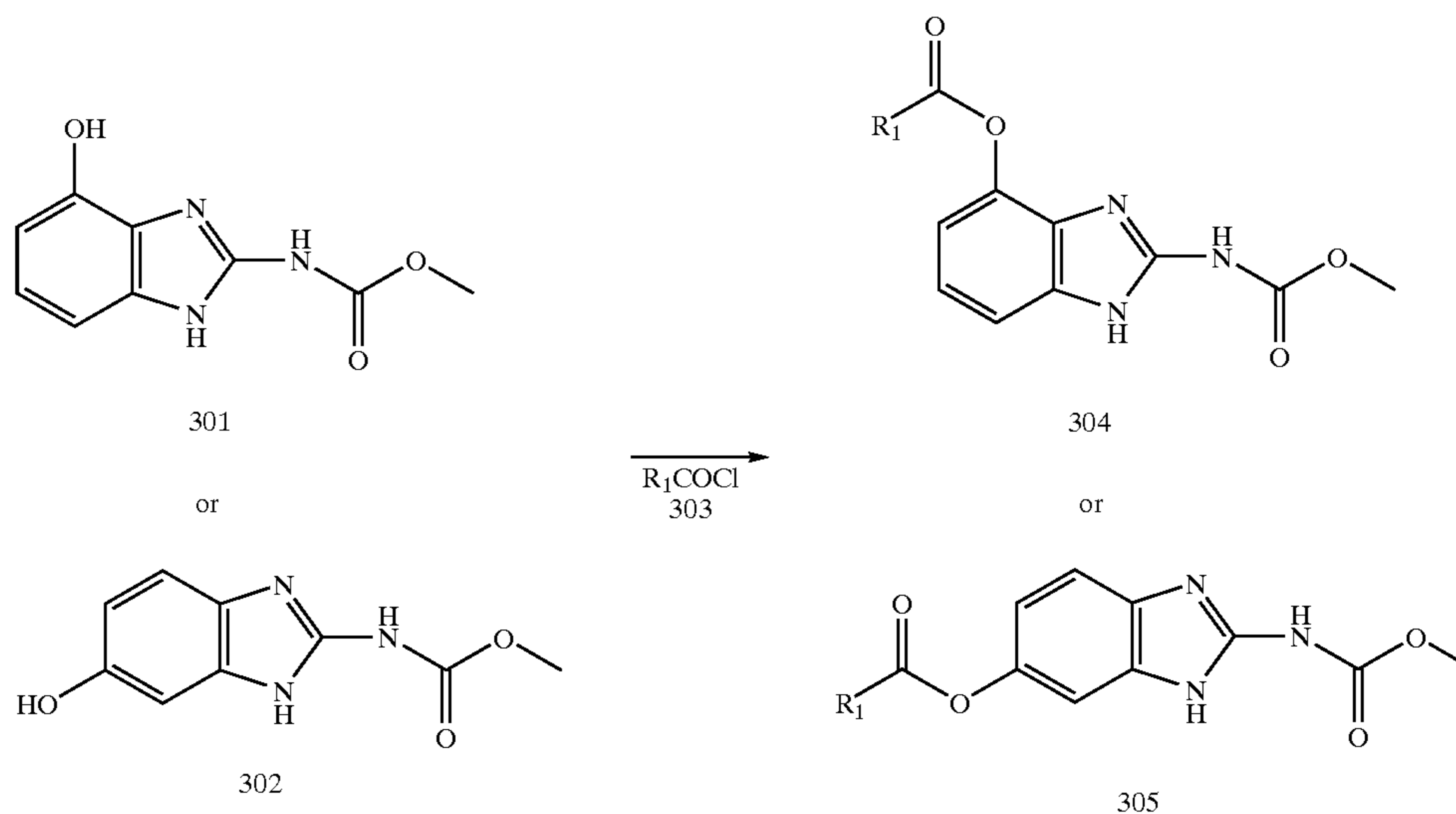
Reaction Scheme 3:
