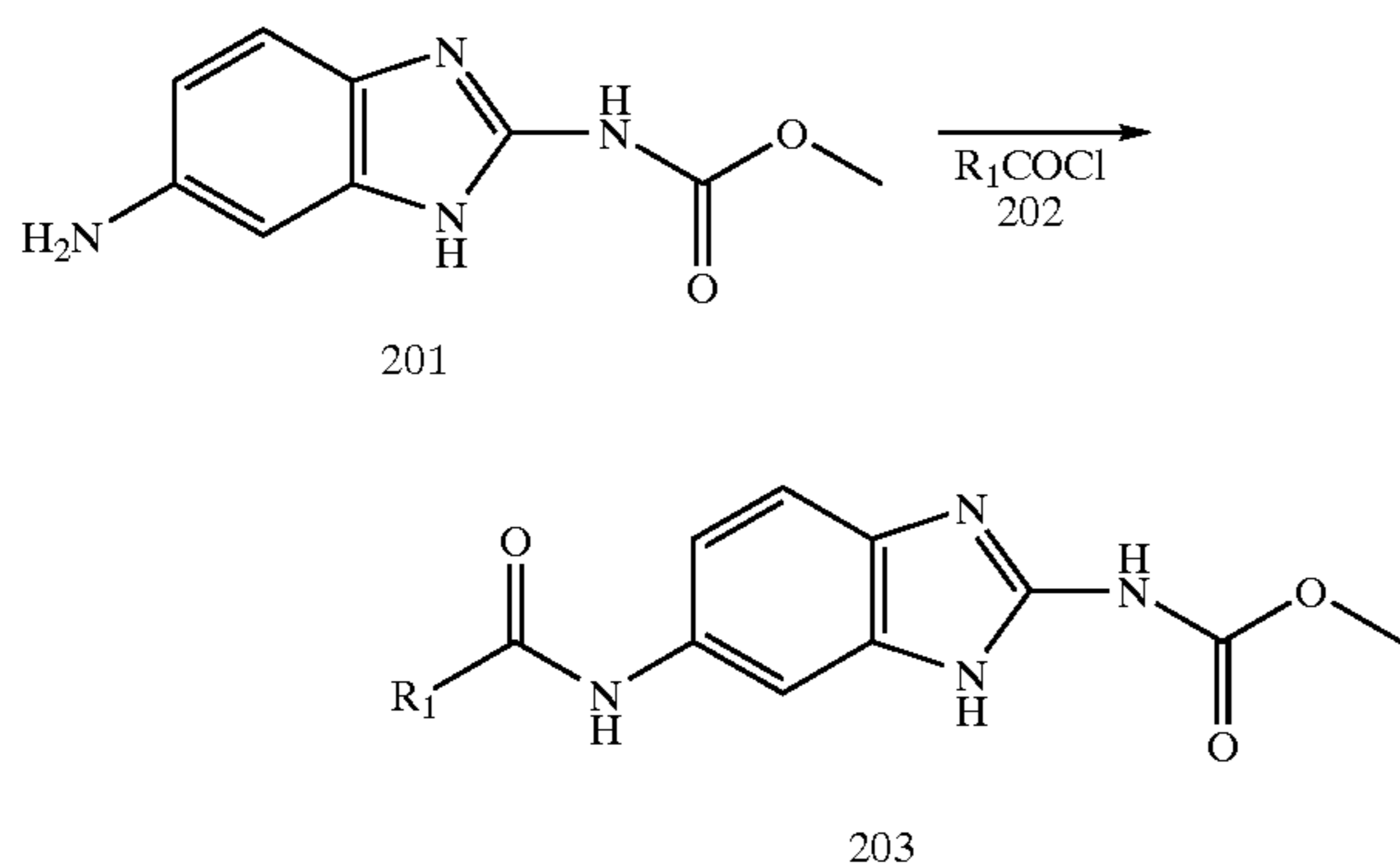
Reaction Scheme 2:
