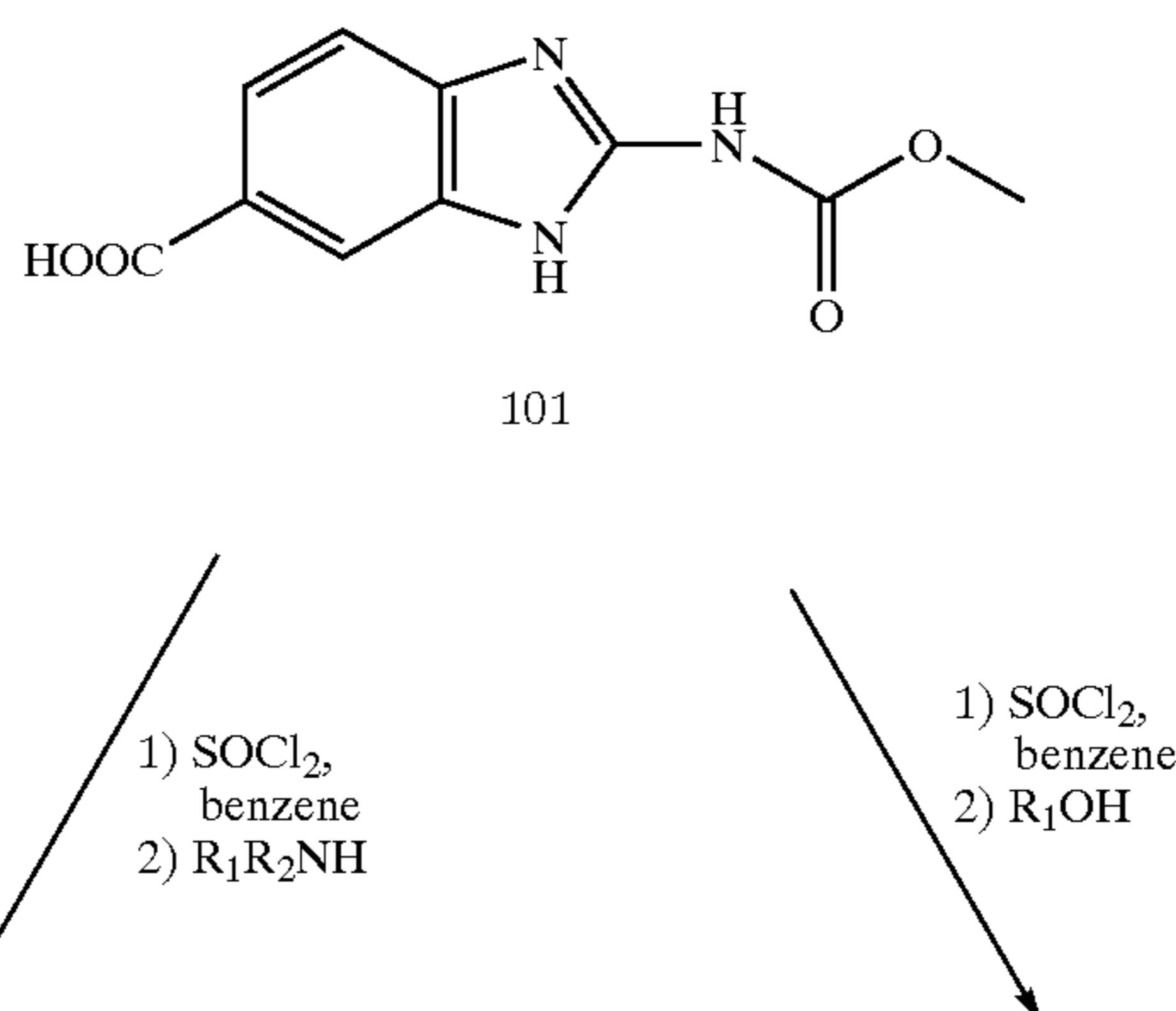
Reaction Scheme 1:
