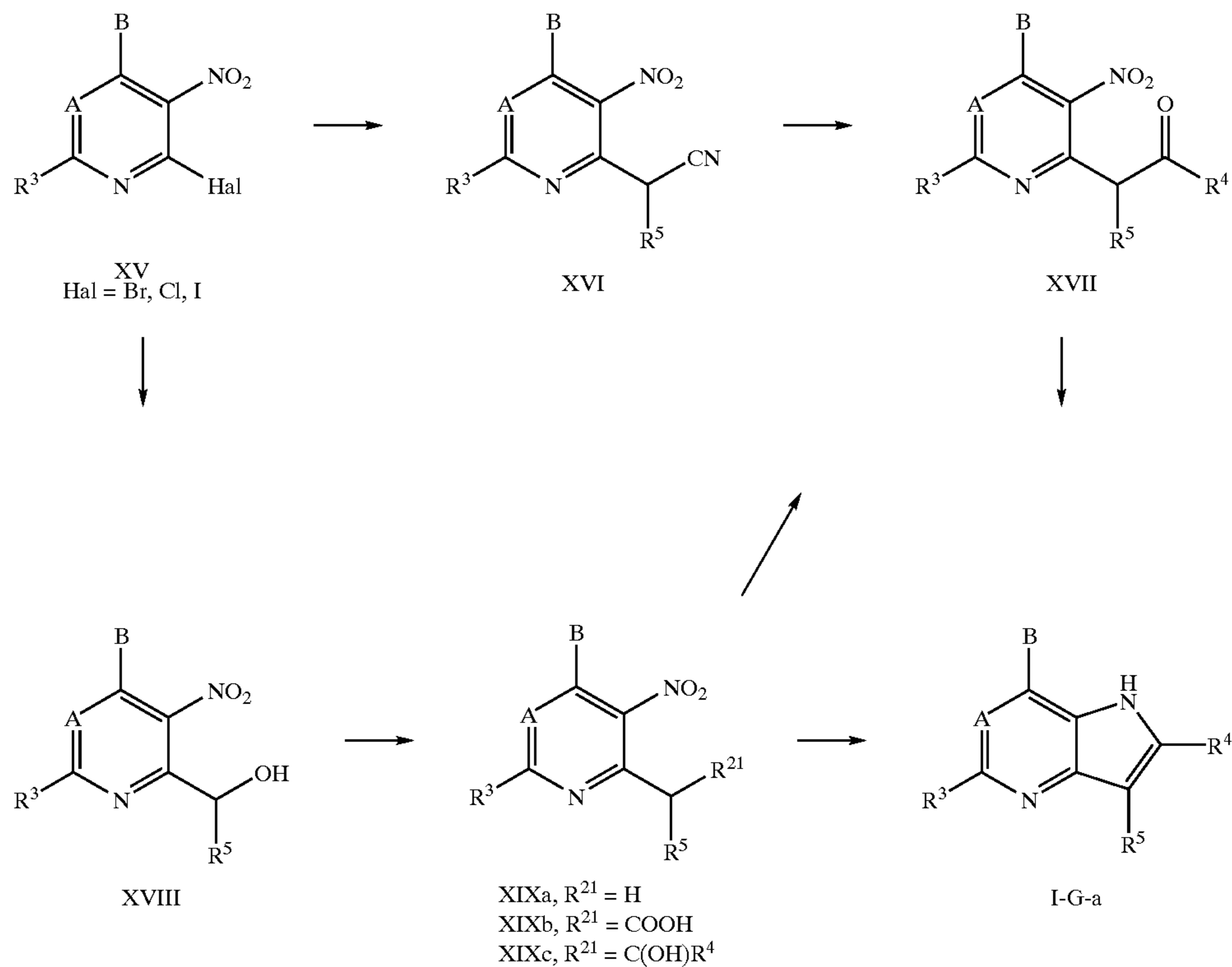
SCHEME 8
