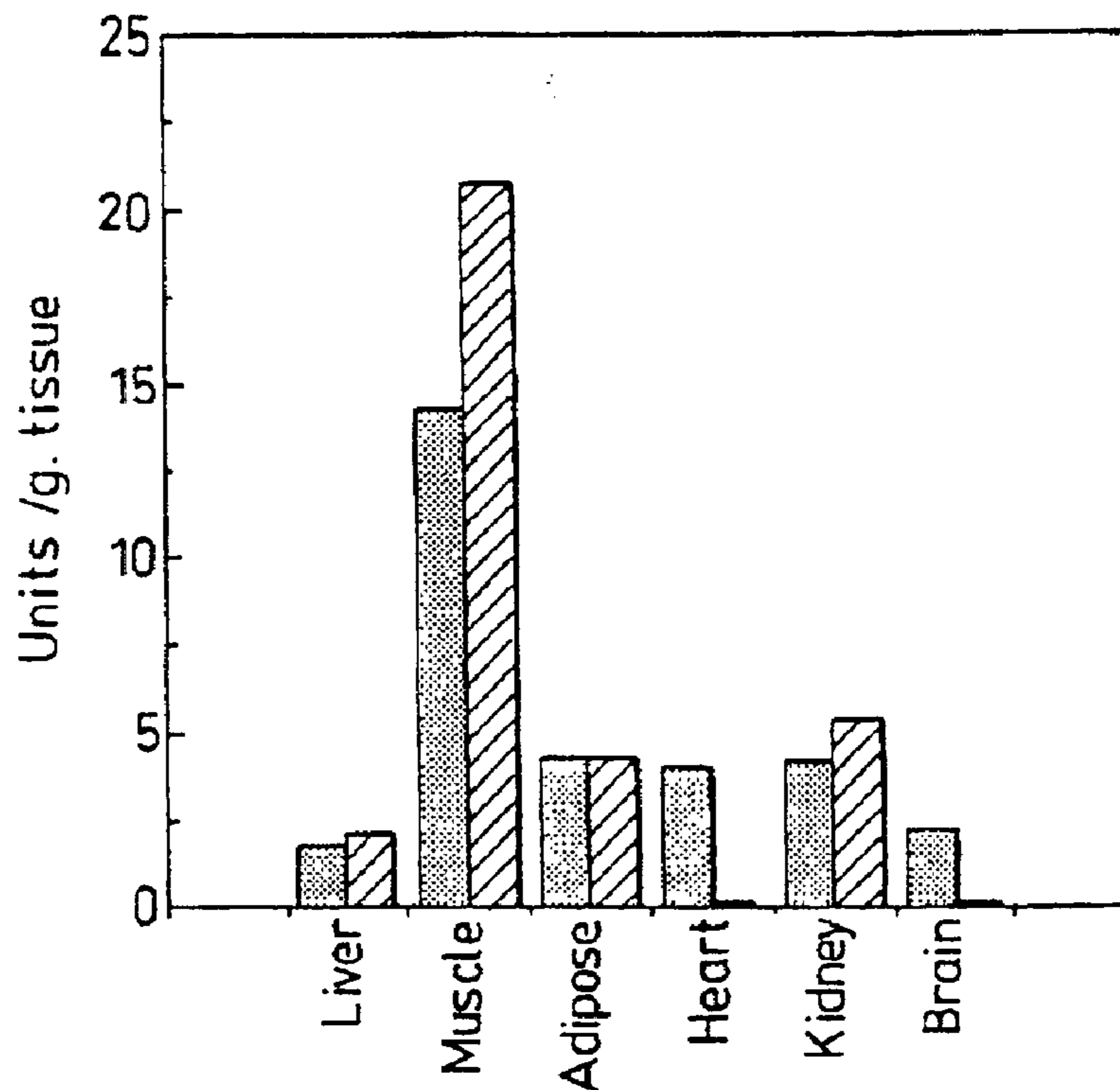
Fig. 4 (A) Lipogenesis. Adipocyte assay.
