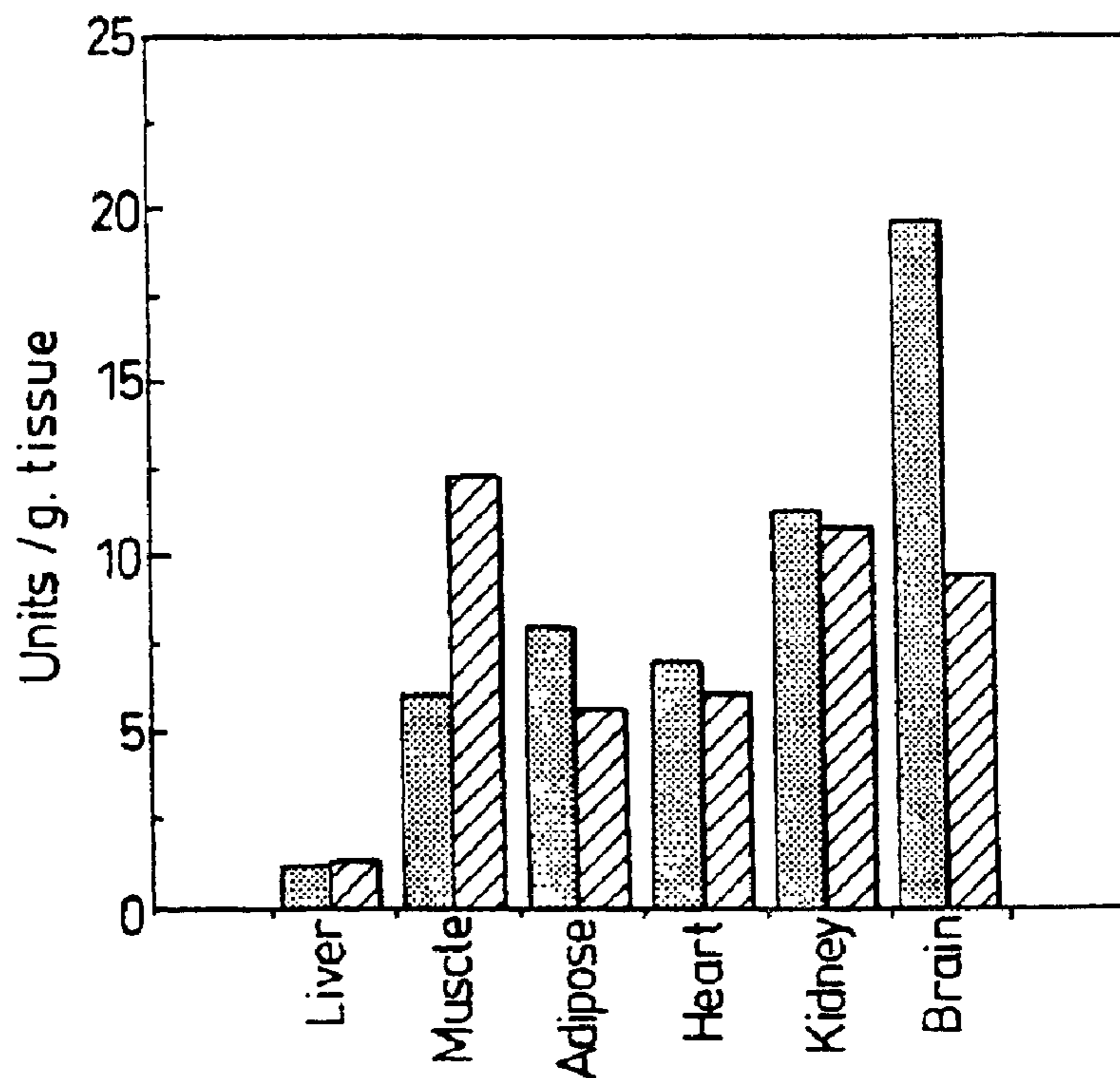
Fig. 4 (B) cAMP-dependent protein kinase-A assay
