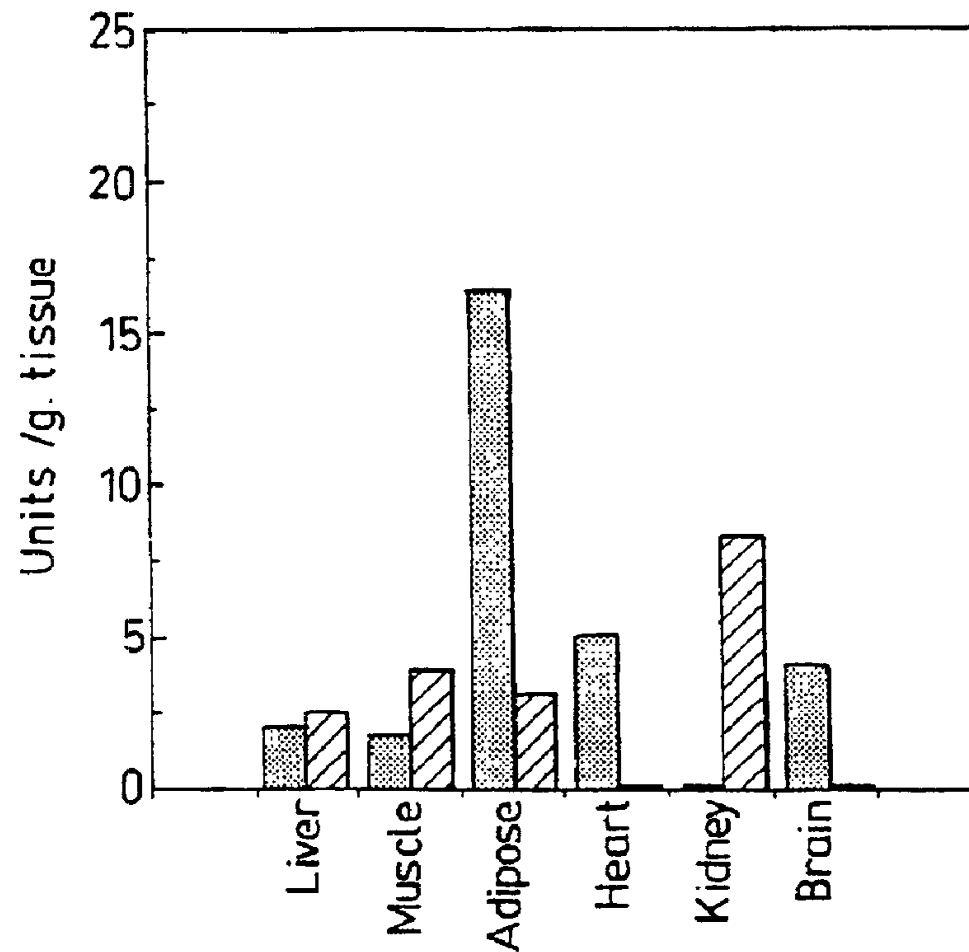
Fig. 4 (C) PDH phosphatase assay
