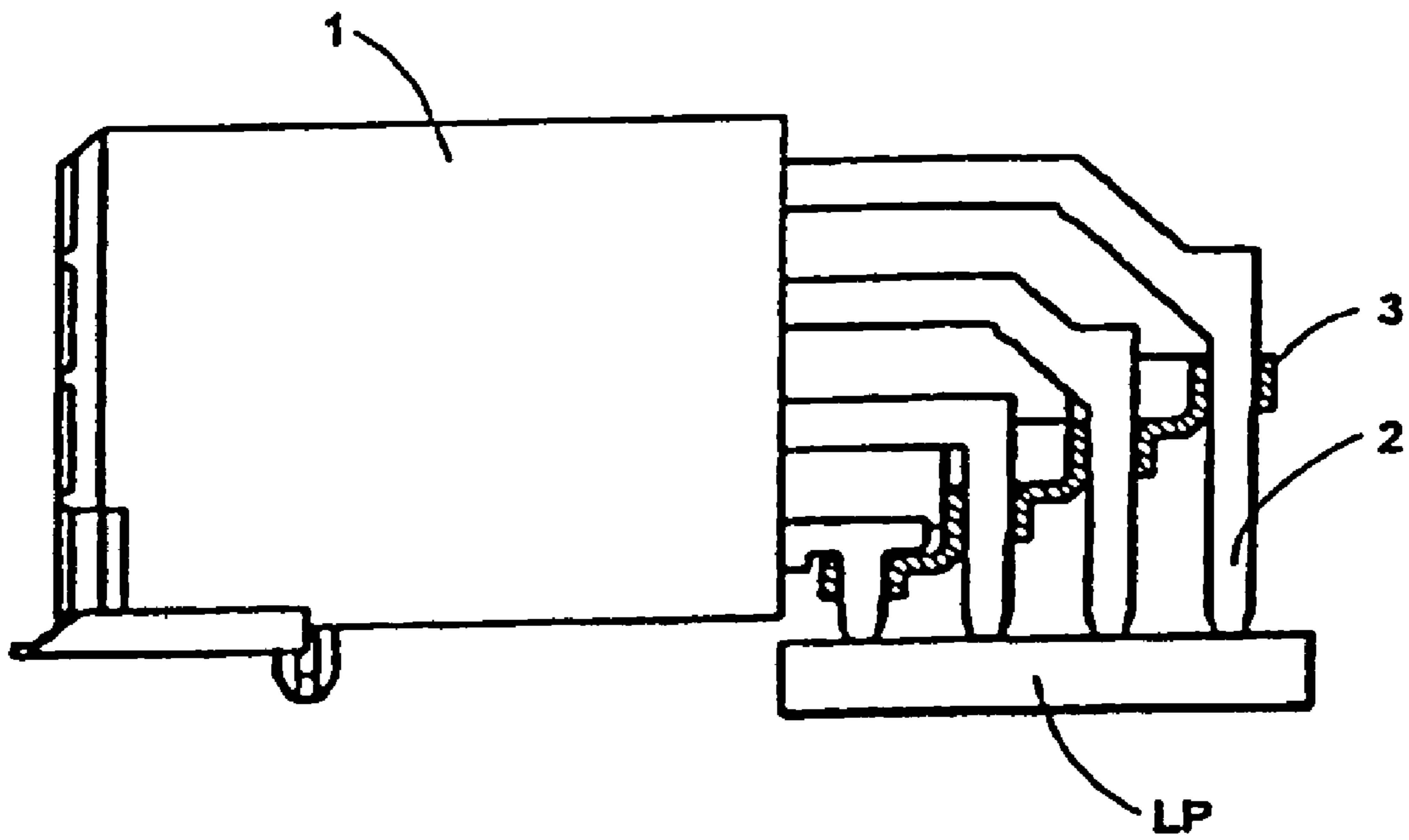
FIG 5 (PRIOR ART)
